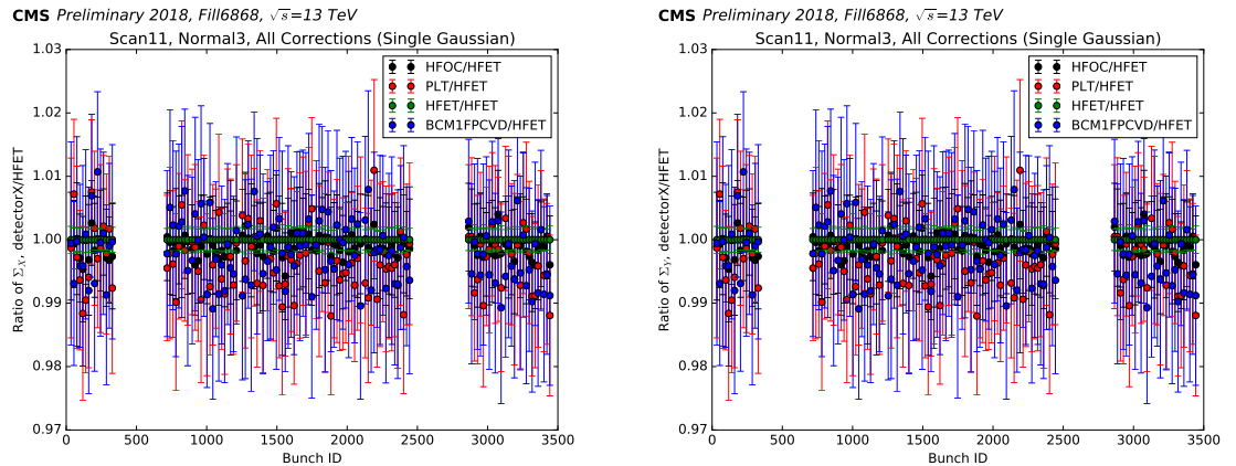
Figure 9.3: Ratio of \Sigma_x (left) and \Sigma_y (right) for each bunch crossing in a normal vdM scan pair (norm3) for each of the online luminometers (HFET, HFOC, PLT, BCM1F) to \Sigma_{x,y} of HFET.
