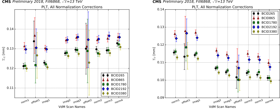
Figure 9.1: The convoluted beam width measured by PLT in the x (left) and y (right) dimension ( \Sigma_x and \Sigma_y ) after all normalization corrections have applied for the five bunch crossings with PCC data available. The uncertainty shown is statistical.
