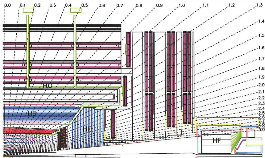
Figure 19. Layout of the CMS HCAL showing the locations of the hadron barrel (HB), endcap (HE), outer (HO), and forward (HF) calorimeter.
