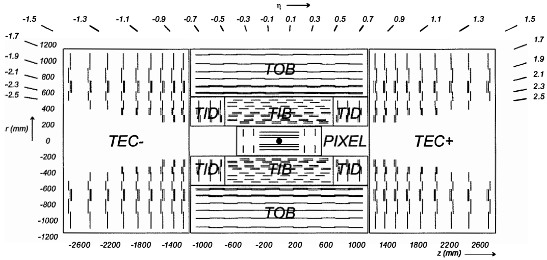
Figure 16. Geometrical layout of the pixel detector.
