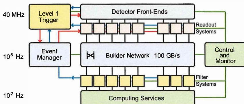
Figure 23. Architecture of the CMS DAQ system.
