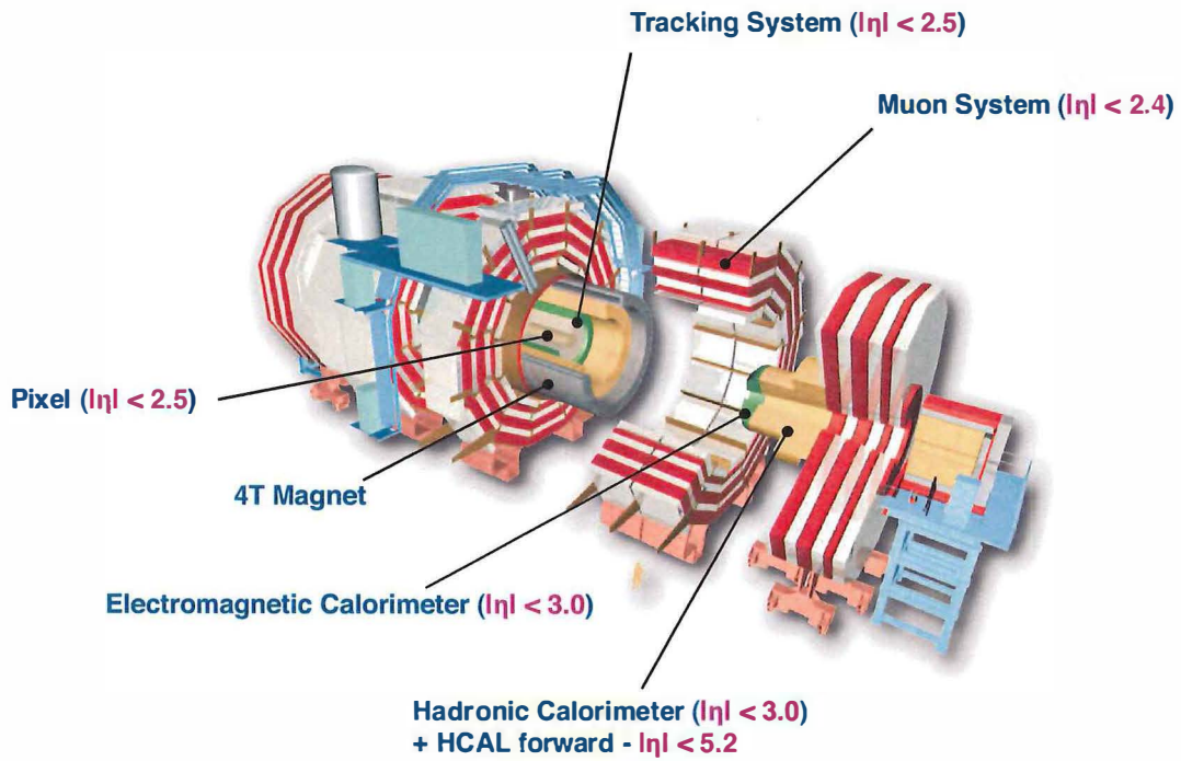
Figure 10. Schematic view of the CMS detector.
