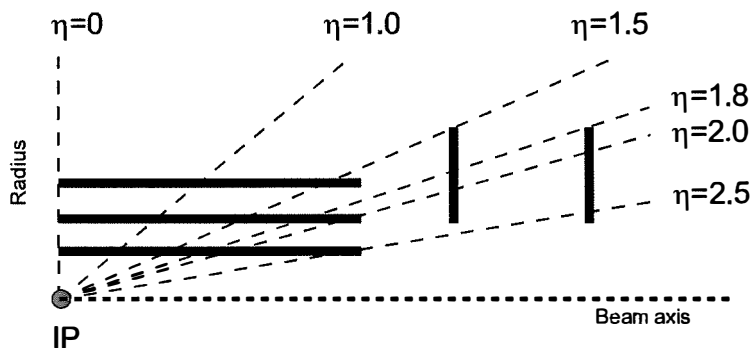
Figure 14. Geometrical layout of the pixel detector.
