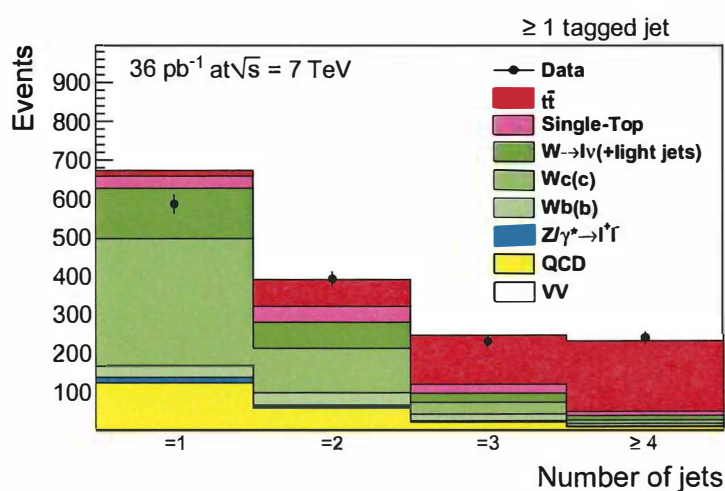
Figure 48. Number of events with at least 1 tag for data and MC samples for each jet multiplicity bin. QCD normalization in each bin is taken from the Matrix Method prediction before tagging. W +jets normalization is also taken from the Matrix Method for events with 1 and 2 jets, and from the Berends' scaling for higher jet multiplicity bins. In this plot, the Wb(b) and Wc(c) contributions were scaled by a heavy flavor scale factor W_{HF} = 2 .
