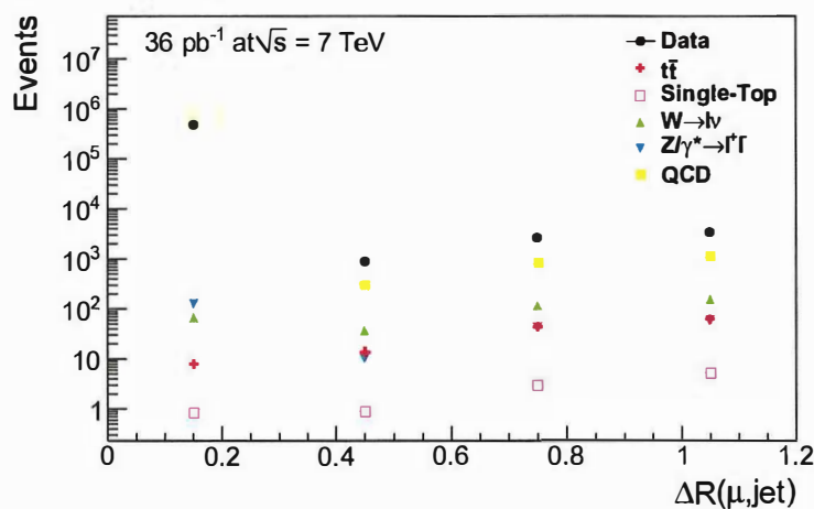
Figure 36. The distribution of \Delta R(\mu, jet) for different samples. The events passed the selection cuts regarding the primary vertex, the Global and Tracker Muon and all the muon selection cuts, except the \Delta R(\mu, jet) . Most of the data events with low \Delta R(\mu, jet) (corresponding to the first bin) are QCD events.
