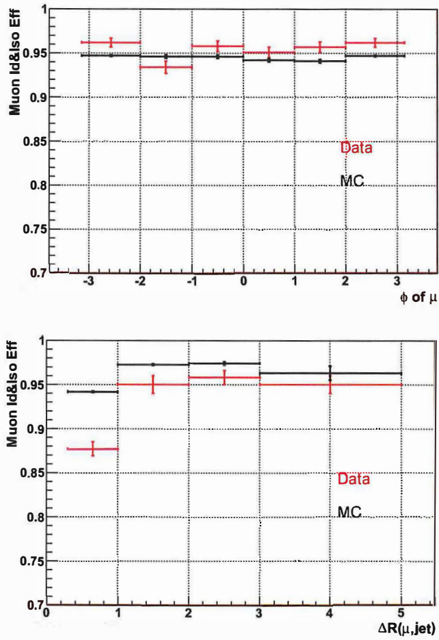
Figure 39. Muon ID and ISO efficiencies as functions of \phi^\mu (top) and the distance between the muon and the closest jet \Delta R(\mu, jet) (bottom).
