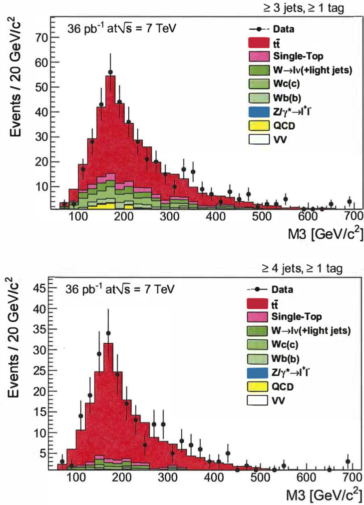
Figure 49. M_3 of the leading jet distributions for the events with \geq 3 jets and at least 1 tag (top) and events with \geq 4 jets and at least 1 tag (bottom). The M_3 values are obtained by taking the largest p_T from the vectorial sum of the two untagged jets and one tagged jet in each event. Only statistical uncertainties are shown.
