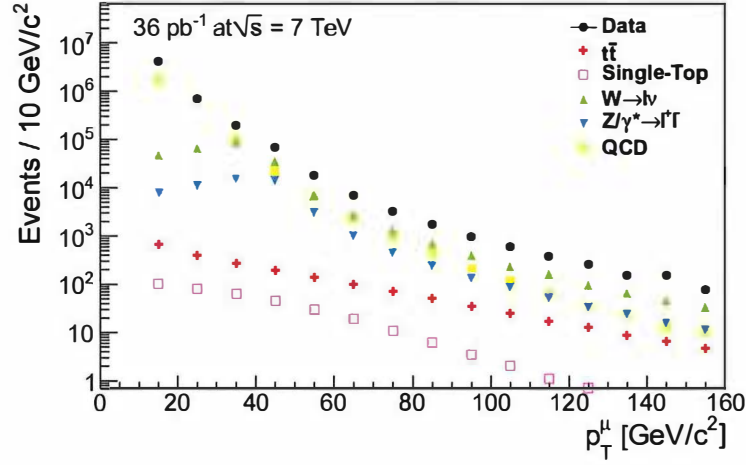
Figure 33. Transverse momentum of the muon for different samples. A preselection cut p_T^\mu > 10 \text{ GeV/c} was applied in the PAT-tuples production. The events passed the selection cuts regarding the primary vertex and the Global and Tracker Muon.
