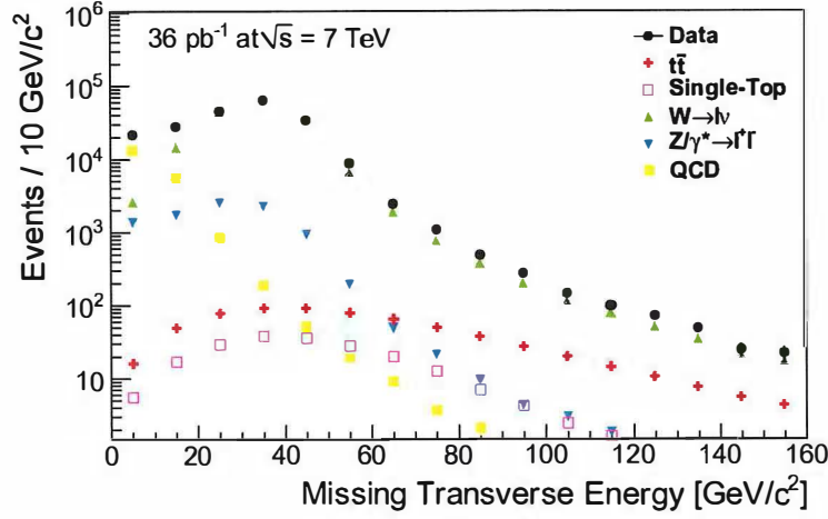
Figure 37. Missing transverse energy for different samples. The events passed the selection cuts regarding the primary vertex, the Global and Tracker Muon, all the muon selection cuts, the cuts for veto events with electrons and events with more than one muon.
