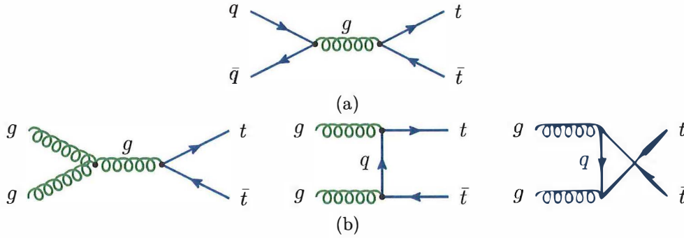
Figure 4. Feynman diagrams of the LO processes for t\bar{t} production: (a) quark-antiquark annihilation q\bar{q} \rightarrow t\bar{t} and (b) gluon-gluon fusion, gg \rightarrow t\bar{t} .
