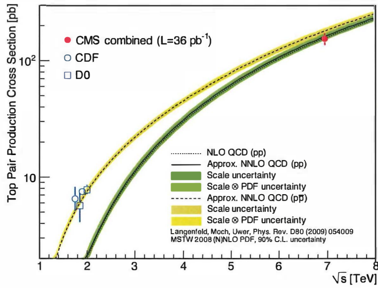
Figure 55. Comparison of the CMS and Tevatron results for the t\bar{t} production cross section with theoretical predictions as a function of \sqrt{s} .
