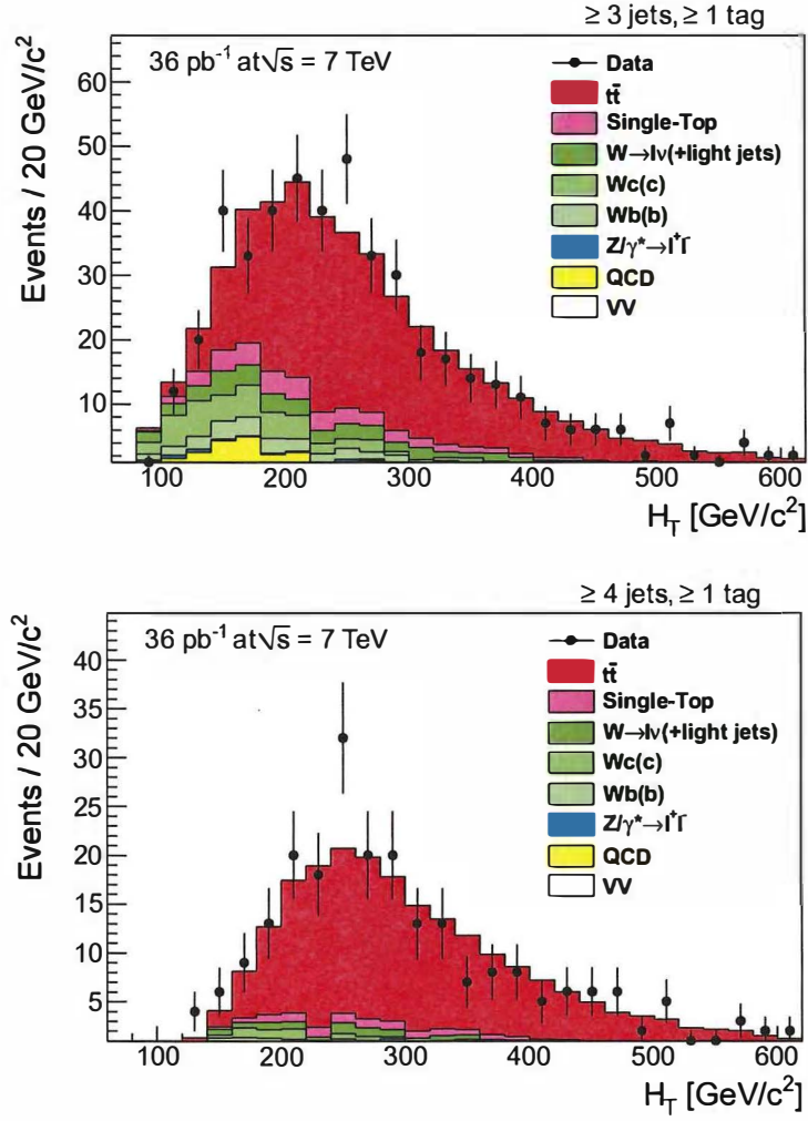
Figure 50. H_T of the leading jet distributions for the events with \geq 3 jets and at least 1 tag (top) and events with \geq 4 jets and at least 1 tag (bottom). Only statistical uncertainties are shown.
