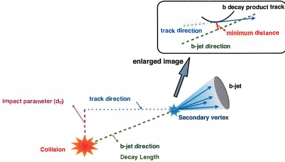
Figure 31. Representation of the secondary vertex, from which the b decay tracks originate. The track impact parameter measured with respect to the primary vertex is also shown.
