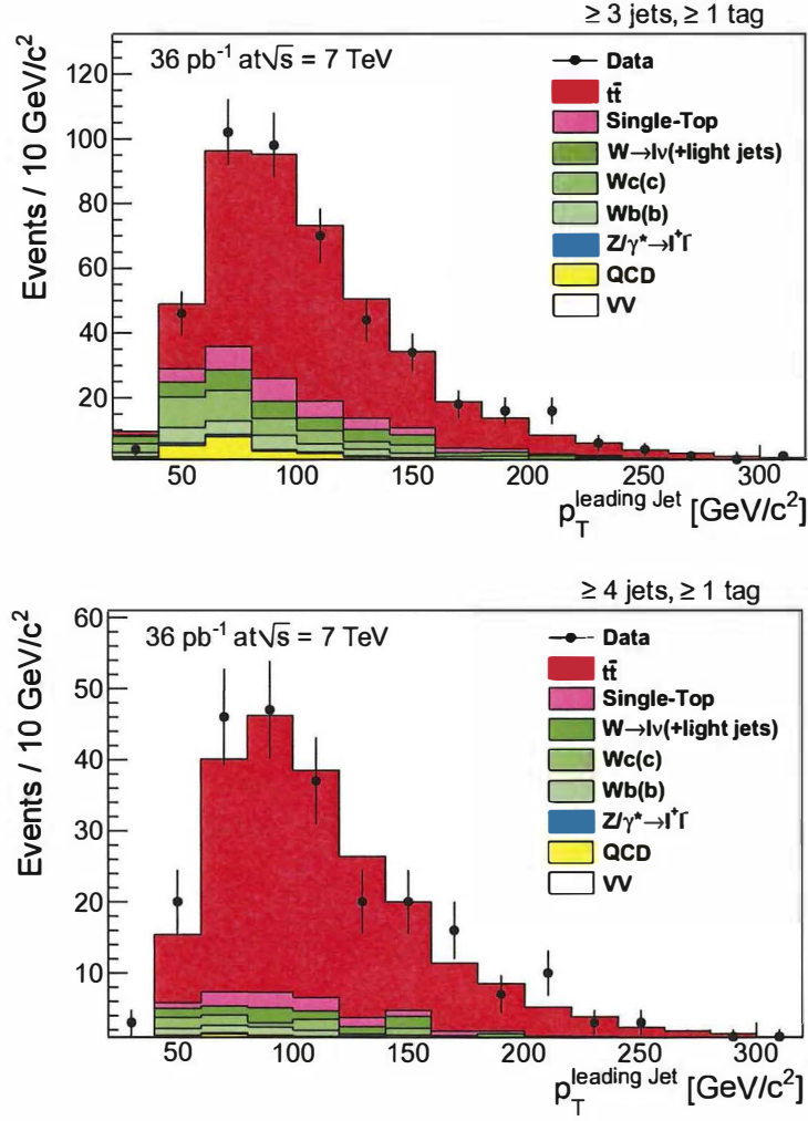
Figure 51. Transverse momentum of the leading jet for the events with \geq 3 jets and at least 1 tag (top) and events with \geq 4 jets and at least 1 tag (bottom). Only statistical uncertainties are shown.
