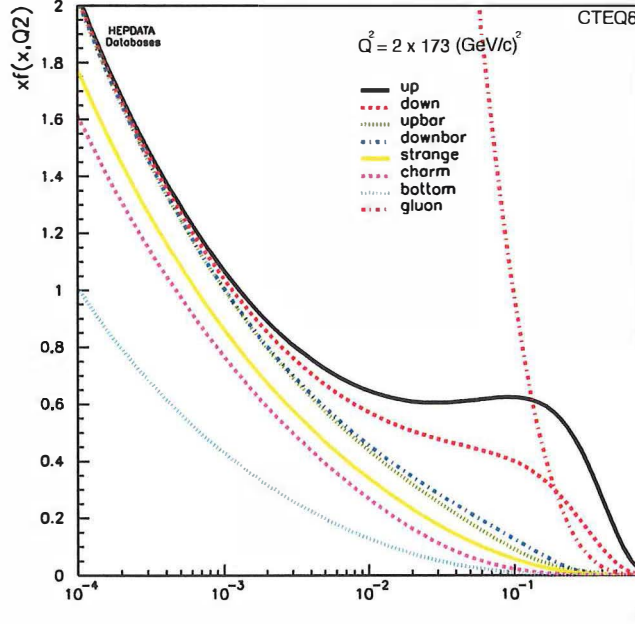
Figure 3. The quark, anti-quark and gluon momentum densities inside the proton as a function of the longitudinal momentum fractions x at \mu^2 = m_t^2 for top mass m_t = 173 GeV. The parametrization is CTEQ6.
