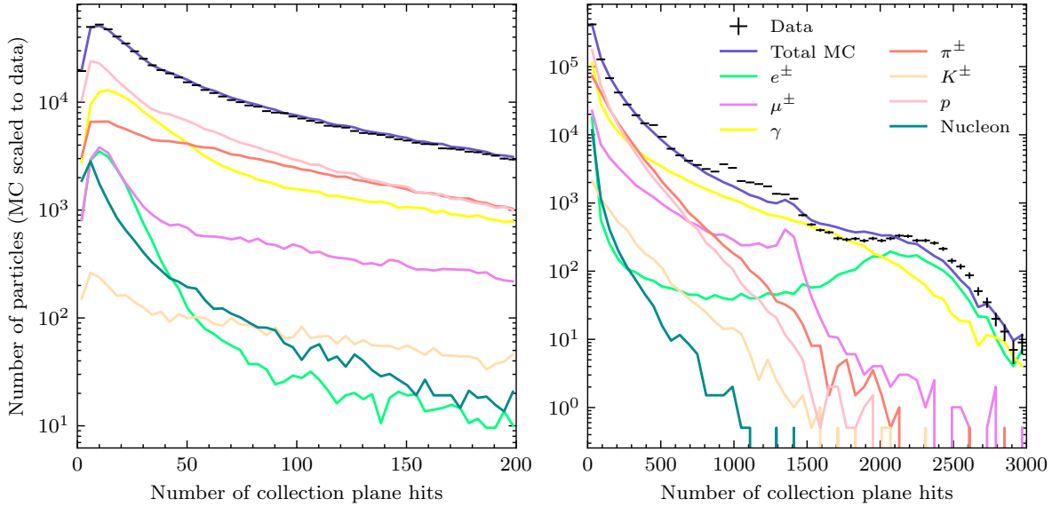
Figure 6.6: The number of collection plane hits of beam track daughter objects by true particle type. A close-up of the low end of the distributions is shown on the left, as well as a more complete range on the right.
