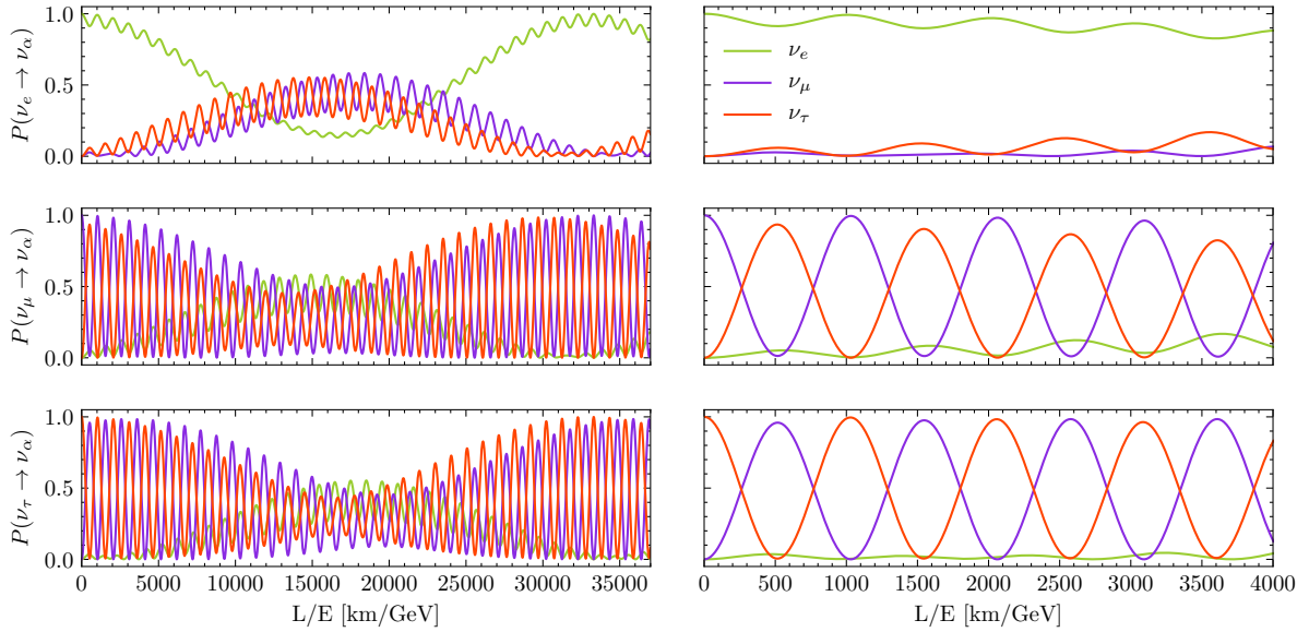
Figure S.2: Three-neutrino oscillation in vacuum for long (left) and short (right) travel length. Shown are an initial electron neutrino (top), muon neutrino (middle) and tau neutrino (bottom). The vertical axis of each graph denotes the probability of detecting a certain neutrino flavour.
