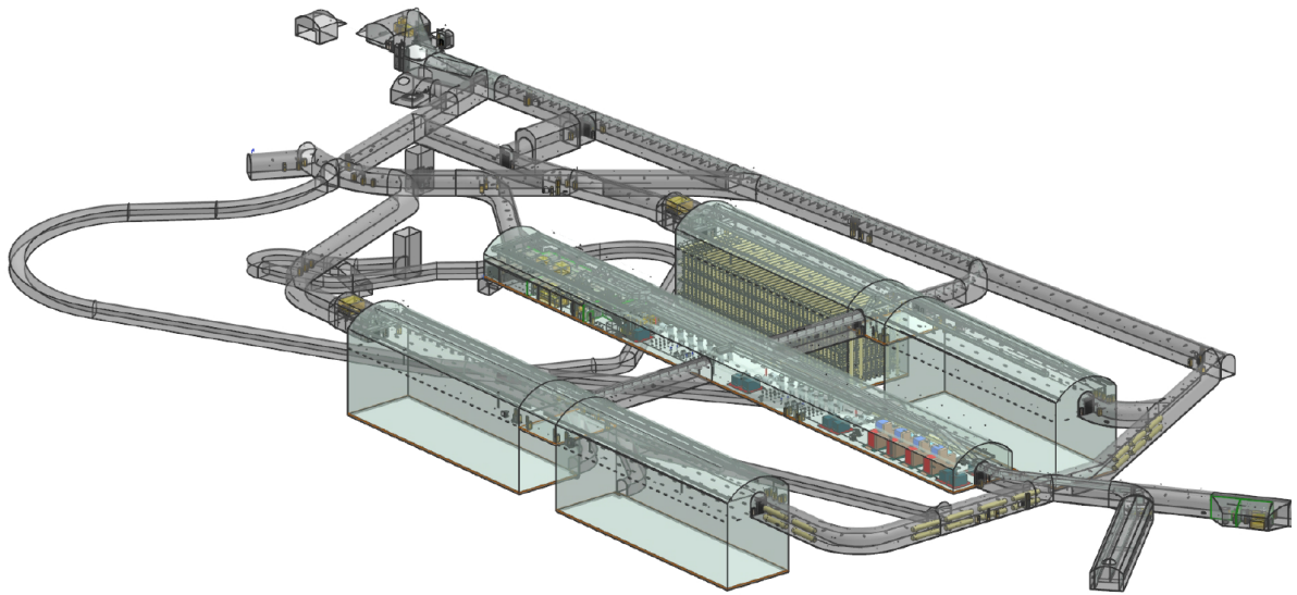
Figure 2.9: The DUNE far detector cavern system. Clearly visible are the four detector module caverns and central service cavern. One detector module is shown installed. Taken from [41].
