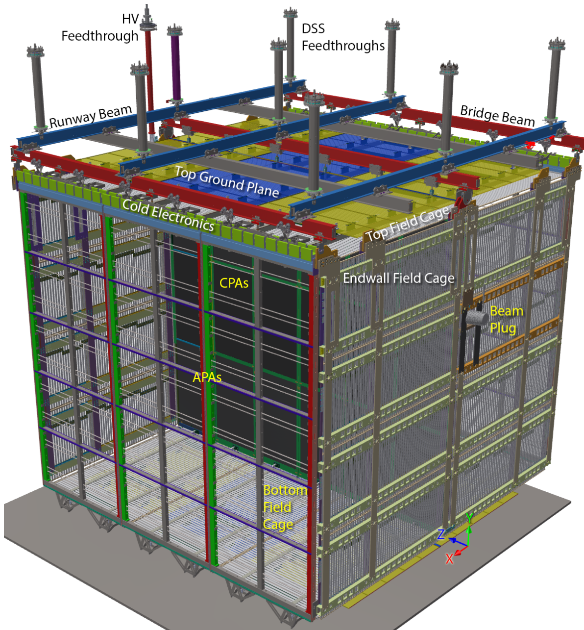
Figure 3.2: An unobstructed view of the ProtoDUNE TPC. The charged particle beam enters from the right through the beam plug. Three APAs are visible in this figure, with three more being positioned on the opposite side of the TPC, making for a TPC with two drift volumes. The entire TPC is submerged in liquid argon during operation. Taken from [55].
