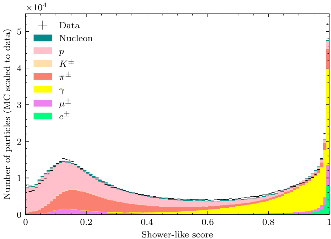
Figure 6.4: The CNN score of reconstructed daughter particles of the beam track.
