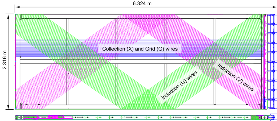
Figure 3.5: A front and side view of an APA. Some wires of each plane are shown in different colours. During normal operation, the APA hangs vertically from what is its right side in this figure. Taken from [39].
