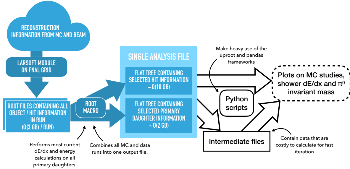
Figure 5.13: The analysis structure in use in this thesis.
