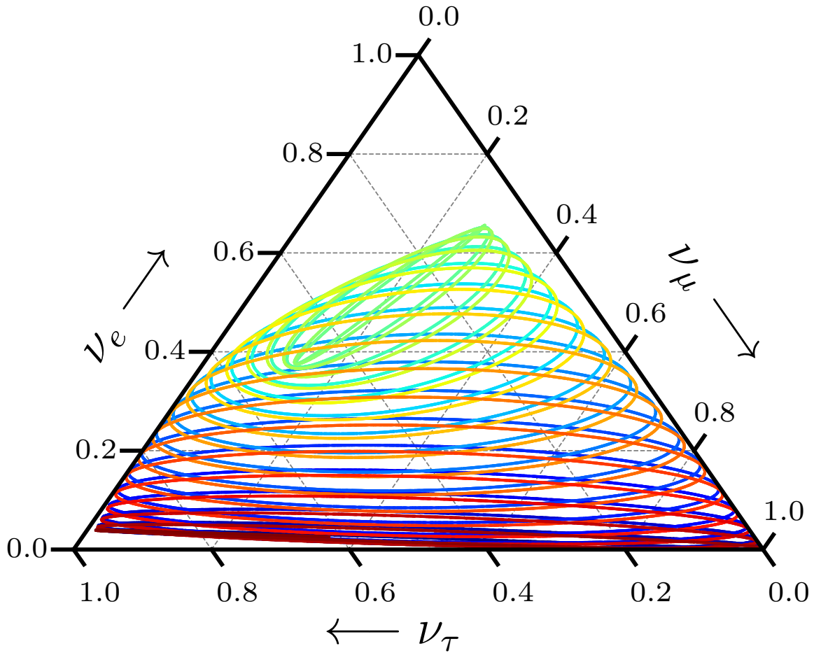
Figure 1.7: A ternary plot that shows the path of an initial 1 GeV muon neutrino through flavour space. The parameters shown in table 1.1 were used, with the exception of \delta_{CP} = 0 . A path length of 33000 km through vacuum was chosen so that the flavour path nearly returns to the pure \nu_\mu state in the bottom right corner of the triangle. The colour scale indicates distance along the path length, starting with blue and shifting via green to red.
