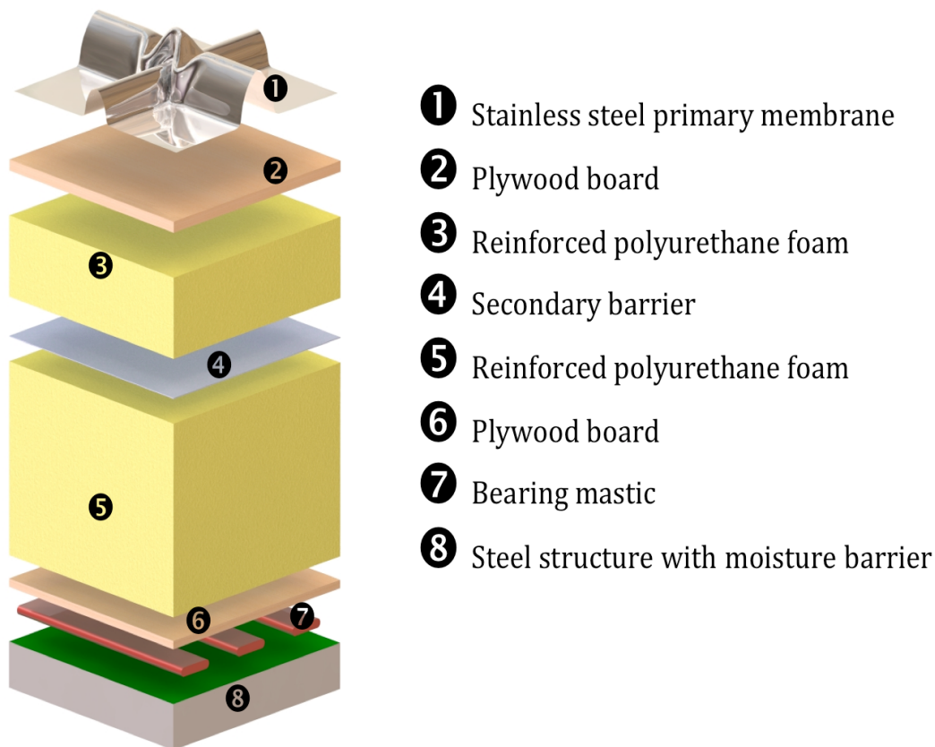
Figure 3.3: The various layers of insulation that ProtoDUNE uses to keep its argon contained and cool. The upper layer, the stainless steel membrane, has the ability to deform and stretch under extreme temperature changes thanks to its corrugated shape. Taken from [68].
