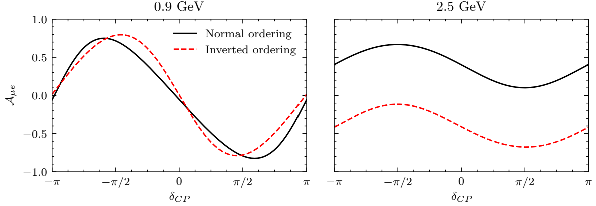
Figure 2.16: The neutrino appearance asymmetry A_{\mu e} as a function of \delta_{CP} and the two mass ordering possibilities, shown both for a neutrino energy of 0.9 GeV (left) and 2.5 GeV (right).
