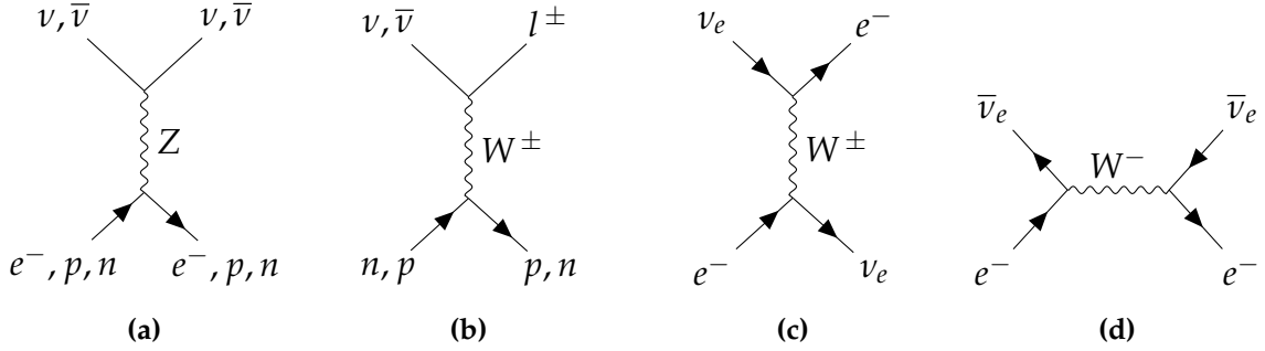
Figure 1.2: The main interactions of neutrinos with ordinary matter. All (anti-)neutrinos undergo neutral current interaction with quarks and electrons (a) and charged current interaction with quarks (b). In the latter, an (anti-)lepton l^\pm is emitted corresponding to the neutrino flavour. At neutrino energies < 11 GeV, only electron neutrinos (c) and anti-electron neutrinos (d) undergo charged current interactions with electrons.
