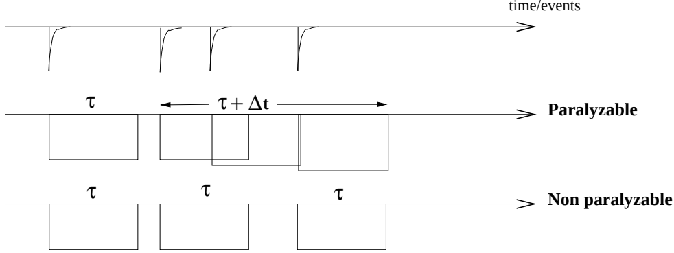
Figure 4.13: Schematic representation of the two types of dead time systems.
