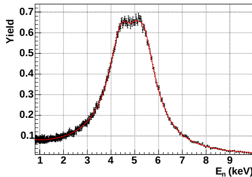
Figure 4.10: 4.9 \text{ eV } ^{197}\text{Au}+n resonance used for inter calibration.
