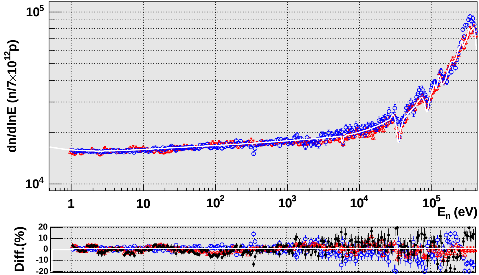
Figure 4.8: Adopted neutron intensity (solid line) from several measurements (open circles correspond to the Si-flux monitor, open triangles stand for the PTB measurement). On the bottom pannel, relative differences with respect to the adopted intensity shape are shown for the two measurements. Solid symbols correspond to relative differences between both measurements.
