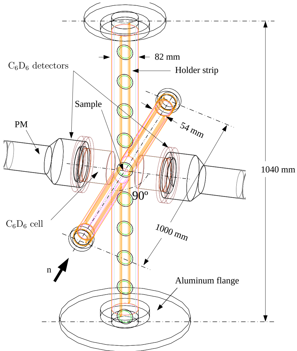
Figure 3.2: Schematic view of the n_{\text{TOF}} ( n, \gamma ) experimental setup with the sample changer and two C 6 D 6 detectors.
