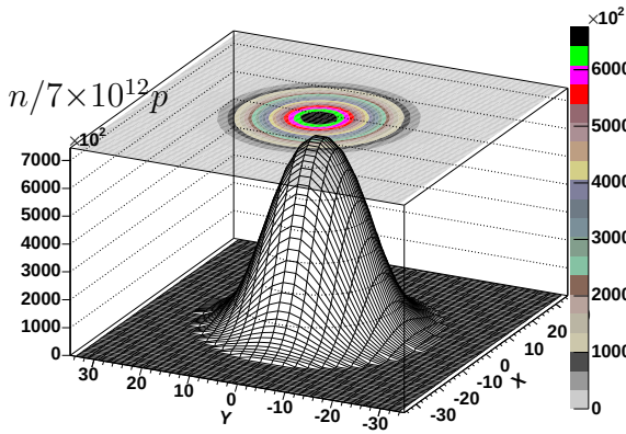
Figure 4.12: Plot of the n_TOF beam profile [52] in the neutron energy range from 10 eV up to 100 eV.
