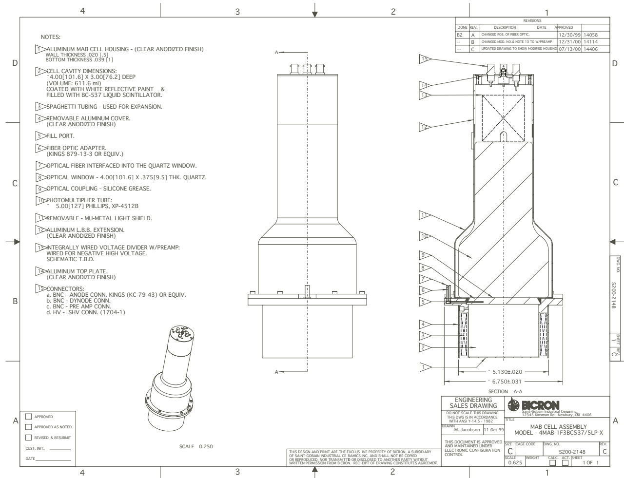
Figure D.1: Bicron detector scheme.
