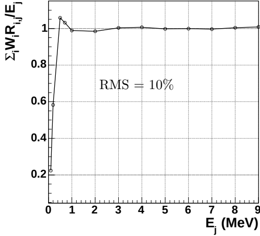
Figure 6.2: Proportionality check for the polynomial WF.
