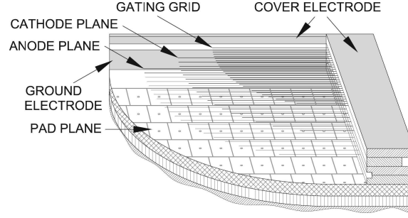
Figure 2.5.: Cross section through a readout chamber of the TPC, with the pad plane, the three wire planes and the cover electrode [111].
