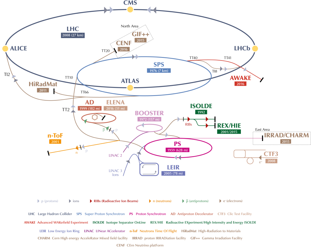
Figure 2.1.: CERN accelerator complex [114].
