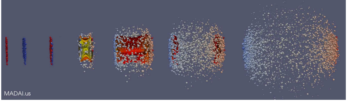
Figure 1.2.: Stages of an ultra-relativistic heavy-ion collision, from UrQMD [36,37].
