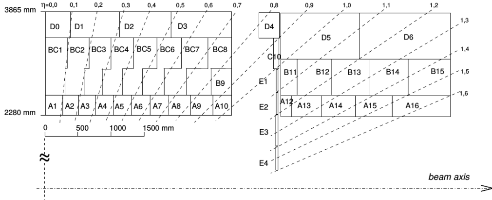
Figure 4.5: Segmentation in depth and \eta of the TileCal modules in the central (left) and extended (right) barrels [57].
