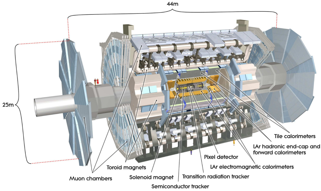
Figure 4.2: Cutaway view of the ATLAS detector [57]. The sub-detectors and main systems are identified, and two persons are visible on the image for scale.
