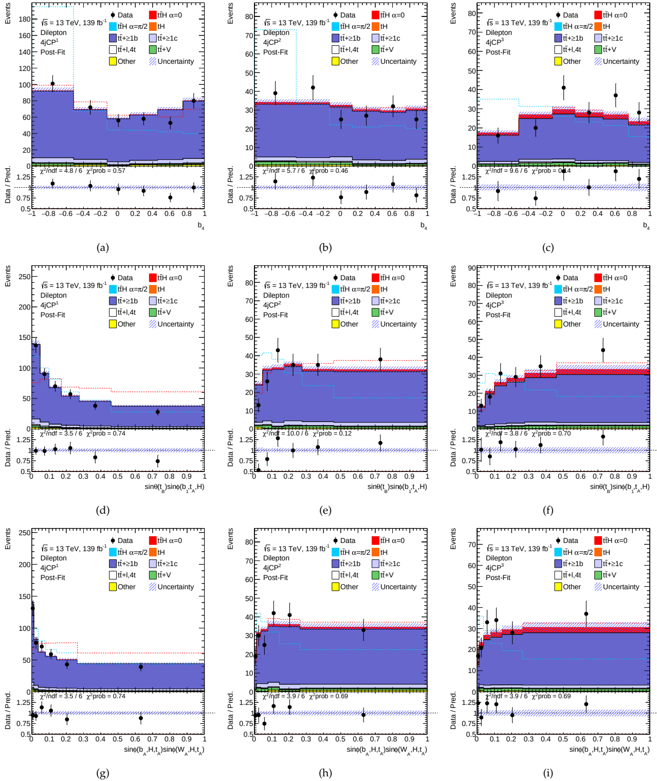
Figure 9.27: Comparison between data and post-fit prediction for the distributions of the most important input variables to the \mathcal{CP} BDT, in 4j\text{CP}^1 (left), 4j\text{CP}^2 (middle), and 4j\text{CP}^3 (right). (a,b,c) b_4 . (d,e,f) \sin\theta(t_B) \sin\phi(b_1, t_A, H) . (g,h,i) \sin\phi(b_A, H, t_A) \sin\phi(W_A, H, t_A) .
