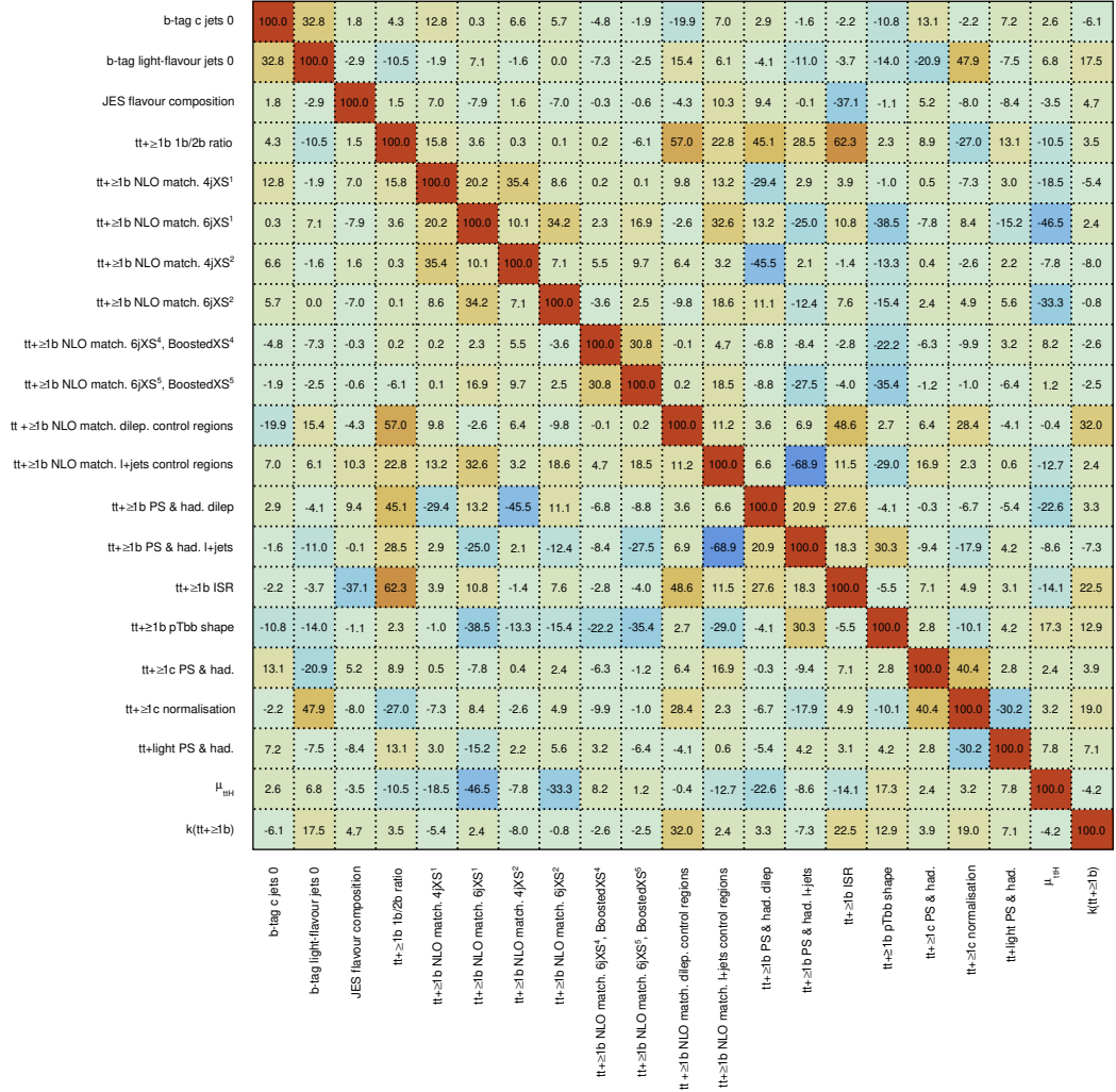
Figure 8.9: Correlation coefficients, in %, between the parameters in the fit to the Asimov dataset.
