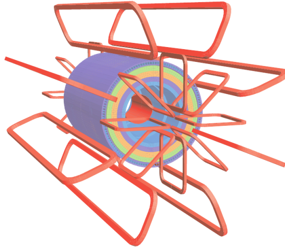
Figure 4.6: Geometry of magnet windings (in red) and TileCal steel. The eight toroidal coils in each end-cap are tilted relative to the barrel coils. The solenoid winding lies inside the calorimeter volume [57].
