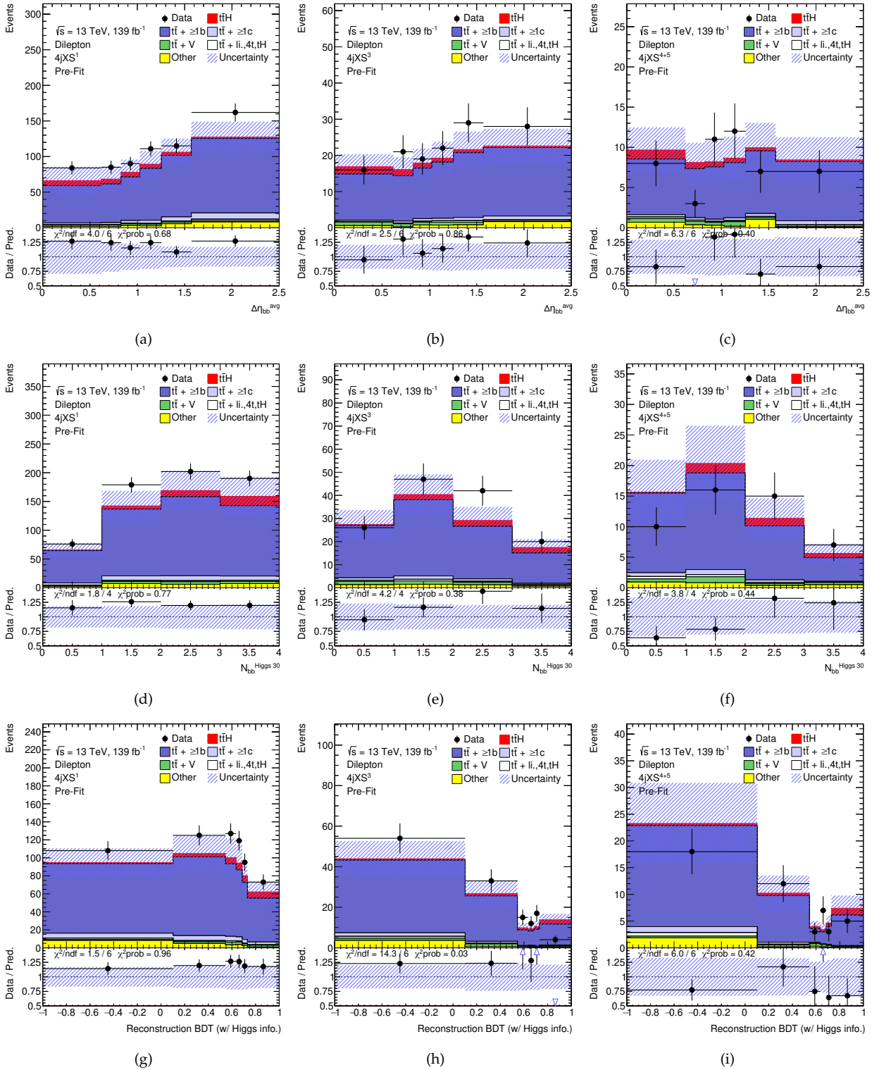
Figure 8.5: Distributions of data and pre-fit prediction for the most relevant input variables to the dilepton Classification BDT, in the regions 4jXS^1 (left), 4jXS^3 (middle) and 4jXS^{4+5} (right). (a,b,c) \Delta\eta_{bb}^{avg} . (d,e,f) N_{bb}^{Higgs 30} . (g,h,i) Reconstruction BDT output with Higgs boson information.
