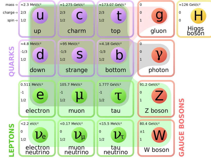
Figure 1.1: Summary of the particle content of the SM. Shaded areas surround each gauge boson and the fermions that interact with it [13]. Upper limits on the neutrino masses are to be interpreted with care, since the flavour eigenstates are strongly mixed with respect to the mass eigenstates.
