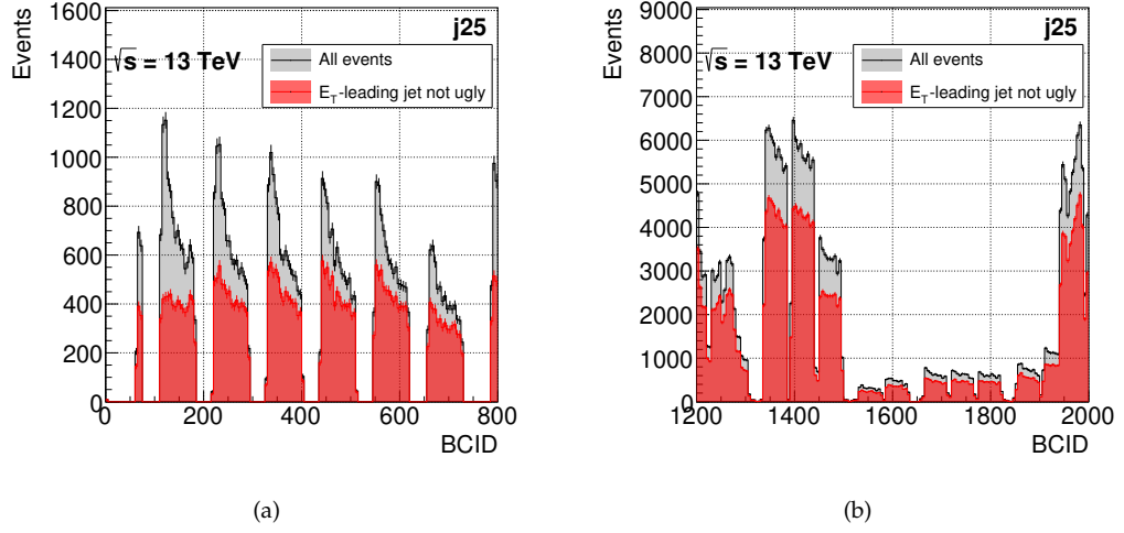
Figure 5.2: Distributions of BCID for events recorded by j25. The grey histograms show all events, while the red ones are restricted to those in which the E_T -leading central jet is not ugly. (a) 2016 period B. (b) 2017 period B.
