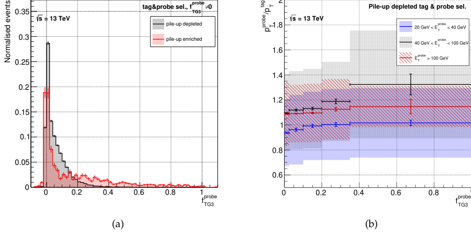
Figure 5.5: (a) Normalised distributions of f_{TG3} of the probe in events passing the tag-and-probe selection, in the pile-up enriched (red) and pile-up depleted (grey) regions. Events with f_{TG3}^{\text{probe}} exactly equal to 0 are excluded from the histograms. (b) Average ratio p_T^{\text{probe}} / p_T^{\text{tag}} as a function of f_{TG3}^{\text{probe}} for three different E_T^{\text{probe}} ranges in the pile-up depleted region. The shaded bands indicate the standard deviation of p_T^{\text{probe}} / p_T^{\text{tag}} , while the vertical lines correspond to the uncertainty on its average value.
