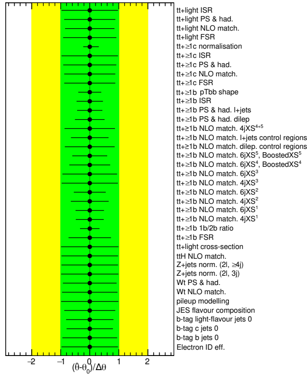
Figure 8.8: Expected uncertainties on nuisance parameters from the fit to the Asimov dataset. Black bars correspond to the post-fit constraint, while the prior constraint on all nuisance parameters is \pm 1 (green band).
