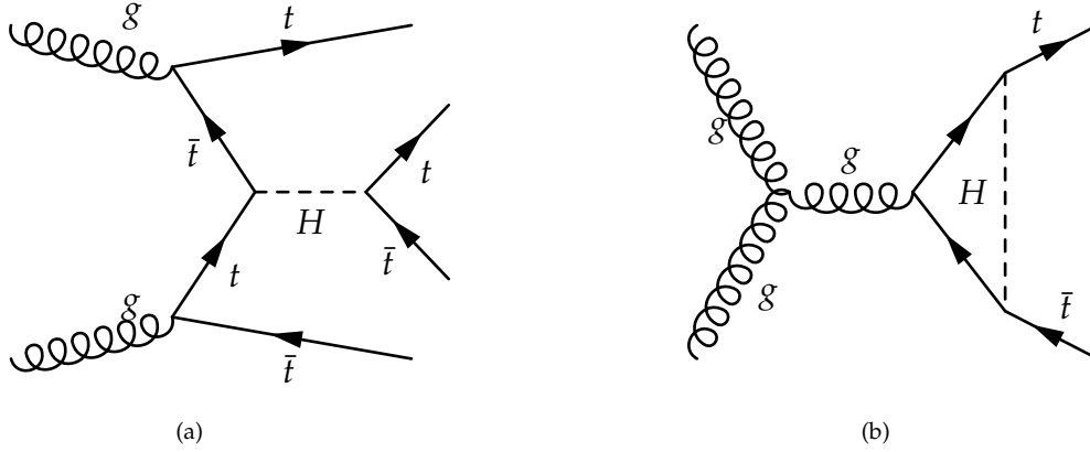
Figure 2.8: Processes at the LHC, besides Higgs boson production processes, that are sensitive to the top quark Yukawa coupling. Examples of Feynman diagrams in which the Yukawa coupling is relevant are shown. (a) t\bar{t}t\bar{t} production. (b) t\bar{t} production.
