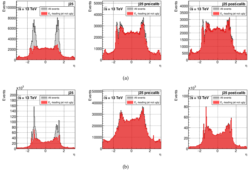
Figure 5.3: Distributions of \eta of the central jet leading in E_T in the original jet collection and in the collections modified by pre-calib and post-calib corrections, for events passing the modified j25 chain. The grey histograms show all events, while the red histograms are restricted to events in which the E_T -leading central jet of the modified chain is not ugly. (a) 2016 period B. (b) 2017 period B.
