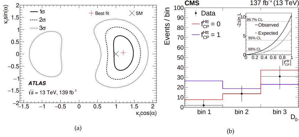
Figure 2.5: Results of the direct measurements of the \mathcal{CP} nature of the top quark Yukawa coupling in t\bar{t}H production, with H \rightarrow \gamma\gamma . (a) ATLAS results in the (\kappa_t, \tilde{\kappa}_t) plane, together with the SM point [76]. The best-fit point is shown, as well as the exclusion contours at significances of 1, 2 and 3 standard deviations. (b) Distributions of the \mathcal{CP} BDT used by CMS, for the observed data and for the \mathcal{CP} -even and \mathcal{CP} -odd signal hypotheses, and the log-likelihood profile of a parameter equivalent to \sin^2 \alpha .
