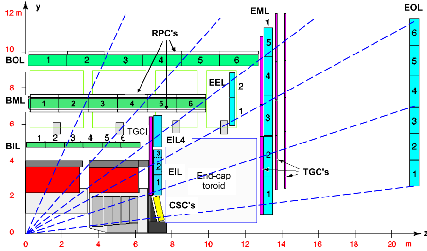
Figure 4.7: Labels: B/E - barrel/end-cap, I/M/O - inner/medium/outer, L - large. Cross-section of the muon system in a plane containing the beam axis. Straight trajectories are illustrated by the dashed lines and most likely traverse three muon stations [57].
