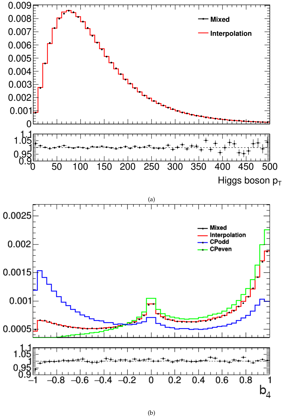
Figure 9.1: Examples of distributions used for validating the parameterisation of \mathcal{CP} -mixed t\bar{t}H . Truth-level observables are compared between the parameterised prediction – ‘interpolation’ – and the sample generated in the \mathcal{CP} -mixed scenario – ‘mixed’. (a) p_T of the Higgs boson in the single-lepton channel. (b) b_4 in the dilepton channel, with the distributions of the pure \mathcal{CP} -even and pure \mathcal{CP} -odd samples also shown.
