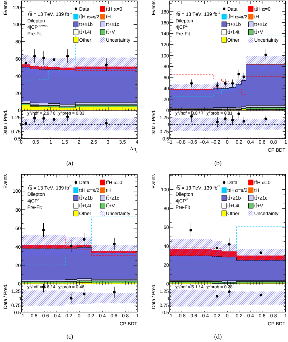
Figure 9.9: Comparison between data and pre-fit prediction of the distributions used in the fit in each of the dilepton \mathcal{CP} -dedicated regions. (a) 4j\text{CP}^{\text{no-reco}} . (b) 4j\text{CP}^1 . (c) 4j\text{CP}^2 . (d) 4j\text{CP}^3 .
