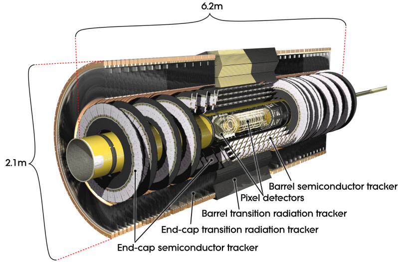
Figure 4.3: Cutaway view of the inner detector, with all of its components labeled [106]. The image portrays the ID before the insertion of the innermost pixel layer, the inner B-layer.
