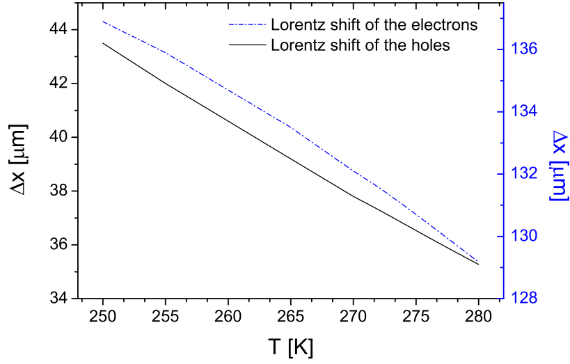
Figure 4.10: The temperature dependence of the Lorentz shift \Delta x for holes (lower curve, left scale) and electrons (top curve, right scale) predicted for a 300\mu\text{m} thick sensor in a 4T magnetic field at a bias voltage U_{\text{bias}} of 100\text{ V} .
