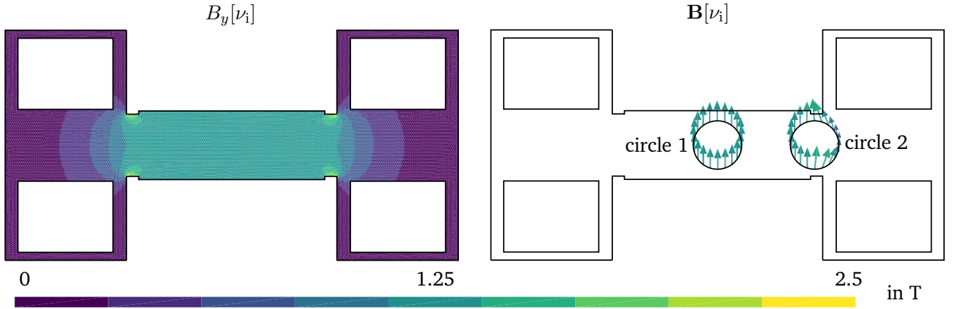
Figure 4.2: Magnetic flux density B[\nu_i] for the excitation current I = 500 A. Left: B_y evaluated on the inner air domain. Right: B evaluated on circles with radius r_0 = 6 cm.
