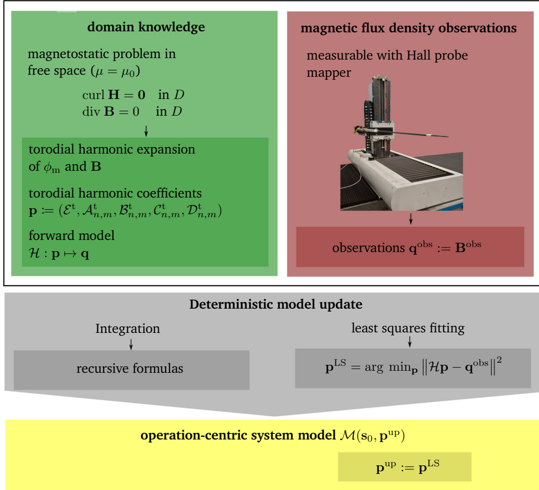
Figure 6.2: Overview of sources of knowledge and methods to build an operation-centric system model on a toroidal domain based on the torodial harmonic expansion. From the magnetostatic problem in free space, the torodial harmonic expansion of the magnetic scalar potential, and the magnetic flux density are derived using R -separation. The coefficients of this expansion are determined using integration and least squares fitting. The least squares fitting method is recommended since the recursive formulas obtained by integration are numerically unstable. The resulting system model can be used to predict the magnetic flux density in positions that were not included in the observations \mathbf{q}^{\text{obs}} .
