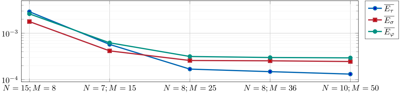
Figure 6.15: Average relative error defined in equation (6.61) on \partial \tilde{D}_{\text{test}} between the predicted magnetic flux density based on the determined toroidal harmonic coefficients for different truncation thresholds N and M and the ground truth magnetic flux density simulated with the ROXIE model for the curved CCT example.
