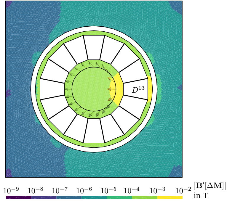
Figure 5.6: Gâteaux derivative \mathbf{B}'[\Delta \mathbf{M}] of the magnetic flux density at the nominal magnetization in the direction of the sample mean magnetization deviation of the 13-th PM block defined in equation (5.26). On the air domain, the absolute value |\mathbf{B}'[\Delta \mathbf{M}]| is visualized. On the circle with radius 75 mm, \mathbf{B}'[\Delta \mathbf{M}] is visualized.
