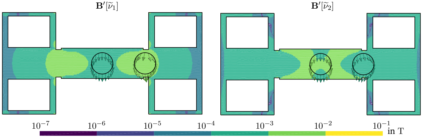
Figure 4.10: Gâteaux derivatives B'[\tilde{\nu}_m] of the magnetic flux density in direction of the relativity perturbations corresponding to the scaled eigenfunctions of the KLE-based H(B) -curve model. On the inner air domain |B'_y[\tilde{\nu}_m]| is visualized, on the circles defined in Figure 4.2 B'[\tilde{\nu}_m] is visualized. Figure adapted from [53].
