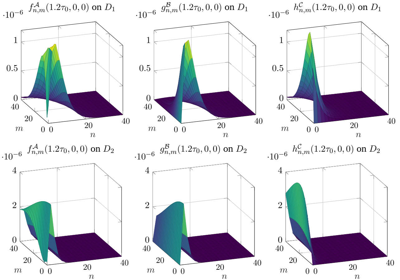
Figure 8.1: Absolute values of the functions f_{n,m}^A , g_{n,m}^B and h_{n,m}^C which are part of the toroidal harmonic expansion of the magnetic flux density evaluated at the point (1.2\tau_0, 0, 0) and plotted as functions of the degree n and the order m . Top row: Toroidal domain D_1 with eccentricity \epsilon = 2 . Bottom row: Toroidal domain D_2 with eccentricity \epsilon = 10 .
