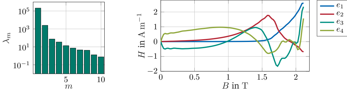
Figure 4.7: Ten largest eigenvalues \lambda_m and eigenfunctions e_m of the operator T_f defined in equation (4.33) evaluated for the ARMCO® Pure Iron Grade 4 specimens without the test specimen. Figure adapted from [53].
