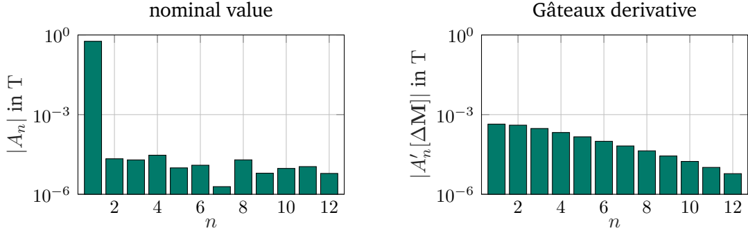
Figure 5.7: Left: Absolute values |A_n| of the nominal skew multipole coefficients on the centered circle with radius 75 mm. Right: Absolute values |A'_n[\Delta \mathbf{M}]| of the Gâteaux derivative of the skew multipole coefficients in the direction of the sample mean magnetization deviation of the 13-th PM block (equation 5.26) and at the nominal magnetization on the centered circle with radius 75 mm.
