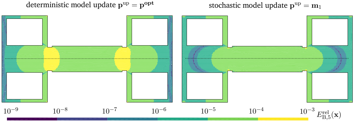
Figure 4.16: Relative error E_{B,5}^{\text{rel}}(\mathbf{x}) (defined in equation (4.98)) of the prediction of the quantity of interest Q_B with the updated models compared to the ground truth prediction at I_5 = 517 A.
