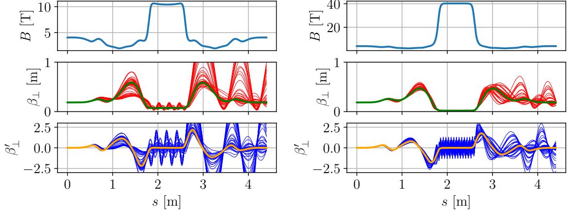
Figure 5.3.: Adiabatic ramping of the magnetic field in a CERN-type solenoid is illustrated. Starting at 10 T ( left ), the optimizer minimizes \beta_{\perp} inside the solenoid while ensuring \beta'_{\perp} = 0 , shown as thick lines . Thin lines represent intermediate optimization steps. Once a solution is found, the solenoid field strength is increased and re-matched, using the previously matched values as a starting point. This process—matching, increasing the field, and re-matching—is repeated in adiabatic steps. Once the target field-strength of 40 T ( right ) is reached and the beam is matched, the process ends. The final and matched solutions of the beam parameters are depicted as the thick lines in the right plots.
