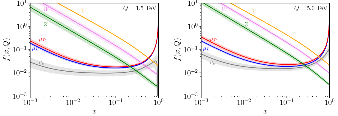
Figure 2.1.: Lepton parton distribution functions ( LePDF ) of various particles at factorization scales Q = 1.5 TeV ( left ) and Q = 5 TeV ( right ). The increase in the neutrino PDF f_{\nu_\mu} of the muon appears as x \rightarrow 1 . The uncertainty bands corresponds to Q/2 and 2Q in both diagrams. The figures were generated with the interpolation [55] of data that are publicly accessible from [56].
