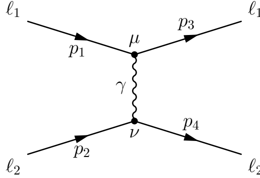
Figure 3.1.: The QED t-channel interaction involves two charged particles, \ell_1 and \ell_2 . These particles carry charges Z_1e and Z_2e , respectively. The interaction is facilitated by the exchange of a photon \gamma at the vertices \mu and \nu via the electromagnetic force.
