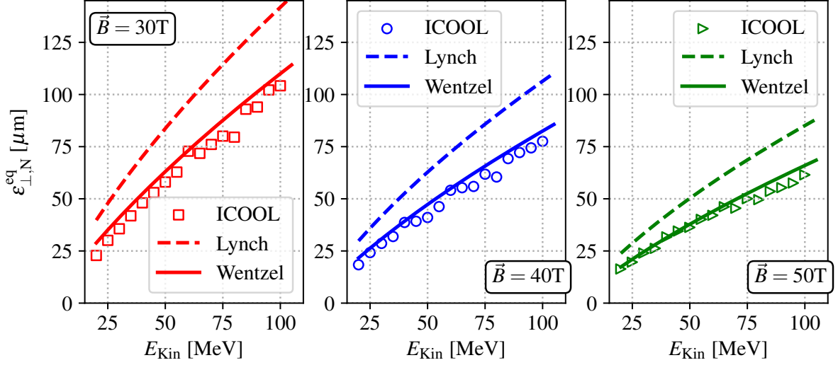
Figure 4.6.: The equilibrium emittance of liquid hydrogen subjected to a longitudinal static field of 30, 40, and 50 T is assessed using ICOOL. The results shows remarkable consistency with the analytical model when the Bethe-Wentzel scattering assumption is considered.
