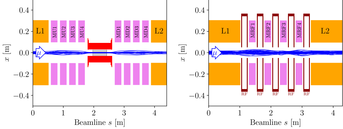
Figure 5.6.: The diagram on the left shows the arrangement of a solenoid within an ionization cooling cell, with the beam envelope represented by thin blue lines. The center of the left diagram features the high-field CERN solenoid, incorporating an absorber illustrated as the gray surface. On the right plot: The setup of a solenoid-cavity configuration includes five 150 MHz RF cavities, each with an accelerating gap of 20 cm powered at 10 MV/m, positioned between two 4 T solenoids (L1 and L2). The cavities are spaced 50 cm apart and interleaved with 20 cm wide matching coils (MRF1-MRF4). The reference particle starts with a momentum of p_{\text{ref}} = 131.8 \text{ MeV}/c and an RF phase of \varphi_{\text{acc}} = 54^\circ .
