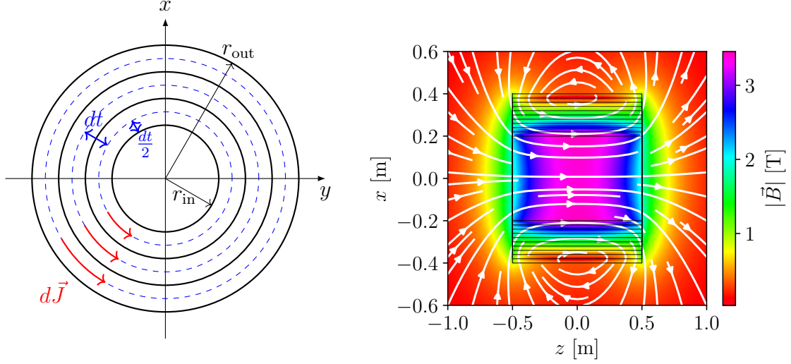
Figure 4.2.: Left figure: a solenoid with finite thickness t can be modeled using a sheet approximation by dividing it into an arbitrary number of coaxial rings with thickness dt . Right figure: An example of a solenoid field composed of 10 finite current sheets with a length of 1 m centered at the origin.
