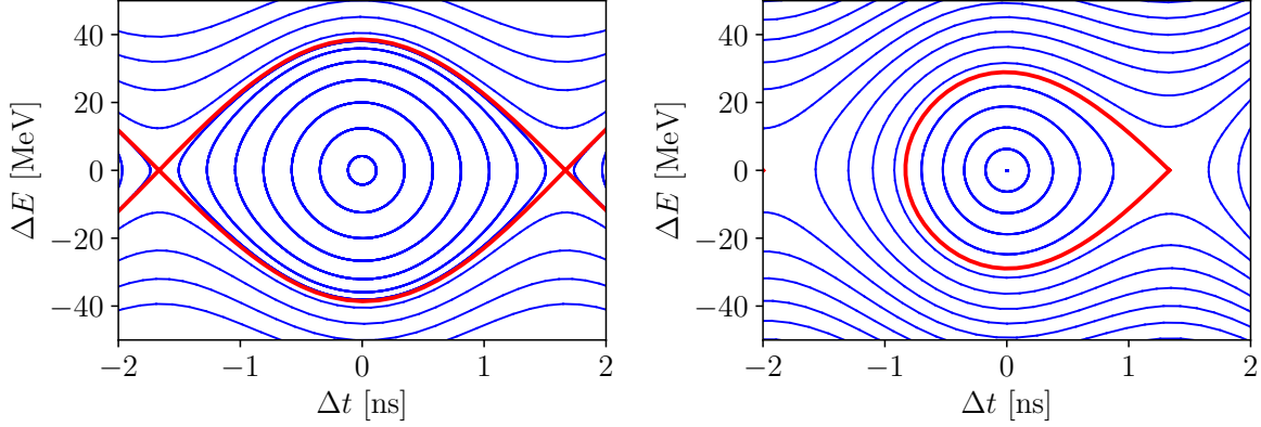
Figure 4.5.: The equipotential lines illustrate particle motions in the longitudinal phase space. Closed contours correspond to stable regions, while the separatrix, shown as a thick red line , marks the boundary between stable and unstable motion. The left plot depicts the case for \psi_0 , where the separatrix forms a stationary bucket. In the accelerating phase 0 < \psi_0 < \pi/2 , the separatrix deforms into a running bucket, as shown in the right plot.
