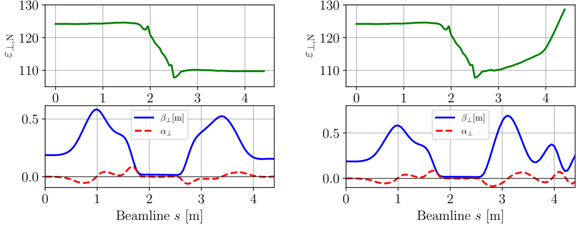
Figure 5.9.: Comparison of matched and mismatched Conditions in an Ionization Cooling Cell. The left upper plot shows the normalized transverse emittance, \varepsilon_{\perp,N} , varying only within the absorber region under matched conditions, with a flat beam envelope in the low and high regions( left below ). The right upper plot illustrates mismatched conditions in the downstream matching sections (MD1-MD4), leading to rapid emittance growth and oscillating \beta_{\perp} and \alpha_{\perp} after the high field area( left below ), highlighting the impact of parameter misalignment.
