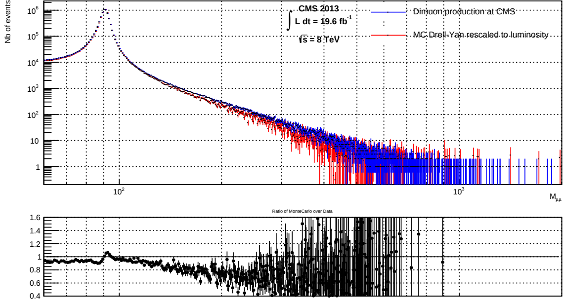
FIGURE 4.6 – Superposition of the dimuon signal and of the MC simulation of the Drell-Yan rescaled to the luminosity and corrected by the scale factors and for the pile-up.
