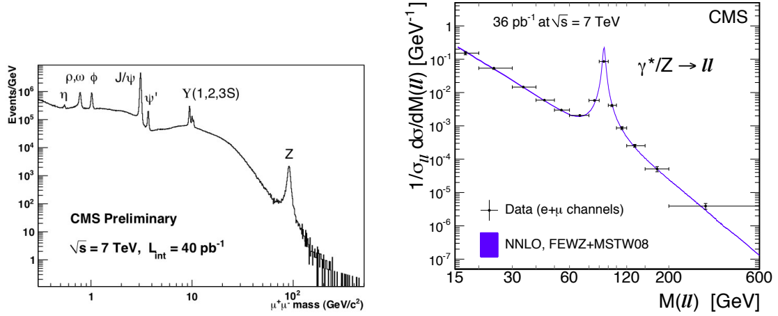
(a) Invariant mass spectrum of the two resulting muons of the Drell-Yan process obtained as a preliminary plot of CMS. One can see the peaks of the resonances, as the J/\Psi 's or the Z^0 's, among others. In our study, we shall be interested by such a plot, but in a range starting at 60 GeV up to 2 TeV, far more on the right.
