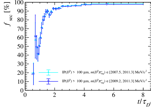
Figure 6.10: Fraction of secondary decays in data satisfying \text{IP}(D^0) > 100 \mu\text{m} , as calculated from the results of the template fit to the \text{IP} vs. t distribution of D^0 mesons, in the enlarged ( [2007.5, 2011.3] \text{ MeV}/c^2 ) and in the nominal ( [2009.2, 2011.3] \text{ MeV}/c^2 ) m(D^0 \pi_{\text{tag}}^+) signal window.
