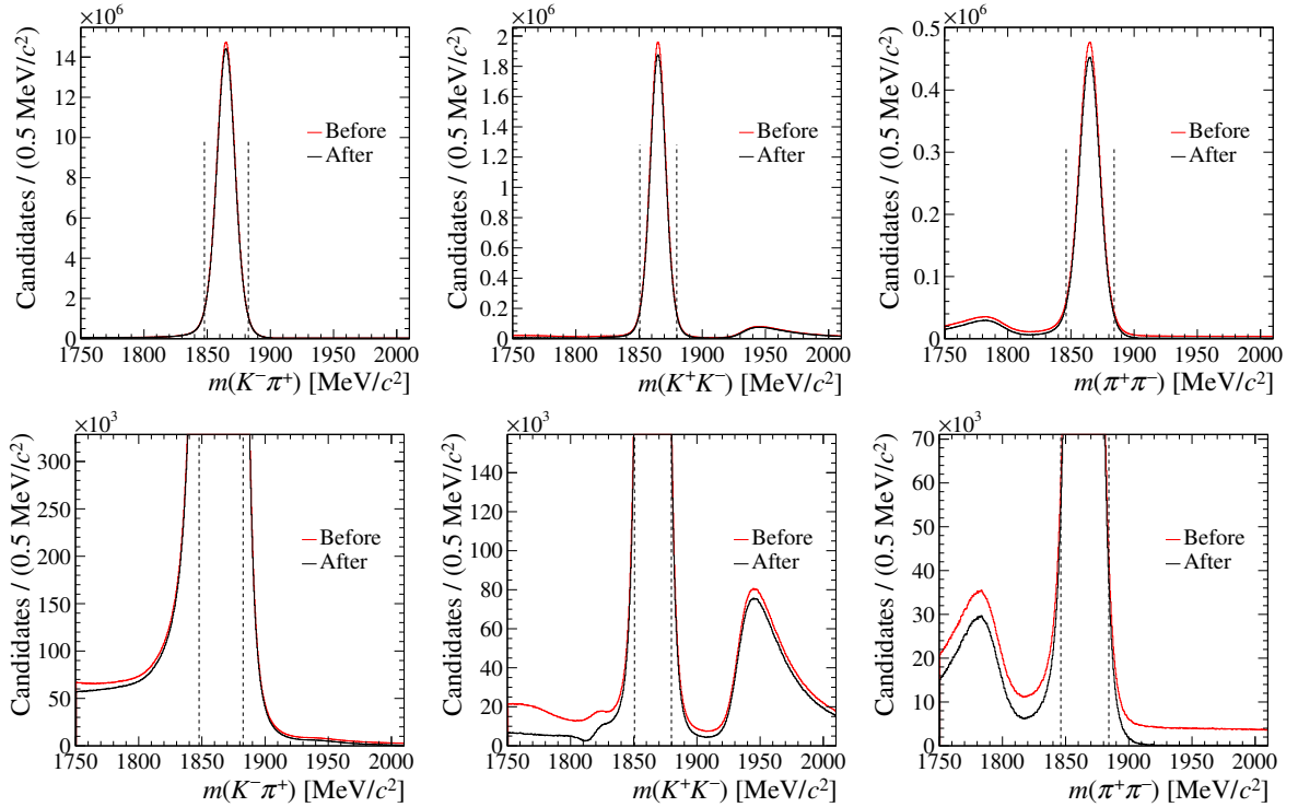
Figure 7.7: (Top): distribution of the invariant mass m(h^+h^-) of the final-state particles of the D^0 candidate (red) before and (black) after the removal of the m(D^0\pi_{\text{tag}}^+) background. The vertical dashed lines delimit the signal window. (Bottom): Magnification to put in evidence the shape of the residual background under the m(D^0) peak.
