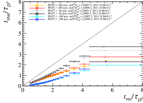
Figure 6.13: True decay time of secondary D^0 mesons as a function of their measured decay time.
