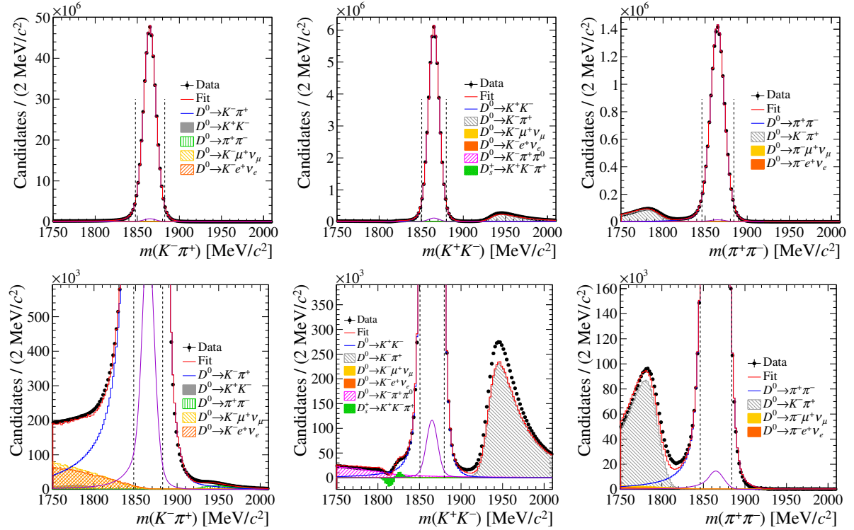
Figure E.4: Template fit to the time and flavour integrated m(h^+h^-) distributions of (left) K^-\pi^+ , (centre) K^+K^- and (right) \pi^+\pi^- decays. The relative normalisation between the background components and the signal is fixed to the expectations of RAPIDSIM and PIDCALIB; the signal component due to decays in flight of D^0 daughter mesons into muons is shown in violet. Bottom plots are magnified to put the background components in evidence.
