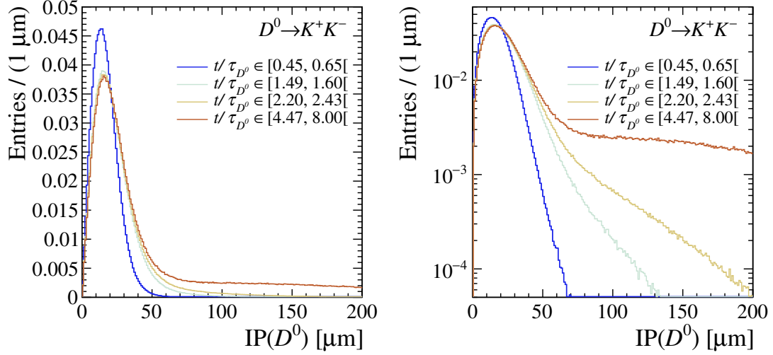
Figure 6.2: Distributions of the D^0 IP in (left) linear and (right) logarithmic scale, for the 0 th , 10 th , 15 th and 20 th bins of decay time. The long tails of the distributions at high decay times are due to secondary decays.
