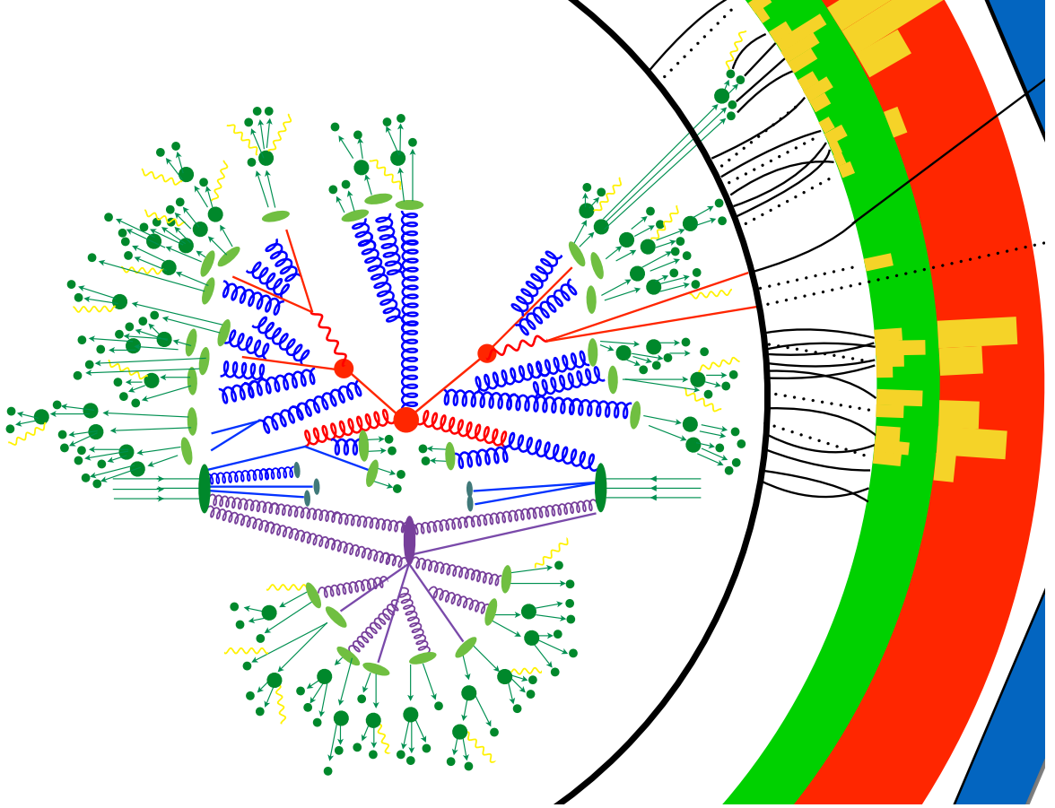
Figure 6.1: Schematic depicting the various steps in generating a simulated gg \rightarrow t\bar{t} \rightarrow q\bar{q}b\mu\nu_\mu\bar{b} event using Monte-Carlo methods. The process starts with the incoming protons represented by the large dark green blobs and arrows pointing towards the centre of the figure. Two partons then interact in the main hard scatter process, depicted in red, from which a top-quark and anti-top-quark are generated. The parton-shower is depicted in blue with the initial stages of the hadronisation process shown by light green blobs. The subsequent decay of the initial hadrons into stable final-state particles is shown in dark green with any generated photons indicated in yellow. The lower part of the image depicts additional decays from multiple parton interactions (MPI) in purple, and proton decay remnants which make up part of the underlying event (UE). Finally the right hand side of the image depicts the process of simulating interactions with different layers of the ATLAS detector. Original image courtesy of [97]
