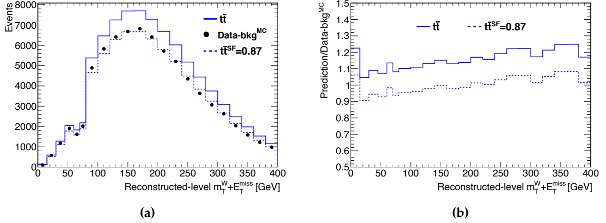
Figure 9.1: Number of events at detector-level in bins of E_T^{\text{miss}} + m_T^W for (a) the data – bkg MC , and the POWHEG+PYTHIA8 t\bar{t} prediction before and after the application of the scale-factor ( t\bar{t}^{\text{SF}} = 0.87 ). (b) The ratios of the t\bar{t} predictions to the data – bkg MC are shown.
