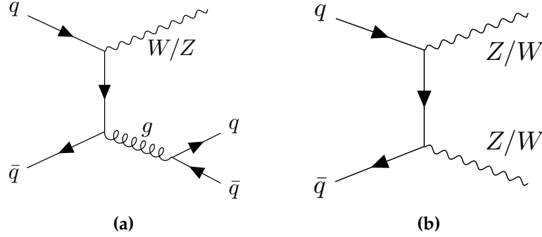
Figure 7.4: Example tree-level Feynman diagrams for background events which do not include a top-quark, (a) W(Z)+\text{jets} (b) diboson
