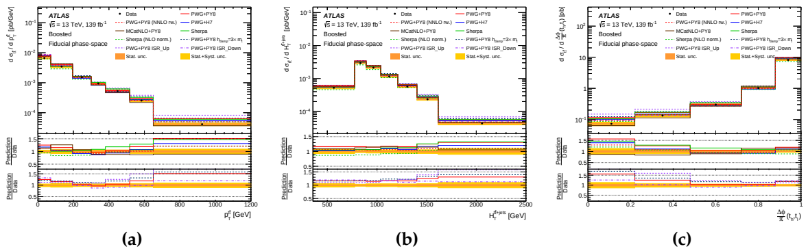
Figure 10.9: Fiducial t\bar{t} cross-section measured as a function of (a) p_T , (b) H_T^{t\bar{t}+\text{jets}} , and (c) \Delta\phi(t_h, t_\ell) . Measured results are compared to SM predictions from various NLO + PS generator setups with different shower and radiation settings. The yellow band shows the size of the total uncertainty in each bin, while the orange band shows the statistical uncertainty only. The two lower panels display the ratios between the different predictions and data.
