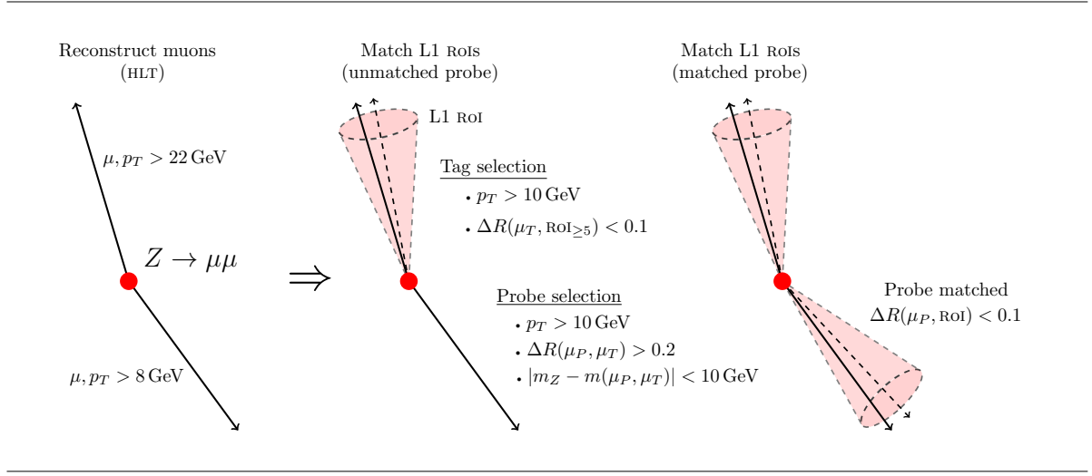
Figure 4.1: Schematic of the Z \rightarrow \mu\mu tag and probe selection criteria used for online muon efficiency monitoring.
