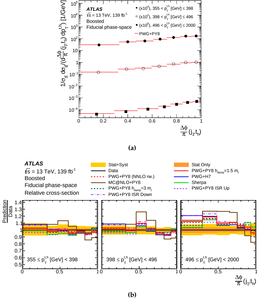
Figure A.4: Normalised double-differential cross-section measurement as a function of \Delta\phi(j_1, t_h) in bins of p_T^{th} . (a) Measured differential cross-section compared directly with predictions from the POWHEG+PYTHIA8 MC event generator. The measurement and predictions are multiplied by the factors shown in parentheses to aid visibility. (b) The ratio of the measured normalised cross-section to different NLO + PS and re-weighted NNLO SM predictions. The yellow band shows the size of the total uncertainty, while the orange band shows the statistical uncertainty only.
