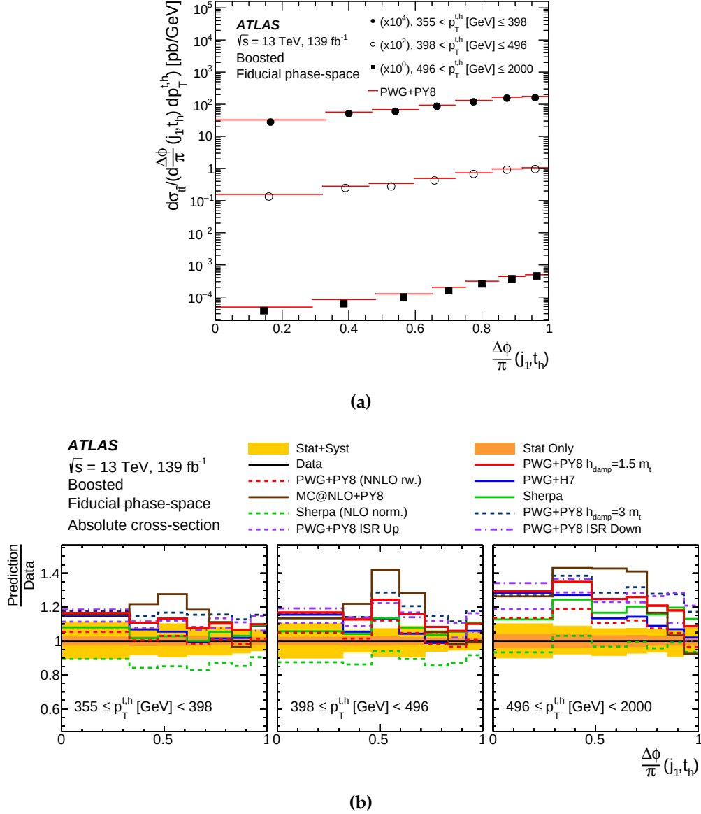
Figure 10.10: Double-differential fiducial cross-section measurement as a function of \Delta\phi(j_1, t_h) in bins of p_T^{th} .
