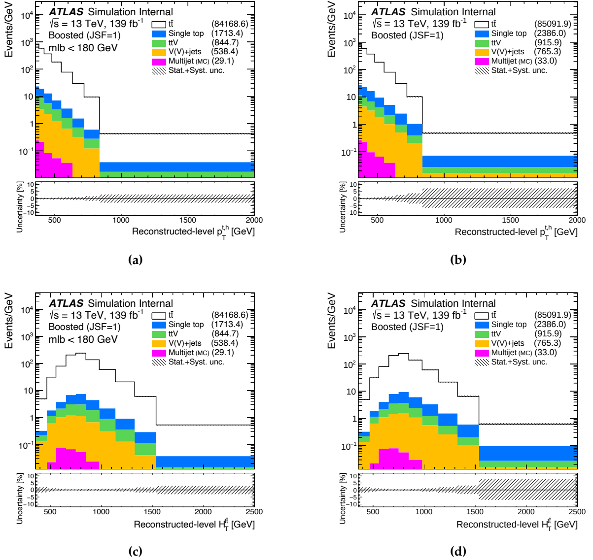
Figure 9.3: Detector-level distribution with/without the m_{\ell,b} < 180 \text{ GeV} requirement for (a)/(b) p_T^{t,h} , (c)/(d) H_T^{t\bar{t}} . The dashed band represents the combined statistical and background modelling uncertainties. A different multijet estimation is used in these plots and the multijet uncertainty discussed in Section 9.3.1 is not included. The overflow and underflow are included.
