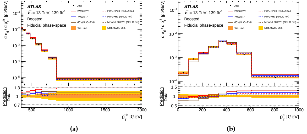
Figure 10.2: Fiducial t\bar{t} cross-section measured as a function of (a) p_T^{t,h} and (b) p_T^{t,l} . Measured results are compared to SM predictions from various NLO generators with (dashed lines) and without (solid lines) the NNLO re-weighting applied. The yellow band shows the size of the total uncertainty in each bin, while the orange band shows the statistical uncertainty only. The lower panel displays the ratios between the different predictions and data.
