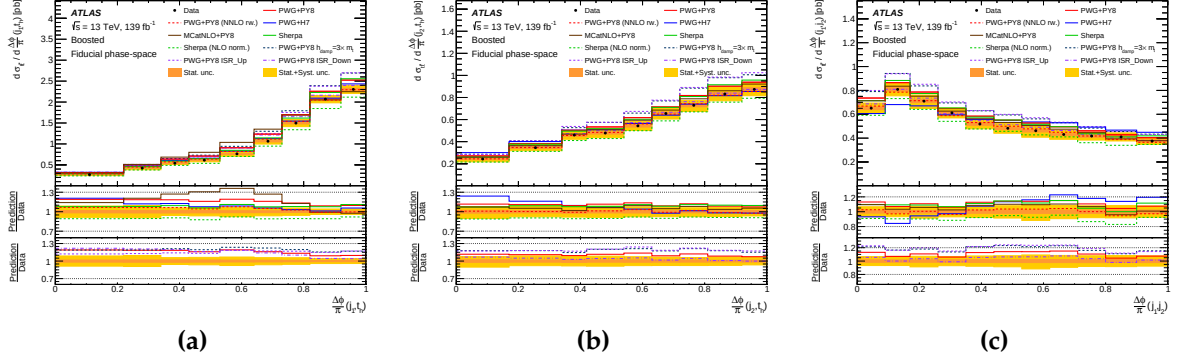
Figure 10.8: Fiducial t\bar{t} cross-section measured as a function of (a) \Delta\phi(j_1, t_h) , (b) \Delta\phi(j_2, t_h) , and (c) \Delta\phi(j_1, j_2) . Measured results are compared to SM predictions from various NLO + PS generator setups with different shower and radiation settings. The yellow band shows the size of the total uncertainty in each bin, while the orange band shows the statistical uncertainty only. The two lower panels display the ratios between the different predictions and data.
