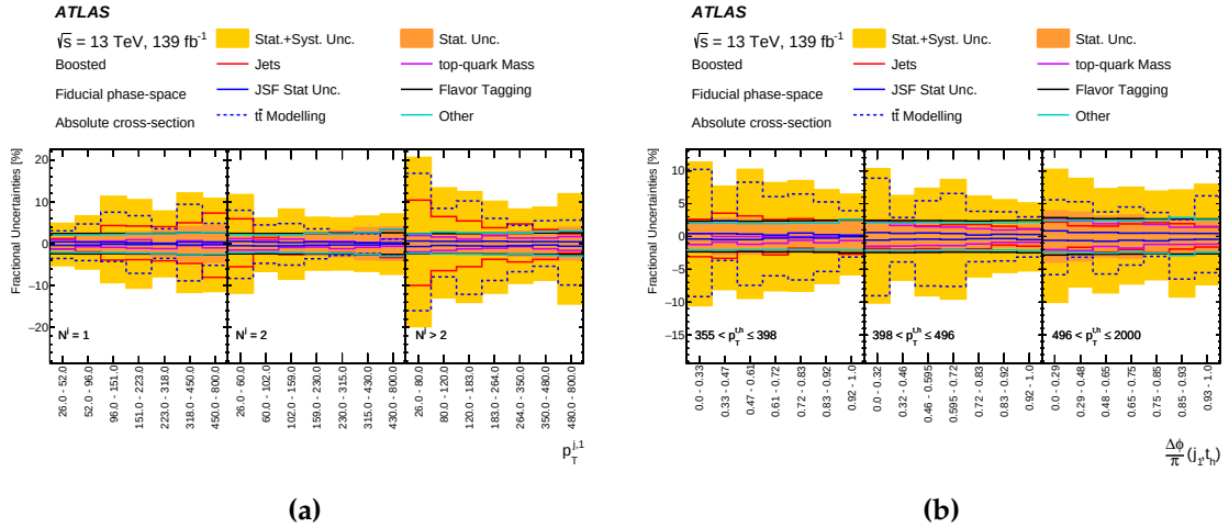
Figure 9.14: Fractional uncertainties for the particle-level cross section as a function of (a) p_T^{j,1} in regions of N^j , (b) \Delta\phi(j_1, t_h) in regions of p_T^{j,1} . The line labelled t\bar{t} modelling includes all uncertainties discussed in Section 9.4, with the exception of the uncertainty on the top-quark mass. The yellow band represents the total uncertainty while the orange band shows the statistical component only.
