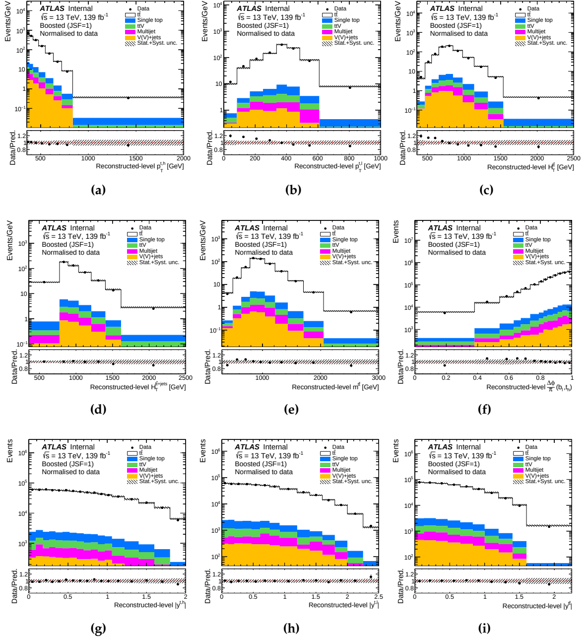
Figure 8.5: Detector-level distributions of the number of events as a function of (a) p_T^h , (b) p_T^l , (c) H_T^l , (d) H_T^{l+jets} , (e) m^{l\bar{l}} , (f) \Delta\phi(b_\ell, t_h) , (g) |y^{t,h}| , (h) |y^{t,l}| , and (i) |y^{t\bar{l}}| . The data are compared to the expectation from simulation and background estimates normalised to match the number of entries in data. The lower panel in each subfigure shows the ratio of the data to the normalised expectation. The dashed band represents the total statistical and systematic uncertainty but does not include modelling uncertainties.
