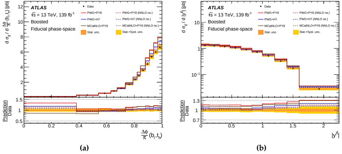
Figure 10.4: Fiducial t\bar{t} cross-section measured as a function of (a) \Delta\phi(b_\ell, t_\ell) and (b) |y^{t\bar{t}}| . Measured results are compared to SM predictions from various NLO generators with (dashed lines) and without (solid lines) the NNLO re-weighting applied. The yellow band shows the size of the total uncertainty in each bin, while the orange band shows the statistical uncertainty only. The lower panel displays the ratios between the different predictions and data.
