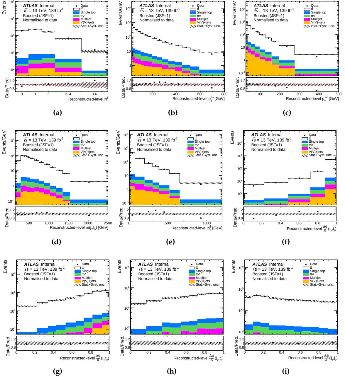
Figure 8.6: Detector-level distributions of the number of events as a function of (a) N^j , (b) p_T^{j1} , (c) p_T^{j2} , (d) m(j_1, t_h) , (e) p_T^{t\bar{t}} , (f) \Delta\phi(t_h, t_\ell) , (g) \Delta\phi(j_1, t_h) , (h) \Delta\phi(j_2, t_h) , and (i) \Delta\phi(j_1, j_2) . The data are compared to the expectation from simulation and background estimates normalised to match the number of entries in data. The lower panel in each subfigure shows the ratio of the data to the normalised expectation. The dashed band represents the total statistical and systematic uncertainty but does not include modelling uncertainties.
