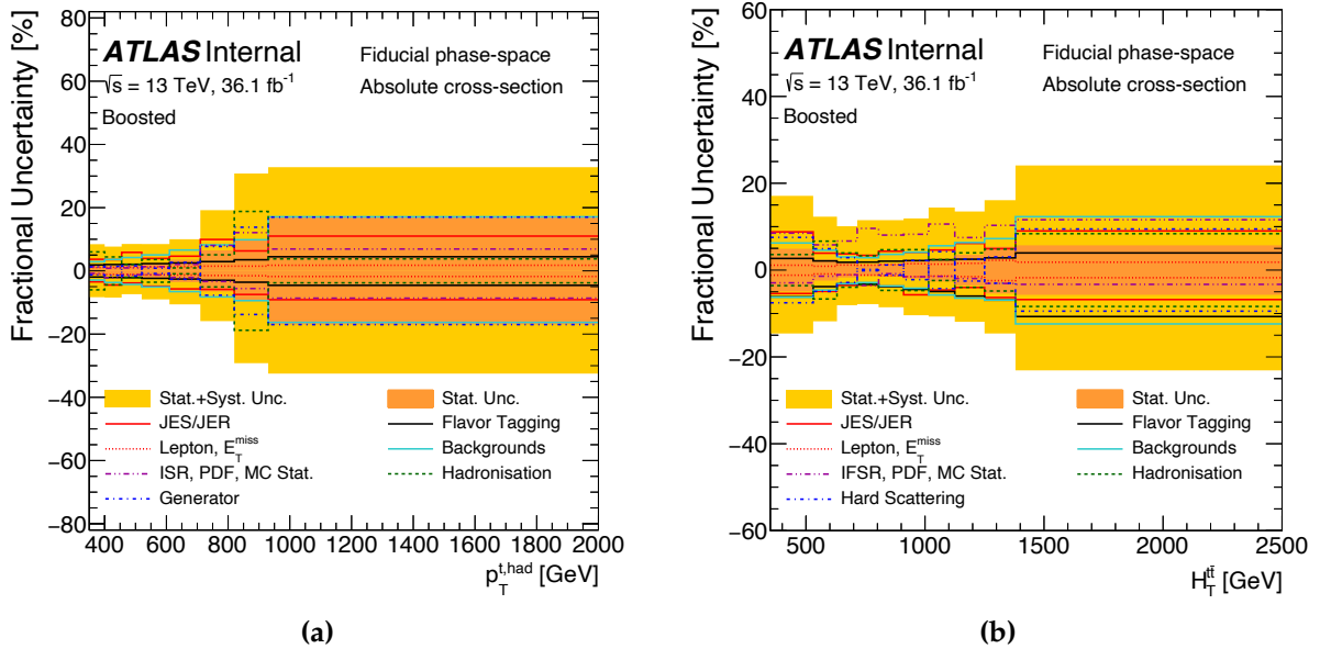
Figure 9.5: Fractional uncertainties on the absolute particle-level cross-section as a function of (a) p_T^{t,h} , (b) H_T^{t\bar{t}} from the preceding 36 fb -1 ATLAS t\bar{t} measurement [124]. In these results the combined JES and JER components (red) make up the dominant detector uncertainty in most bins. Additionally the large background uncertainties (cyan) in the tails of the distributions are dominated by the DS/DR single-top uncertainty demonstrating the likely scale of this without a maximum m_{\ell,b} requirement.
