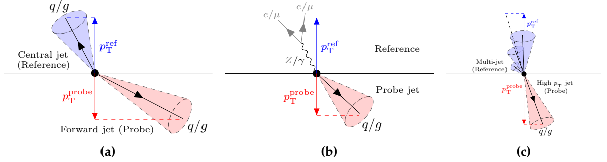
Figure 5.5: Example diagrams showing the processes used in the in-situ calibration of small-radius jets: (a) \eta -intercalibration, (b) Z/\gamma + \text{jet} , (c) multi-jet balance.
