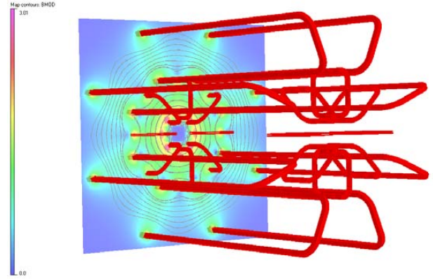
Figure 3.10: Simulated mapping of the magnetic field generated by the ATLAS superconducting toroid. Unlike the solenoid, the toroidal field is not perfectly uniform [64].
