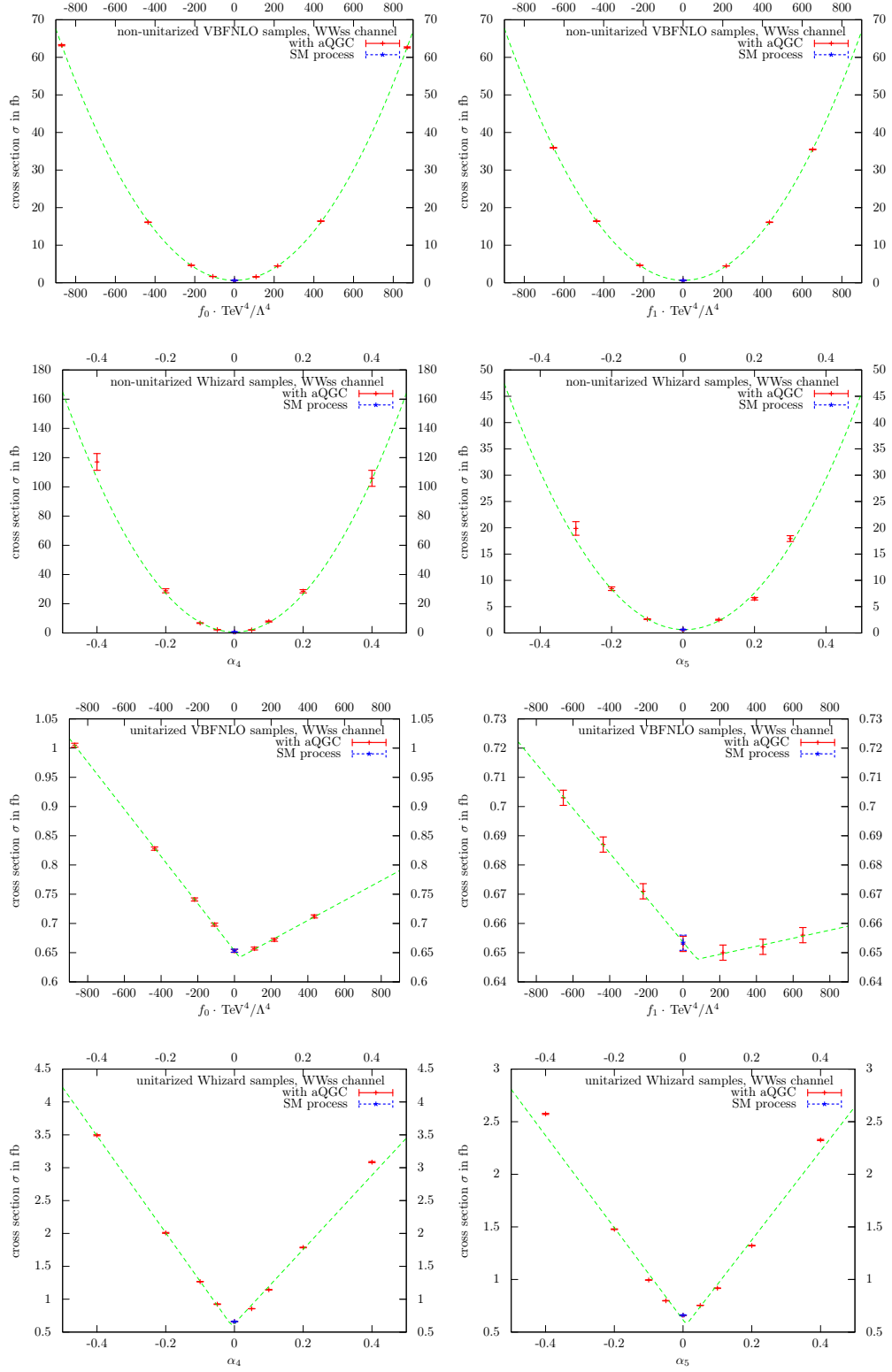
Figure C.2: Dependency of \sigma on the aQGC parameter f_0 for the WWss channel. Red crosses correspond to the cross sections of the generated samples. Blue data points refer to the cross section of the samples generated using the mode for the SM process. The green dashed line is a parabolic fit for non-unitarized samples. For the unitarized samples it is a combination of two linear fits with independent slopes for different values for the aQGC parameter.
