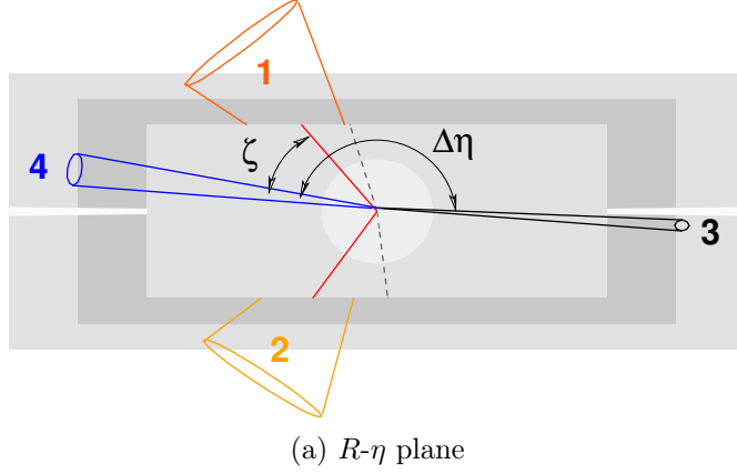
Figure 2.4: Schematic view of a Vector Boson Scattering event in the ATLAS detector. 1 and 2 are leptons and 3 and 4 are jets. Observables \Delta\eta_{jj} and \zeta_{ll} as described in the text are shown. Graph is taken from [10].
