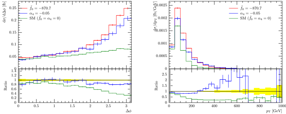
Figure C.22: Comparison of values for aQGC parameter f_0 and \alpha_4 , with similar cross section, with f_1 = \alpha_5 = 0 , in the WWss channel. Unitarization was applied. The left distribution shows the differential cross section over |\Delta\phi(\ell\ell)| of the most forward lepton. The right distribution shows the differential cross section dependency on the transverse momentum of the leading lepton p_T(\ell_1) .
