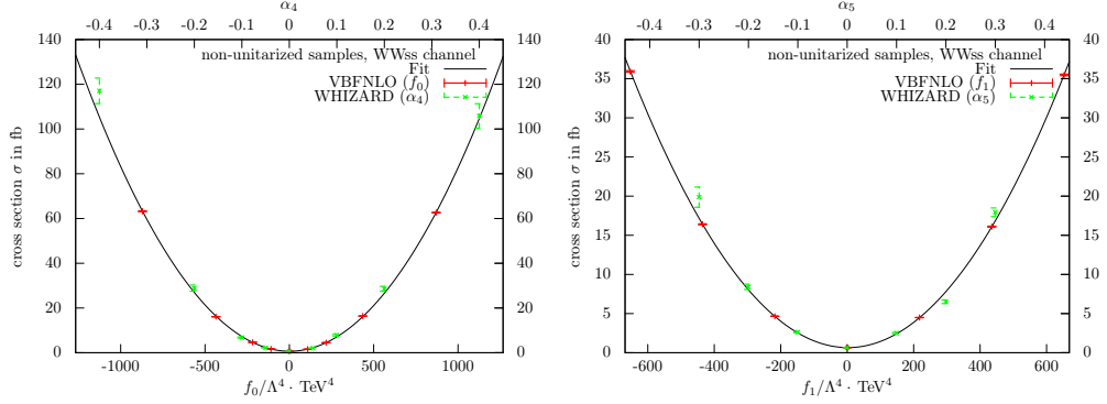
Figure C.17: Dependency of \sigma on the aQGC parameter f_i and \alpha_{i+4} for the WW_{ss} channel, non-unitarized samples. Left: parameters f_0 and \alpha_4 . Right: parameters f_1 and \alpha_5 . Red crosses correspond to the cross sections of the samples generated by VBFNLO. Green data points refer to the cross section of the samples generated by WHIZARD. The black line is a parabolic fit for all samples. f_i -axis was scaled to match \alpha_{i+4} -axis according to fit parameter t_i .
