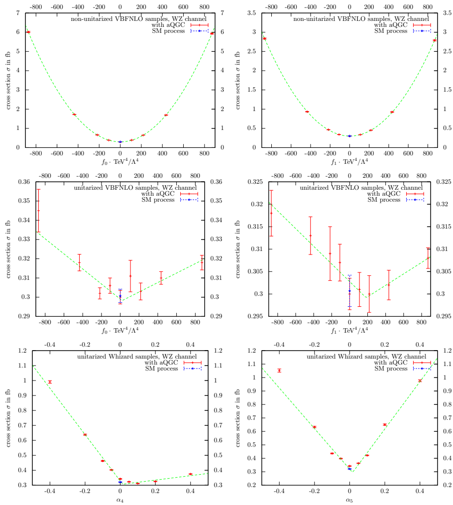
Figure C.1: Dependency of total cross sections on the aQGC parameter for different samples in the WZ channel. For further information see next figure.
