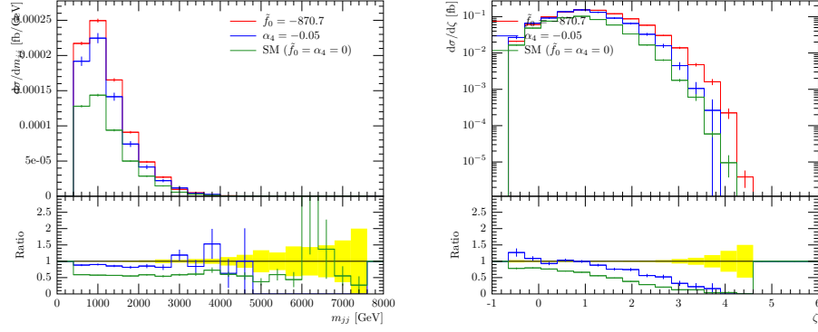
Figure C.23: Comparison of values for aQGC parameter f_0 and \alpha_4 , with similar cross section, with f_1 = \alpha_5 = 0 , in the WWss channel. Unitarization was applied. The left distribution shows the differential cross section over the invariant mass of the jet pair M_{jj} . The right distribution shows the differential cross section dependency on the transverse momentum of the lepton centrality \zeta .
