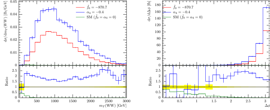
Figure 8.2: Comparison of values for aQGC parameter f_0 and \alpha_4 , that are predicted to match, with f_1 = \alpha_5 = 0 , in the WWss channel. No unitarization was used. The left distribution shows the differential cross section over m_T(WW) . The right distribution shows the differential cross section dependency on the absolute value of the angle between the projections of the leptons' momenta in the x - y plane \Delta\phi(\ell\ell) . In the ratio plot the ratio to the distribution with \tilde{f}_0 = -870.7 is given.
