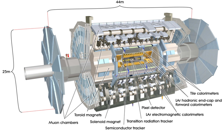
Figure 3.2: Schematic overview of the ATLAS detector. Graphic is taken from [17].
