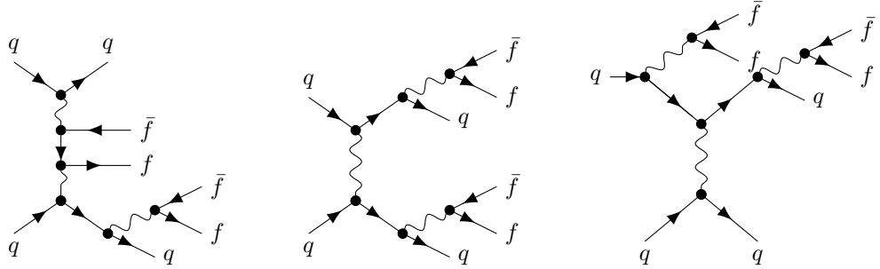
Figure 2.3: Feynman graphs of other processes with the same final state as VBS. These are not gauge invariantly separable processes.
