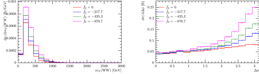
Figure C.7: Comparison of different values for aQGC parameter f_0 , with f_1 = 0 , in the WWss channel. Unitarization was applied. The left distribution shows the differential cross section over the transverse mass of the pair of vector bosons m_T(WW) . The right distribution shows the differential cross section dependency on the absolute value of the angle between the projections of the leptons' momenta in the x - y plane \Delta\phi(\ell\ell) . The different colors represent different values for \tilde{f}_0 as listed in the key.
