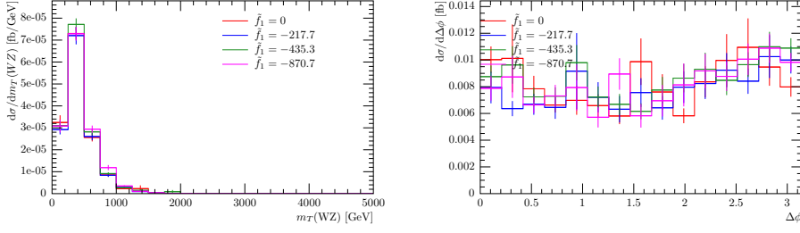
Figure C.14: Comparison of different values for aQGC parameter f_1 , with f_0 = 0 , in the WZ channel. Unitarization was applied. The left distribution shows the differential cross section over the transverse mass of the pair of vector bosons m_T(WZ) . The right distribution shows the differential cross section dependency on the absolute value of the angle between the projections of the vector bosons' momenta in the x - y plane \Delta\phi(WZ) . The different colors represent different values for f_0 as listed in the key.
