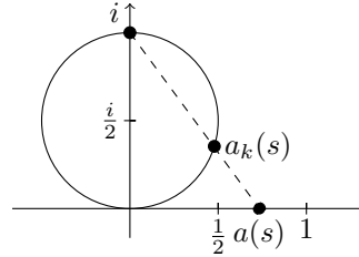
Figure 2.7: Schematic diagram of the k matrix method and the Argand circle. a(s) is projected onto the Argand circle resulting in point a_k(s) . Since all point on the Argand circle obey the unitarity criterion these projections are unitarized.
