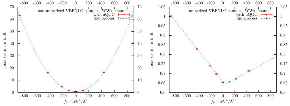
Figure 6.1: Dependency of \sigma on the aQGC parameter f_0 for the WWss channel. Left: non-unitarized samples. Right: unitarized samples. Red crosses correspond to the cross sections of the generated samples. Blue data points refer to the cross section of the samples generated using the mode for the SM process. The green dashed line is a parabolic fit for non-unitarized samples. For the unitarized samples it is a combination of two linear fits with independent slopes for different values for the aQGC parameter. Other channels and parameters can be found in appendix C.1
