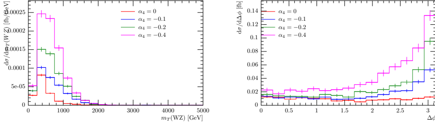
Figure C.15: Comparison of different values for aQGC parameter \alpha_4 , with \alpha_5 = 0 , in the WZ channel. Unitarization was applied. The left distribution shows the differential cross section over the transverse mass of the pair of vector bosons m_T(WZ) . The right distribution shows the differential cross section dependency on the absolute value of the angle between the projections of the vector bosons' momenta in the x - y plane \Delta\phi(WZ) . The different colors represent different values for f_0 as listed in the key.
