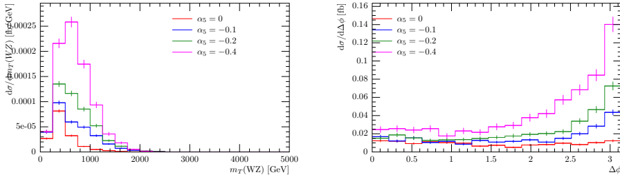
Figure C.16: Comparison of different values for aQGC parameter \alpha_5 , with \alpha_4 = 0 , in the WZ channel. Unitarization was applied. The left distribution shows the differential cross section over the transverse mass of the pair of vector bosons m_T(WZ) . The right distribution shows the differential cross section dependency on the absolute value of the angle between the projections of the vector bosons' momenta in the x - y plane \Delta\phi(WZ) . The different colors represent different values for f_0 as listed in the key.
