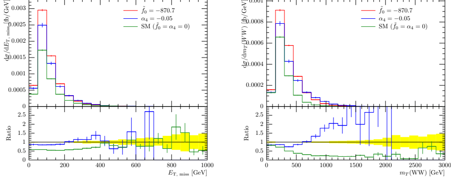
Figure C.20: Comparison of values for aQGC parameter f_0 and \alpha_4 , with similar cross section, with f_1 = \alpha_5 = 0 , in the WWss channel. Unitarization was applied. The left distribution shows the differential cross section over E_T^{\text{miss}} . The right distribution shows the differential cross section dependency on the invariant mass of the vector boson pair m_T(WW) .
