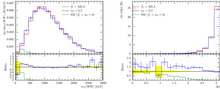
Figure 8.3: Comparison of values for aQGC parameter f_1 and \alpha_5 , with similar cross section, with f_0 = \alpha_4 = 0 , in the WWss channel. No unitarization was used. The left distribution shows the differential cross section over m_T(WW) . The right distribution shows the differential cross section dependency on the absolute value of the angle between the projections of the leptons' momenta in the x - y plane \Delta\phi(\ell\ell) . In the ratio plot the ratio to the distribution with \tilde{f}_1 = -435.3 is given.
