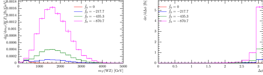
Figure C.11: Comparison of different values for aQGC parameter f_0 , with f_1 = 0 , in the WZ channel. No unitarization was used. The left distribution shows the differential cross section over the transverse mass of the pair of vector bosons m_T(WZ) . The right distribution shows the differential cross section dependency on the absolute value of the angle between the projections of the vector bosons' momenta in the x - y plane \Delta\phi(WZ) . The different colors represent different values for \tilde{f}_0 as listed in the key.
