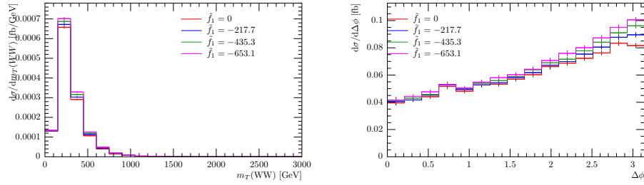
Figure C.8: Comparison of different values for aQGC parameter f_1 , with f_0 = 0 , in the WWss channel. Unitarization was applied. The left distribution shows the differential cross section over the transverse mass of the pair of vector bosons m_T(WW) . The right distribution shows the differential cross section dependency on the absolute value of the angle between the projections of the leptons' momenta in the x - y plane \Delta\phi(\ell\ell) . The different colors represent different values for \tilde{f}_0 as listed in the key.
