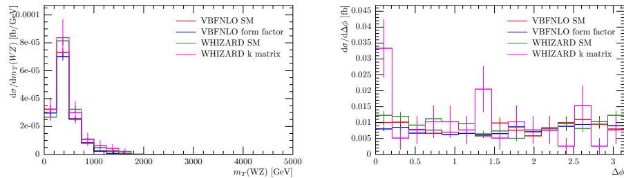
Figure 5.2: Comparison of different models for the WZ SM process. The left distribution shows the differential cross section over the transverse mass of the pair of vector bosons m_T(WZ) . The right distribution shows the differential cross section dependency on the absolute value of the angle between the projections of the vector bosons’ momenta in the x - y plane \Delta\phi(WZ) . The red and green lines show the distributions of the SM process generated by VBFNLO or WHIZARD respectively. The blue and magenta distributions are generated using the SM extended with aQGC (SM values) by VBFNLO or WHIZARD respectively.
