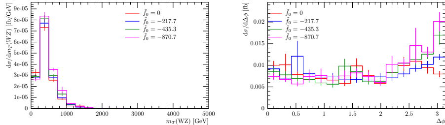
Figure C.13: Comparison of different values for aQGC parameter f_0 , with f_1 = 0 , in the WZ channel. Unitarization was applied. The left distribution shows the differential cross section over the transverse mass of the pair of vector bosons m_T(WZ) . The right distribution shows the differential cross section dependency on the absolute value of the angle between the projections of the vector bosons' momenta in the x - y plane \Delta\phi(WZ) . The different colors represent different values for \tilde{f}_0 as listed in the key.
