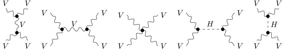
Figure 2.2: Feynman graphs for all possible VBS channels. Initial and final state as shown in figure 2.1
