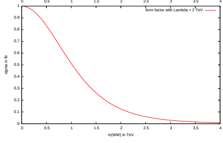
Figure 2.6: Shape of implemented form factor using the parameters \Lambda_{FF} = 2 \text{ TeV} and n = 2 .
