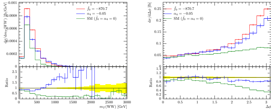
Figure 8.6: Comparison of values for aQGC parameter f_0 and \alpha_4 , with similar cross section, with f_1 = \alpha_5 = 0 , in the WWss channel. Unitarization was applied. The left distribution shows the differential cross section over m_T(WW) . The right distribution shows the differential cross section dependency on the absolute value of the angle between the projections of the leptons' momenta in the x - y plane \Delta\phi(\ell\ell) . In the ratio plot the ratio to the distribution with \tilde{f}_0 = -870.7 is given.
