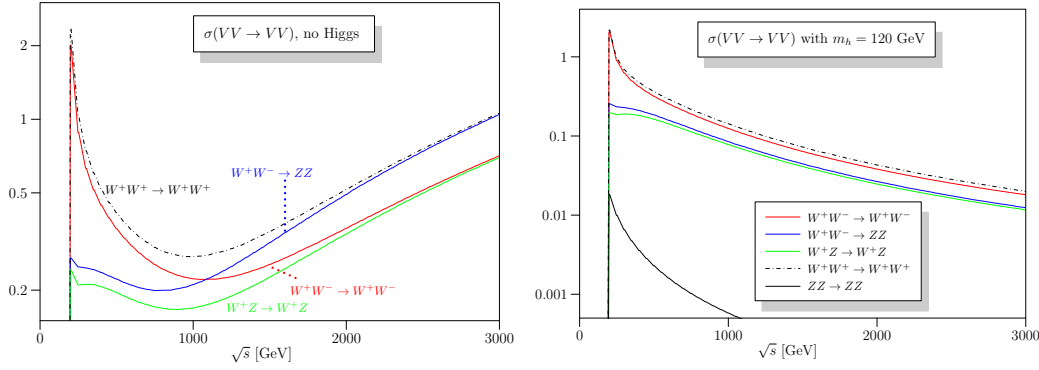
Figure 2.5: Cross sections for different Vector Boson Scattering processes. Left: Without a Higgs boson. Right: With SM-Higgs boson of mass 120 GeV. Graphics taken from [9].
