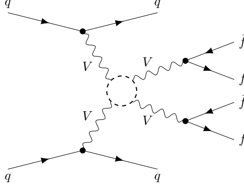
Figure 2.1: Feynman graph of a general VBS process. Straight lines with arrows represent fermions. Curved lines represent vector bosons. Dashed circle stands for the different possibilities of interactions between the vector bosons shown in figure 2.2.
