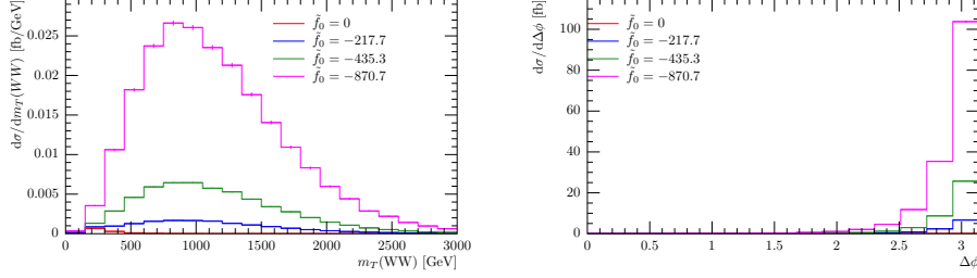
Figure 7.1: Comparison of different values for aQGC parameter f_0 , with f_1 = 0 , in the W\bar{W}ss channel. No unitarization was used. The left distribution shows the differential cross section over the transverse mass m_T(WW) . The right distribution shows the differential cross section dependency on the absolute value of the angle between the projections of the leptons' momenta in the x - y plane \Delta\phi(l\bar{l}) . The different colors represent different values for \tilde{f}_0 as listed in the key.
