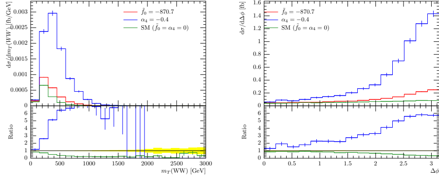
Figure 8.5: Comparison of values for aQGC parameter f_0 and \alpha_4 , that are predicted to match, with f_1 = \alpha_5 = 0 , in the WWss channel. Unitarization was applied. The left distribution shows the differential cross section over m_T(WW) . The right distribution shows the differential cross section dependency on the absolute value of the angle between the projections of the leptons' momenta in the x - y plane \Delta\phi(\ell\ell) . In the ratio plot the ratio to the distribution with \tilde{f}_0 = -870.7 is given.
