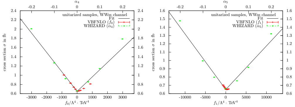
Figure C.18: Dependency of \sigma on the aQGC parameter f_i and \alpha_{i+4} for the WW_{ss} channel, unitarized samples. Left: parameters f_0 and \alpha_4 . Right: parameters f_1 and \alpha_5 . Red crosses correspond to the cross sections of the samples generated by VBFNLO. Green data points refer to the cross section of the samples generated by WHIZARD. The black line is a fit for all samples according to equation(8.1). f_i -axis was scaled to match \alpha_{i+4} -axis according to fit parameter t_i .
