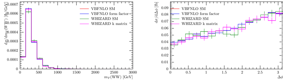
Figure 5.1: Comparison of different models for the WWss SM process. The left distribution shows the differential cross section over the transverse mass of the pair of vector bosons m_T(WW) . The right distribution shows the differential cross section dependency on the absolute value of the angle between the projections of the leptons’ momenta in the x - y plane \Delta\phi(l\bar{l}) . The red and green lines show the distributions of the SM process generated by VBFNLO or WHIZARD respectively. The blue and magenta distributions are generated using the SM extended with aQGC (SM values) by VBFNLO or WHIZARD respectively.
