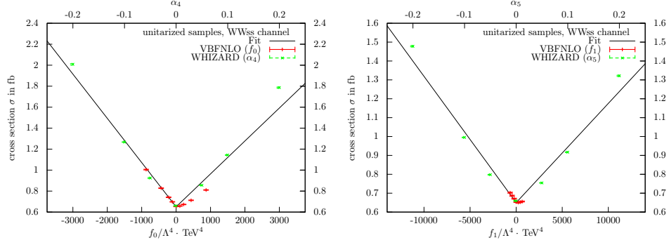
Figure 8.4: Dependency of \sigma on the aQGC parameter f_i and \alpha_{i+4} for the WWss channel, unitarized samples. Left: parameters f_0 and \alpha_4 . Right: parameters f_1 and \alpha_5 . Red crosses correspond to the cross sections of the samples generated by VBFNLO. Green data points refer to the cross section of the samples generated by WHIZARD. The black line is a fit for all samples according to equation (8.1). f_i -axis was scaled to match \alpha_{i+4} -axis according to fit parameter t_i . Other channels and parameters can be found in appendix C.3.
