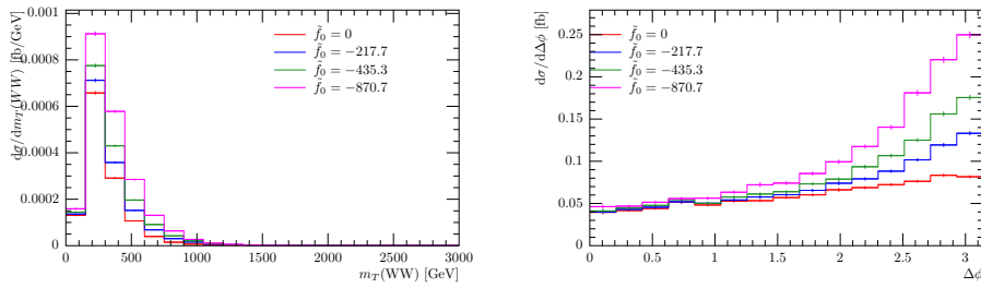
Figure 7.2: Comparison of different values for aQGC parameter f_0 in the W\bar{W}ss channel. For unitarization a form factor was applied. The left distribution shows the differential cross section over the transverse mass m_T(WW) . The right distribution shows the differential cross section dependency on the absolute value of the angle between the projections of the leptons' momenta in the x - y plane \Delta\phi(l\bar{l}) . The different colors represent different values for \tilde{f}_0 as listed in the key.
