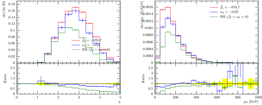
Figure C.21: Comparison of values for aQGC parameter f_0 and \alpha_4 , with similar cross section, with f_1 = \alpha_5 = 0 , in the WWss channel. Unitarization was applied. The left distribution shows the differential cross section over |\eta| of the most forward jet. The right distribution shows the differential cross section dependency on the transverse momentum of the leading jet p_T(j_1) .
