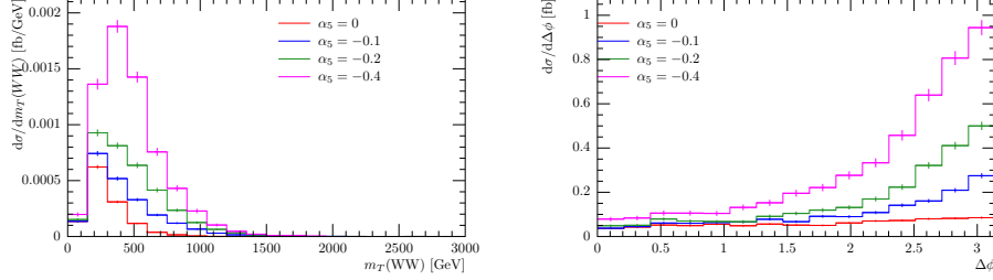
Figure C.10: Comparison of different values for aQGC parameter \alpha_5 , with \alpha_4 = 0 , in the WWss channel. Unitarization was applied. The left distribution shows the differential cross section over the transverse mass of the pair of vector bosons m_T(WW) . The right distribution shows the differential cross section dependency on the absolute value of the angle between the projections of the leptons' momenta in the x - y plane \Delta\phi(\ell\ell) . The different colors represent different values for \tilde{f}_0 as listed in the key.
