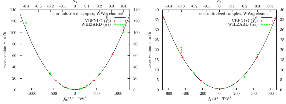
Figure 8.1: Dependency of \sigma on the aQGC parameter f_i and \alpha_{i+4} for the WWss channel, non-unitarized samples. Left: parameters f_0 and \alpha_4 . Right: parameters f_1 and \alpha_5 . Red crosses correspond to the cross sections of the samples generated by VBFNLO. Green data points refer to the cross sections of the samples generated by WHIZARD. The black line is a parabolic fit for all samples. f_i -axis was scaled to match \alpha_{i+4} -axis according to fit parameter t_i . Other channels and parameters can be found in appendix C.3.
