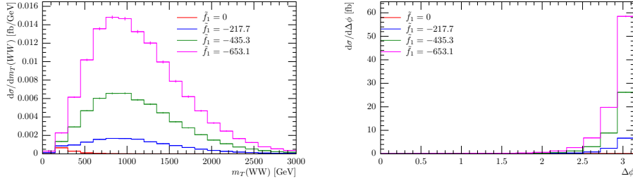
Figure C.4: Comparison of different values for aQGC parameter f_1 , with f_0 = 0 , in the WWss channel. No unitarization was used. The left distribution shows the differential cross section over the transverse mass of the pair of vector bosons m_T(WW) . The right distribution shows the differential cross section dependency on the absolute value of the angle between the projections of the leptons' momenta in the x - y plane \Delta\phi(\ell\ell) . The different colors represent different values for \tilde{f}_0 as listed in the key.
