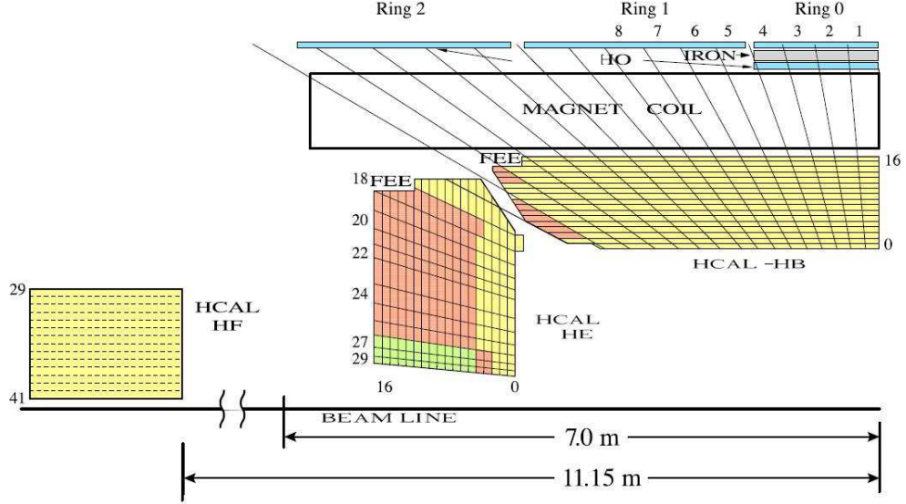
Figure 3.5: Structure of a quadrant of the CMS hadronic calorimeter in y-z plane with the hadronic barrel (HB), the the hadronic endcap (HE), the hadronic forward (HF) and the hadronic outer calorimeter (HO) [41]
