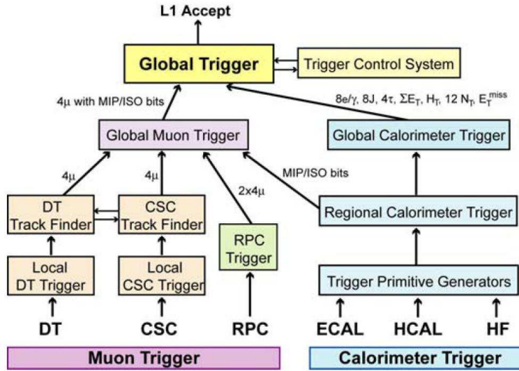
Figure 3.7: Structure of the Level-1 CMS Trigger [37]
