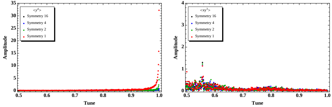
Figure 3.31: Discrete Fourier Transformation of the \langle y^4 \rangle (left) and \langle xy^3 \rangle (right) moment of the beam after 1024 turns.
