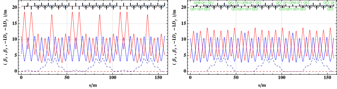
Figure 3.6: Example of a 21 cell FODO lattice with 3 \times 2 cells of straight section using a dispersion suppression by adjusting the phase advance to 2\pi over the arc. The mismatch caused by the missing dipoles in the straight section can be considerably reduced by additional individual matching quadrupoles next to the straight section and the dispersion matched to 0 in the straight sections.
