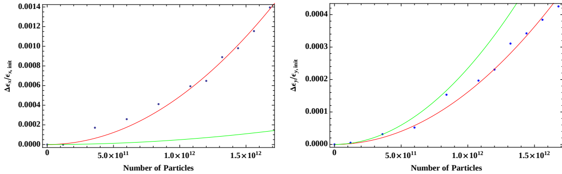
Figure 3.17: Difference between horizontal (left) and vertical (right) rms emittance of the undisturbed lattice and the rms emittance determined from the tracked distribution after 200 turns for a working point of Q_x/Q_y = 4.29/3.38 . In both planes the emittance increases quadratically with the intensity as derived in appendix H. The simulation results are shown in blue, the quadratic fit in red and the analytical estimation using Eqn. H.10 in green.
