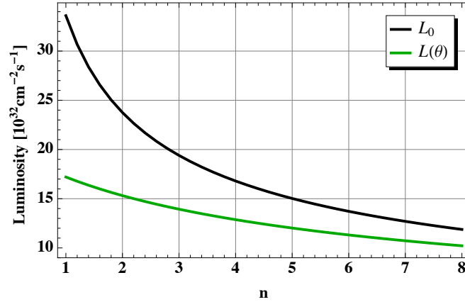
Figure 2.5: Maximum luminosity with ( L(\theta) ) and without ( L_0 ) geometric reduction factor S(\theta) versus ratio n between horizontal and vertical proton beam beta-functions at the IP assuming \beta_{yp}^* = \beta_{p,\text{min}}^* and a constant crossing angle of \theta = 1 mrad.
