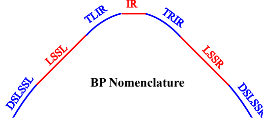
Figure 2.26: Bypass nomenclature: The straight sections are named Long Straight Section Left side (LSSL), Interaction Region (IR) - for the straight section parallel to the interaction region of the LHC - and Long Straight Section Right side (LSSR) and are marked in red. The dispersion suppressor sections are Dispersion Suppressor of LSSL (DSLSSL), Transfer line Left of IR (TLIR), Transfer line Right of IR (TRIR) and Dispersion Suppressor of LSSR (DSLSSR) and are indicated in blue.
