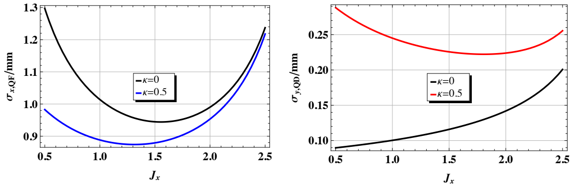
Figure 2.24: Horizontal beam size at the focusing quadrupole of the LHeC arc cell (left) and vertical beam size of the defocusing quadrupole of the LHeC arc cell (right) versus the horizontal damping partition J_x for two different emittance ratios \kappa = 0 and \kappa = 0.5 .
