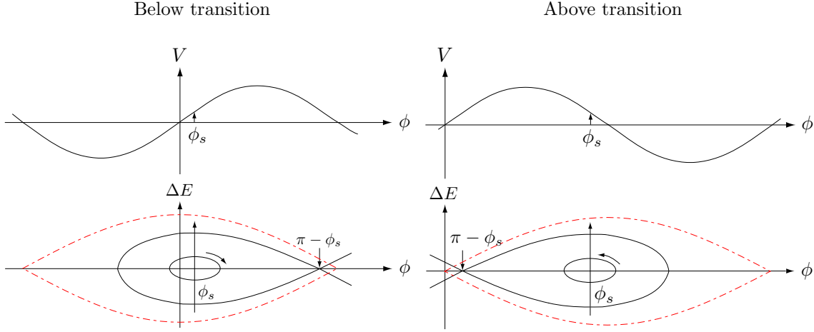
Figure 1.6: RF-voltage and bucket in the case of acceleration with a synchronous phase \phi_s . The bucket with \phi_s = 0 is shown in dot-dashed red . For \phi_s \neq 0 the energy and phase acceptance is reduced. For small phase and energy deviations the RF-voltage is approximately linear and the synchrotron motion can be described by an ellipse in the \Delta E - \phi -space, where the motion is clockwise below transition (left) and anticlockwise above transition (right).
