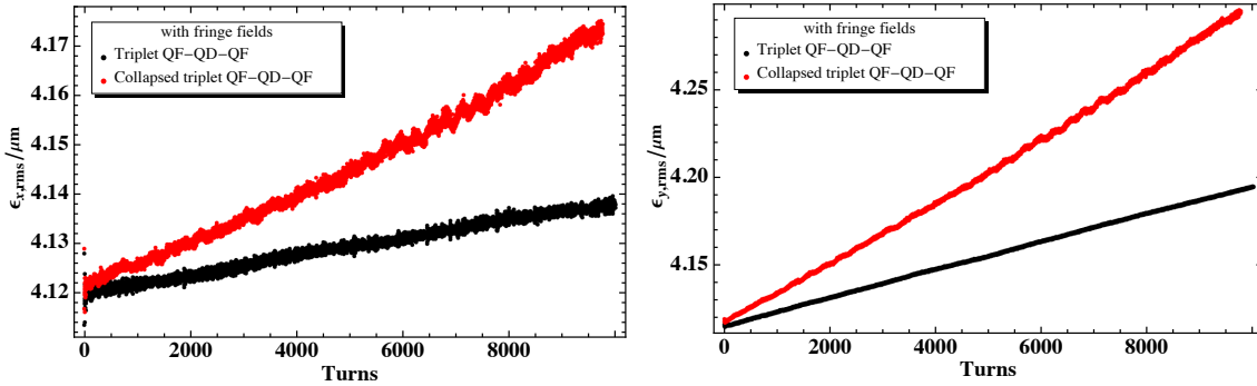
Figure 3.27: Time evolution of horizontal (left) and vertical (right) rms emittance for the triplet and collapsed triplet including fringe fields.
