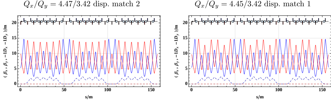
Figure 3.62: Optics of two different matches of the 21 cell FODO lattices with 3 \times 2 cells of straight section and a half missing bend dispersion suppressor scheme.
