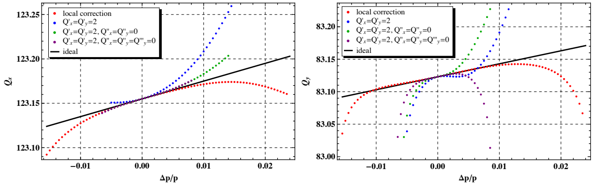
Figure 2.34: Dependence of the horizontal (left) and vertical (right) tune on the momentum deviation. The tune is calculated with PTC as MAD-X might not deliver correct results for large momentum deviations. Ideally, the chromaticity would be linear with Q'_{x/y} = 2 , which is indicated by a black line.
