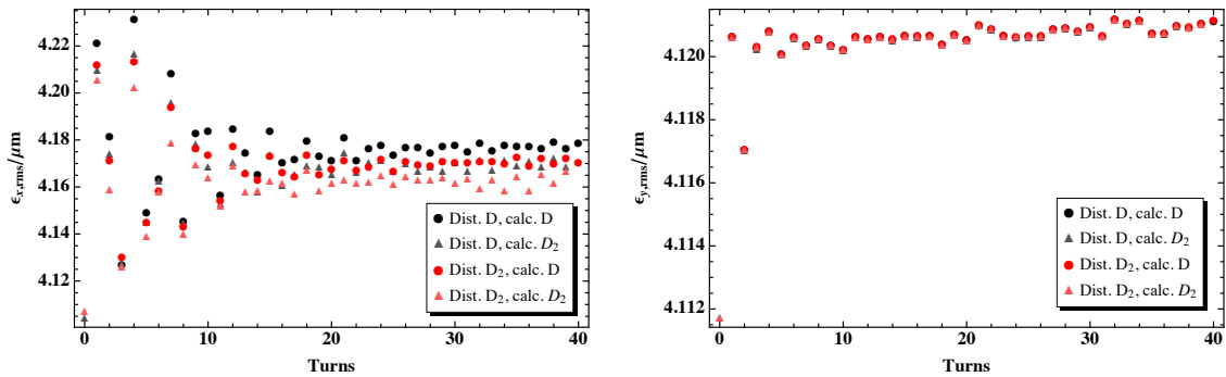
Figure 3.50: Time evolution over the first 40 turns of the horizontal (left) and vertical (right) rms emittance for the 24 cell FODO lattice with 4 \times 1 cells of straight sections with a working point of Q_x/Q_y = 4.47/3.45 . The initial distribution has been generated taking only the linear dispersion (Dist. D) and the linear and second order dispersion (Dist. D_2 ) into account. The same is valid for the emittance which has been calculated including only the linear dispersion (calc. D) and the linear and second order dispersion (calc. D_2 ).
