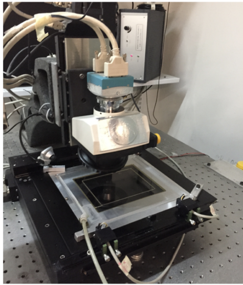
Figure 4.1: Optical microscope used in emulsion scanning (left). Diagram illustrating the scanning process (right) [2].
