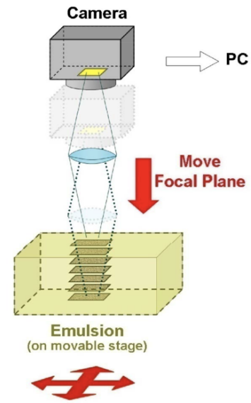
Figure 4.1: Optical microscope used in emulsion scanning (left). Diagram illustrating the scanning process (right) [2].
