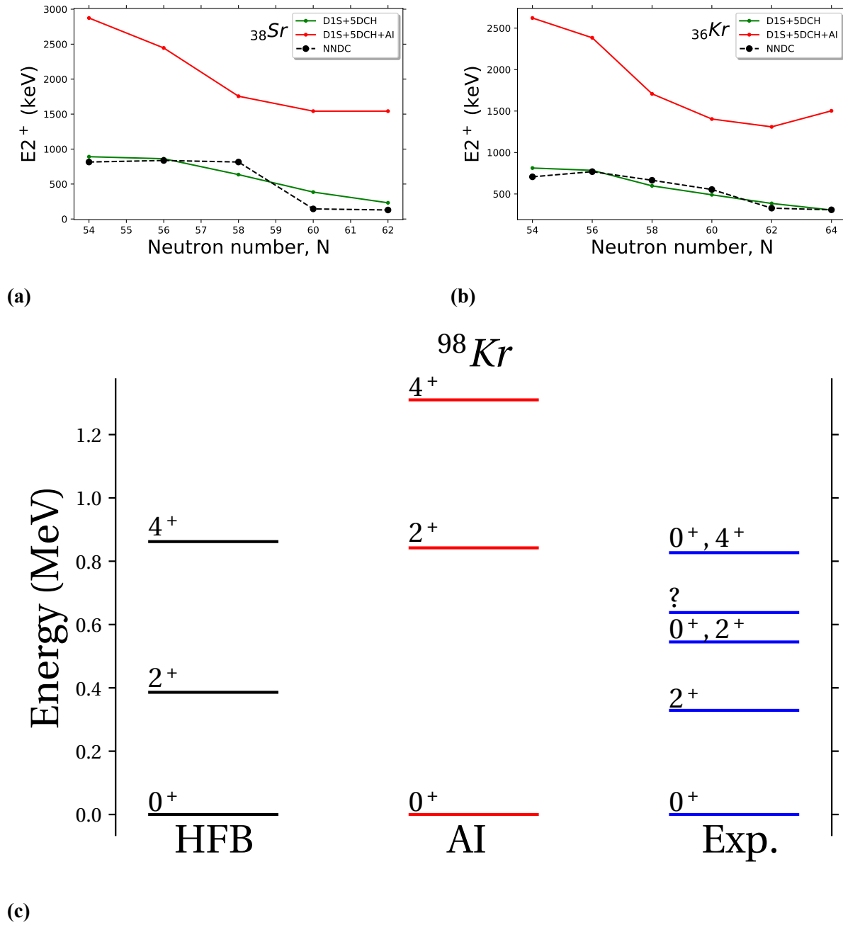
Figure 3.14. (a)- the first 2^+ excited states in ^{38}\text{Sr} isotopes. (b)- the first 2^+ excited states in ^{36}\text{Kr} isotopes. (c)- the representation of the energy levels for ^{98}\text{Kr} isotope. The HFB value is calculated by HFB approach with Gogny interaction, the AI value calculated by the same approach but with artificial neural network, experimental values are taken from [Lab].
