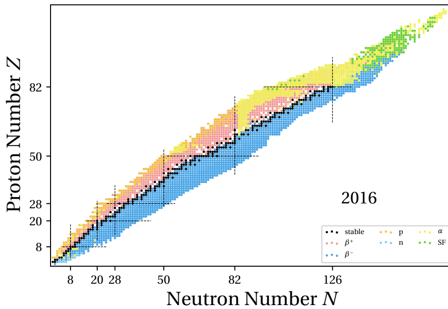
Figure 1.1. The nuclear chart presenting all experimentally known isotopes. Each square represents a nuclide and the colors represent main decay modes.
