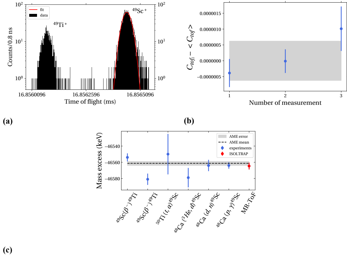
Figure 2.11. (a)- the Gaussian fit of ^{49}\text{Sc} ions. (b)-the difference between individual C_{Tof_i} and weighted \overline{C_{Tof}} . The total uncertainty is shown with a grey band. (c)-the experimental mass excess values of ^{49}\text{Sc} are taken from [R + 61, F + 69, E + 66, W + 66, G + 68, V + 68]. For a better visibility, the values from [O + 56, M + 56] are excluded from the plot since they have uncertainties of 50 and 100 keV.
