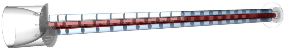
Figure 2.2. The basic layout of the RFQ buncher. It consists of an egg-cup electrode, rod system, and ejection electrodes [And18].
