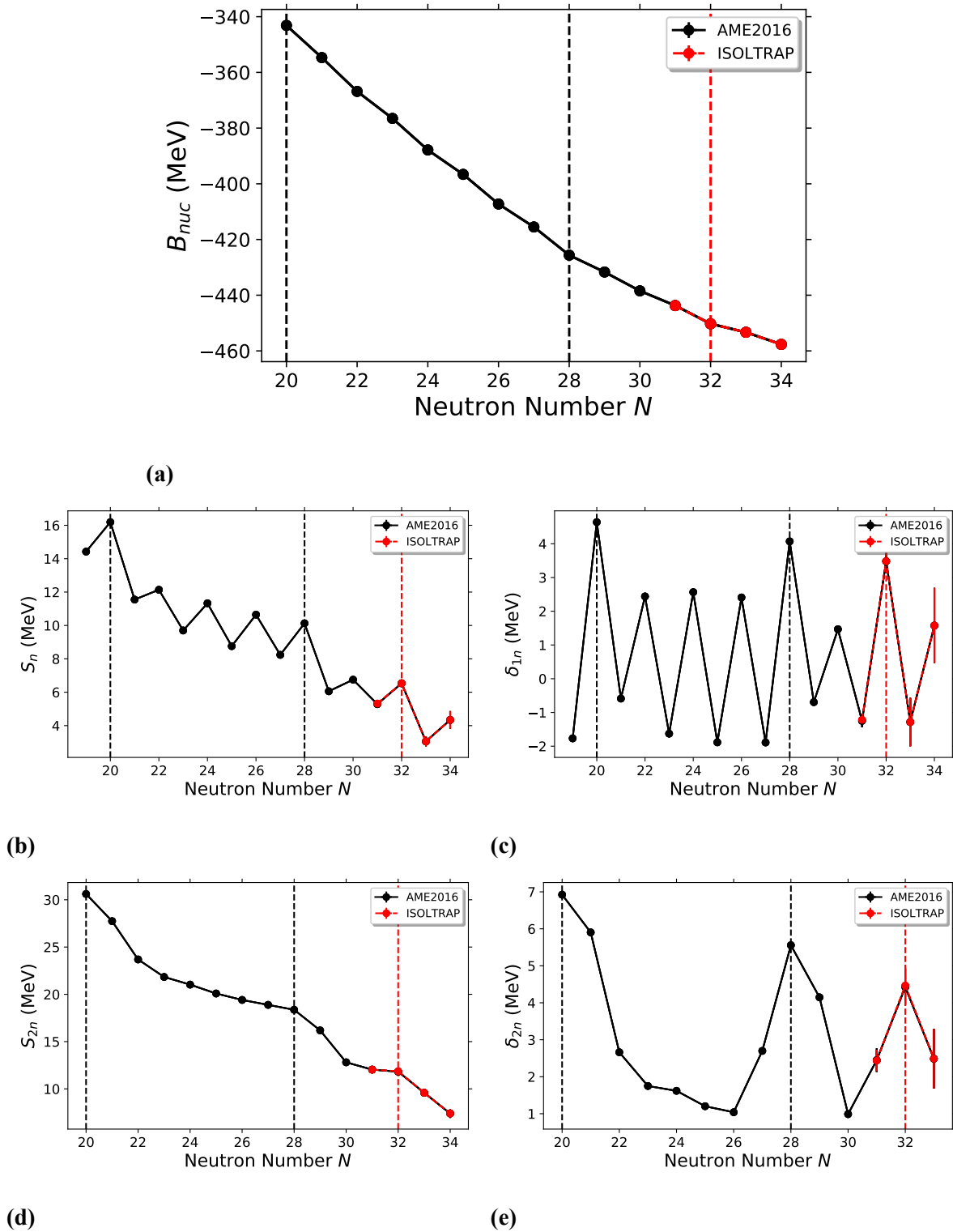
Figure 1.2. (a)- the trend of the binding energy in calcium isotopic chain [ H^+17 ]. (b)- one neutron separation energy in calcium isotopic chain. (c)- one neutron shell-gap energy in calcium isotopic chain. (d)- Two neutron separation energy in calcium isotopic chain. (e)- two neutron shell-gap energy in calcium isotopic chain.
