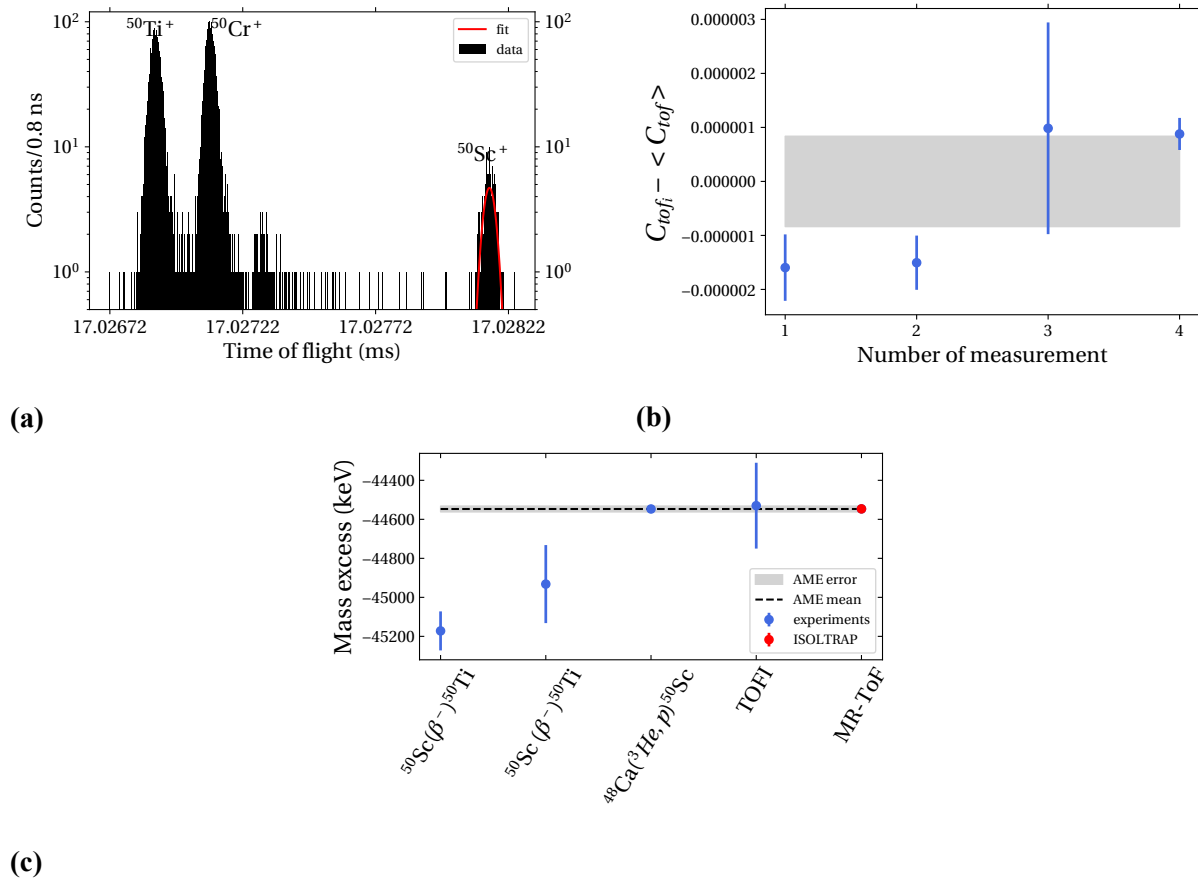
Figure 2.12. Same as figure 2.11 but for ^{50}\text{Sc} ions. The literature mass excess values of ^{50}\text{Sc} are taken from [W + 69, C + 63, O + 69, B + 98].
