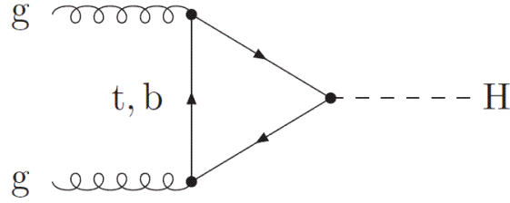
Figure 1.3: Feynman diagram contributing to gg \rightarrow H at lowest order.
