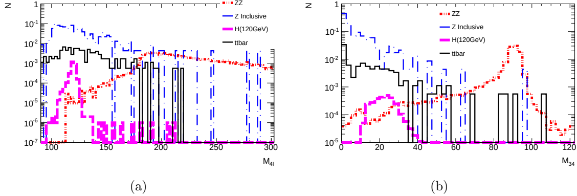
Figure 4.7: Mass distributions of the quadruplets of the 4\ell final state 4.7(a) and the non-leading dilepton pair 4.7(b) for t\bar{t} , ZZ , Z Inclusive processes and Higgs (120GeV) as signal for the luminosity of our Data ( 40 \text{ pb}^{-1} ).
