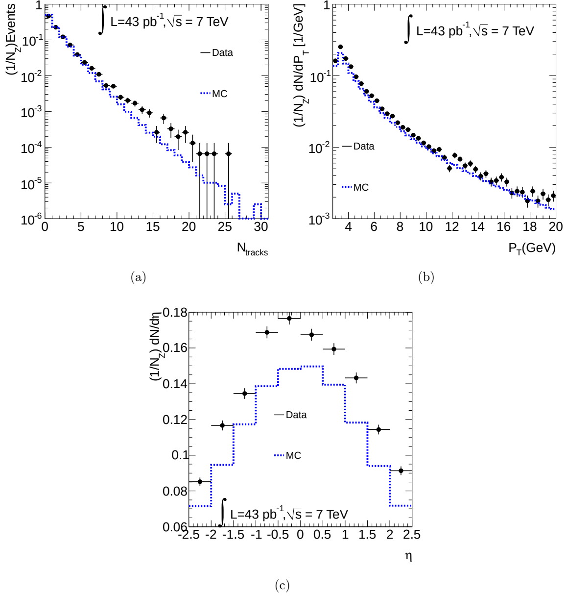
Figure 4.11: Additional tracks properties, 4.11(a) track multiplicity, 4.11(b) P_T and 4.11(c) \eta distributions. The selection is the same of the muons accompanying the Z boson.
