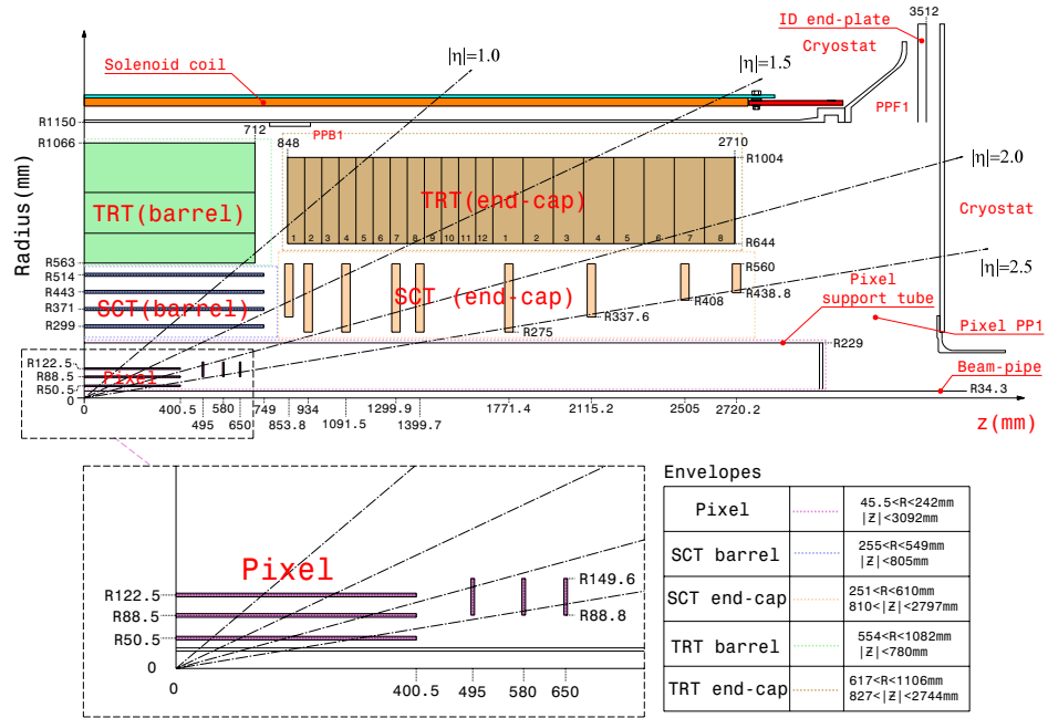
Figure 3.2: Plan view of a quarter-section of the ATLAS inner detector showing each of the major elements with its active dimensions.
