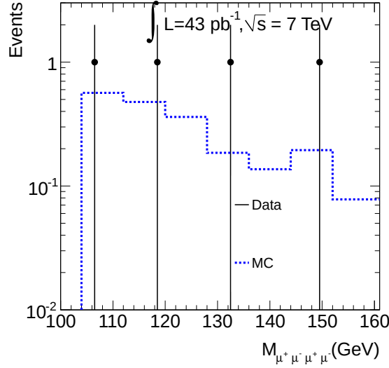
Figure 4.12: Mass distribution of four lepton events, where the non-leading dimuon is opposite sign and the P_T cut is 3GeV.
