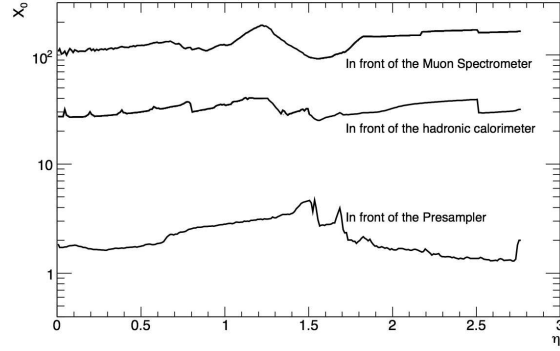
Figure 4.2: Material distribution before the Muon Spectrometer in ATLAS as a function of \eta . The material is expressed in radiation lengths ( X_0 ) [8].
