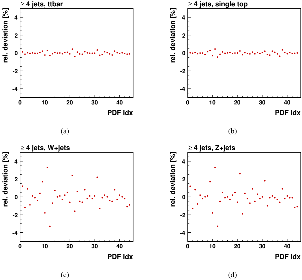
Figure 5.4: Impact of varying the values of the 22 orthogonal eigenvectors in the CTEQ6.6 PDF set within their 90% confidence interval boundaries on the expected event yields. In particular, the relative differences of expected event yields for the 44 eigenvector variations, denoted by PDF Idx, with respect to the central CTEQ6.6 PDF value are shown for t\bar{t} (a), single top quark (b), W +jets (c), and Z +jets (d) production, employing a requirement on at least four jets per event.
