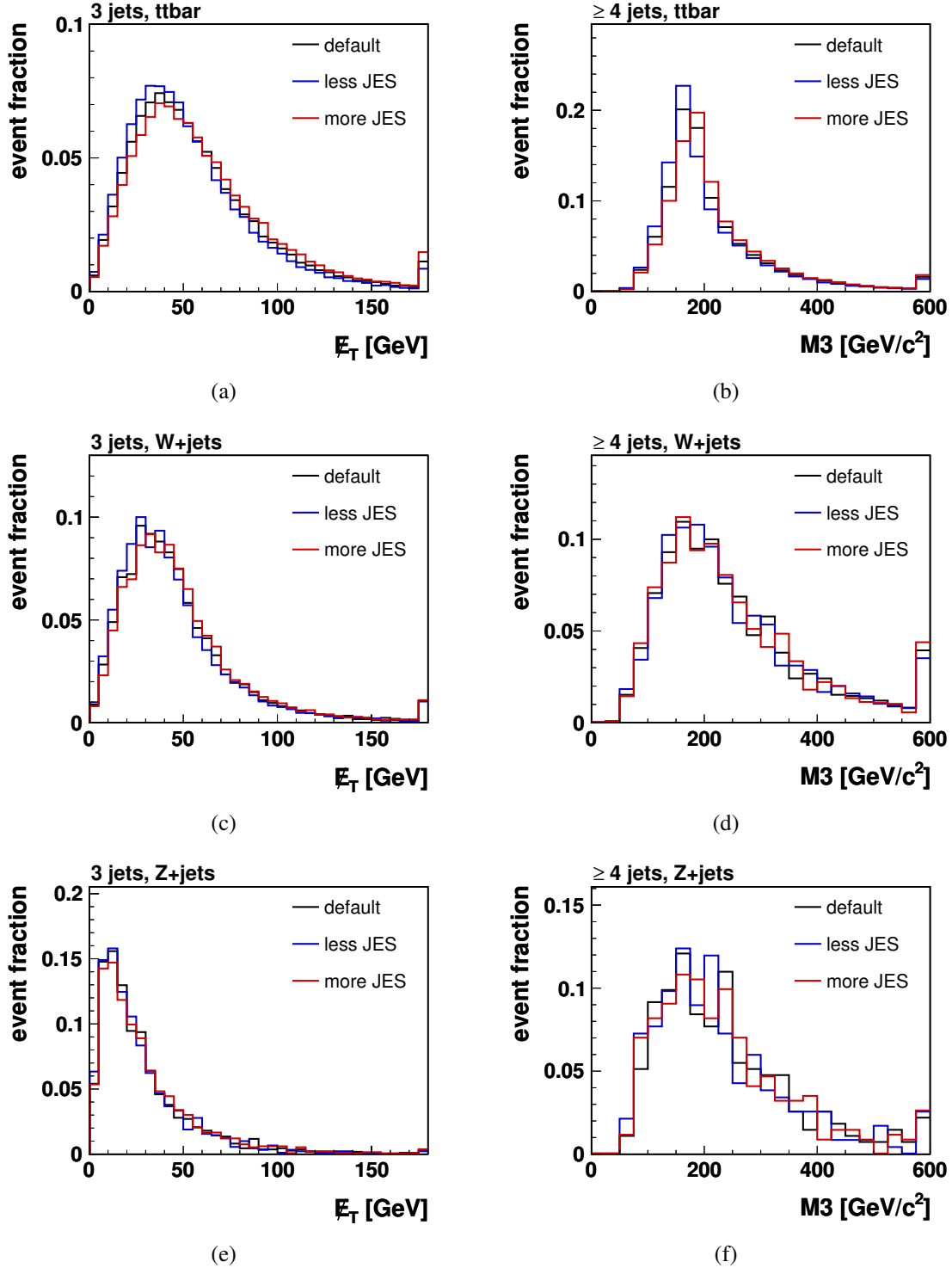
Figure 5.9: Impact of varying the jet energy scale (JES) on the probability distributions \mathcal{T}_k of the discriminating observables. Shape comparisons between the nominal \cancel{E}_T distributions and the ones derived by applying \pm 1\sigma variations of the jet energy scale are depicted in (a), (c), and (e) for t\bar{t} , W +jets, and Z +jets production, respectively. Similarly, in (b), (d), and (f), the corresponding shape comparisons for the M3 distributions are shown.
