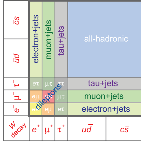
Figure 1.7: Decay channels for t\bar{t} events [100]. The graphic shows the three different t\bar{t} event topologies, i.e. the all-hadronic, the lepton+jets, and the dilepton channel. The branching ratios for the various channels are thereby indicated by the size of the different areas.
