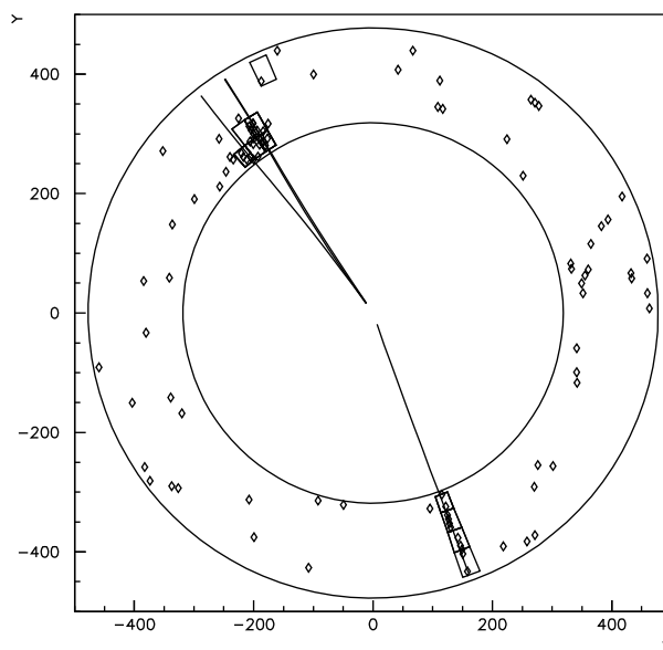
Figure 5.8: A \tau^+\tau^- event seen in the HCAL with cathode readout. One \tau decays into three pions, the other one into a \mu and two neutrinos (not seen).
