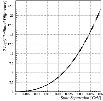
Figure 8.26: Likelihood difference for the scenario including two states (the 1^+ and 2^+ ) at 80 MeV contributing to the observed peak. The plot shows the scanned distance between the two states and on the y-axis two times the log likelihood difference to the optimal full fit result.
