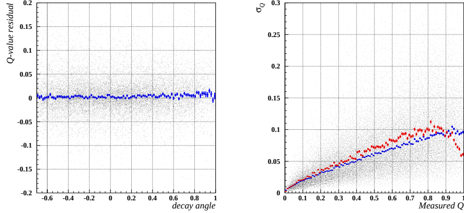
Figure 8.3: Left: The distribution shows the Q -value residual as a function of the \pi decay angle after the application of the Q Corr network. The bias of figure 8.1 is not present any more. Right: \sigma_Q as a function of the Q -value. The blue (dark) points represent the median of the distribution. Superimposed is the deviation from the true Q value in red (light), showing a good agreement with the estimate. The break-down at high Q -values is due to effects caused by the nature of conditional probability densities.
