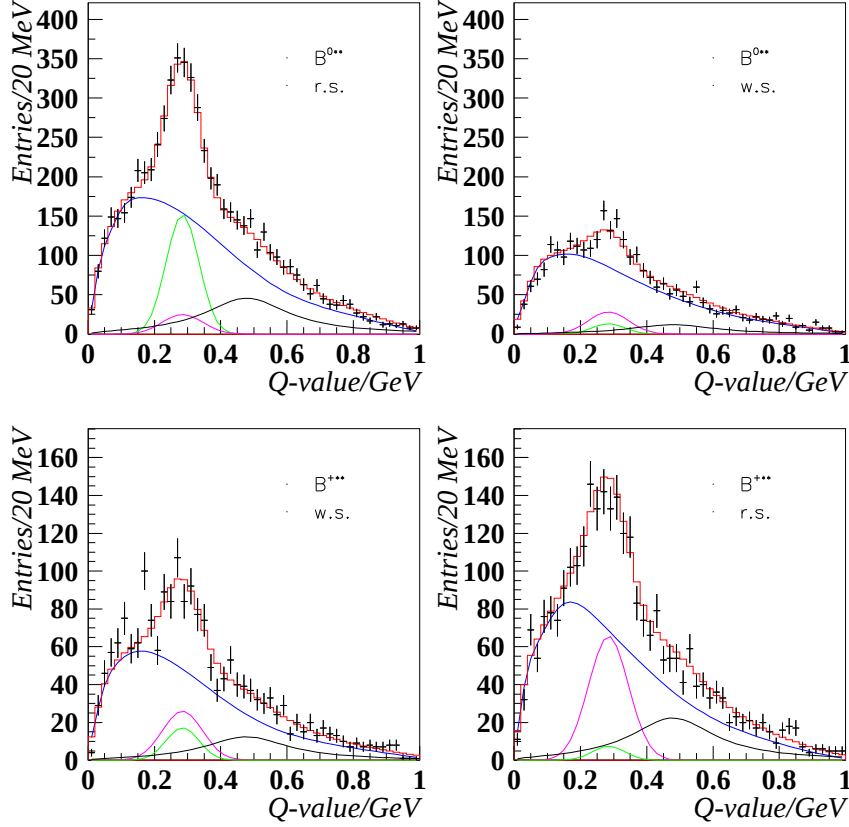
Figure 8.9: Distribution of the Q-value of B^{(*)}\pi pairs.
