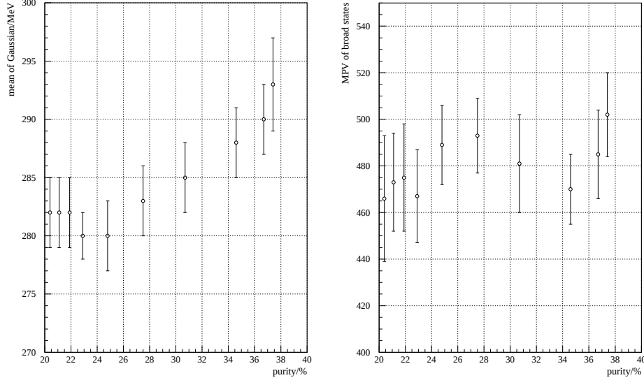
Figure 8.11: A mass scan over B_{u,d}^{**} purities at different enrichment net cuts for the Gaussian (left) and Breit-Wigner (right) fit components.
