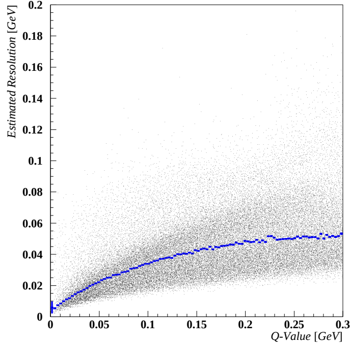
Figure 8.16: Median of the Q -value resolution \sigma_Q provided by the B_s^{0**} Q Corr Network as a function of the measured Q -value.
