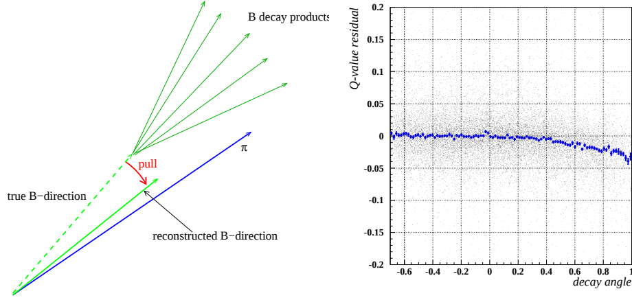
Figure 8.1: Left: A schematic view of a B^{**} decay into a pion and a b -hadron. The presence of the signal pion effects the reconstruction of the B -direction. This effect is enhanced if the decay angle in the B^{**} rest frame is very forward with respect to the B^{**} flight direction, as can be seen in the plot on the right. The distribution shows the resulting Q -value residual as a function of the \pi decay angle.
