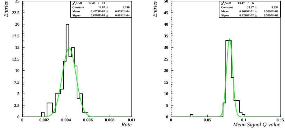
Figure 8.23: Left: The B_s^{**} \rightarrow B^+ K^- rate in a systematic scan over B_s^{**} purities. Right: the distribution of the signal Q-value in the scan. The width of the fitted Gaussian provides the value for the systematic error on the parameters.
