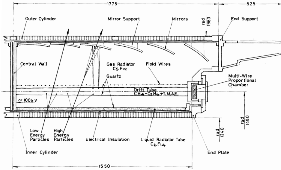
Figure 5.12: Schematic view of the barrel RICH detector. The upper volume shows the gas radiator. The thin liquid radiator is indicated as well. The Cherenkov photons are converted in the TMAE gas. The converted electrons drift in both systems to the proportional chamber indicated on the right hand side.
