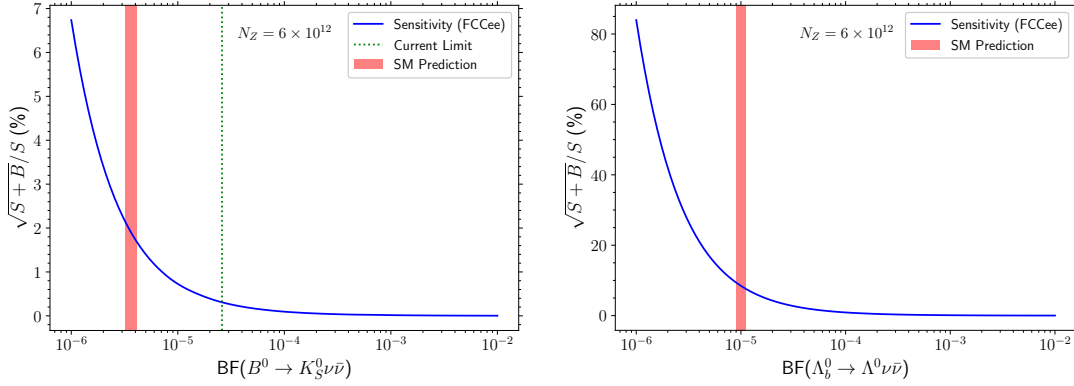
Figure 9: The expected sensitivity of the Tera-Z run at FCC-ee to the branching fraction of B^0 \rightarrow K_S^0 \nu \bar{\nu} (left) and \Lambda_b^0 \rightarrow \Lambda^0 \nu \bar{\nu} (right).
