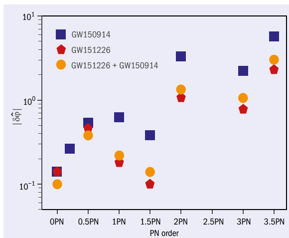
Fig. 4. The 90%-credible upper bounds on deviations in the post-Newtonian coefficients from GW150914 and GW151226, and the joint upper bounds from the two detections.
