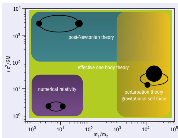
Fig. 3. Current range of validity of the main analytical and numerical methods to solve the two-body problem. The horizontal axis shows the binary mass ratio, while the vertical axis shows the radial separation between the two black holes in the binary.
