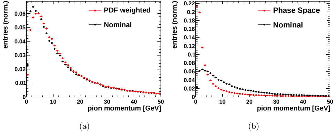
Figure 6.16: Left: Nominal MC momentum distribution (black) compared to MC with |A_{\perp}|^2 increased to 0.27 and |A_{\parallel}|^2 increased to 0.39 (red); Right: Nominal MC momentum distribution (black) compared to phase space MC (red)
