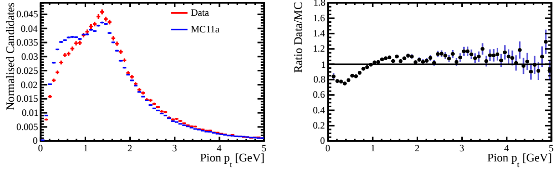
(b) Pion transverse momentum
