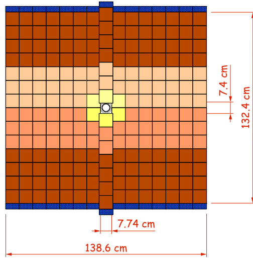
Figure 2.10: One layer of the Tracker Turicensis. The beam line goes through the centre.
