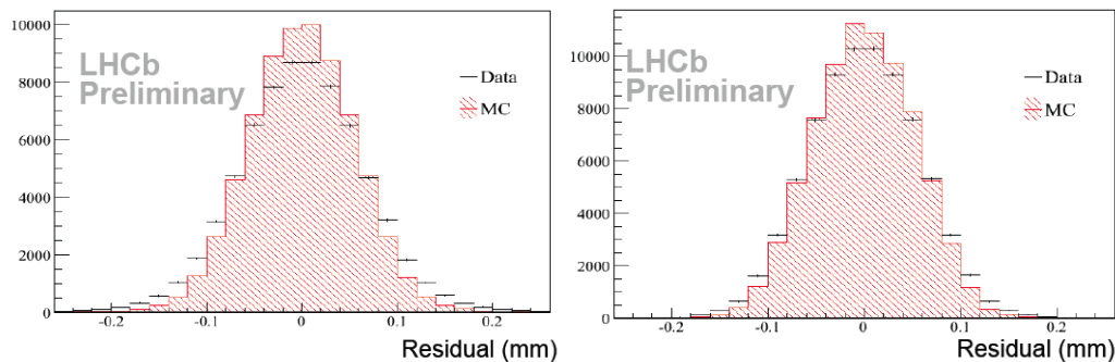
Figure 2.13: Hit Resolutions for IT (left) and OT (right) with 2011 data.
