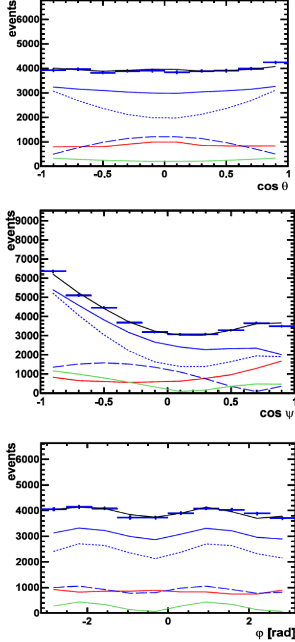
Figure 6.19: Projections of the transversity angles from fit to data. The black points show the data points, the black curve the total fit, the blue curve the signal fit (dotted blue CP-even contribution, dashed blue CP-odd contribution, the red curve the background fit and the green curve the S-wave contribution).
