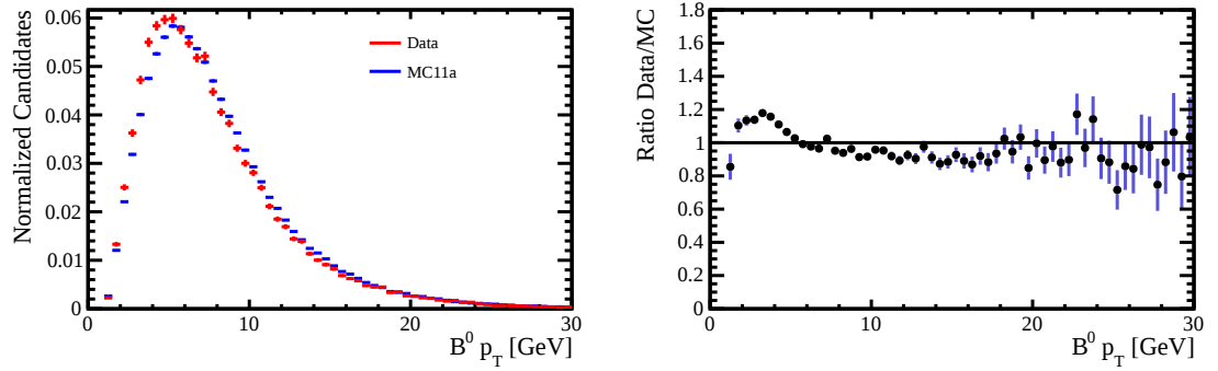
(b) B^0 Transverse momentum
