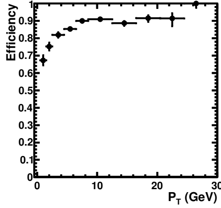
Figure 2.29: Efficiency as a function of transverse momentum for the HLT2 dimuon detached J/\psi line.
