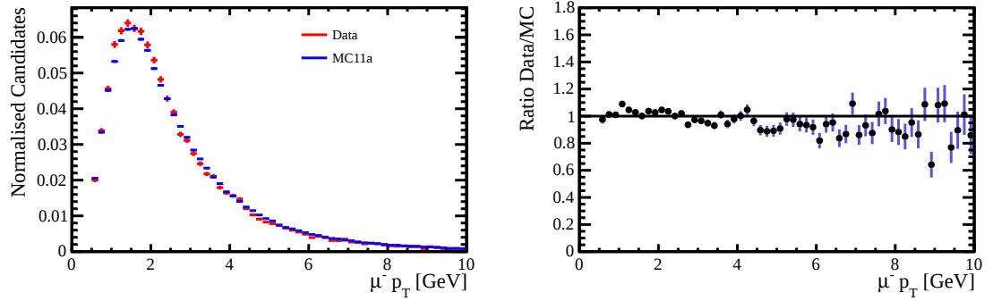
(b) \mu^- transverse momentum
