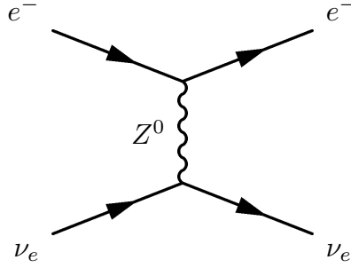
Figure 1.4: Feynman diagram showing neutrino scattering via neutral current weak interaction.
