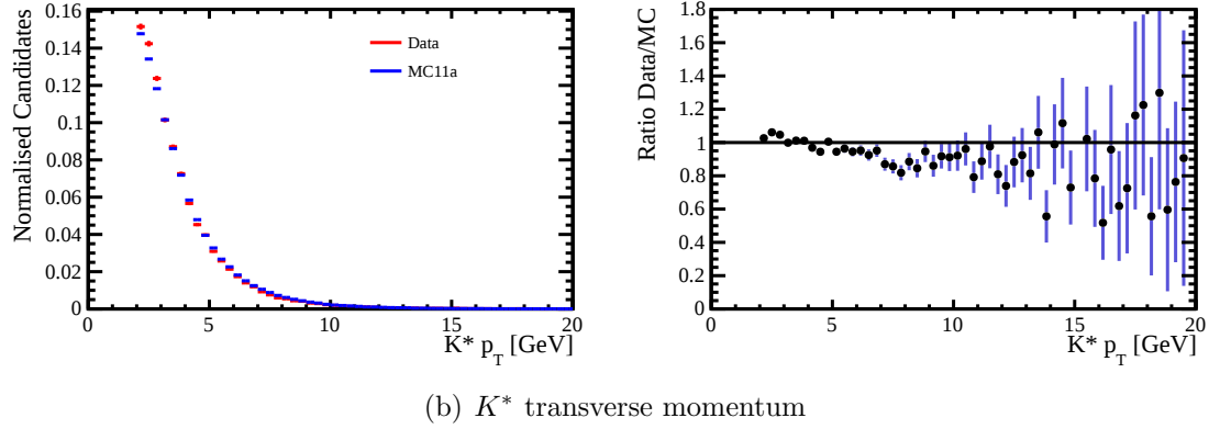
Figure 6.5: Momentum and transverse momentum distributions for the K^* particle for MC11a and data, with the ratio of the two distributions. The cut at K^* p_T > 2 GeV is clear.
