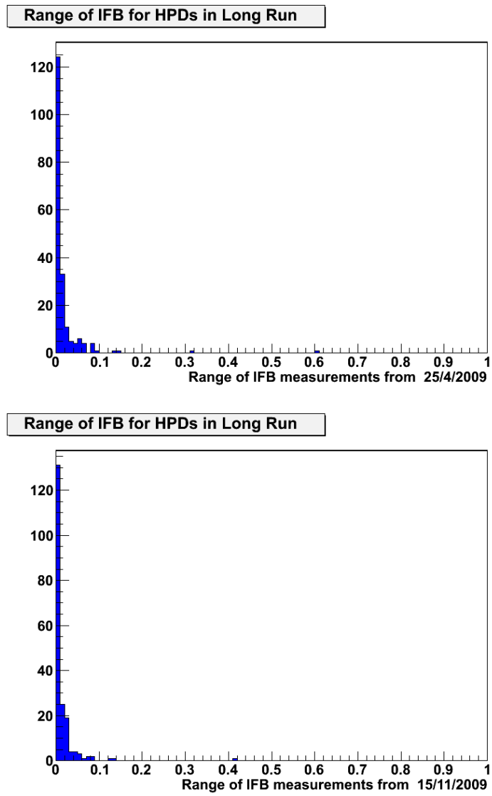
Figure B.2: Histograms of the range of the long laser runs
