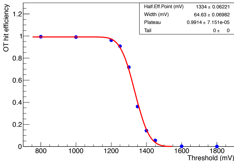
Figure 2.14: Threshold scan for the OT.
