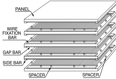
Figure 2.23: Exploded view of one muon chamber.
