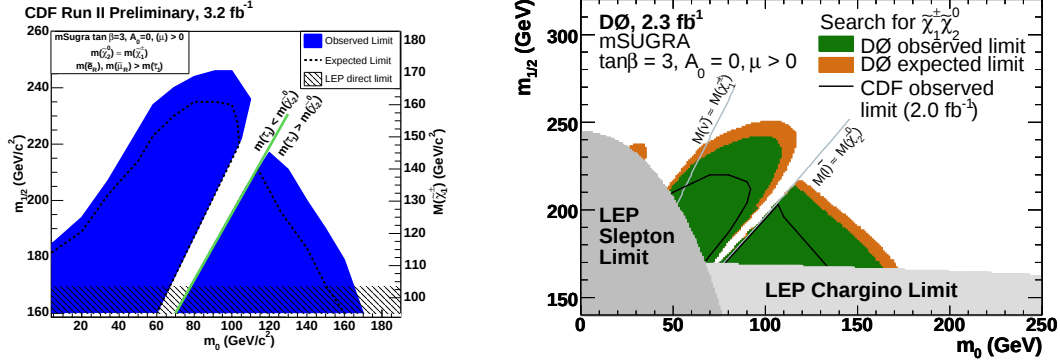
Figure 2-5. The blue regions on left plot show the areas (in m_0 - m_{1/2} plane) excluded (at 95% C.L.) by CDF experiment with 3.2 fb -1 of data from the non-observation of any tri-lepton signal excess over background in the framework of mSUGRA assuming R-parity conservation [123]. The green regions on right plot show the areas (in m_0 - m_{1/2} plane) excluded (at 95% C.L.) by DØ experiment with 2.3 fb -1 of data from the non-observation of any tri-lepton signal excess over background in the framework of mSUGRA with R-parity conservation [124].
