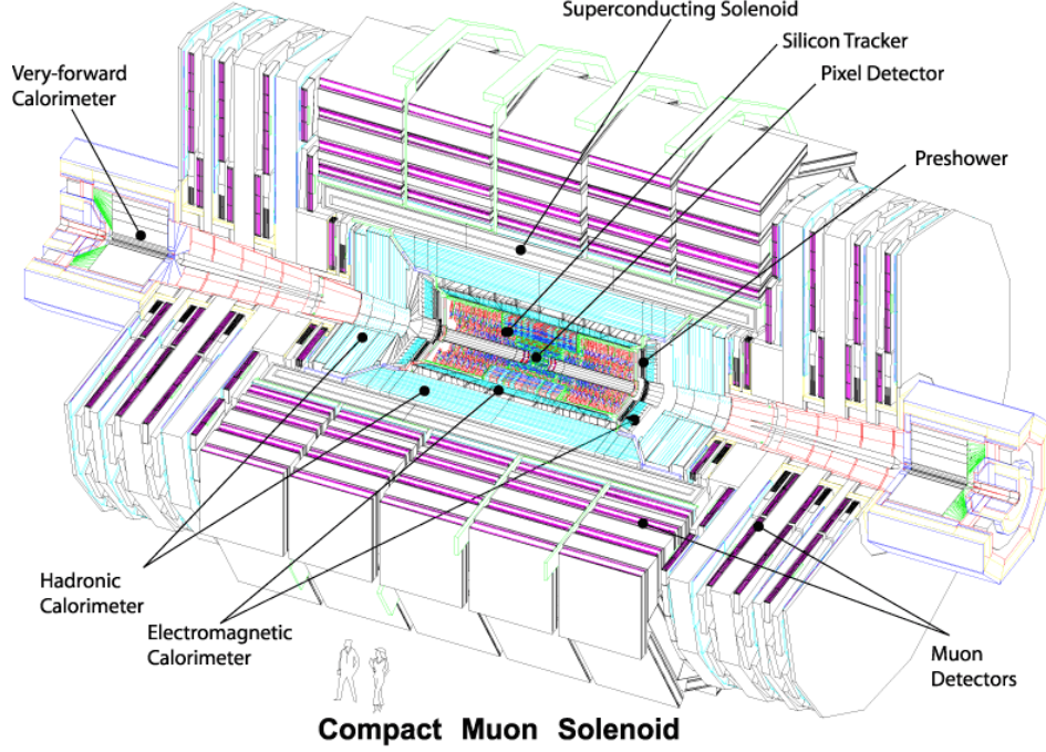
Figure 2.4: The CMS detector consists of layers of subdetectors, each with a specific purpose in the measurement of final-state particles in proton collisions. A strong superconducting magnet curves the trajectories of charged particles.
