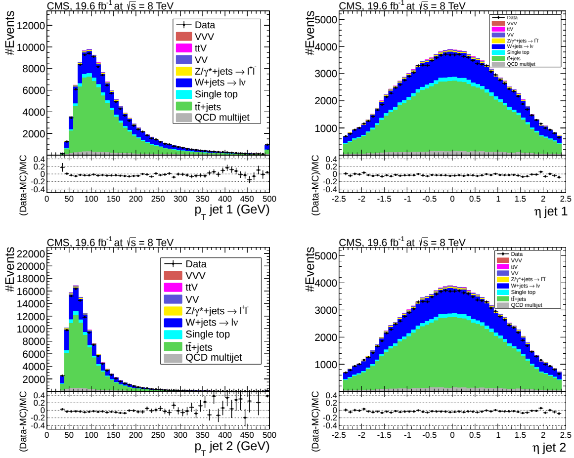
Figure 5.3: Control plots for the jets in single-muon events: the p_T (left) and \eta (right) of the leading (top) to subleading (bottom) jet in the event. The observed data and simulation agree reasonably well.
