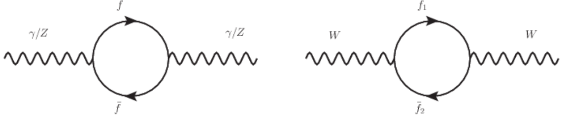
Figure 1.2: The vacuum polarization of the photon and Z boson (left) and W boson involves fermion-loop quantum corrections to the gauge fields.
