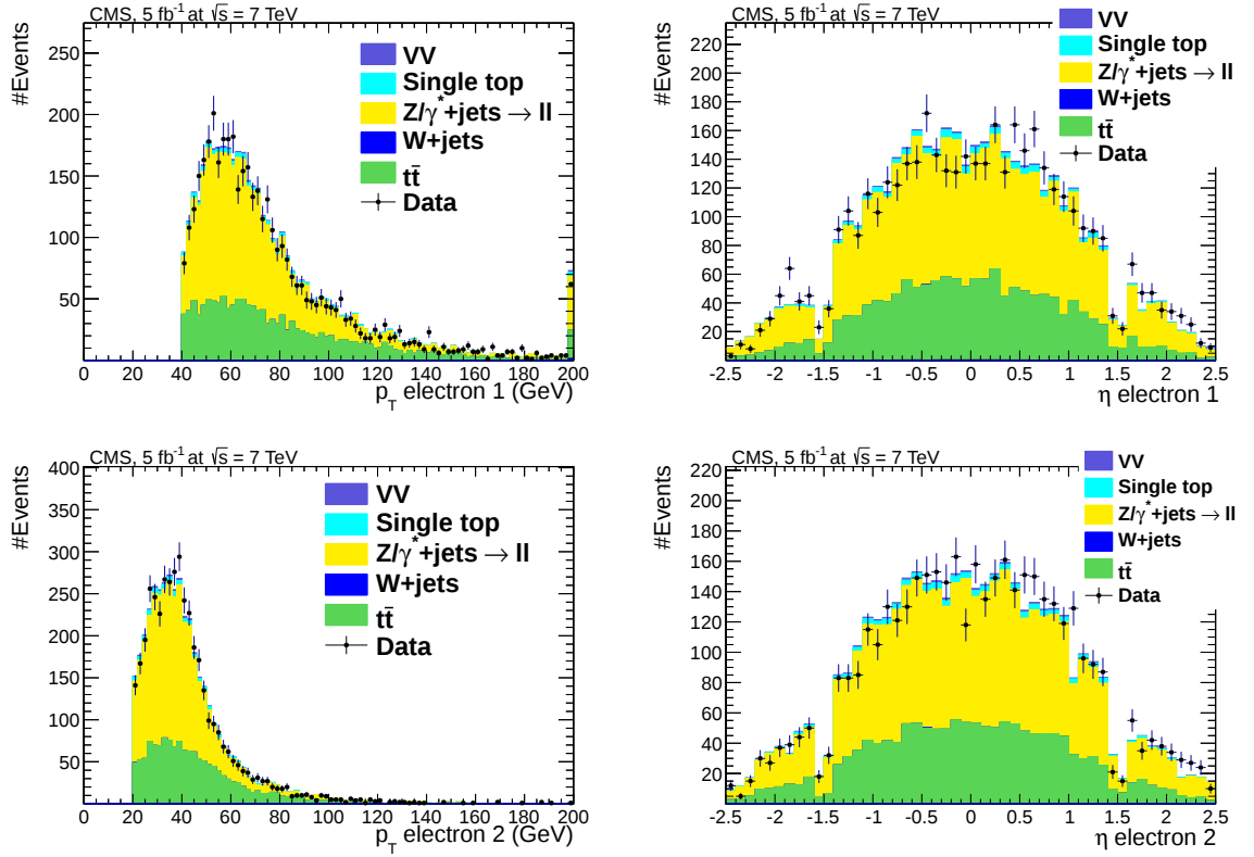
Figure 4.2: Control plots for opposite-sign dielectron events; the p_T (left) and \eta (right) of the highest- p_T electron (top), and the p_T and \eta of the second-highest- p_T electron (bottom). The total simulated background is normalized to the observed number of data events. The shapes of the observed and simulated distributions agree reasonably well.
