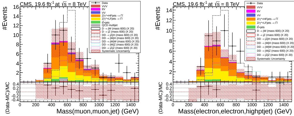
Figure 5.19: The reconstructed mass of the vector-like quark candidate in the ZHqq subsample, in the muon channel (left) and the electron channel (right). The pair-production reference signal is scaled up by a factor 20 for visibility.
