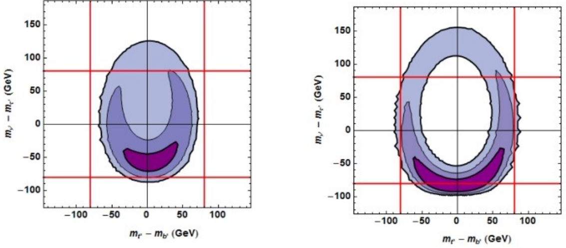
Figure 1.6: The 68%, 95% and 99% confidence level contours (dark to light) for the mass differences m_{t'} - m_{b'} ( x axis) and m_{\nu_{t'}} - m_{\tau'} ( y axis) [24]. The constraints are obtained with |V_{t'b}| = |V_{tb'}| = 0.01 (left) and |V_{t'b}| = |V_{tb'}| = 0.1 (right), no mixing between fourth-generation and first and second generation quarks, m_H = 125 GeV, m_t' = 500 GeV and m_{\tau'} = 100 GeV. The red lines indicate a mass difference equal to the W -boson mass.
