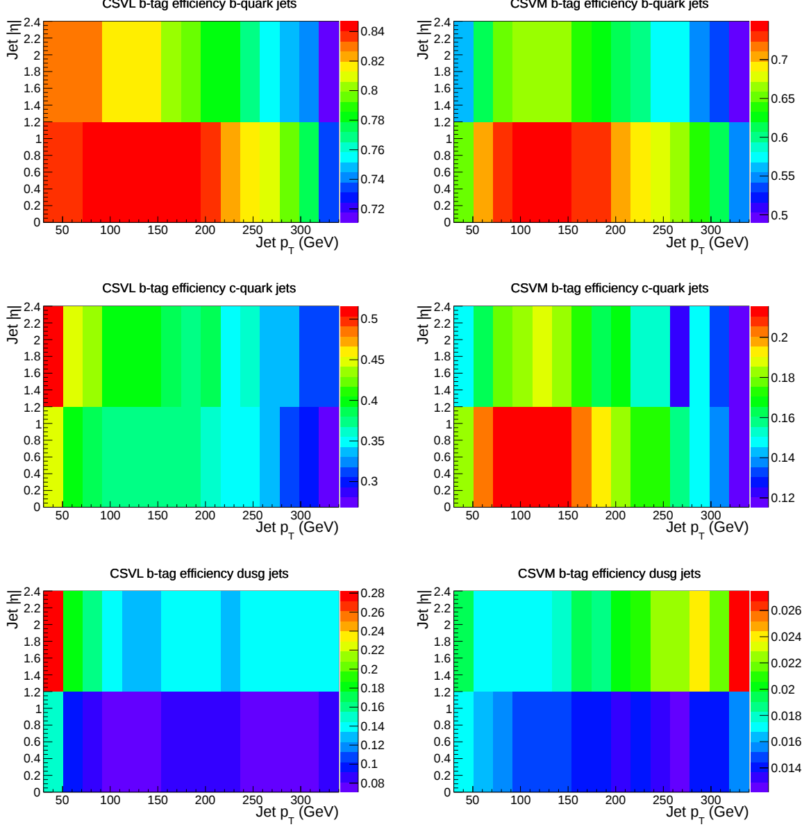
Figure 5.5: The b -tag efficiency for simulated jets originating from b quarks (top), c quarks (middle) and d, u, s quarks and gluons (bottom) are determined in bins of jet p_T and \eta , and for the loose (left) and the medium (right) Combined Secondary Vertex operating points. These efficiencies, obtained from t\bar{t} simulated events, are used in the determination of the simulated-event weights to account for differences in b -tag and anti- b -tag efficiencies in data and simulation.
