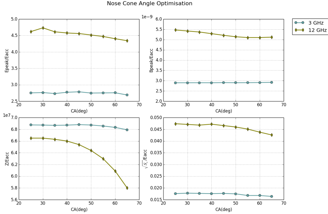
Fig. 3.12 The effect of the nose cone angle on shunt impedance and peak fields for both S and X-band.
