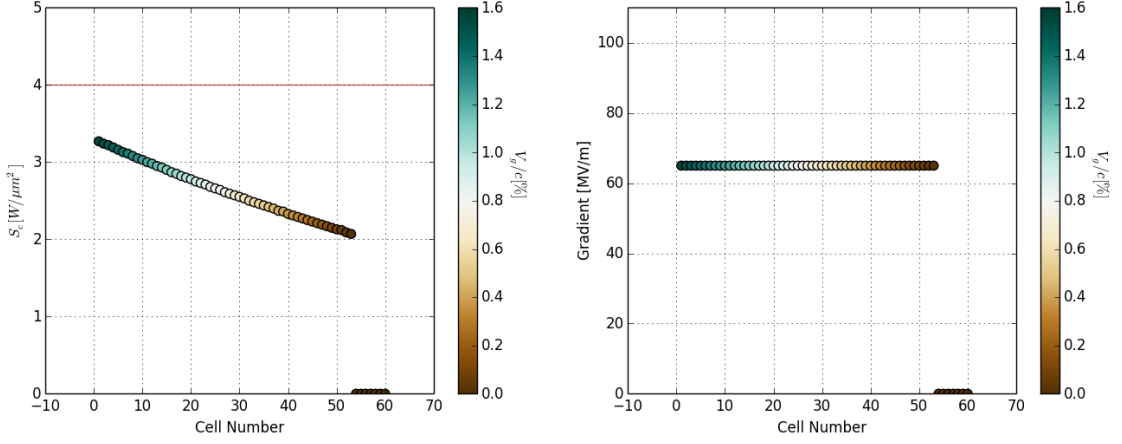
Fig. 3.43 The modified Poynting vector and gradient across the 60 cell 12 GHz \varphi = \frac{2\pi}{6} constant gradient structure. The red line indicates the peak S_c limit.
