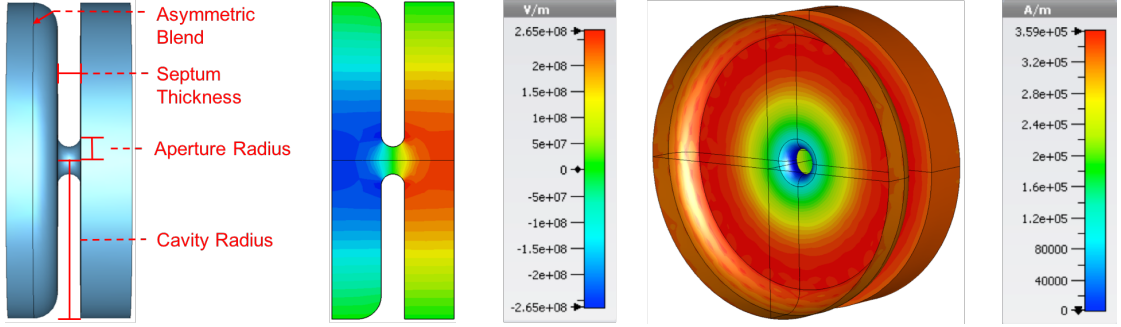
Fig. 3.1 A pillbox cavity vacuum model (left) Electric field profile (centre) and magnetic field profile (right).
