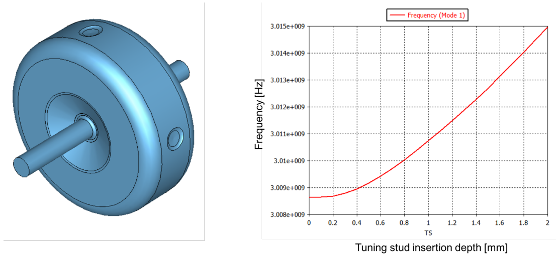
Fig. 6.1 The simulation model for the ‘push’ tuning studs and a plot showing the resulting frequency shift in Hz. The x-axis is how many mm the tuning stud has been inserted into the cavity wall.
