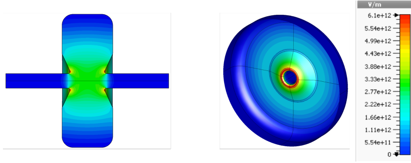
Fig. 2.21 Absolute part of the electric field inside a re-entrant pillbox cavity.
