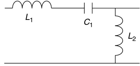
Fig. 2.26 Dispersion for magnetically coupled resonators [77].
