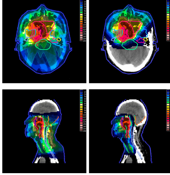
Fig. 1.7 Illustrates the differences between photon radiotherapy (left) where dose is deposited across the entire cross section of the patient and proton therapy (right) where the dose ends half way through, the back of the head, spine and back see no dose [27].
