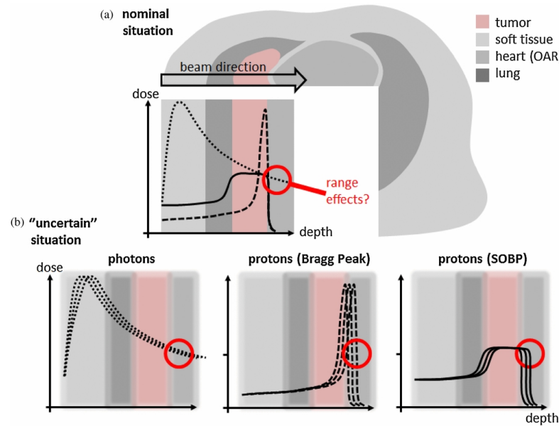
Fig. 1.9 (a) Potential dose benefit of a proton treatment compared to a photon treatment (dotted line: photon depth-dose curve; dashed line: mono-energetic proton depth dose curve known as Bragg Peak; straight line: spread out proton Bragg curve (SOBP) to cover the whole tumour). (b) Influence of uncertainties to these depth-dose curves [34].
