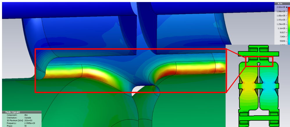
Fig. 6.17 Magnetic peak field on the coupling slot.
