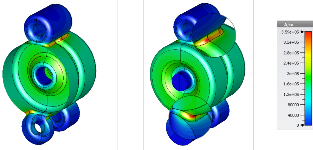
Fig. 4.7 Magnetic field profile of a C-band side-coupled quadruplet.
