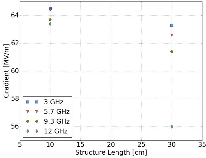
Fig. 3.26 Maximum gradient achieved for side-coupled standing wave structures of different lengths and frequencies. Gradient is limited by 50 MW/m input power and available shunt impedance using S_c \leq 4\text{W}/\mu\text{m}^2 as a peak field limit.
