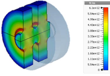
Fig. 2.23 Abs e-field plot of ‘electric’ or ‘capacitive’ coupling through the iris of a pillbox cavity [81].
