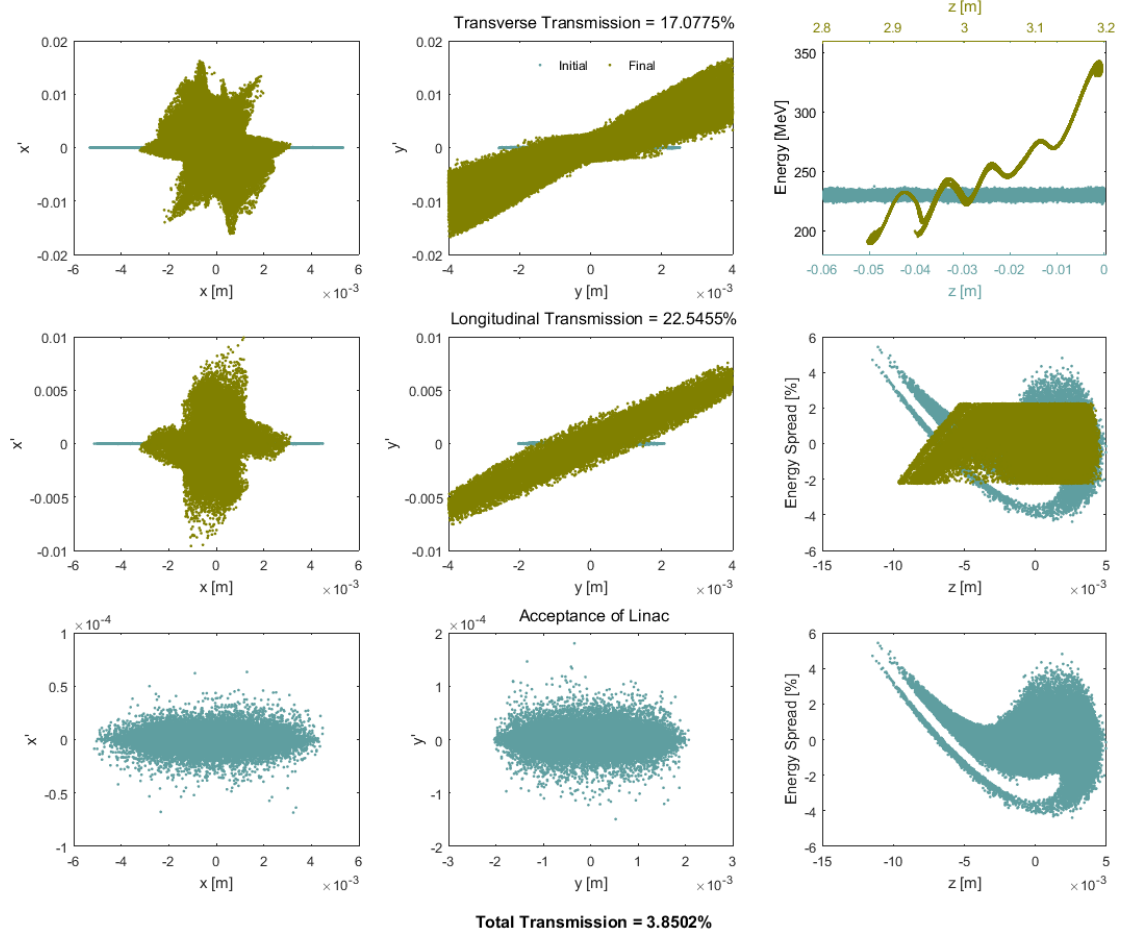
Fig. 5.10 Transmission through 7x7-cell cavities and matching sections between.
