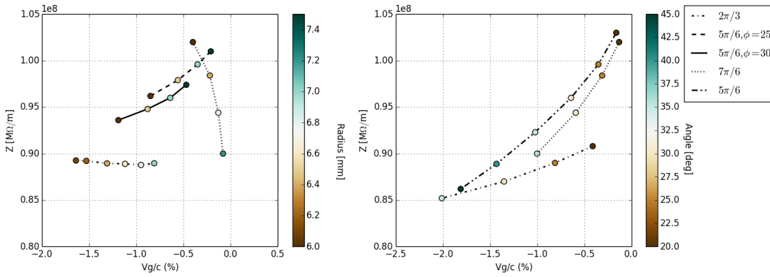
Fig. 3.37 Shunt impedance of structures with varying phase advances. \phi in this plot represents the slot angle \psi for the only structures with fixed \psi .
