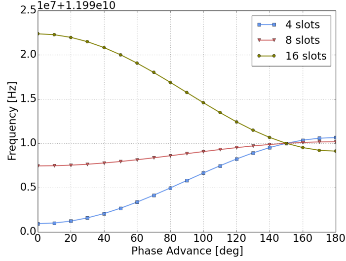
Fig. 3.27 Dispersion diagrams of increasing numbers of circular couplings slots. Only the 16 slot structure exhibits a bTW.
