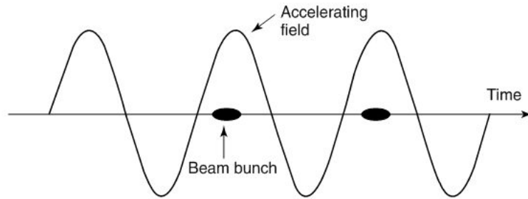
Fig. 2.2 Beam bunches in the positive phase of an RF voltage [77].
