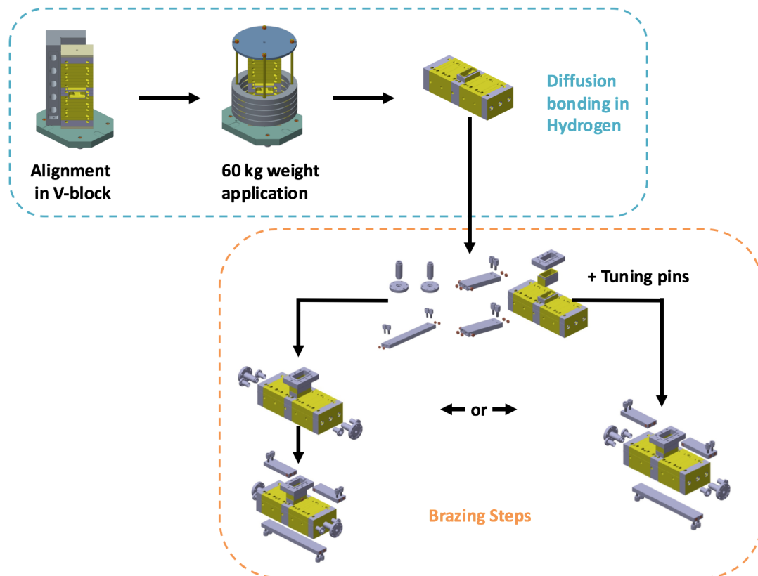
Fig. 6.24 Figure shows the alignment, and weight tools for hydrogen bonding of the disks. After the disks have been bonded together the remaining pieces are brazed on in various steps of decreasing temperature. (Design and images courtesy of Niklas Templeton at Daresbury Laboratory, UK).
