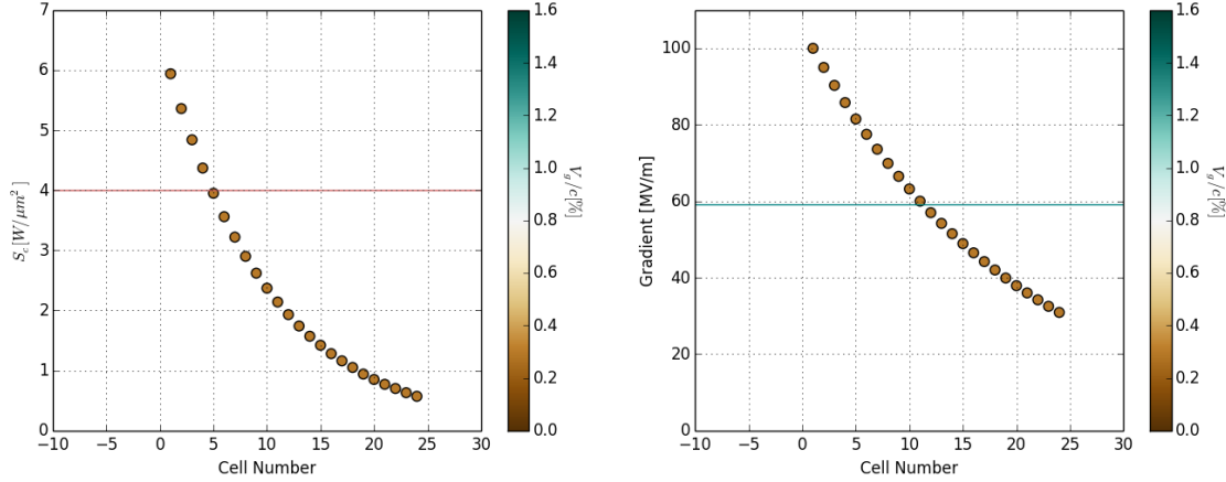
Fig. 3.49 The modified Poynting vector and gradient across the 24 cell 12 GHz \varphi = \frac{5\pi}{6} constant impedance structure. Red line indicates the maximum allowable S_c whilst the blue line indicates the overall structure gradient 59.1 MV/m.
