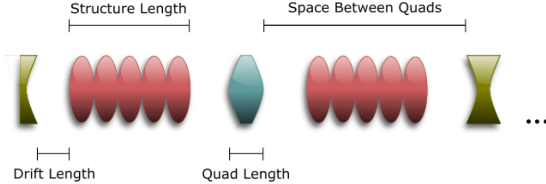
Fig. 2.10 Typical FODO arrangement with focussing quadrupoles (blue) defocussing quadrupoles (green) and RF cavities (red) in the drift spaces between.
