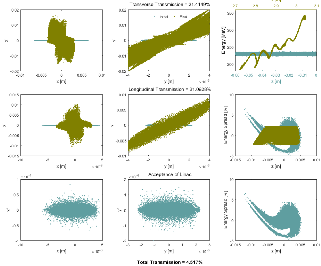
Fig. 5.9 Transmission through 7x3-cell cavities and matching sections between.
