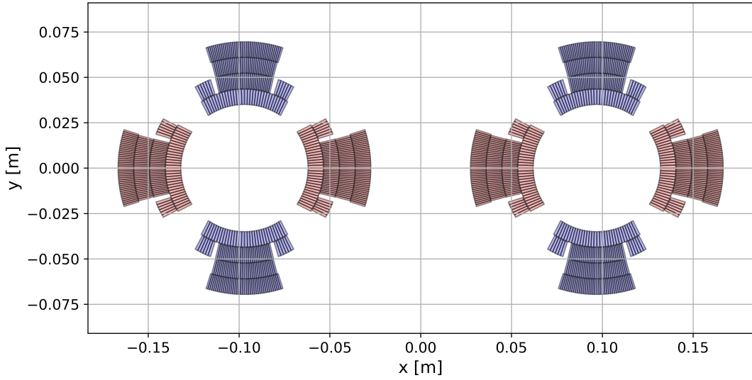
FIGURE 3.9: MQY quadrupole magnet geometry generated by the SWAN notebook.
