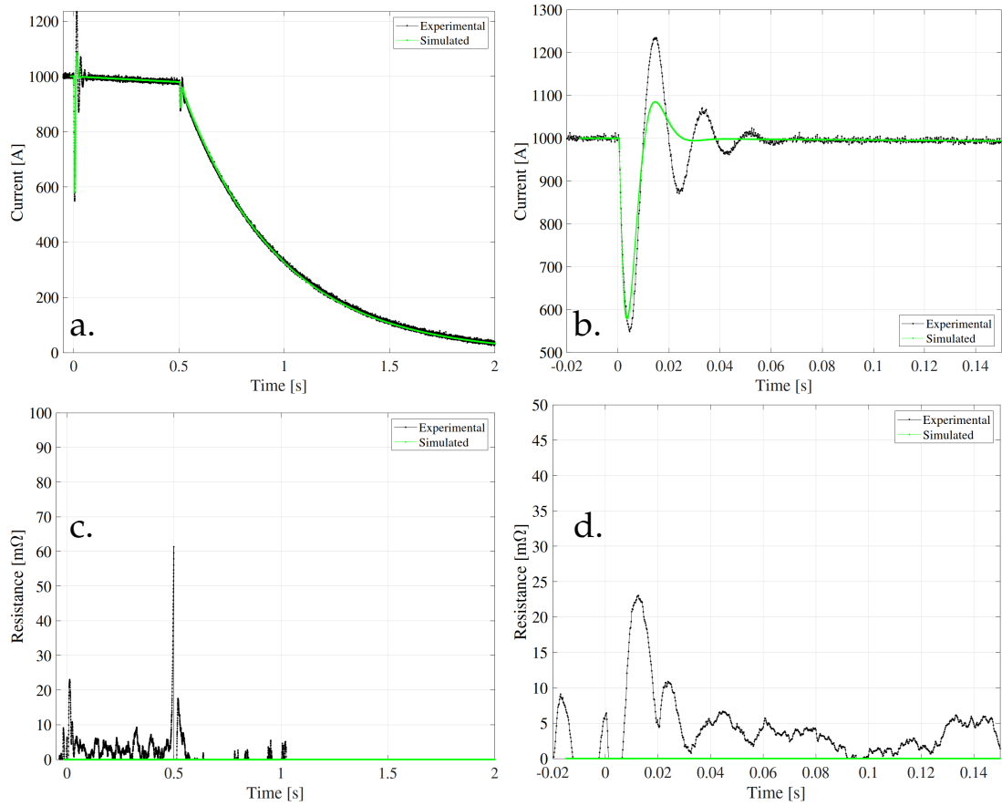
FIGURE 5.25: CLIQ and Delayed Energy Extraction (Test 13, see Tab. 5.1). a. Magnet current versus time. b. Zoom in the magnet current. c. Magnet resistance versus time. d. Zoom in magnet resistance.
