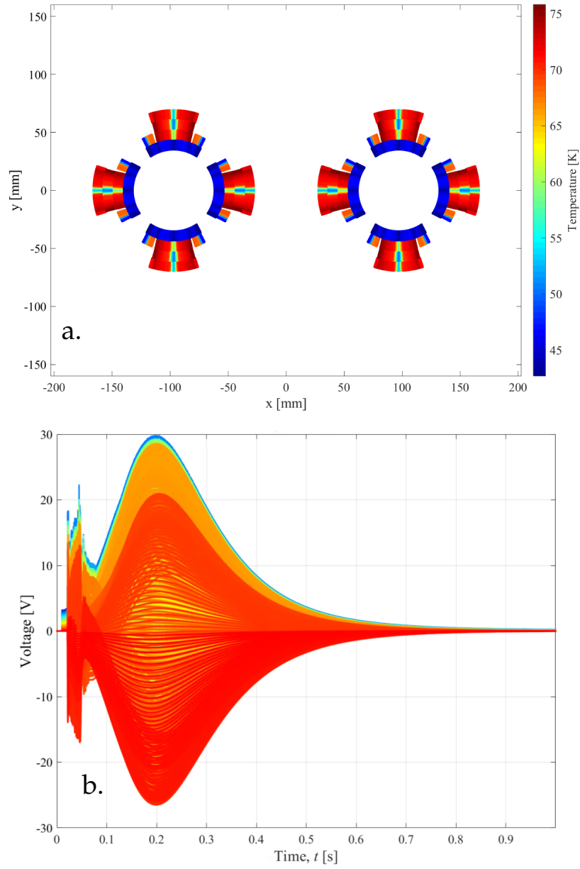
FIGURE 6.10: Temperature (a.) and Voltage to ground versus time (b.) on the MQY magnet cross-section after a co-simulation at 4.5 K (circuit RQ4.L8).
