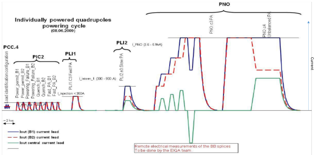
FIGURE 4.4: Powering cycles for the IPQ circuits [58].
