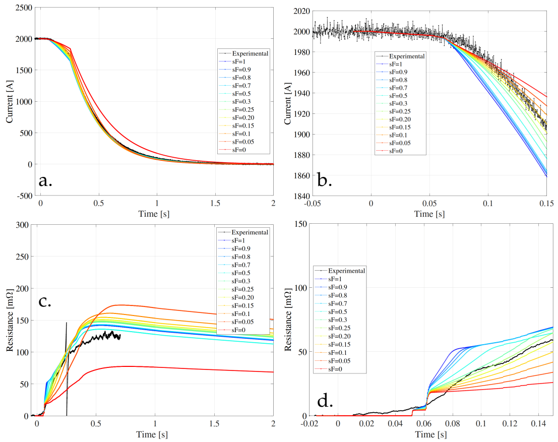
FIGURE 5.11: Experimental curve and simulations for different scaling factor values. a. Magnet current versus time. b. Zoom in the magnet current. c. Magnet resistance versus time. d. Zoom in magnet resistance.
