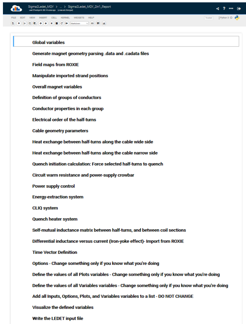
FIGURE 3.8: Complete overview of all the cells that compose the SWAN notebook.
