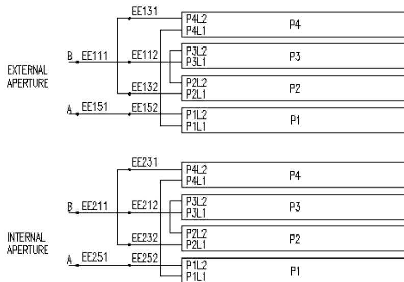
FIGURE 2.4: Electrical scheme of the two individually powered apertures of the MQM magnet [30].
