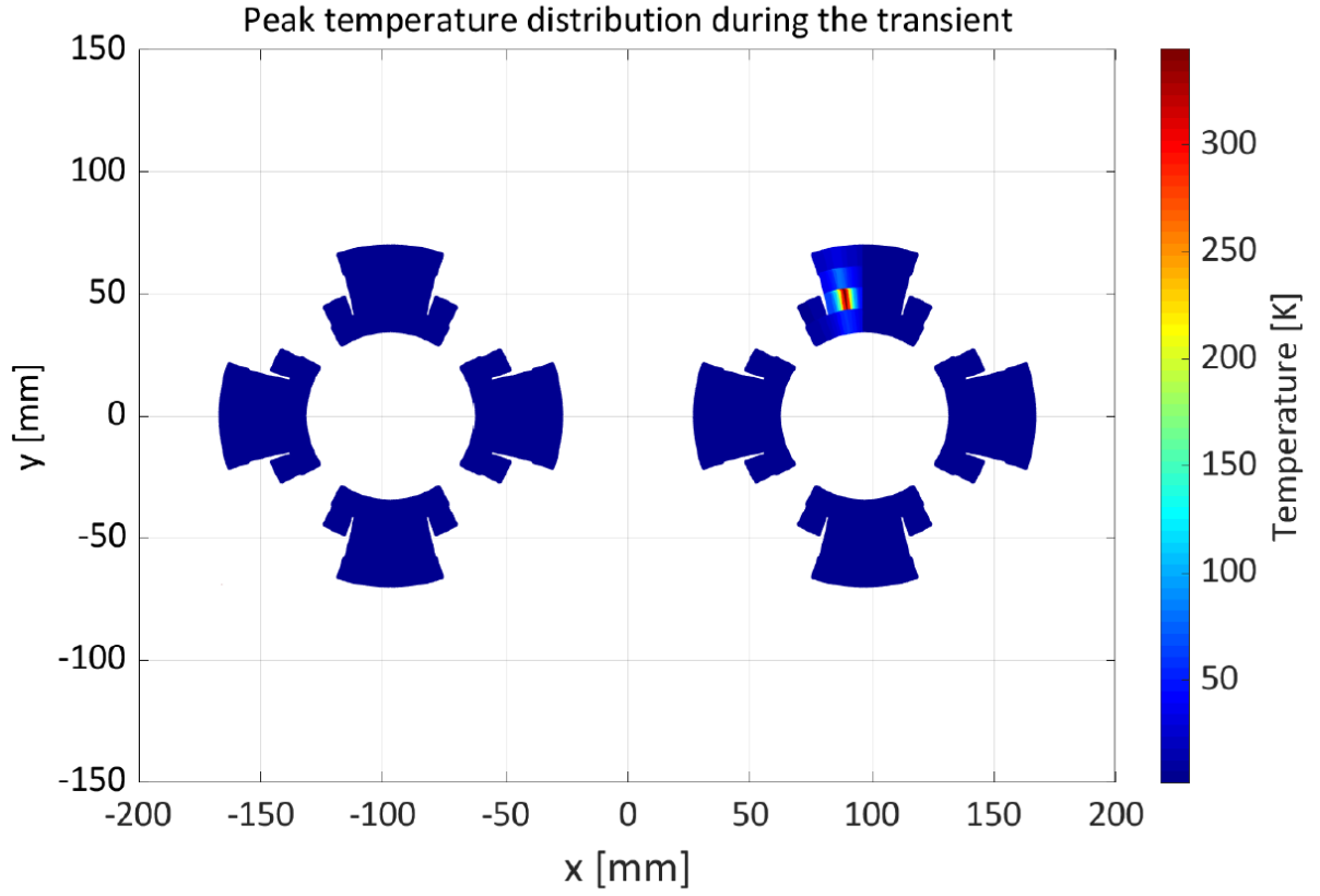
FIGURE 5.1: Temperature distribution in case of a forced quench in an unprotected MQY magnet.
