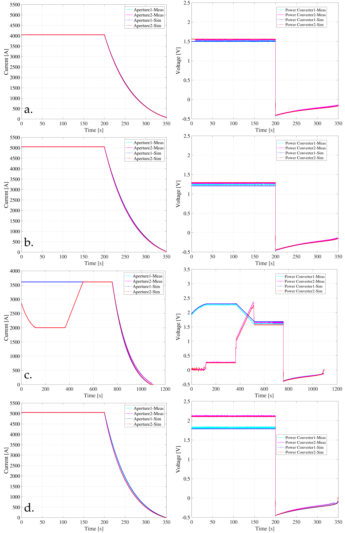
FIGURE 4.5: Validation of four different IPQ circuits. Measured and simulated DDCT current vs time and measured and simulated voltage across the power converter vs time. a. RQ5.L8 (2xMQM magnets at 4.5 K and 4.1 kA). b. RQ8.L1 (MQML magnet at 1.9 K and 5 kA). c. RQ4.L1 (MQY magnet at 4.5 K and 3.6 kA). d. RQ9.R2 (MQM+MQMC magnets at 1.9 K and 5 kA).
