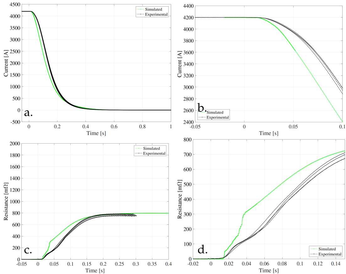
FIGURE 5.27: Simulation vs Experimental data for the validation of the MQM magnet model at 4.5 K. a. Magnet current versus time. b. Zoom in the magnet current. c. Magnet resistance versus time. d. Zoom in magnet resistance.
