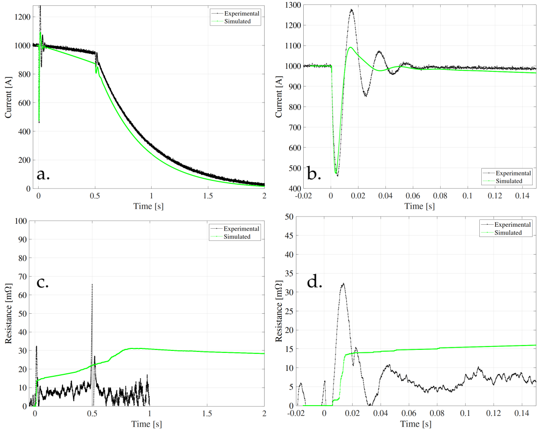
FIGURE 5.24: CLIQ and Delayed Energy Extraction (Test 12, see Tab. 5.1).
