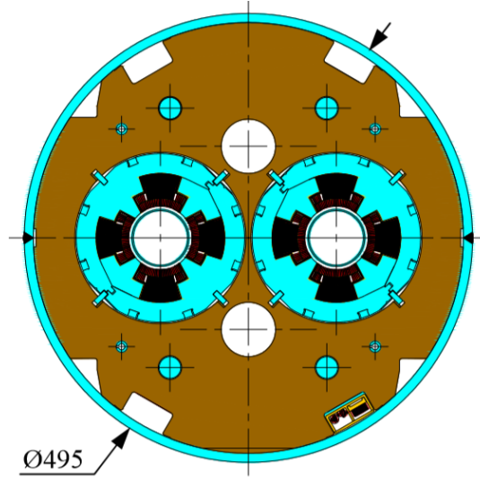
FIGURE 2.3: Cross-section of the MQY quadrupole [28].
