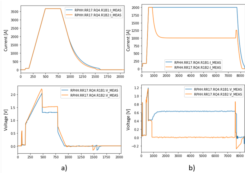
FIGURE 3.1: Tests found by the notebook. a) Current and voltage measures versus time in case of the same current value in both magnet apertures. b) Current and voltage measures versus time in case of different current values in the magnet apertures.
