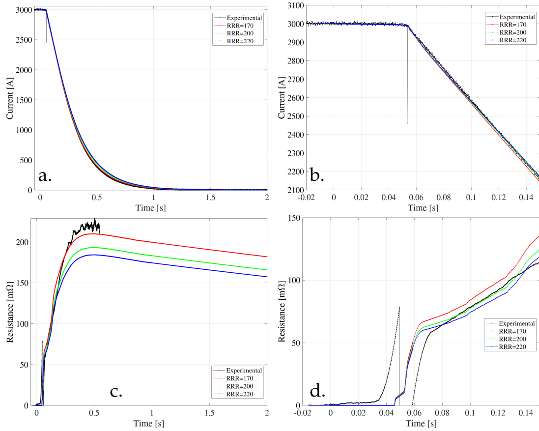
FIGURE 5.9: Simulations and measurement for different Residual Resistivity Ratio. a. Magnet current versus time. b. Zoom in the magnet current. c. Magnet resistance versus time. d. Zoom in the magnet resistance.
