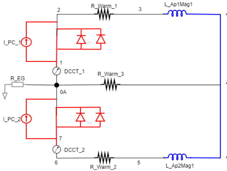
FIGURE 2.8: Simplified schematic of the IPQ for one magnet configuration.
