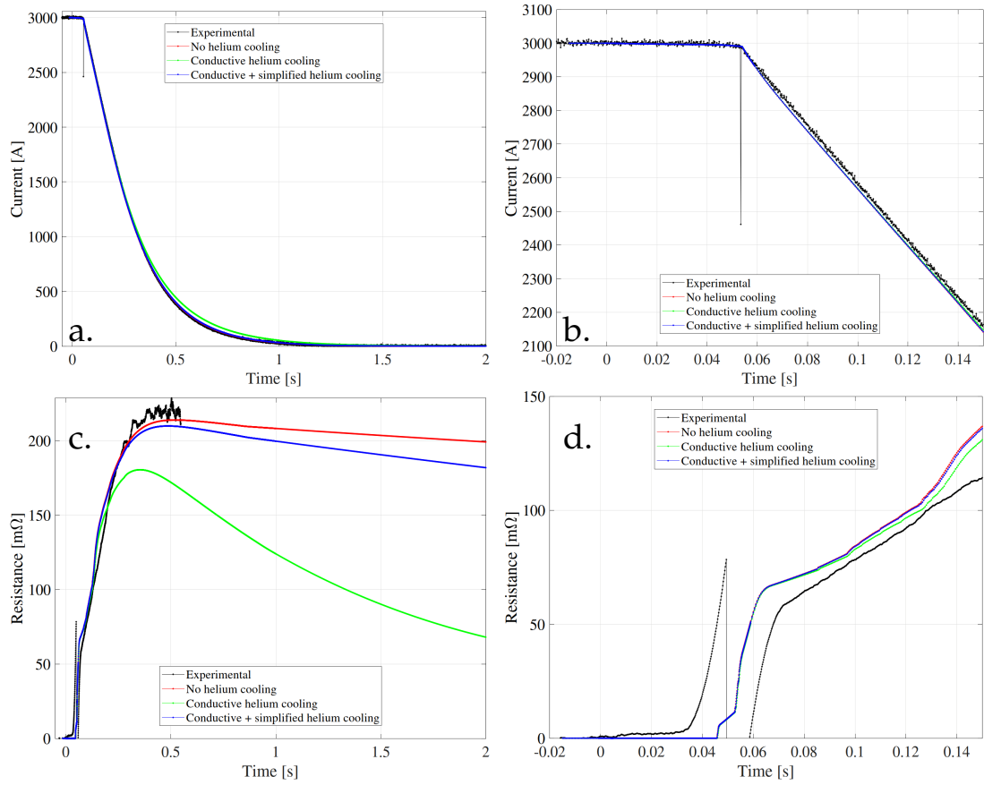
FIGURE 5.3: Simulation and measurement for different settings of the LEDET helium cooling assumptions. a. Magnet current versus time. b. Zoom in the magnet current. c. Magnet resistance versus time. d. Zoom in the magnet resistance.
