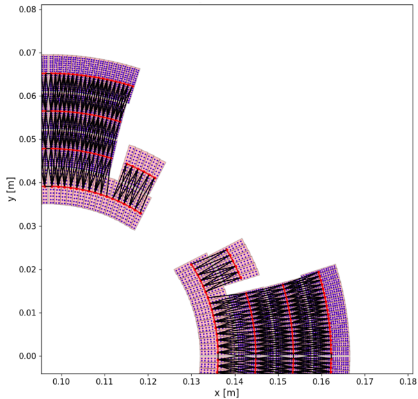
FIGURE 3.11: Heat exchange connections between the half-turns of the MQY magnet. The red lines represent the heat exchange along the cable wide side, while the black lines represent the heat exchange along the cable narrow side. The blue color on the figure are dots that represent the strands in each half-turn.
