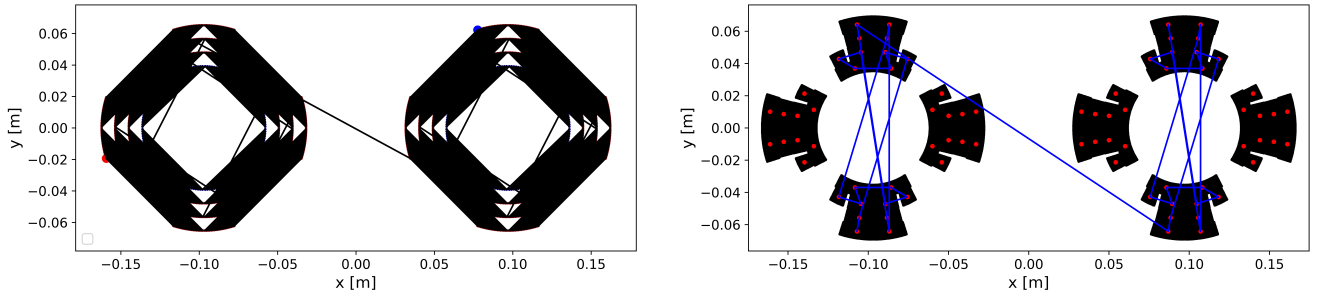
FIGURE 3.10: Electrical order of the half-turns (a) and groups (b) of the MQY magnet generated by the SWAN notebook.
