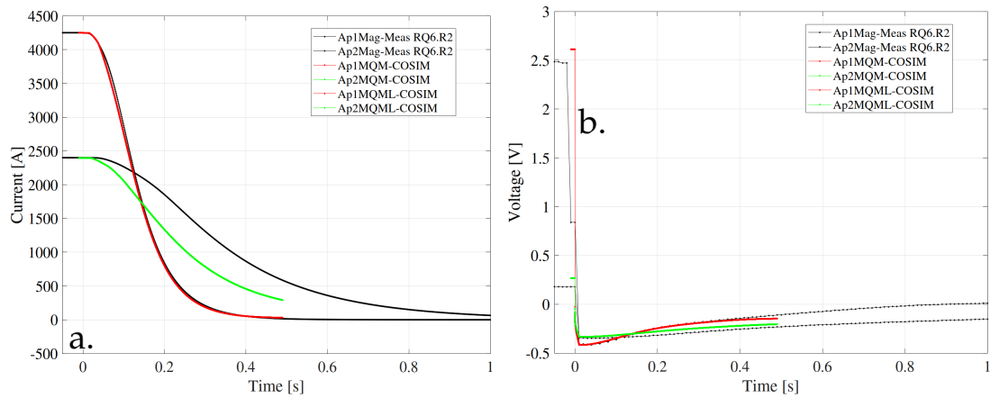
FIGURE 6.20: Simulations and measurements for a co-simulation at 4.5 K with different current values in the magnet apertures (circuit RQ6.R2). a. DCCT Current versus time. b. Voltage across the power converter versus time.
