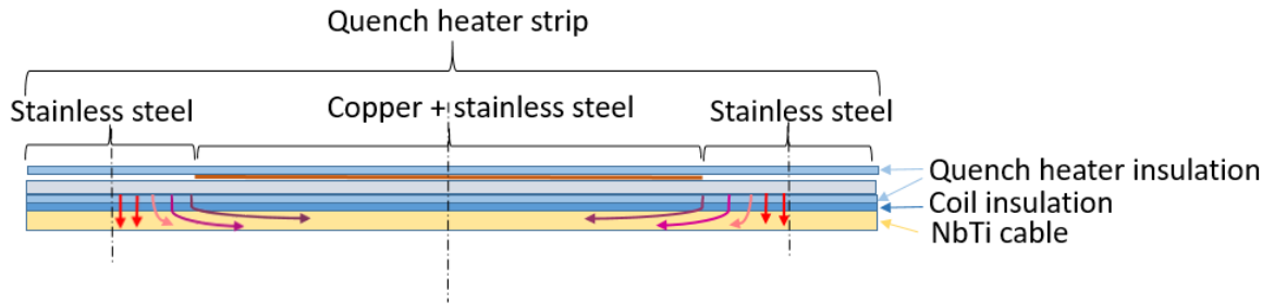
FIGURE 5.7: Simplified representation of the thermal layout along the length of the conductor. The heat flux flow from the quench heater heating stations to the conductors. Different colors of the arrows represent different cases of heat propagation.
