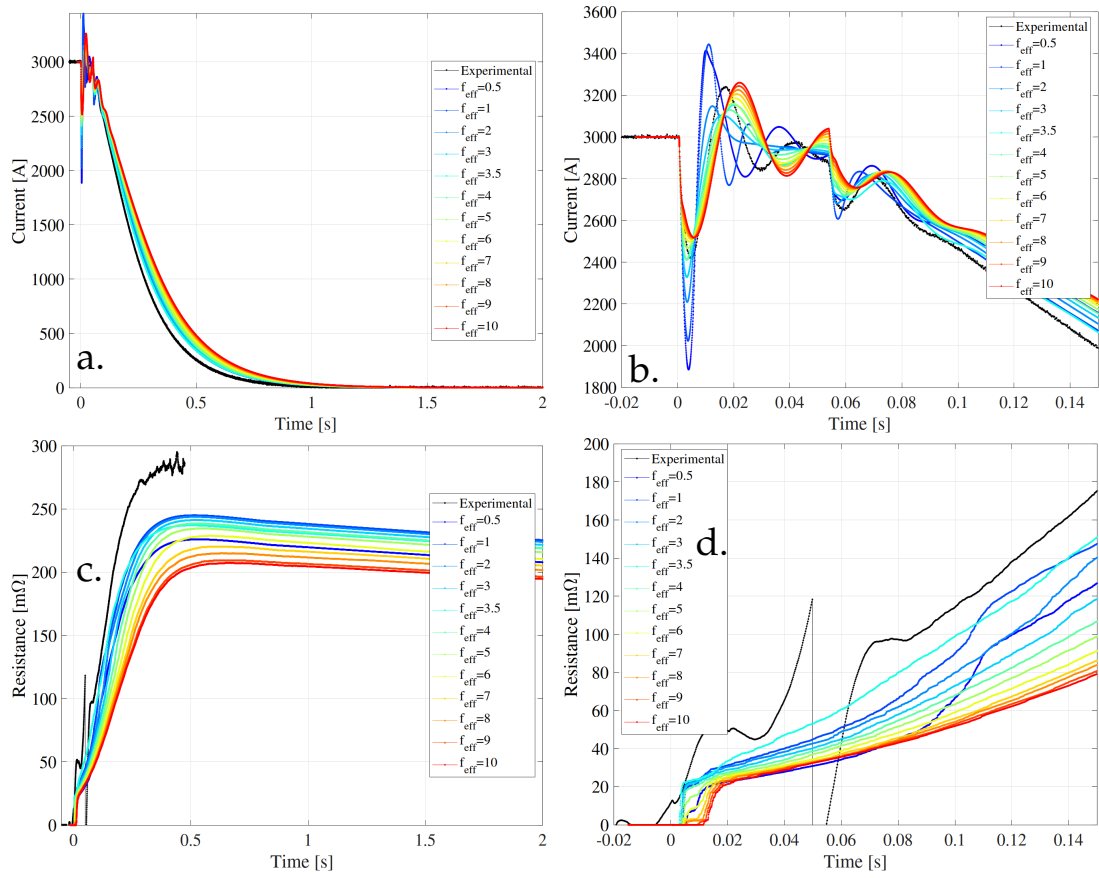
FIGURE 5.17: Experimental curve and simulations for different f_{eff} values. a. Magnet current versus time. b. Zoom in the magnet current. c. Magnet resistance versus time. d. Zoom in magnet resistance.
