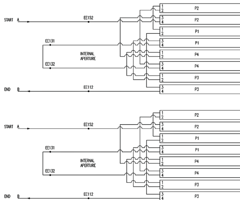
FIGURE 2.2: Electrical scheme of the two individually powered apertures of the MQY magnet [30].
