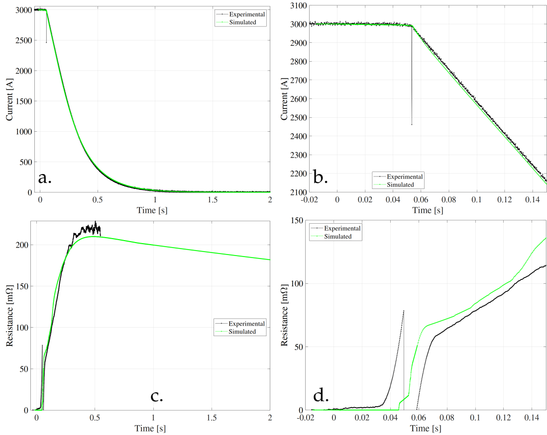
FIGURE 5.10: Quench Heaters and Delayed Energy Extraction (Test 2, see Tab. 5.1). a. Magnet current versus time. b. Zoom in the magnet current. c. Magnet resistance versus time. d. Zoom in the magnet resistance.
