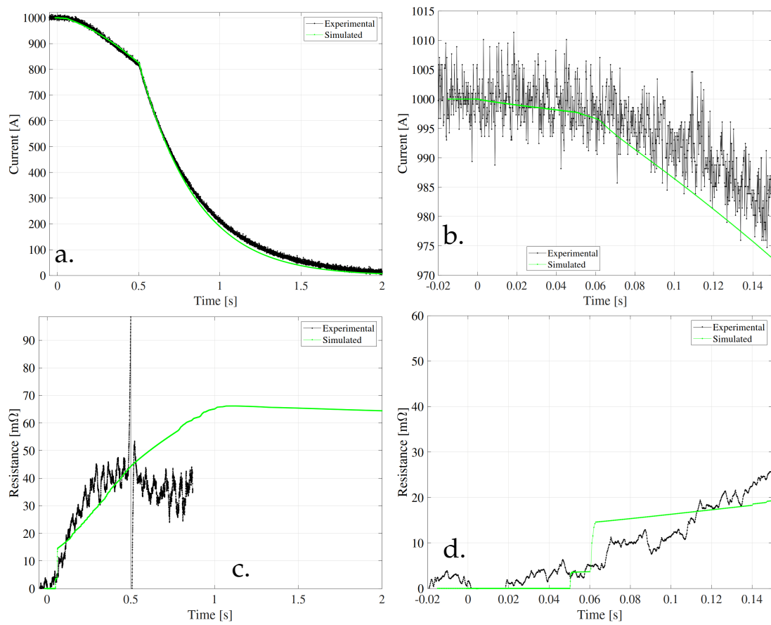
FIGURE 5.14: Quench Heaters and Delayed Energy Extraction (Test 5, see Tab. 5.1). a. Magnet current versus time. b. Zoom in the magnet current. c. Magnet resistance versus time. d. Zoom in magnet resistance.
