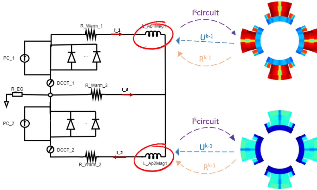
FIGURE 3.14: Working principle of the co-simulation on the LHC quadrupole circuit and the magnet.
