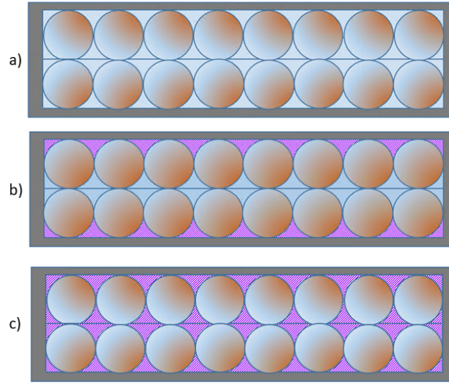
FIGURE 3.6: Quantity of helium inside the insulated cable-cross section: (a) All the voids are filled with helium. (b) Half of the voids are filled with the helium and the remaining part is filled with the insulation. (c) All the voids are filled with the insulation, the quantity of helium inside the cable cross section is zero.
