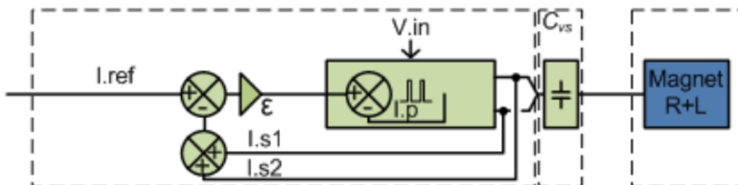
FIGURE 2.10: 2kA-8V Power Brick, high frequency. Marked in green, the current source, and in blue the load [32].
