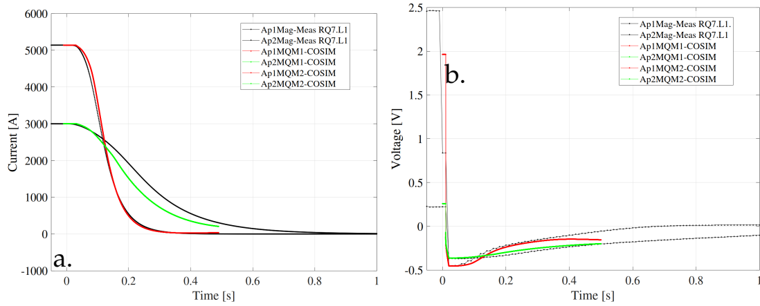
FIGURE 6.17: Simulations and measurements for a co-simulation at 1.9 K with different current values in the magnet apertures (circuit RQ7.L1). a. DCCT Current versus time. b. Voltage across the power converter versus time.
