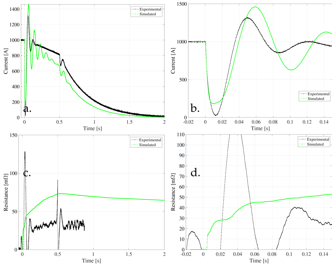
FIGURE 5.23: CLIQ and Delayed Energy Extraction (Test 11, see Tab. 5.1).
