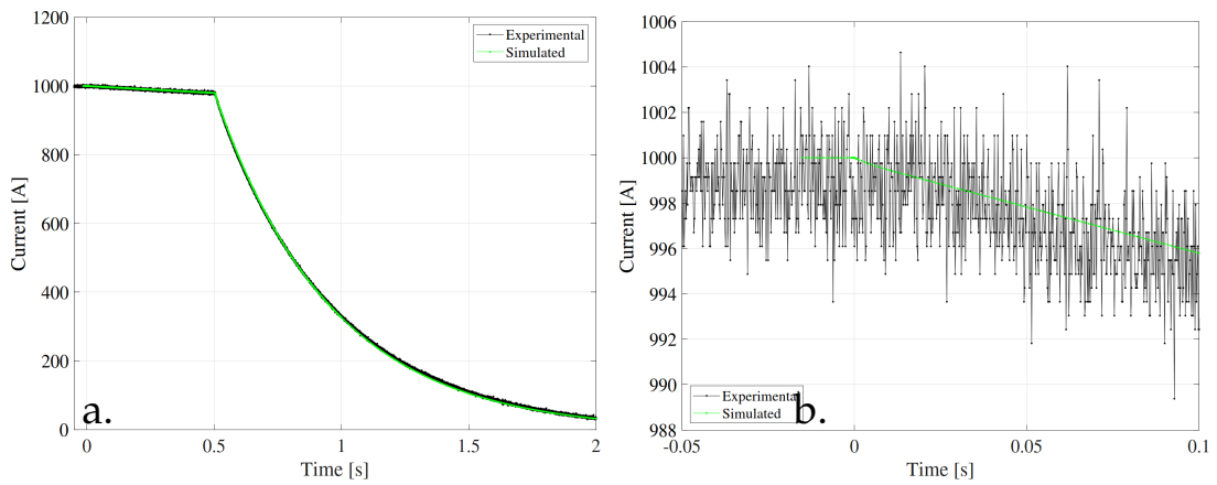
FIGURE 5.2: Delayed energy extraction only (Test 1, see Tab. 5.1). a. Measured and simulated magnet current versus time. b. Current zoom after the quench protection system starts.
