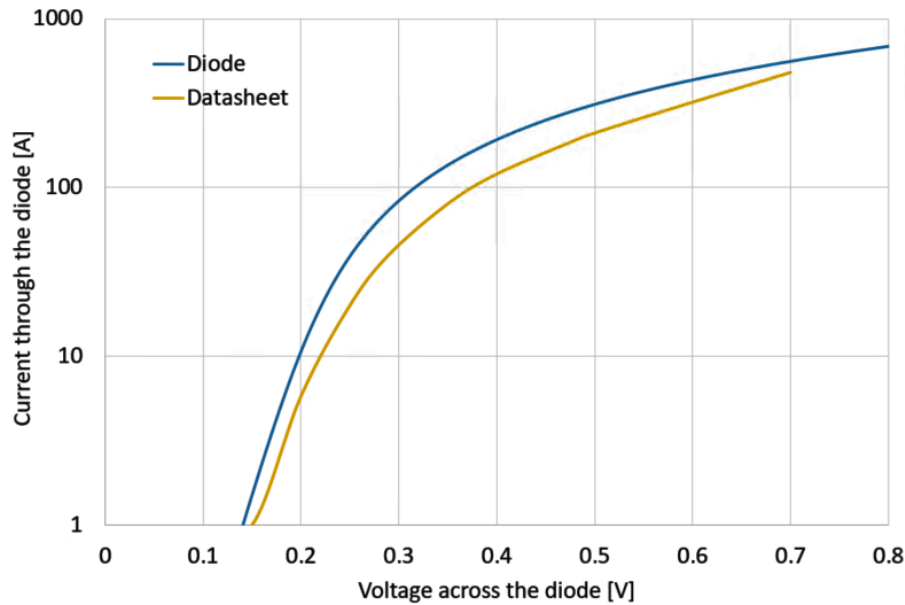
FIGURE 4.1: Diode forward characteristic curve, current versus voltage across the diode. Comparison between the data-sheet diode characteristic and the characteristic chosen during the validation of the diode.
