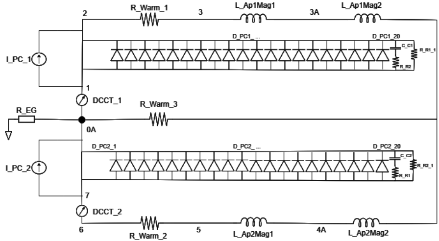
FIGURE 2.7: Schematic of the IPQ superconducting circuit, in two magnets configuration (four apertures).
