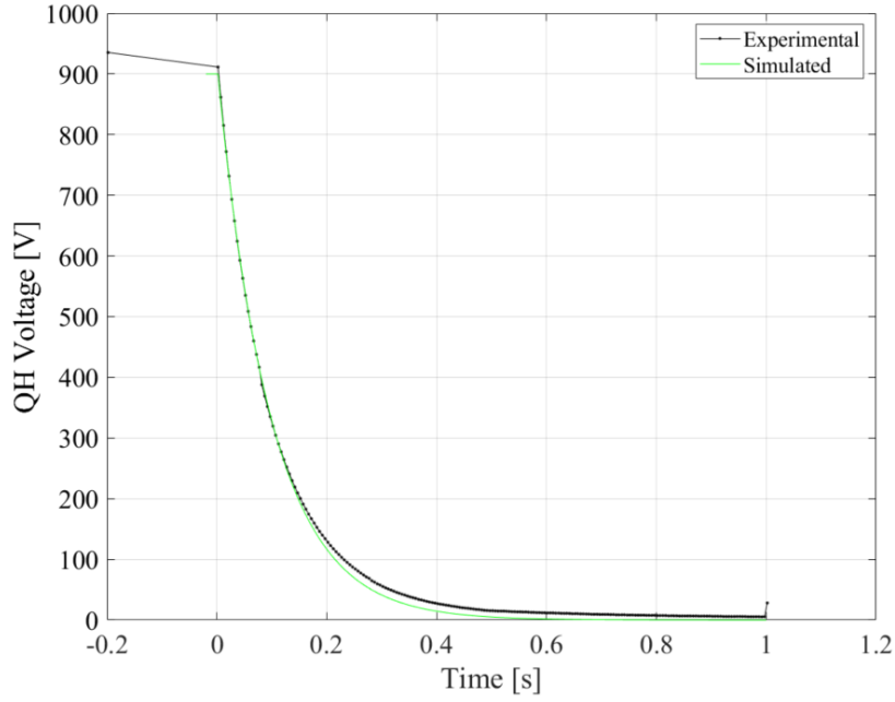
FIGURE 6.5: Voltage across the eight quench heaters versus time.
