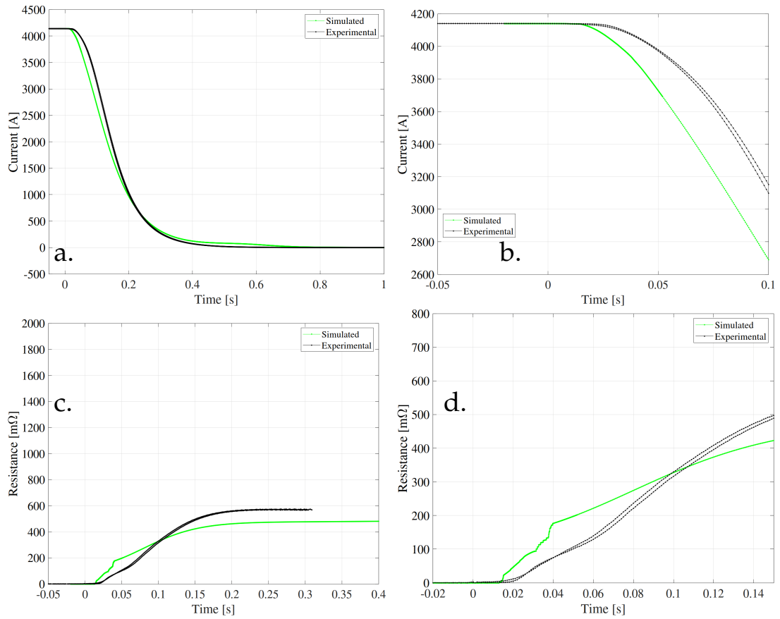
FIGURE 5.29: Simulation vs Experimental data for the validation of the MQML magnet model at 4.5 K. a. Magnet current versus time. b. Zoom in the magnet current. c. Magnet resistance versus time. d. Zoom in magnet resistance.
