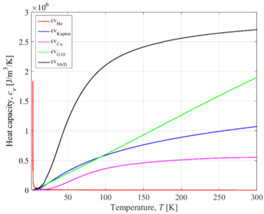
FIGURE 3.4: Heat capacity for different materials [46, 47].
