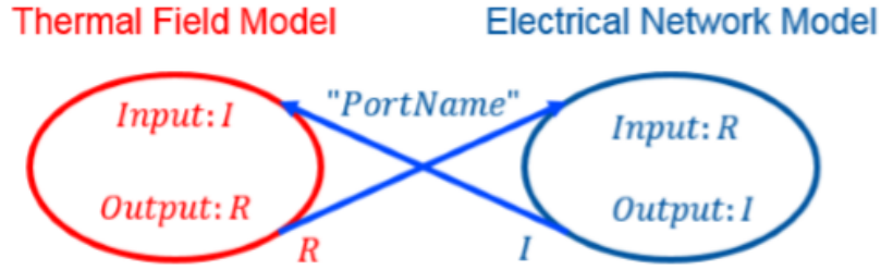
FIGURE 3.13: Representation of two ports, exchanging information [51]
