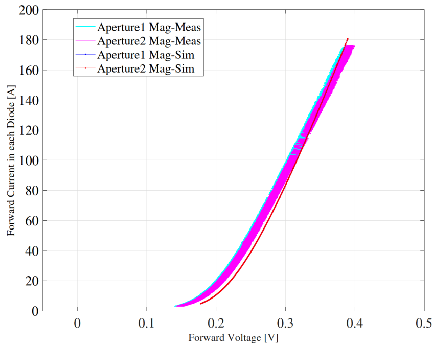
FIGURE 4.2: Forward Current vs Forward voltage. Comparison between simulated and the measured diode behaviour.
