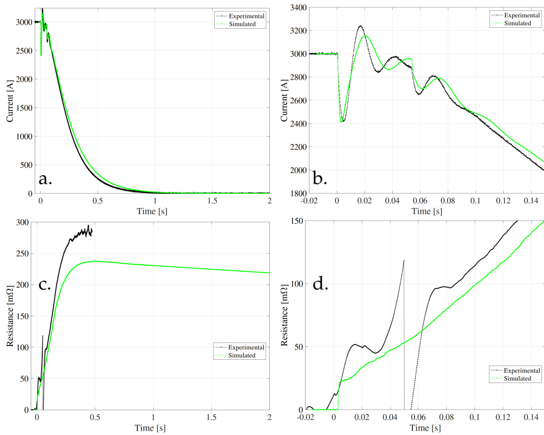
FIGURE 5.18: CLIQ and Delayed Energy Extraction (Test 6, see Tab. 5.1).
