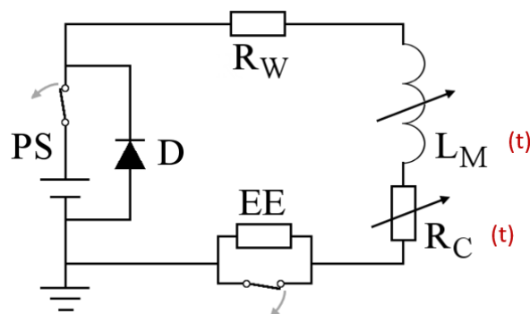
FIGURE 1.13: Simplified magnet circuit with schematic parameter of the energy-extraction protection system [15].
