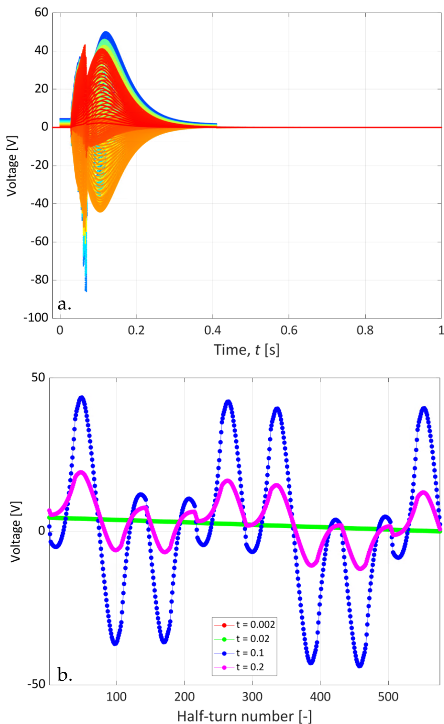
FIGURE 6.3: Voltage to ground of the co-simulation at 1.9 K (circuit RQ8.L1). a. Voltage to ground of the magnet turns versus time. b. Voltage to ground after each magnet half-turns at different selected time.
