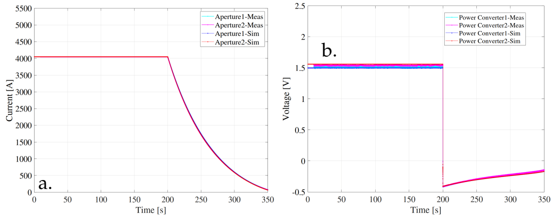
FIGURE 6.12: Simulations and measurements for a co-simulation at 4.5 K with the same current value in both magnet apertures (circuit RQ5.L8). a. DCCT Current versus time. b. Voltage across the power converter versus time.
