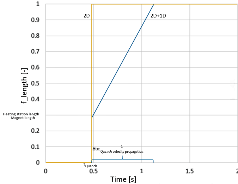
FIGURE 3.7: Longitudinal fraction of magnet turns quenched in time. The yellow curve represents the fraction of the magnet turn quenched in time on the 2D model. It quenches immediately the entire length of the turn. The blue curve represents the 2D+1D model. In this case, only the fraction of the turn in direct contact with the heating station quenches immediately.
