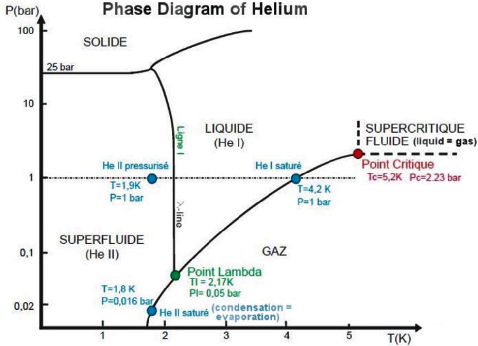
FIGURE 3.3: Phase diagram of the helium [44]
