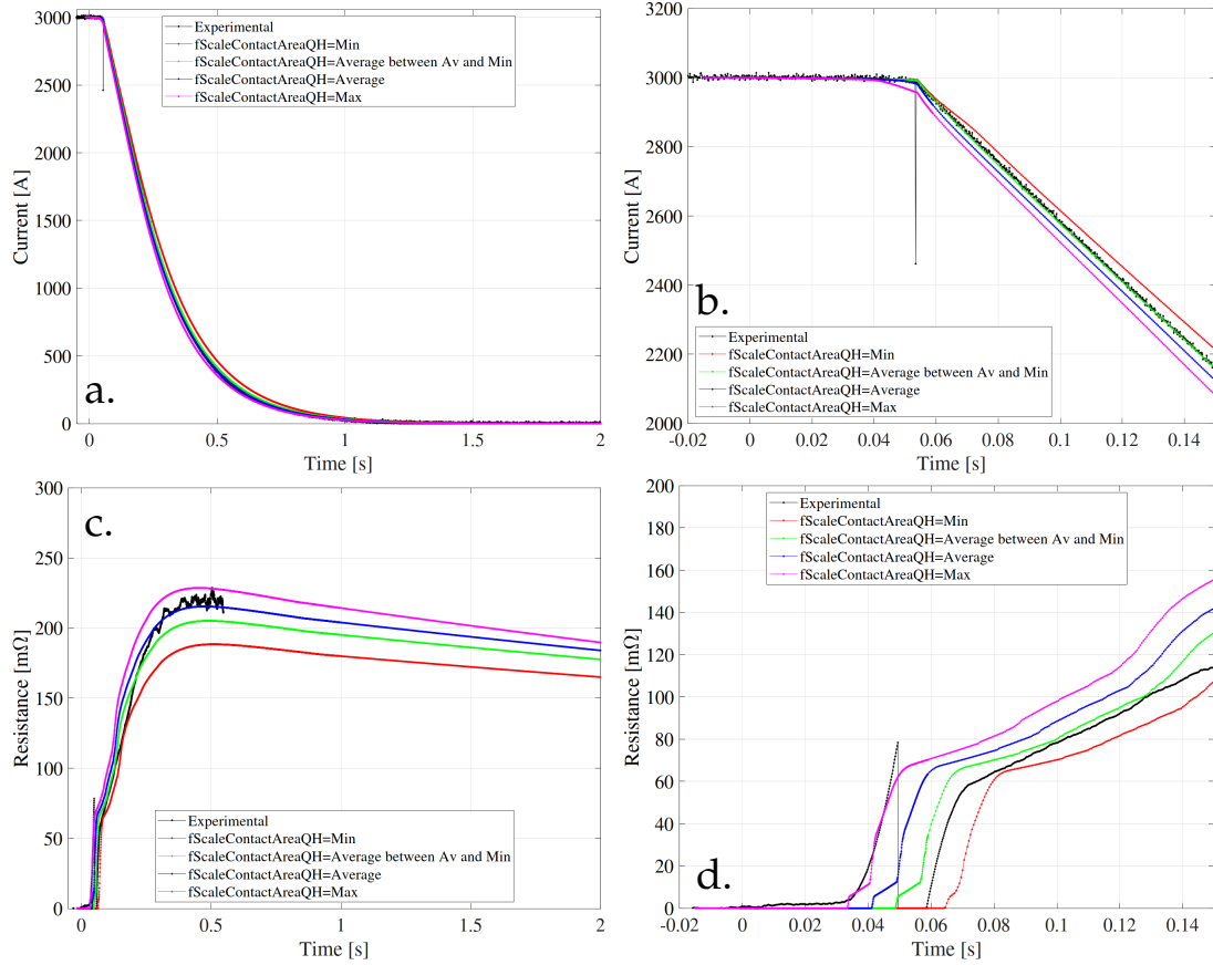
FIGURE 5.8: Simulations and measurements for different fScaleContactAreaQH . fScaleContactAreaQH=Min , represents the minimum spread of the heat flux on the cables (case1).
