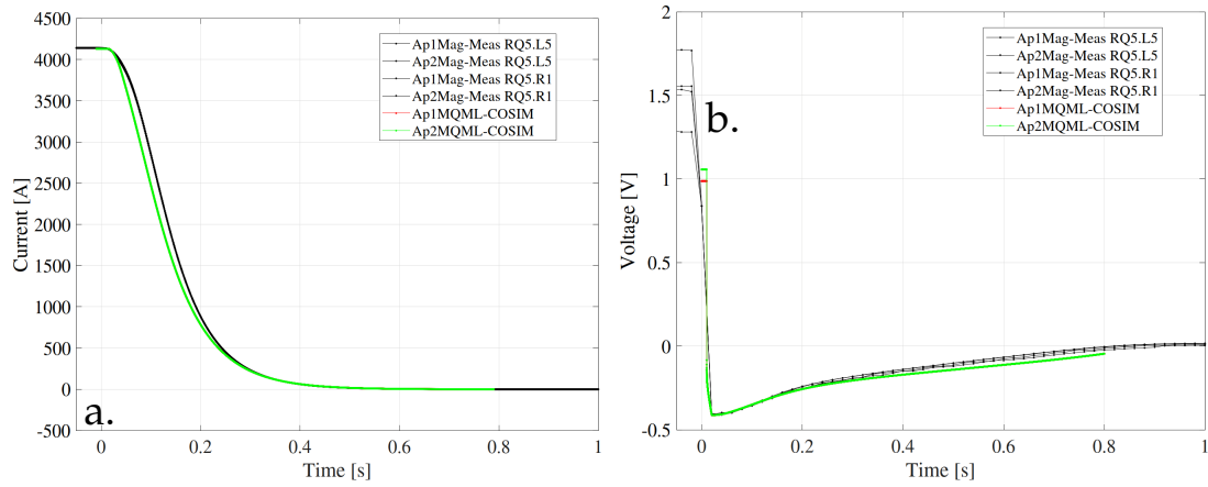
FIGURE 6.11: Simulations and measurements for a co-simulation at 4.5 K with the same current value in both magnet apertures (circuit RQ5.L5). a. DCCT Current versus time. b. Voltage across the power converter versus time.
