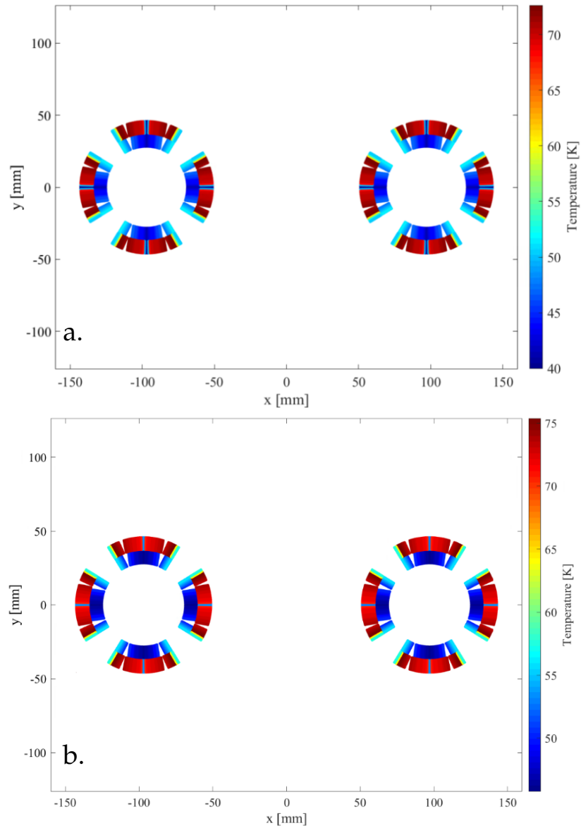
FIGURE 6.19: Temperature distribution in the magnet cross-section for a co-simulation at 1.9 K (circuit RQ9.L8). a. Temperature distribution in the MQM magnet cross-section. b. Temperature distribution in the MQMC magnet cross-section.
