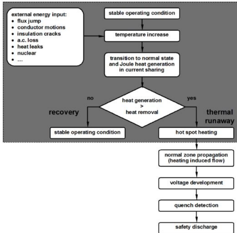
FIGURE 1.9: An event tree following an external energy input, and leading from stable operating conditions back to stable operation or to a magnet quench. The stability design and analysis are concentrated on the shaded area in the event tree [20].
