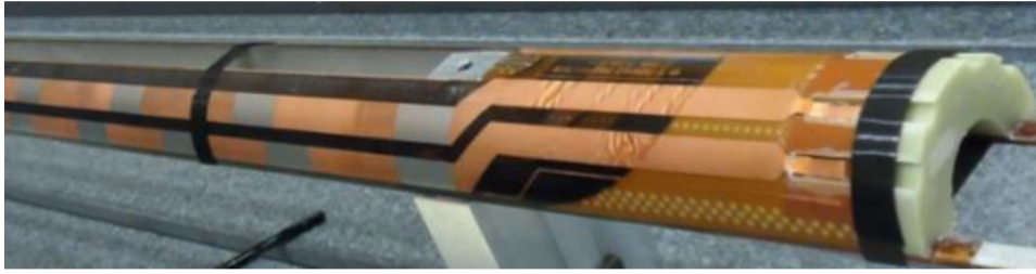
FIGURE 5.6: Photo of the HL-LHC quench heaters. The fractions of stainless steel (heating station) and copper are well identifiable [61].
