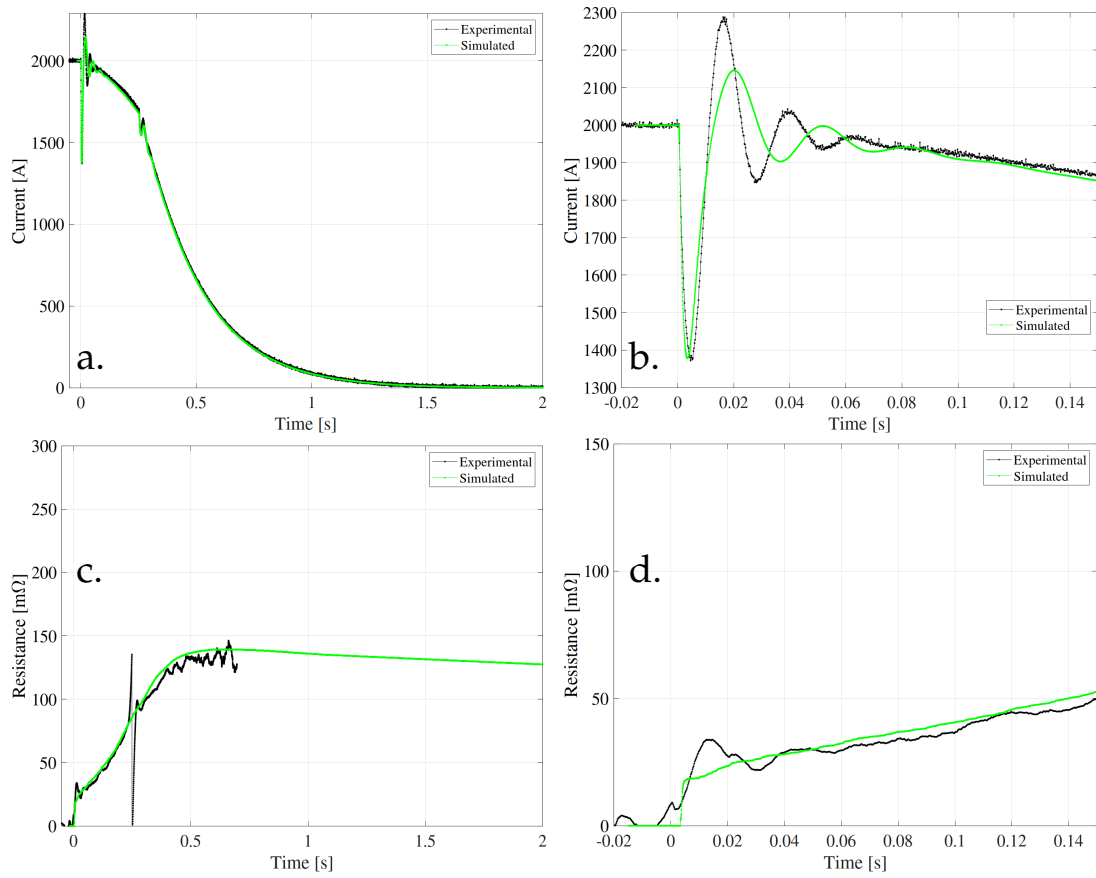
FIGURE 5.19: CLIQ and Delayed Energy Extraction (Test 7, see Tab. 5.1). a. Magnet current versus time. b. Zoom in the magnet current. c. Magnet resistance versus time. d. Zoom in magnet resistance.
