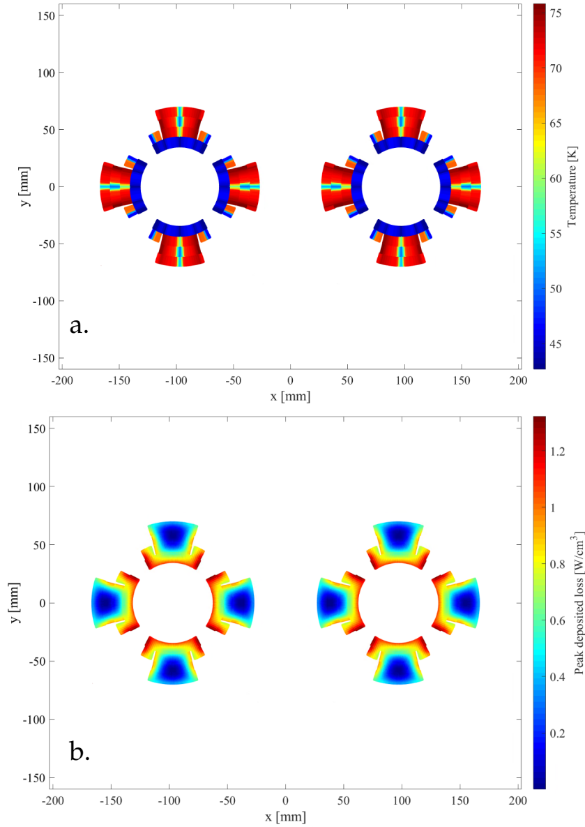
FIGURE 6.8: Temperature (a.) and deposited loss (b.) on the MQY magnet cross-section after a co-simulation at 4.5 K (circuit RQ4.L6).
