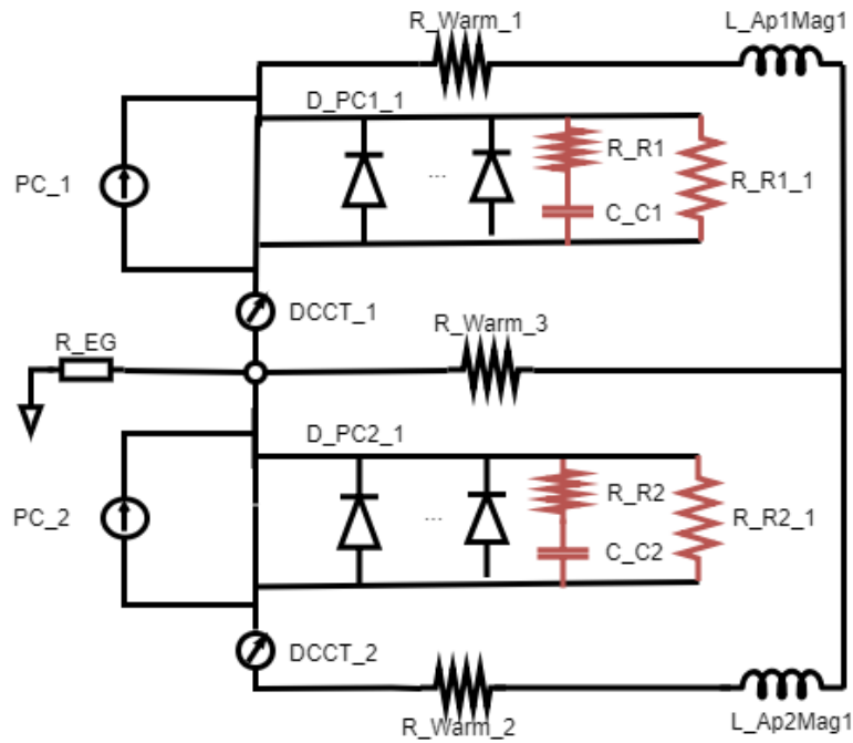
FIGURE 4.3: Schematic of the IPQ circuit with the highlighted parasitic components.
