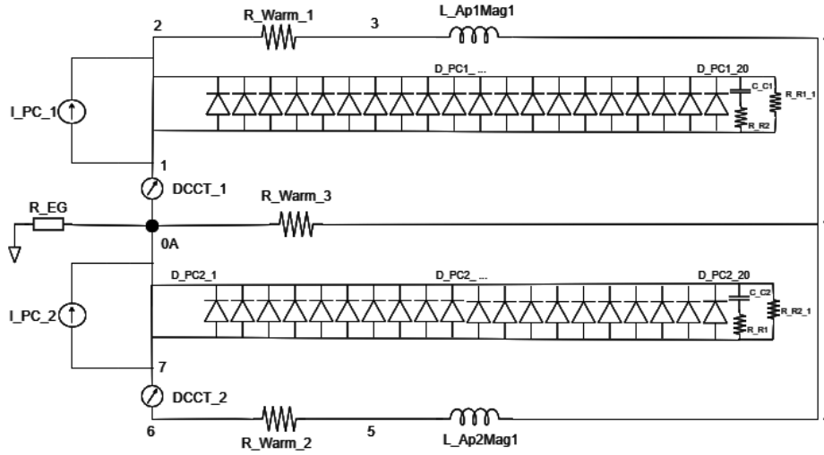
FIGURE 2.6: Schematic of the IPQ superconducting circuit, in one magnet configuration (two apertures).
