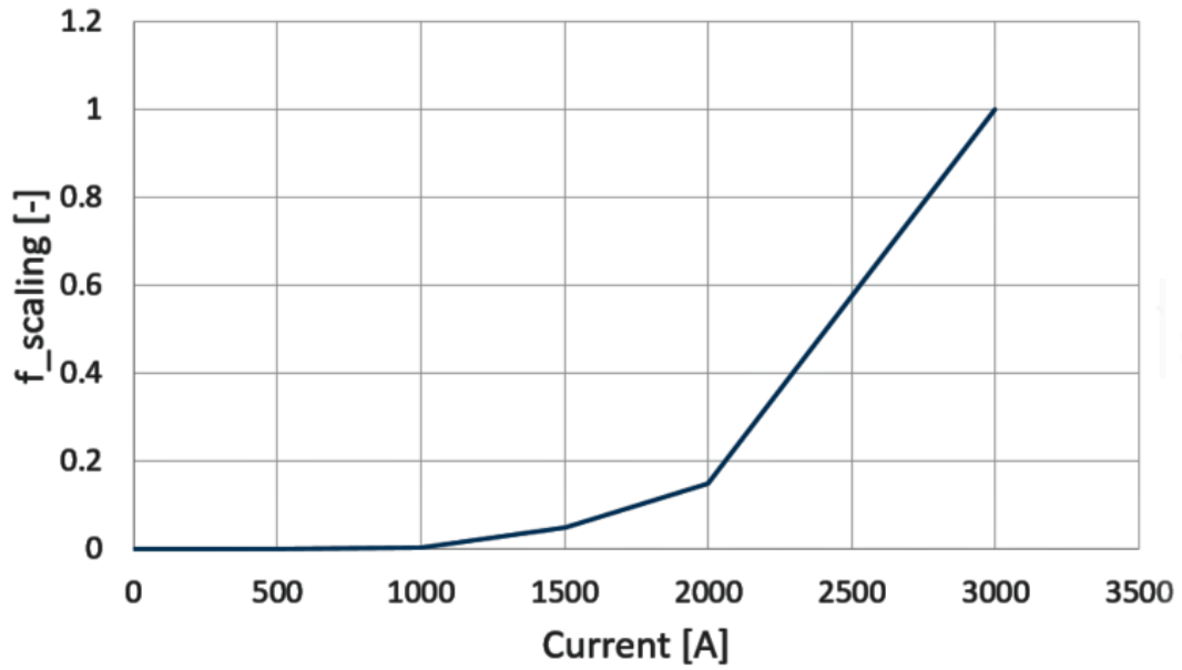
FIGURE 5.15: Trend of the scaling factor. At 3 kA the effect of the scaling factor is negligible, while it have a big impact at low currents.
