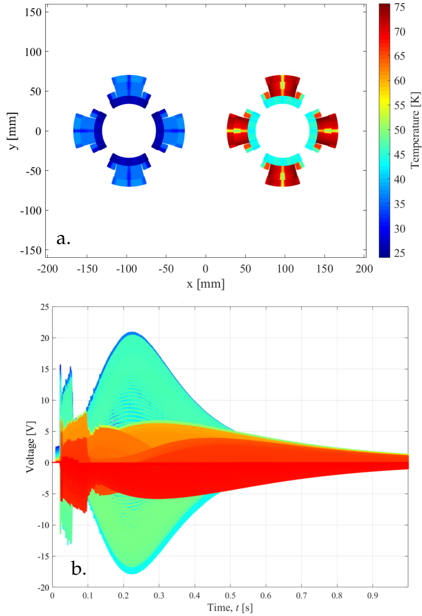
FIGURE 6.16: Simulations and measurements for a co-simulation at 4.5 K with unbalanced current in the magnet apertures (circuit RQ4.L5). a. Temperature distribution in the MQY magnet cross-section. b. Voltage to ground versus time of all the magnet turns.
