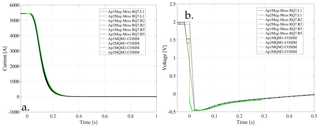
FIGURE 6.6: Simulations and measurements for a co-simulation at 1.9 K with the same current value in both magnets apertures (circuit RQ7.L1). a. DCCT Current versus time. b. Voltage across the power converters versus time.
