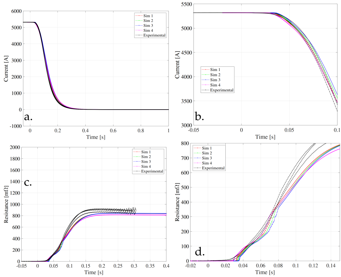
FIGURE 5.28: Best simulations for the MQML magnet model using the Sweep Parameter Notebook. a. Magnet current versus time. b. Zoom in the magnet current. c. Magnet resistance versus time. d. Zoom in magnet resistance.
