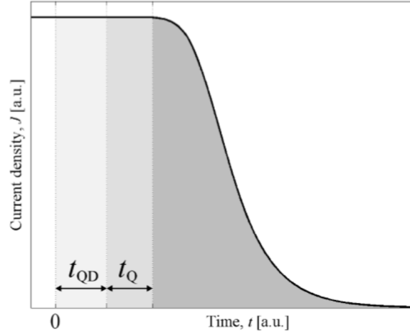
FIGURE 1.10: Coil protection phases. The quench starts in t=0 . The quench is detected, validated and the protection system is triggered in the time window t_{QD} . The entire coil is transferred to the normal state by the protection system during the time t=t_{QD}+t_Q [15].
