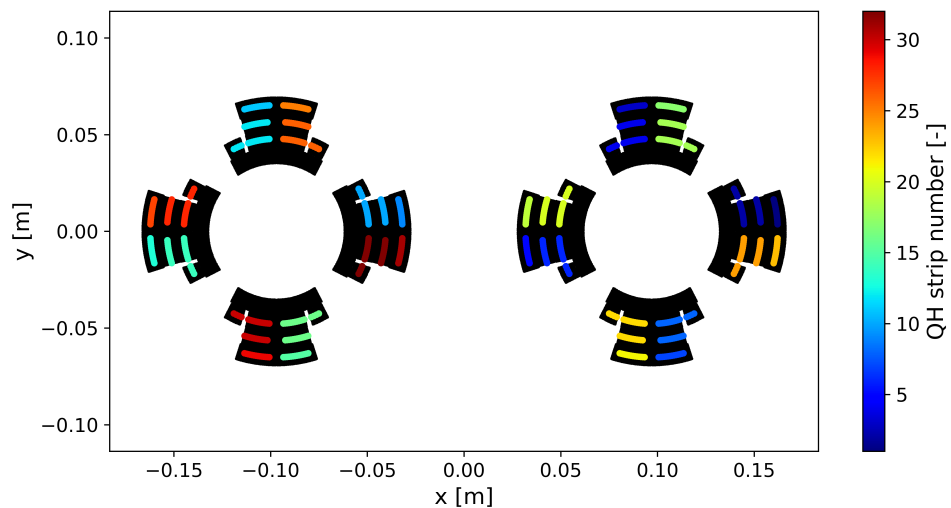
FIGURE 3.12: Heat exchange between half-turns and quench heaters generated by the SWAN notebook. The half-turns to which quench heater strips are attached are highlighted with colored points. The different colors follow the number of the quench heater strips assumed in the LEDET file.
