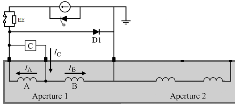
FIGURE 5.16: Schematic of the magnet test circuit including the CLIQ system protection in one aperture [59].
