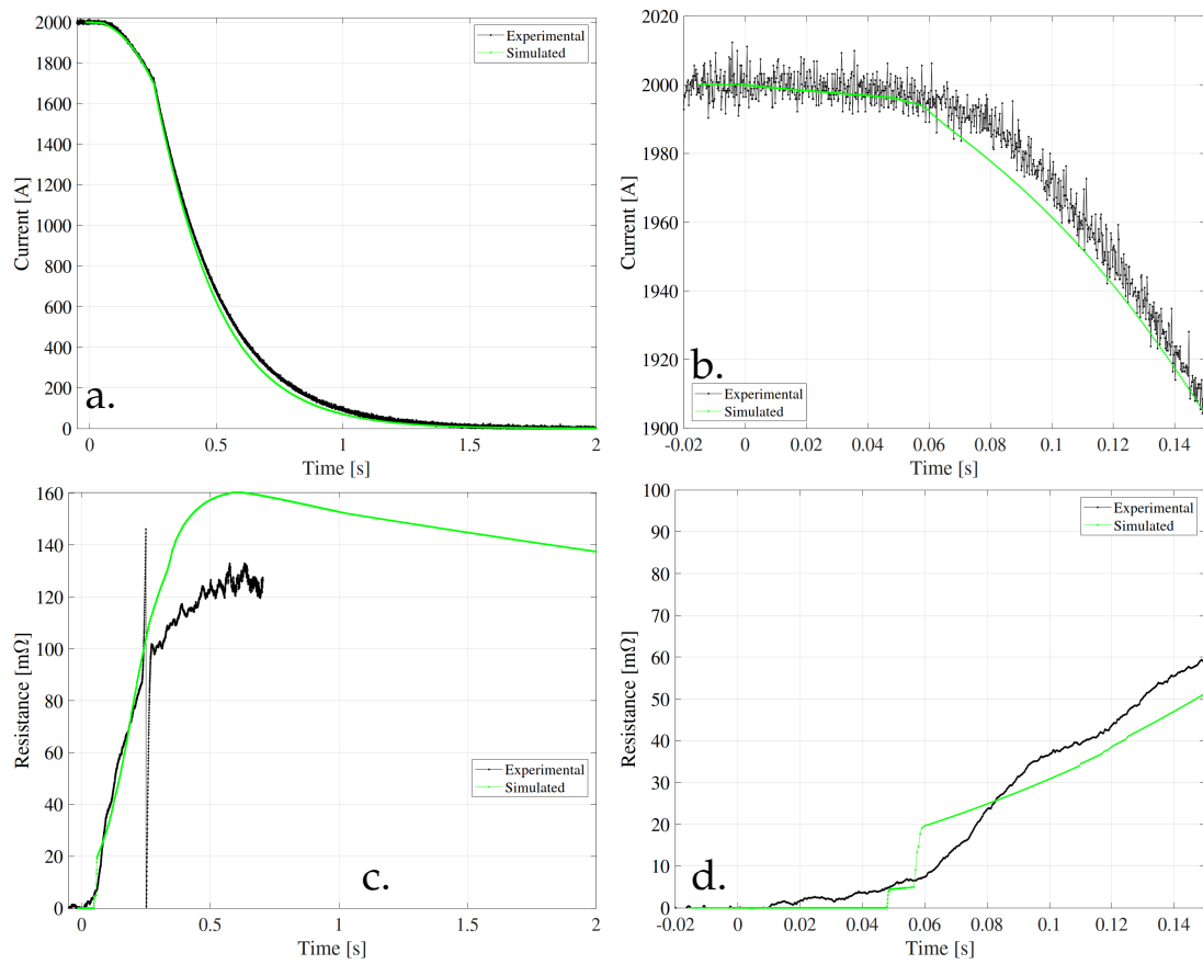
FIGURE 5.12: Quench Heaters and Delayed Energy Extraction (Test 3, see Tab. 5.1). a. Magnet current versus time. b. Zoom in the magnet current. c. Magnet resistance versus time. d. Zoom in magnet resistance.
