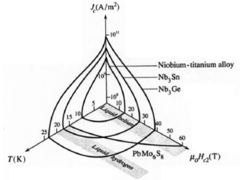
FIGURE 1.4: Critical surface of Nb-Ti, Nb 3 Sn and Nb 3 Ge in the T,B,J space [13].
