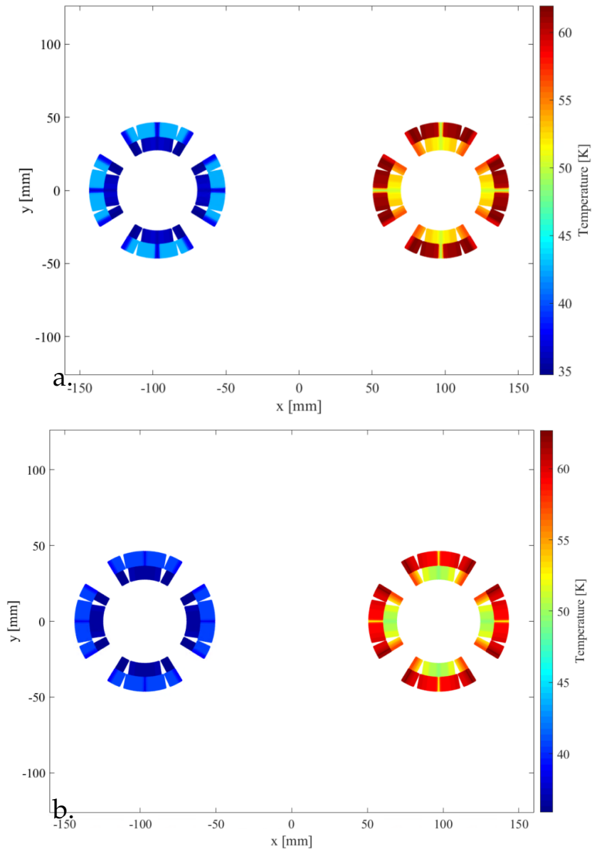
FIGURE 6.21: Temperature distribution in the magnet cross-section for a co-simulation at 4.5 K (circuit RQ6.R2). a. Temperature distribution in the MQM magnet cross-section. b. Temperature distribution in the MQML magnet cross-section.
