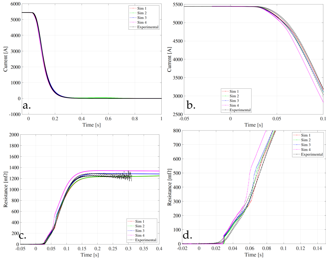
FIGURE 5.26: Best simulations for the MQM magnet model using the Sweep Parameter Notebook. a. Magnet current versus time. b. Zoom in the magnet current. c. Magnet resistance versus time. d. Zoom in magnet resistance.
