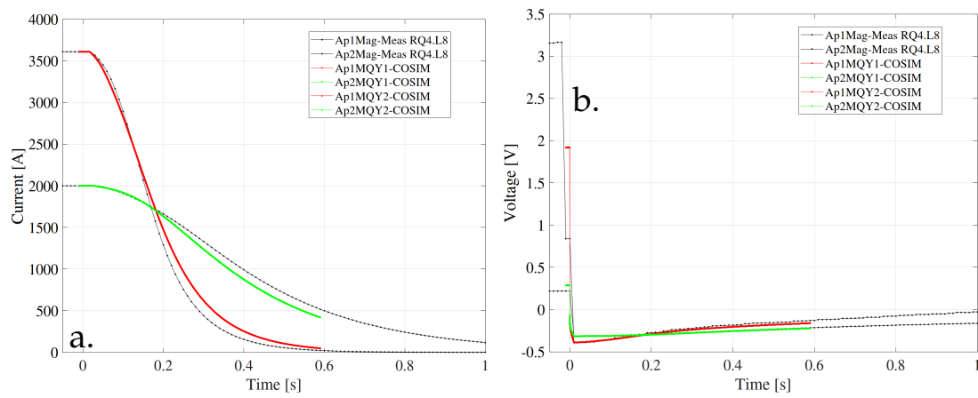
FIGURE 6.15: Simulations and measurements for a co-simulation at 4.5 K with different current values in the magnet apertures (circuit RQ4.L8). a. DCCT Current versus time. b. Voltage across the power converter versus time.
