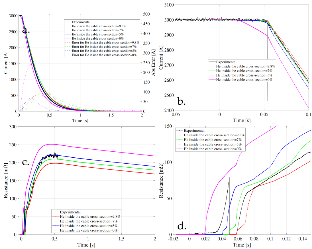
FIGURE 5.5: Simulations and measurement for different fractions of helium inside the insulated cable cross-section. a. Magnet current versus time. b. Zoom in the magnet current. c. Magnet resistance versus time. d. Zoom in the magnet resistance.
