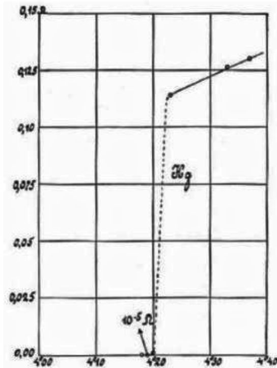
FIGURE 1.2: Historic plot of resistance versus temperature of the mercury material. From the 1922 Onnes experiment, shows the superconducting transition at 4.20 K [7].
