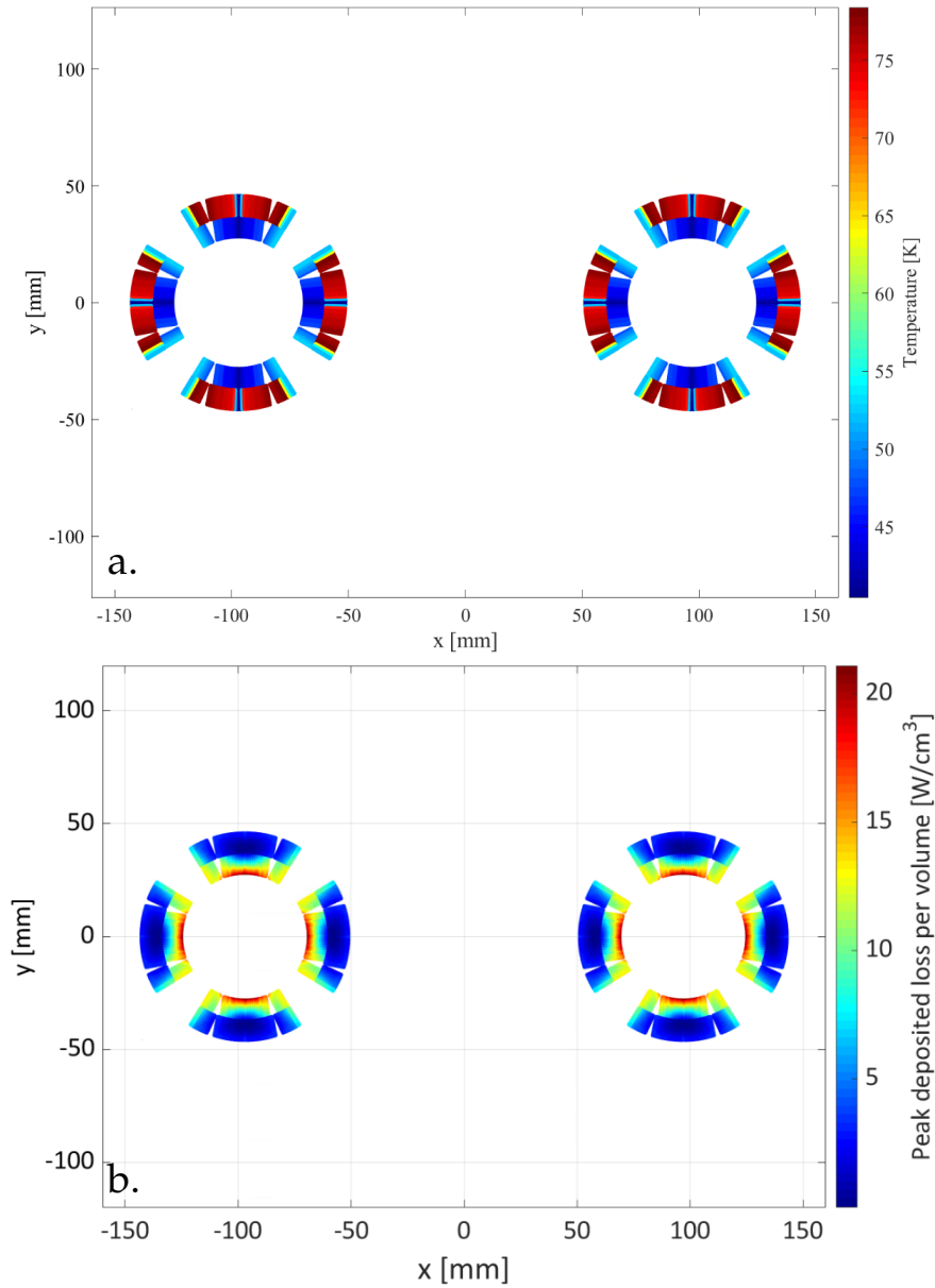
FIGURE 6.2: Temperature in the magnet model cross-section and peak inter-filament coupling loss for a co-simulation at 1.9 K with the same current value in both magnet apertures (circuit RQ8.L1). a. Peak temperature in the MQML magnet model cross-section. b. Peak inter-filament coupling loss per unit volume in the magnet cross-section.
