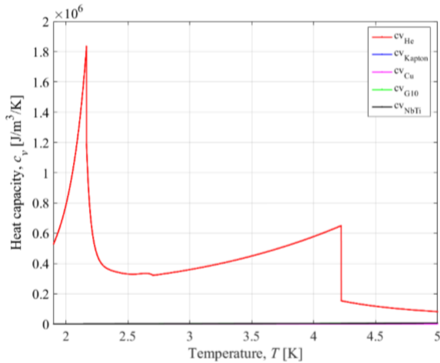
FIGURE 3.5: Heat capacity of the Helium [46, 47].
