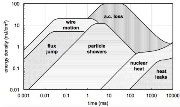
FIGURE 1.8: Spectrum of energy perturbations as a function of the characteristic time of energy deposition [20].
