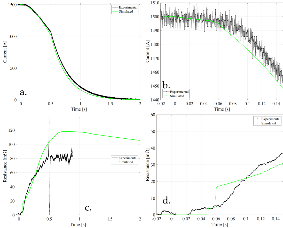
FIGURE 5.13: Quench Heaters and Delayed Energy Extraction ( Test 4 , see Tab. 5.1). a. Magnet current versus time. b. Zoom in the magnet current. c. Magnet resistance versus time. d. Zoom in magnet resistance.
