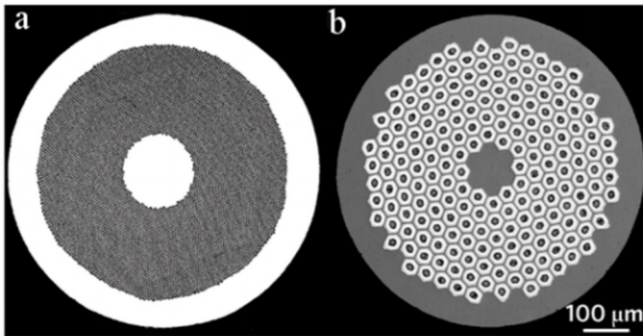
FIGURE 1.6: Wires with superconducting filaments.(a) Wire made of Nb-Ti filaments embedded in a copper matrix. (b) Wire made of Nb 3 Sn filaments [17].
