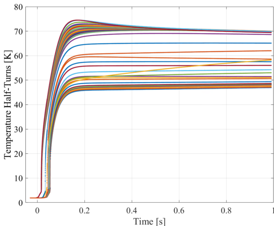
FIGURE 6.13: Temperature of each half-turn in the MQML magnet model versus time at 4.5 K (circuit RQ5.L5).
