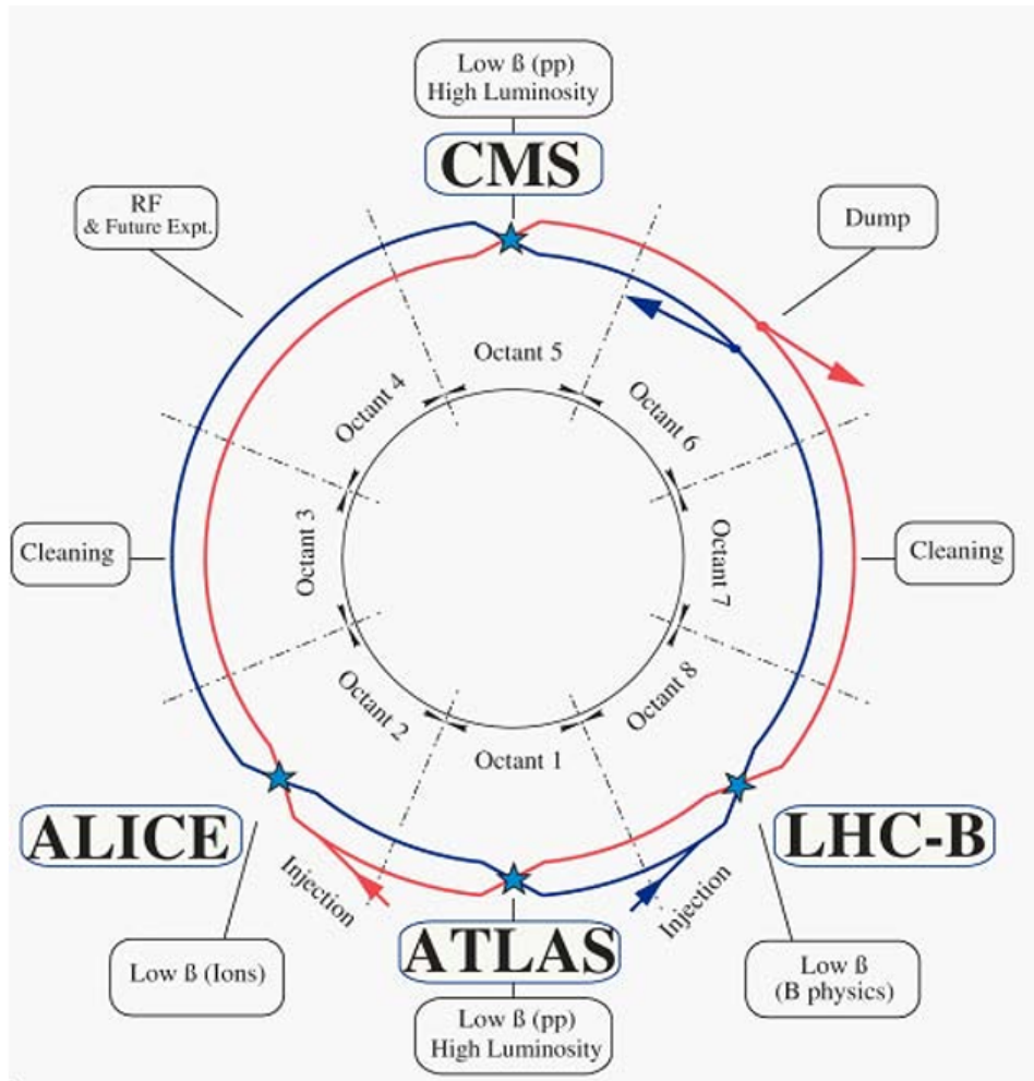
FIGURE 2.1: Schematic layout of the LHC. [28]
