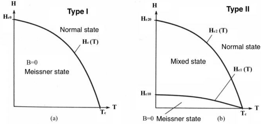
FIGURE 1.5: Comparison between the H-T diagram of type-I (a) and type-II (b) superconductor [14].
