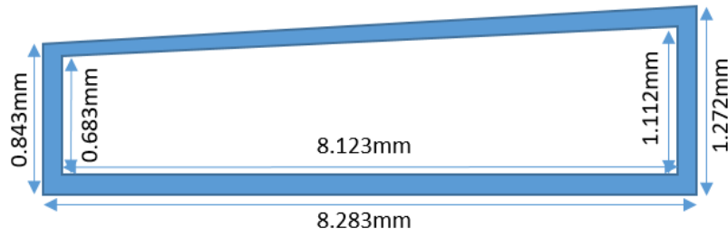
FIGURE 5.4: Schematic design and size of the MQY cable bare.
