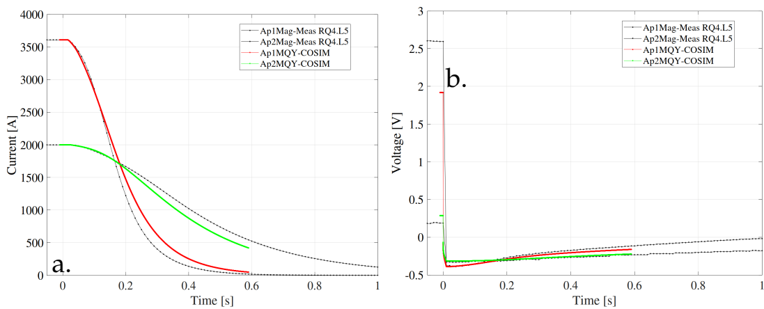
FIGURE 6.14: Simulations and measurements for a co-simulation at 4.5 K with different current values in the magnet apertures (circuit RQ4.L5). a. DCCT Current versus time. b. Voltage across the power converter versus time.
