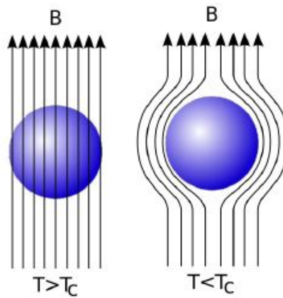
FIGURE 1.3: Diagram of the Meissner-Ochsenfeld effect. Magnetic field lines, represented as arrows, are excluded from a superconductor when it is below its critical temperature [12].
