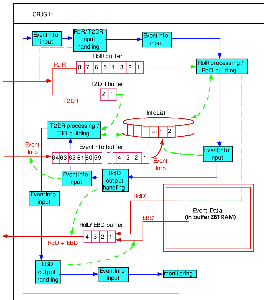
Figure 3.3: Schematic view of the software used in the performance measurement of the CRUSH module. See the text for details. Figure taken from [48].
