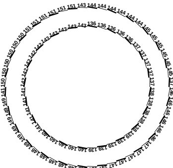
Module to MUR map of SCT endcap wheel 6.
