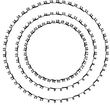
SCT endcap ROB tower mapping endcap wheel 5.
