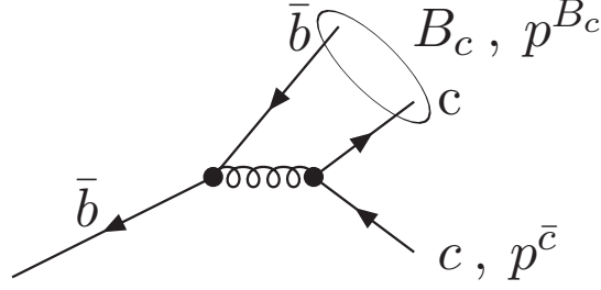
Figure 6.7: Kinematical variables used in the derivation of b \rightarrow B_c(^1S_0) .
