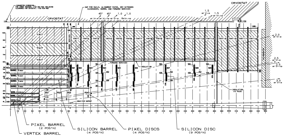
Figure 2.4: Cross-sectional view of the cylindrical Inner detector. The view is cut along the z axis and shows only the forward part of the Inner detector. The picture shows the geometry which was foreseen in 1997 [35]. In the most recent geometry the pixel detector has three discs instead of the four depicted here.
