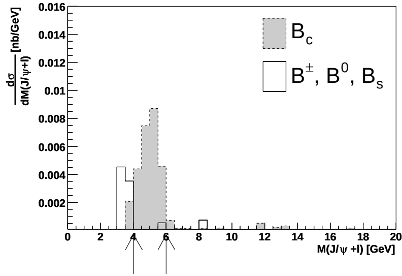
Figure 7.24: Invariant J/\psi + l^\pm mass distribution, where the J/\psi candidate passes offline mass and vertex cuts. The three lepton vertex fit satisfies \chi^2/N_{d.o.f.} < 8.0 . The mass range associated with the B_c is limited to the region between the arrows.
