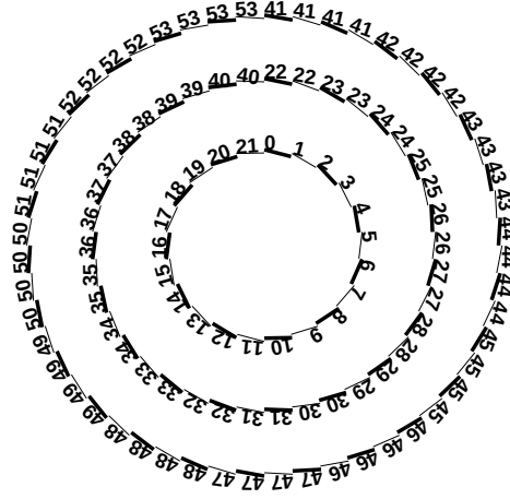
Pixel barrel ROB layer mapping.
