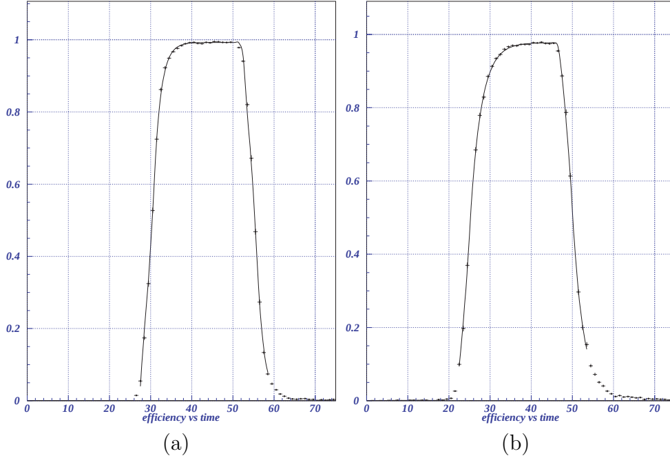
Figure 2.6: Full pixel module (sensor + integrated electronics) efficiencies vs. time at \sim -5^\circ\text{C} . Unirradiated pixel module, \langle \epsilon \rangle = 99.3\% during a time plateau of \sim 10\text{ ns} (a). Irradiated pixel module, i.e. after a dose of 60\text{ MRad} or 1 \times 10^{15}\text{ }1\text{ MeV}_{n\text{-equiv}} , \langle \epsilon \rangle = 97.7\% during a time plateau of 12\text{ ns} (b). Figures taken from [36].
