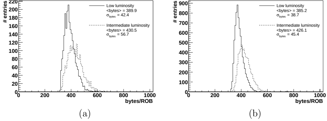
Figure 5.4: Distribution of input event fragment sizes per barrel ROB (a) and per endcap ROB (b). The distribution was made by looping over all appropriate ROB. The solid line gives the distribution for low luminosity, the dashed line for intermediate luminosity.
