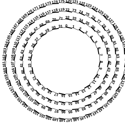
Figure A.1: Map of SCT barrel modules to MURs. Shown are the four concentric SCT barrels. The view is perpendicular to the beam-axis, cutting the SCT barrel in half. One MUR here contains 6 SCT modules along the z direction.
