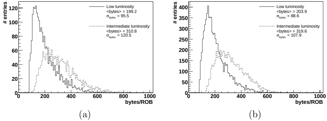
Figure 5.5: Distribution of output event fragment sizes per barrel ROB (a) and endcap ROB (b) where the zero suppression algorithm with offset has been used. For the barrel ROB, the optimal number of 5 header bits for low luminosity (solid line) and 4 header bits for intermediate luminosity (dashed line) was used. For endcap ROB, the optimal number of 5 header bits for low luminosity and 4 header bits for intermediate luminosity was used.
