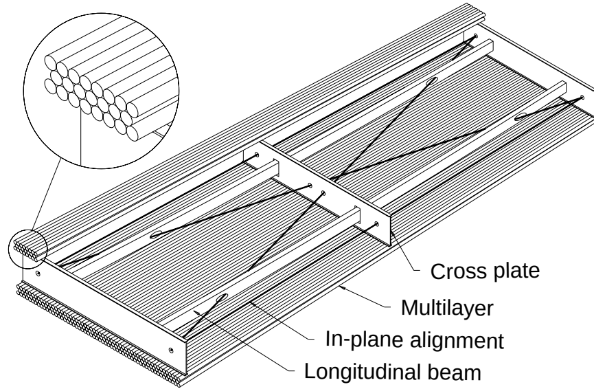
Figure 2.14: Schematic overview of a MDT chamber with 2 multi-layers, each consisting of 3 rows of staggered tubes.
