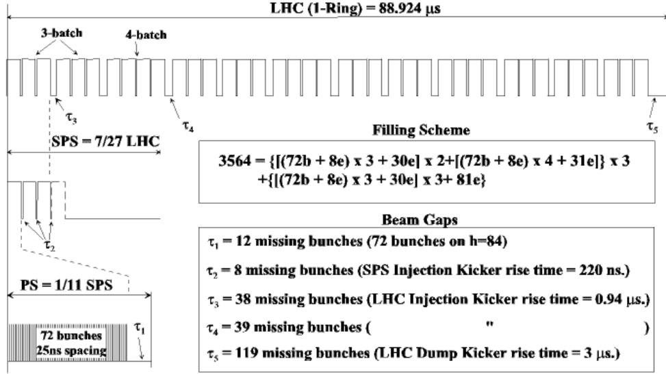
Figure 2.2: Summary of the LHC bunch structure for protons. Figure taken from [33].
