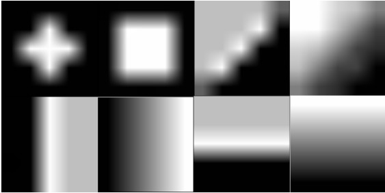
Figure 3: Sample of the initial filters used in the convolution layer of the network. 22 filters total including 16 from smooth-sharp edges each rotated eight times.
