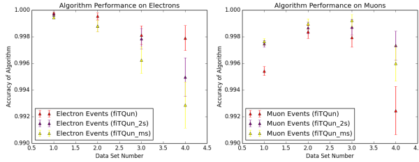
Figure 4: Performance of three fiTQun regimes for electron and muon events and each image set. Red: default fiTQun with single ring electron and muon fits (99.77%), Purple: fiTQun with two-ring segmented muon fit (99.846%), Yellow: fiTQun with three-ring segmented muon fit (99.836%).
