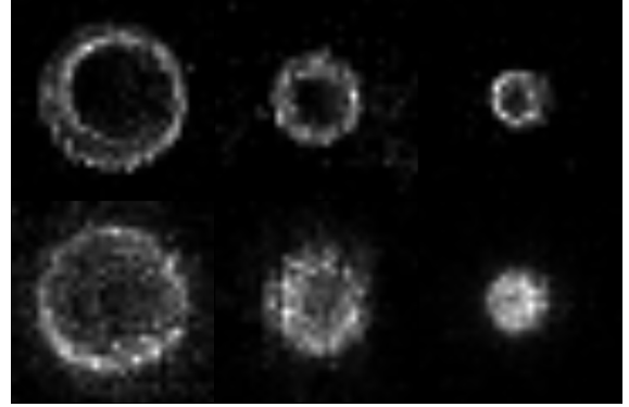
Figure 2: Output images of the cone projection described in figure 1. Top: muon rings, Bottom: electron rings, Left to Right: data set 1, 3, and 4.
