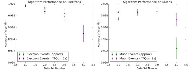
Figure 5: Comparison of CNN classification (Green: 99.89%) to fiTQun with two-ring segmented muon fit (Purple: 99.846%).
