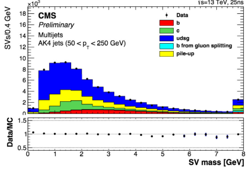
Figure 4.18: A plot of the mass of the jet originating at the secondary vertex which is used in order to differentiate jets from heavy and light flavor decay.
