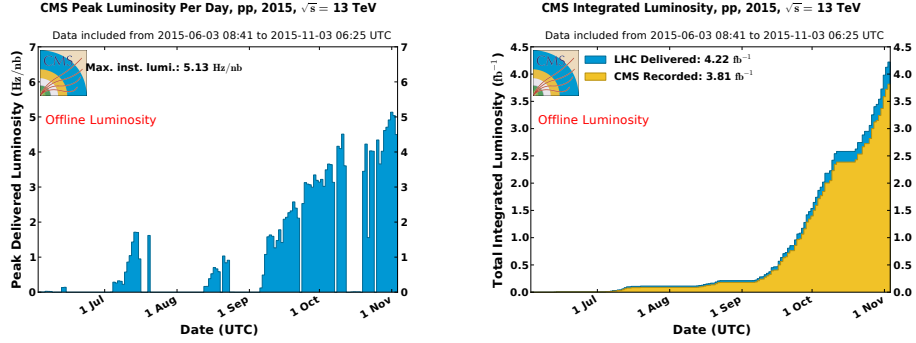
Figure 2.3: The peak instantaneous luminosity per day during the 2015 data taking period is shown on the left and the total integrated luminosity is shown on the right in this figure.
