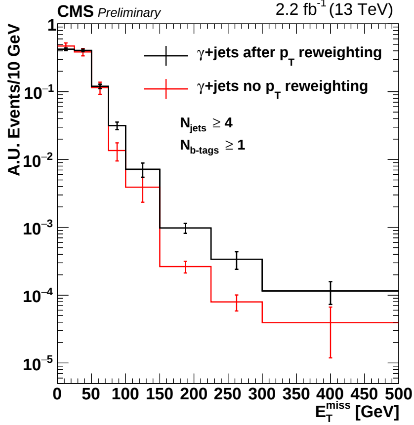
Figure 5.2: The E_T^{\text{miss}} distributions are shown before reweighting the \gamma + \text{jets} sample in p_T (red) and after reweighting (black) for \gamma + \text{jets} events in signal region B where at least 1 jet is required to be b-tagged. The distributions are normalized to unit area.
