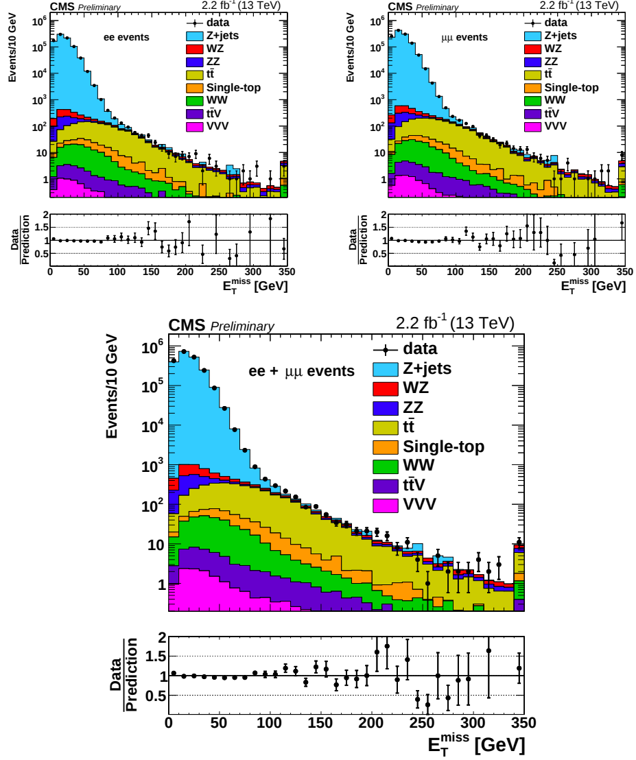
Figure 3.5: The E_T^{\text{miss}} distribution is shown with data vs. MC for events while only requirement two leptons with |M_{\ell\ell} - M_Z| < 10 \text{ GeV} . The top row shows ee events on the left and \mu\mu events on the right, and the bottom row shows ee + \mu\mu events together. The MC is normalized to data.
