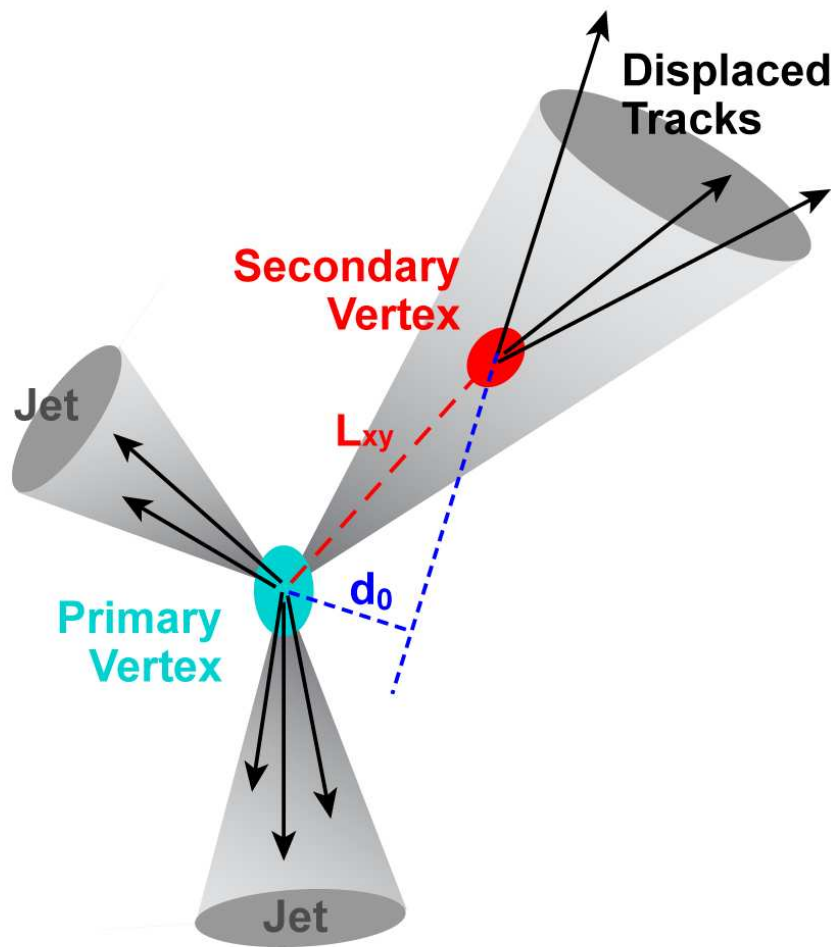
Figure 4.19: A plot showing a jet forming away from the primary vertex of a heavy flavor parton, for example a b or c quark.
