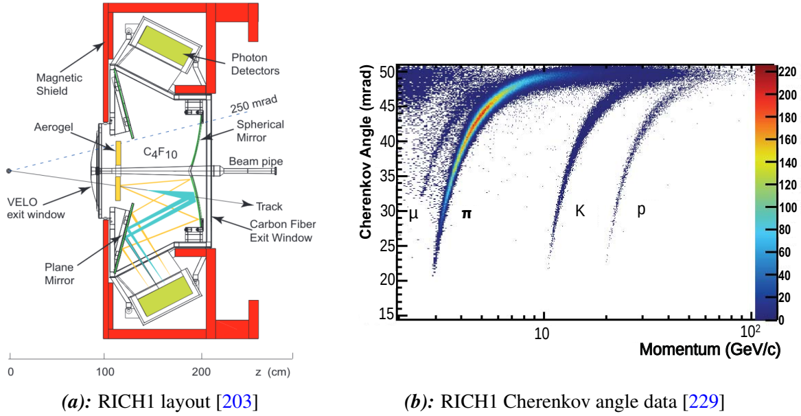
Fig. 2.10: Left - Side-view of the RICH1 detector as found in run-1, including typical paths taken by Cherenkov photons emitted in the aerogel and C_4F_{10} radiators. Right - Distribution of reconstructed Cherenkov angles against track momentum, for photons produced in the C_4F_{10} radiator in RICH1, as recorded in data. The “band” structures arising from different particles are highlighted.
