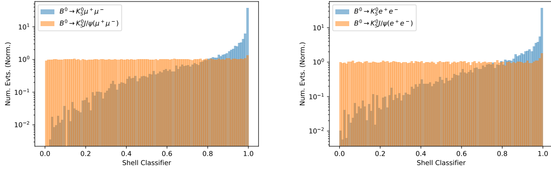
Fig. 6.2: Output distributions of \text{BDT}_{\text{Shell}} , as found in fully-selected B^0 \rightarrow K_S^0 \mu^+ \mu^- (left) and B^0 \rightarrow K_S^0 e^+ e^- (right) MC samples, plus the corresponding J/\psi control-mode decays.
