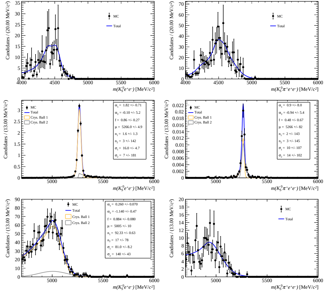
Fig. 4.35: Results of fits to m(B) , determining fit PDFs for J/\psi leakage (top), misidentified B \rightarrow K^{(*)} \pi^+ \pi^- (middle), and partially-reconstructed kaon (bottom) backgrounds, in the B^0 \rightarrow K_S^0 e^+ e^- (left) and B^+ \rightarrow K^{*+} e^+ e^- (right) channels.
