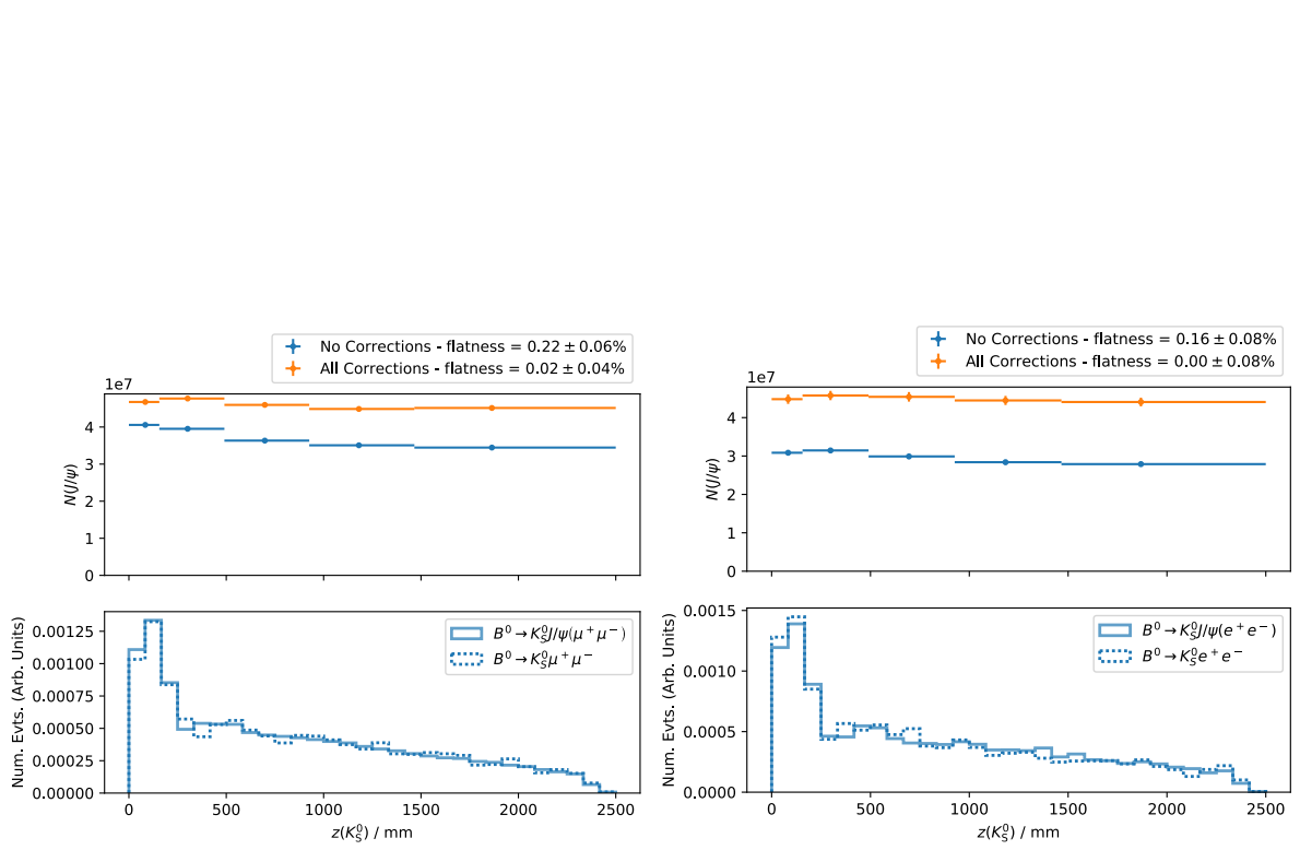
Fig. C.1: Differential measurements of efficiency-adjusted yields across different variables, found from fits to B^0 \rightarrow J/\psi(\mu^+ \mu^-) K_S^0 (left) and B^0 \rightarrow J/\psi(e^+ e^-) K_S^0 (right) data, across all years, with different weighting schemes applied when calculating efficiencies (top halves of plots), and the distributions of binned variables in the fully-selected and corrected rare-mode and control-mode MC (bottom halves of plots). Flatness parameter values are shown in the legends above the plots. ( Cont. )
