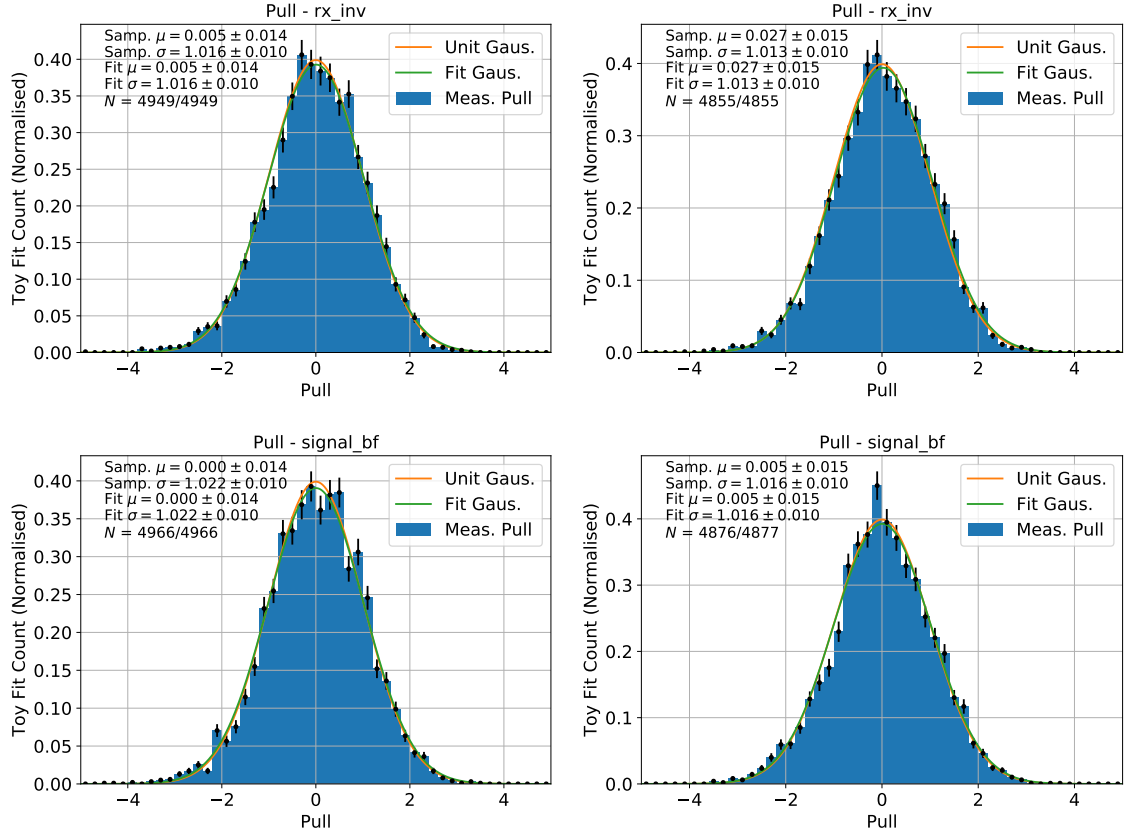
Fig. 7.3: Distributions of pull values for R_{K_S}^{-1} (top left), R_{K^{*+}}^{-1} (top right), and the differential branching fractions for B^0 \rightarrow K^0 e^+ e^- (bottom left) and B^+ \rightarrow K^{*+} e^+ e^- (bottom right), as found from post-unblinding toy fits for these observables. Unit Gaussian PDFs are superimposed on these distributions, as are Gaussian PDFs found from a maximum likelihood fit to the pull distribution. Note that ensembles of 5000 toys were used to produce each of these pull distributions. The numbers in the legends (formatted N = x/y ) indicate how many of these 5000 toy fits converged properly, and how many of these fall within a range of -5 < Pull < 5 .
