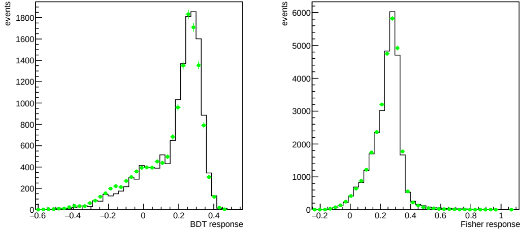
Figure 8.14: Distributions of the MVA classifier output for the two categories of events of the B_s^0 \rightarrow D_s^- \pi^+ decay. Data and simulation are shown in green and black, respectively. The simulation plots have been built by adding the different signal and background contributions taken from simulation and from data (combinatorial background only) according to the fitted yields. Each simulation plot has been reweighted to match the distributions of nTracks and nSPDHits between data and simulation.
