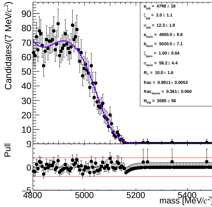
Figure A.3: Fit to the invariant mass distribution of the B_s^0 \rightarrow D_s^{*-} \rho^+ simulation sample.
