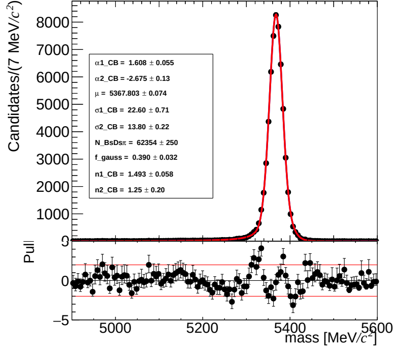
Figure A.1: Invariant-mass distribution of selected B_s^0 \rightarrow D_s^- \pi^+ decays from B_s^0 \rightarrow D_s^- \pi^+ simulation sample (data points) with the result of the best fit (red line) and the normalised residuals (pull).
