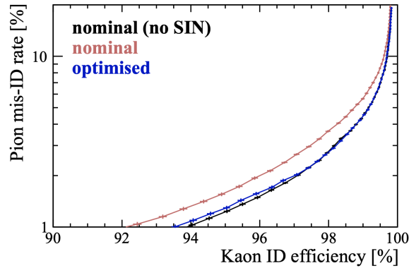
Figure 3.12: Probability to misidentify a pion as a kaon in function of the efficiency of identifying a kaon. In red the nominal scenario, in blue the optimised one obtained by considering the mitigation strategies and in black the nominal scenario obtained without considering the SIN contribution.
