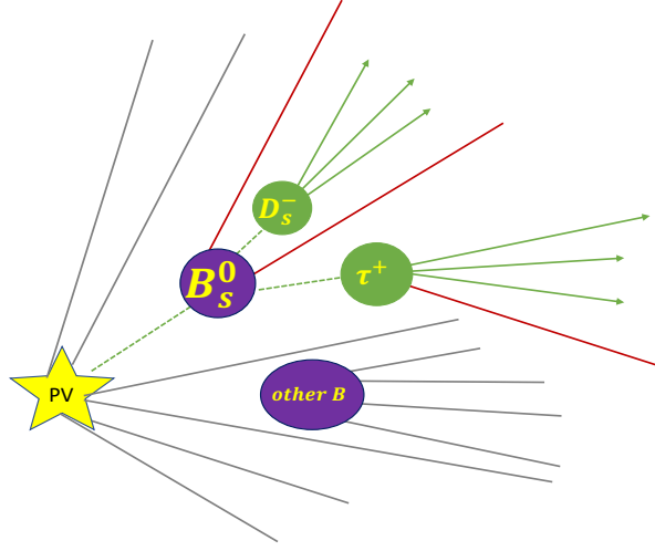
Figure 7.1: Schematic view of an event containing the signal decay. Isolated tracks are shown in grey, non-isolated tracks are represented in red and signal tracks are drawn in green.
