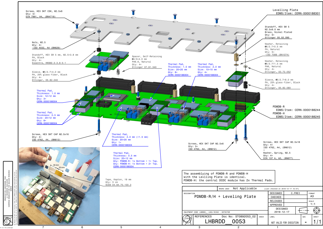
Figure 2.7: Leveling Plate scheme.
