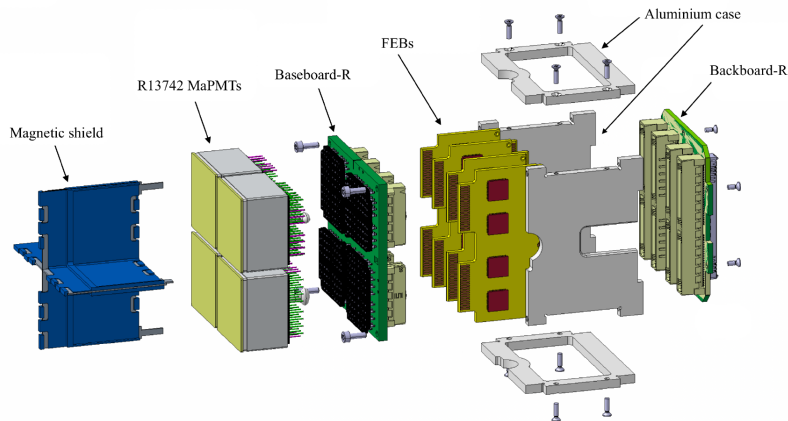
Figure 2.3: Schematic view of the R-type elementary cell.
