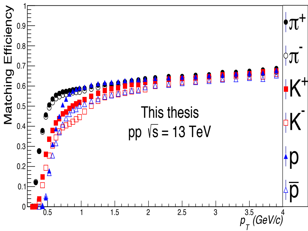
Fig. 3.19 p_T dependent matching efficiencies for pions, kaons and protons in MB (INEL>0) pp collisions at \sqrt{s} = 13 TeV.
