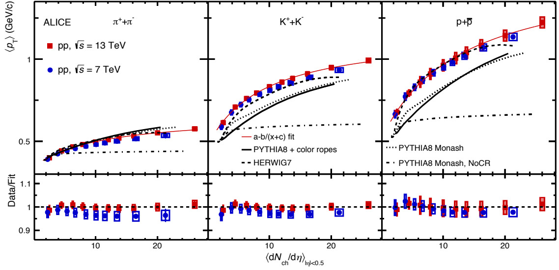
Fig. 6.3 (Upper panels) The \langle p_T \rangle of \pi , K and p as a function of multiplicity in pp collisions at \sqrt{s} = 13 TeV are compared with the results of lower energy pp collisions as well as with different MC event generators. The solid line represents the a - \frac{b}{\langle dN_{ch}/d\eta \rangle + c} fit of pp 13 TeV data. (Lower panels) The ratios of \langle p_T \rangle in different collisions energies to the fitted line.
