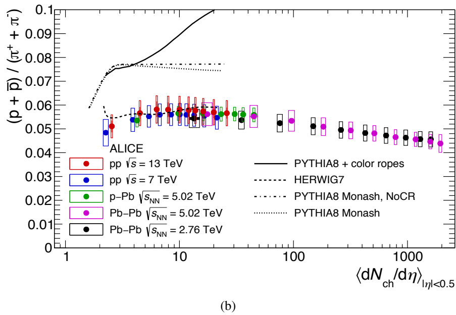
Fig. 4.14 p_T -integrated (a) K/\pi and (b) p/\pi yields ratios as a function of charged-particle multiplicity in pp collisions at \sqrt{s} = 13 TeV are compared with the results of the lower energy pp, p-Pb and Pb-Pb collisions. The prediction from different Monte Carlo event generators are also shown.
