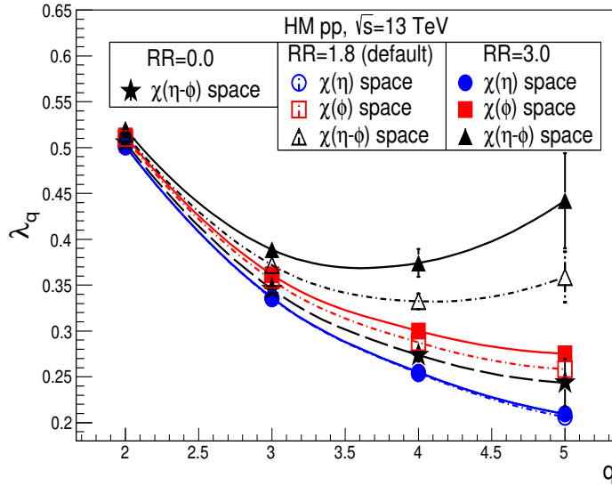
Fig. 6.10 Variation of \lambda_q against q for high multiplicity pp event at \sqrt{s} = 13 TeV for PYTHIA Monash generated data with RR = 0.0 in \chi(\eta - \phi) space and with RR = 1.8 and 3.0 in \chi(\eta) , \chi(\phi) and \chi(\eta - \phi) spaces.
