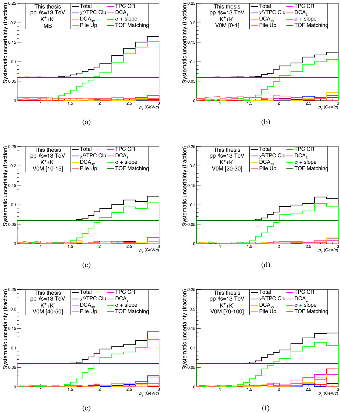
Fig. 3.37 Systematic uncertainty from different sources as well as the total uncertainties are shown for kaons in (a) MB, (b) 0-1%, (c) 10-15%, (d) 20-30%, (e) 40-50% and (f) 70-100% VOM multiplicity classes.
