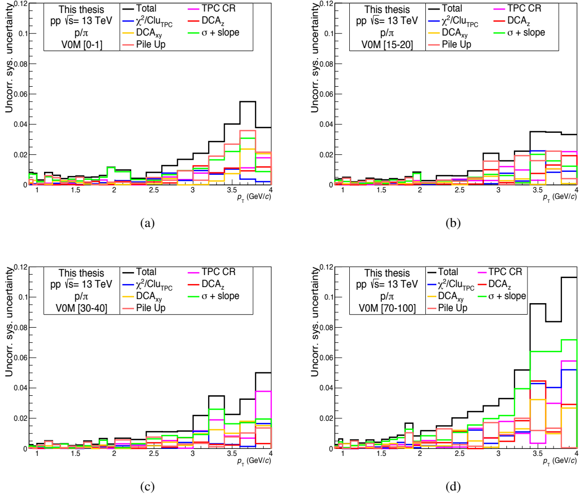
Fig. 3.45 Uncorrelated systematic uncertainty from different sources as well as the total uncertainties are shown for p/\pi ratio in (a) 0-1%, (b) 15-20%, (c) 30-40%, and (d) 70-100% V0M multiplicity classes.
