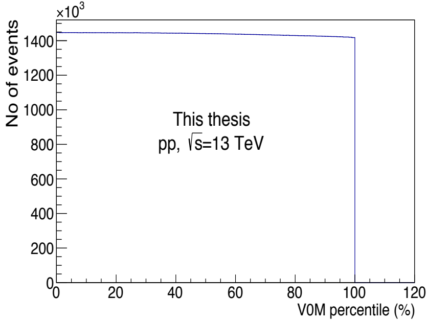
Fig. 3.4 Number of selected events as a function of VOM percentile after application of all the event selection cuts in pp collisions at \sqrt{s} = 13 TeV.
