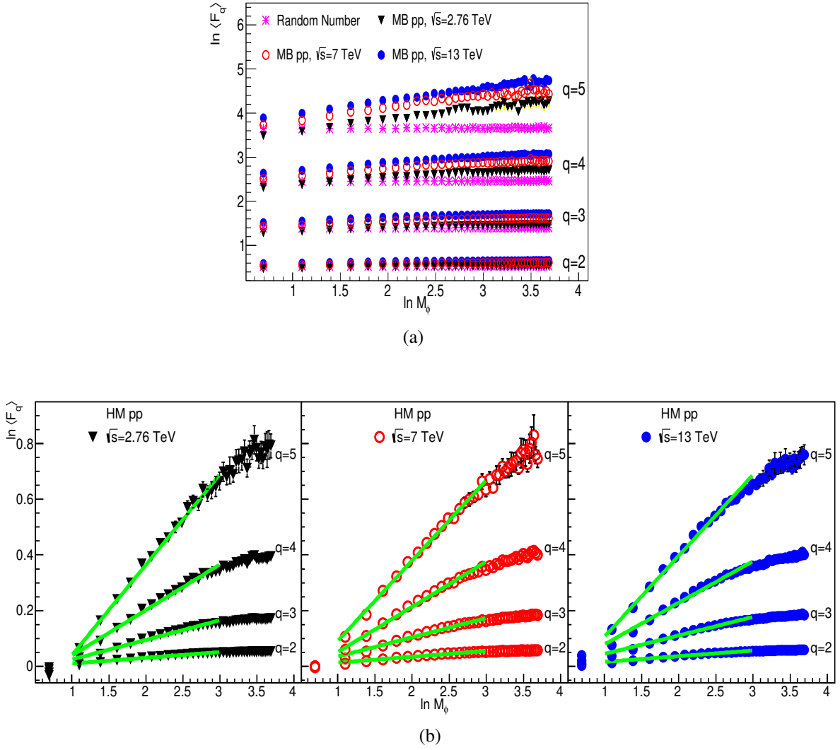
Fig. 5.6 \ln \langle F_q \rangle vs. \ln M plots for moments q = 2 - 5 for (a) RAN, MB pp collisions and (b) HM pp collisions at \sqrt{s} = 2.76, 7 and 13 TeV in one-dimensional \chi(\phi) space with PYTHIA Monash (default) generated data.
