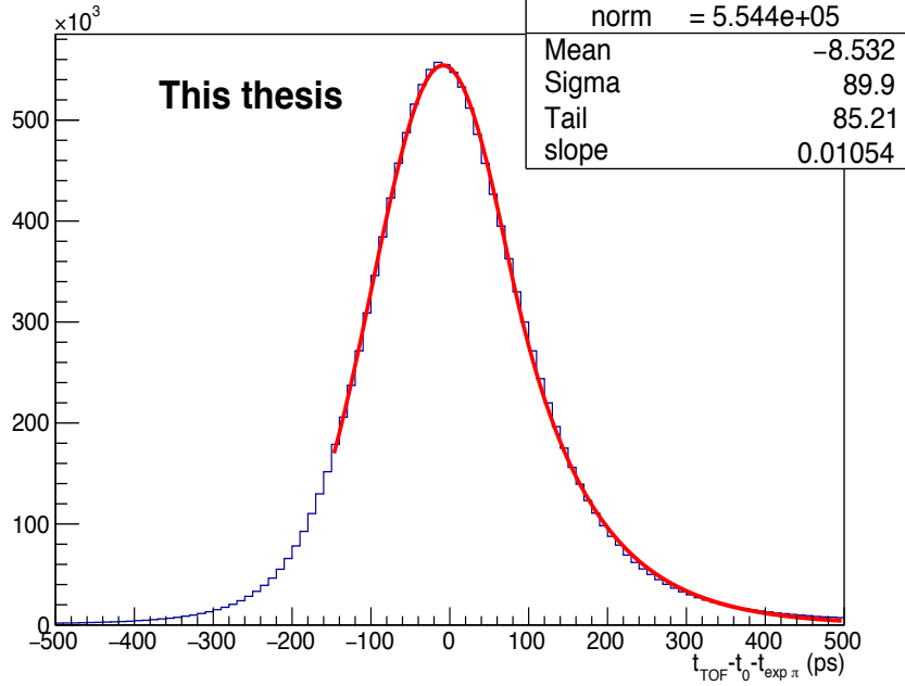
Fig. 3.10 The t_{TOF} - t_{ev} - t_{exp,\pi} distribution of all the tracks in the p_T range 0.9 to 1.1 GeV/c is fitted with the TOF signal function to have an idea about different parameters of the function.
