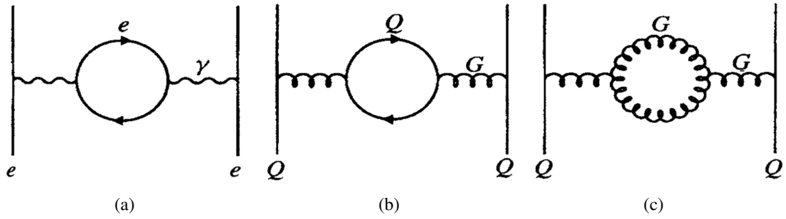
Fig. 1.4 The quantum vacuum polarisation which effectively changes the interactions strength. (a) In QED, the loop is shared by fermions only, (b) in QCD for a loop containing quarks and (c) in QCD for a gluon loop, involving gluon-gluon coupling, absent in QED [50].
