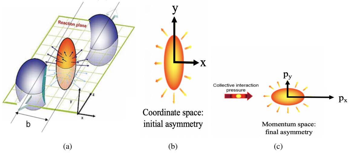
Fig. 1.15 (a) Schematic of the collisions overlapping zone between the incoming nuclei, (b) the initial-state anisotropy in the collisions zone that is finally converted into the final-state elliptic flow, and (c) the anisotropy in particle momentum space [99].
