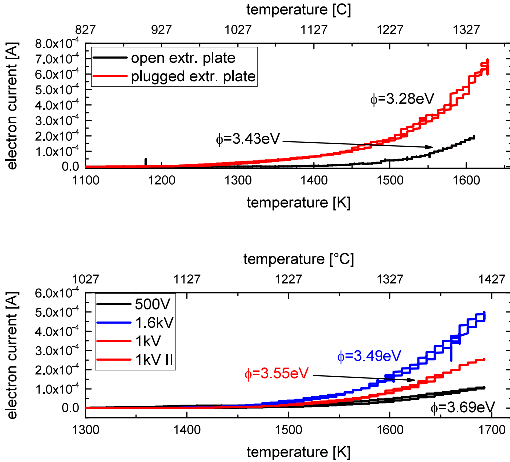
FIGURE 5.6: Electron emission of SrVO 3 acquired during a full heating and cooling cycle. Top: Electron emission of SrVO 3 at 500 V extraction potential with open (black) and plugged (red) pre-extraction plate before the use as ion source. Bottom: Electron emission with a plugged pre-extraction plate at 0.5 kV (black), 1 kV (red) and 1.6 kV (blue).
