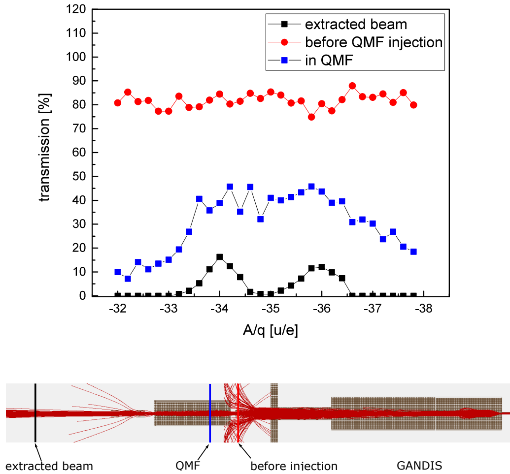
FIGURE 6.14: QMF transmission simulation. Top: Ion beam transmission before (red), in (blue) and after the last Einzel lens (black). Bottom: Trajectories of the ion beam with planes for transmission measurements indicated in red, blue and black, respectively.
