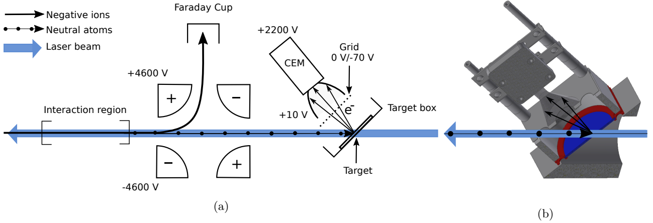
FIG. 1: a) A schematic drawing of the interaction region and the neutral particle detector. A negative ion beam, entering from the left in the figure, is merged with a counterpropagating laser beam in the interaction region. Afterwards, all ions are deflected by a quadrupole deflector into a Faraday cup. Neutralized particles from the photodetachment process impinge on the target where secondary electrons are generated and consequently detected by a CEM. The potential on the metal grid facing the CEM can be switched in order to repel or attract electrons. b) CAD-Drawing of the neutral particle detector with a clear view of the detector box housing the graphene target as well as the CEM entrance cone.
