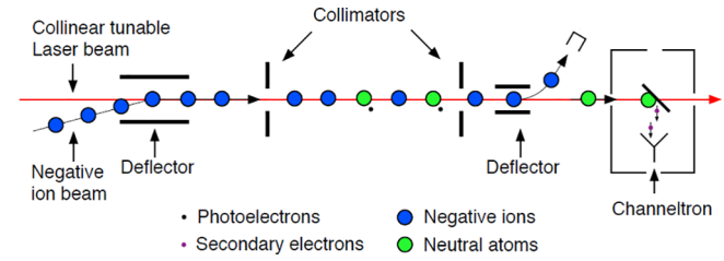
Fig. 1. Schematic depiction of the GANDALPH beamline. The incoming negative ions (blue) are merged with the laser beam (red arrow) by two electrostatic deflector plates. Neutral atoms produced in the photodetachment process (green) proceed straight into the neutral particle detector where they impinge on a target and create secondary electrons which are detected with a SEM. Residual negative ions are bent into a Faraday cup. (For interpretation of the references to colour in this figure legend, the reader is referred to the web version of this article.)
