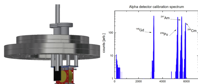
Fig. 5. Left: 3D model of the alpha detector mount. The alpha particles are implanted on the aluminium plate (black) which is then retracted from the beam path to the alpha particle detector (gold) held sandwiched between two mounting plates (red). The signal and voltage bias is delivered via an SMA feedthrough. Right: Calibration spectrum performed with a source containing Am, Gd, Pu and Cm. (For interpretation of the references to colour in this figure legend, the reader is referred to the web version of this article.)
