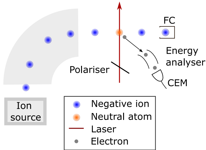
FIGURE 2.8: Photoelectron spectroscopy. A laser is intersected perpendicular with a negative ion beam. The detached electrons are guided into an electron energy analyser, residual negative ions are detected in a Faraday cup.
