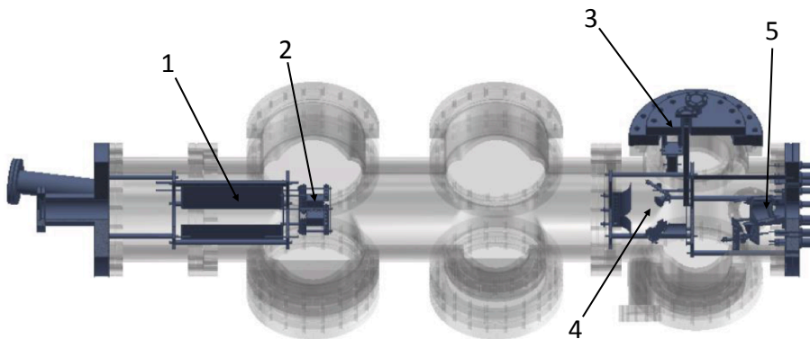
Fig. 2. CAD-model of the upgraded GANDALPH beamline. 1) Deflector plates to bend the incoming ions into the chamber. 2) Steering box with aperture. 3) Silicon detector: Neutral atoms are implanted onto a moveable plate which is then retracted in front of the detector. 4) Faraday cup and SEM for beam tuning and background measurements. 5) Neutral particle detector.
