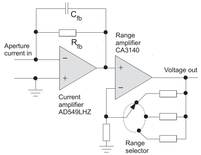
Fig. 3. The current-to-voltage amplifier is implemented by an ultra-low bias current op amp, succeeded by a conventional op amp for voltage amplification and range selection.
