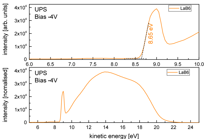
FIGURE 5.3: UPS spectrum of \text{LaB}_6 . Top: Zoom in of the onset region with extrapolated onset energy. Bottom: Complete spectrum. The kinetic energy of the electron at the onset subtracted by the bias voltage corresponds to the work function.
