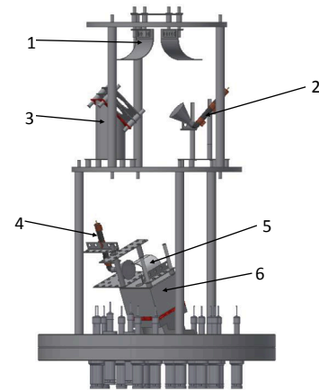
Fig. 4. 3D model of the neutral particle detector flange. 1) ion beam deflectors 2) secondary electron multiplier 3) Faraday cup 4) secondary electron multiplier 5) electron bend 6) neutral particle detector box with graphene coated glass plate. The detector was assembled using self-produced as well as Kimball-physcis eV parts [18].
