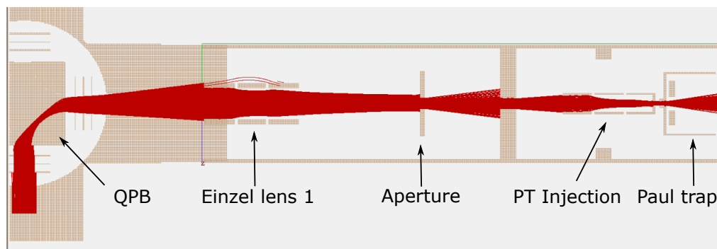
FIGURE 6.5: Simulation of Paul trap injection. Ions coming from the GANDIS beamline (bottom left) are bent by a quadrupole bend (QPB), where they are focussed into the Paul trap using an Einzel lens and additional injection optics.
