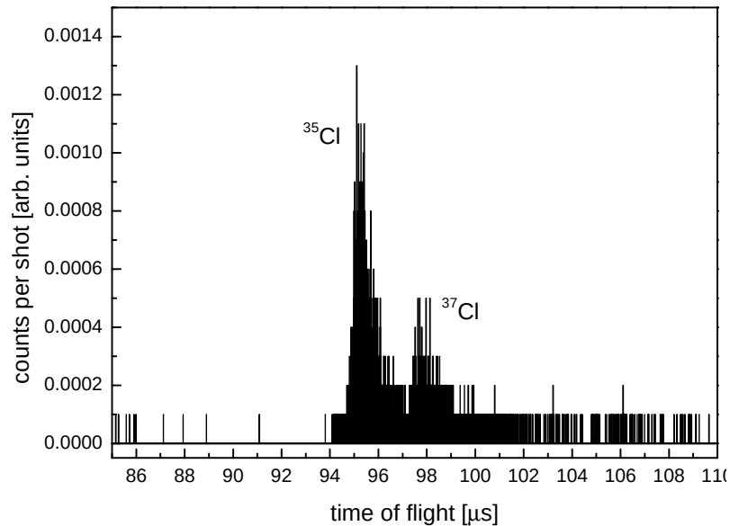
FIGURE 6.7: Time of flight spectrum of negative chlorine isotopes, ^{35}\text{Cl} and ^{37}\text{Cl} .
