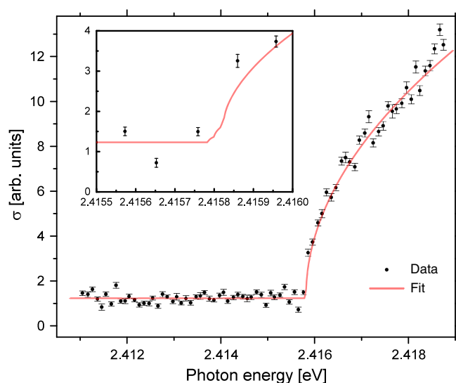
Fig. 3 Threshold scan of the photodetachment of astatine. The neutralization cross section is measured as a function of the photon energy. The data points are the experimental measurements with one standard deviation represented by error bars, and the solid line is a fit of Eq. (1). The onset corresponds to the EA of ^{211}\text{At} . The inset shows the region around threshold, where the different onsets in the fit function represent the detachment to the hyperfine levels of the groundstate of the neutral atom.
