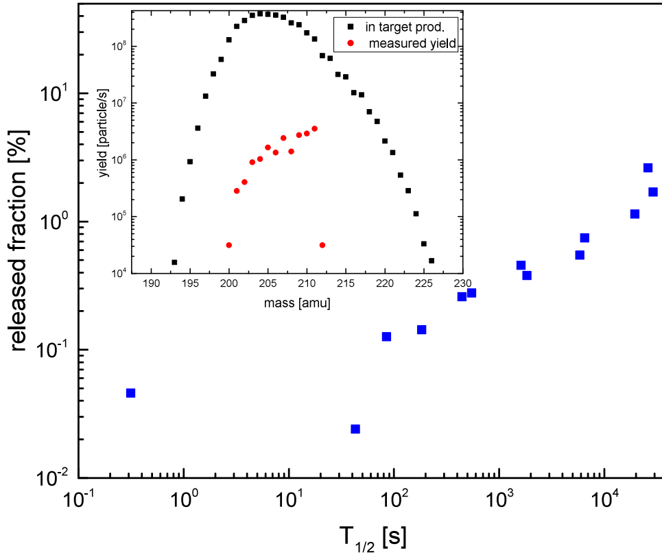
FIGURE 6.1: Fraction of measured particles per second compared to predicted in-target production as a function of the half-life of the respective isotope. Inset: Theoretical in target production yields predicted via FLUKA and extracted particles per second measured on a Faraday cup. Simulation values courtesy of J.P. Ramos.
