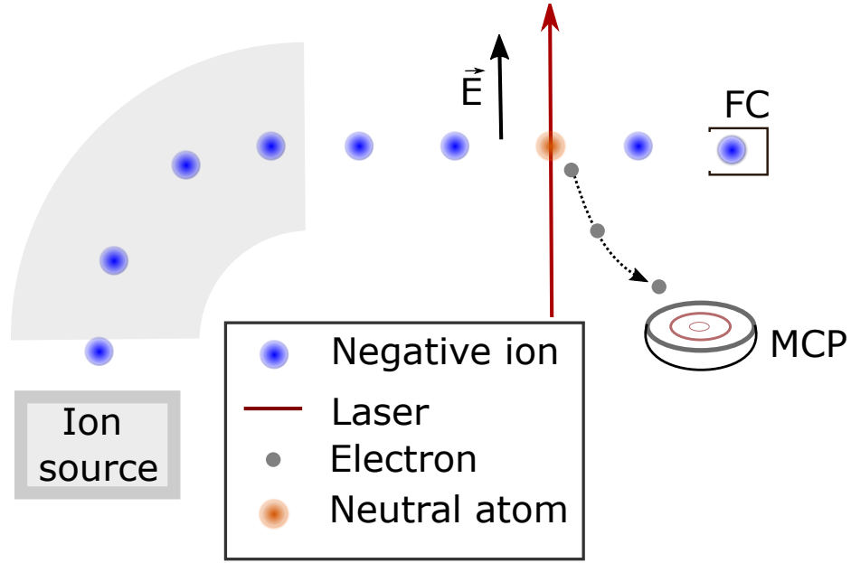
FIGURE 2.9: Schematic view of photodetachment microscopy. A detached electron is interfering with itself due to an static external electric field. The interference pattern can then be detected by a position sensitive detector such as a MCP.
