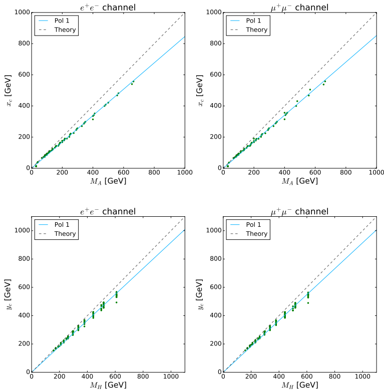
Figure 5.19. | Centroid coordinates well extracted from a Gaussian fit of the reconstructed mass distributions as a function of the mass hypothesis m_A (upper) and m_H (lower). The blue line represents the best-fit function, while the dashed line represents the theoretical scenario, where x_c = m_A and y_c = m_H .
