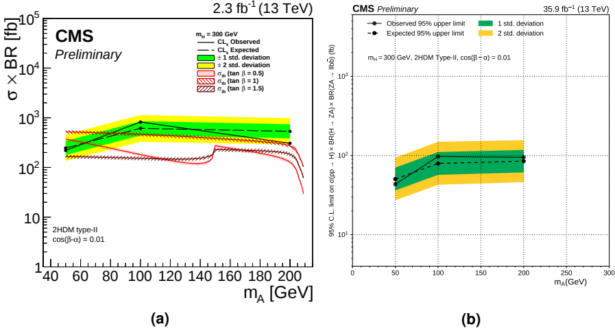
Figure 5.38. | Expected and observed 95% CL upper limits on the product of the signal production cross section and branching ratio \text{BR}(H \rightarrow ZA) \times \text{BR}(A \rightarrow b\bar{b}) \times \text{BR}(Z \rightarrow \ell^+ \ell^-) for three representative mass hypotheses m_H = 300 \text{ GeV} and m_A = 50, 100, 200 \text{ GeV} from the search at \mathcal{L} = 2.3 \text{ fb}^{-1} (a) and \mathcal{L} = 35.9 \text{ fb}^{-1} (b) [4].
