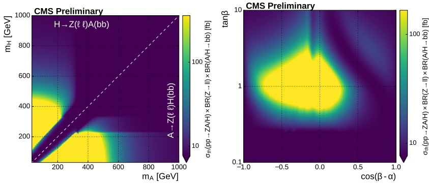
Figure 5.3. | Product of the theoretical cross section and branching ratio \text{BR}(H/A \rightarrow ZA/H) \times \text{BR}(Z \rightarrow e\bar{e}/\mu\bar{\mu}) \times \text{BR}(A/H \rightarrow b\bar{b}) in the m_A vs. m_H parameter space for \tan\beta = 1.5 and \cos(\beta - \alpha) = 0.01 (left) and in the \cos(\beta - \alpha) vs. \tan\beta parameter space for m_H = 379 GeV and m_A = 172 GeV (right).
