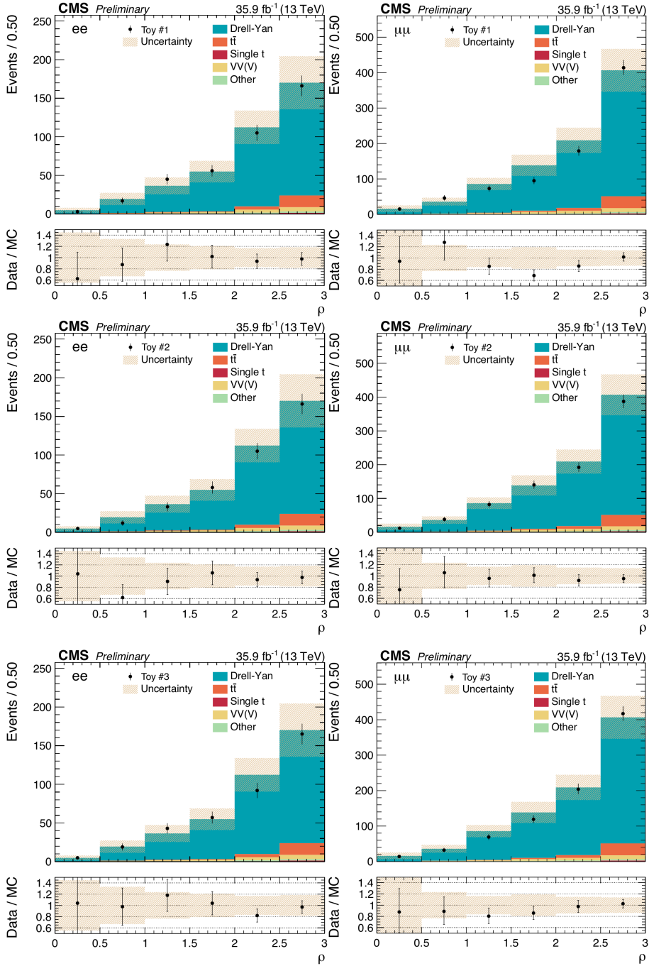
Figure 5.35. Final templates with background toys instead of the real data. The rows show histograms with three different toys, while the columns show the ee and \mu\mu channels. All histograms are relative to the mass point (m_H, m_A) = (652, 64) GeV.
