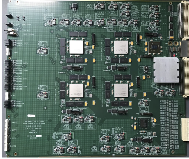
Figure 3.9: Picture of a FTK Second Stage Board. This board is responsible of the second-stage processing of the candidate FTK tracks.
