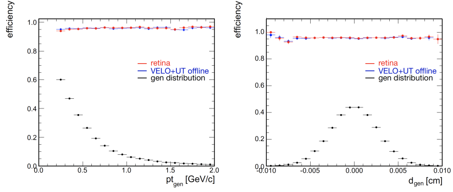
Figure 2.13: Tracking reconstruction efficiency of the retina algorithm (in red) and of the offline VELO+UT algorithm (in blue), as function of p_T and d . The distribution of the considered parameter is, also, reported in black. Luminosity of L = 3 \times 10^{33} \text{ cm}^{-2} \text{ s}^{-1} .
