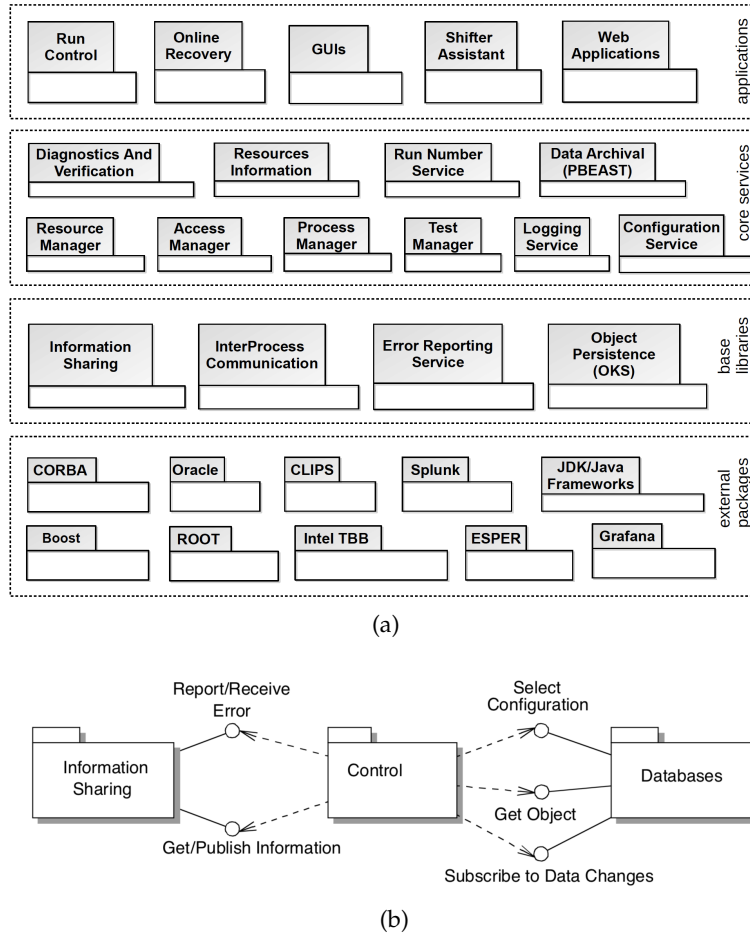
Figure 5.2: (a) Control and Configuration software: high-level architecture. (b) Internal interaction between the Online Software packages.
