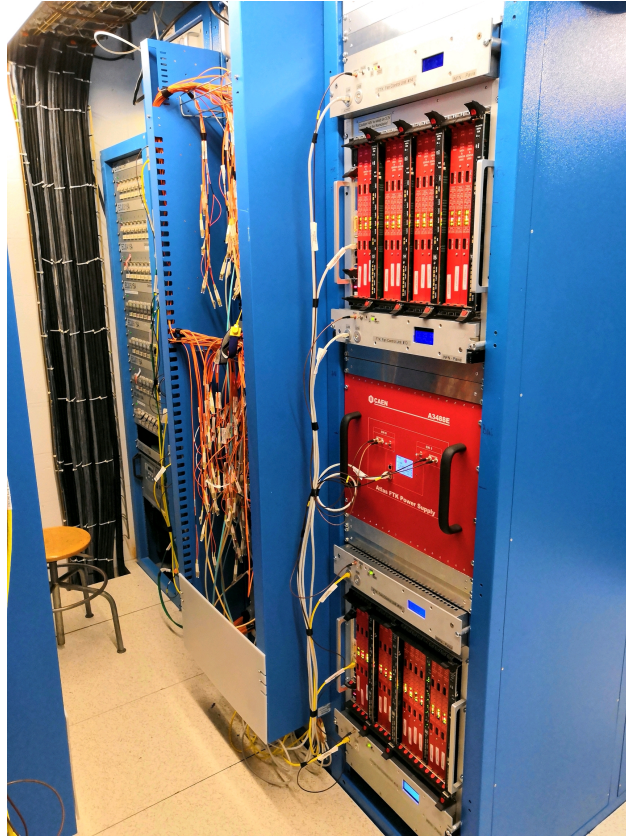
Figure 3.13: Picture of a full VME rack. In the photo the two VME crates are visible, together with the FTK Power Supply (PS), the red box, providing the required power to the crates and to the fan trays, and the 4 custom fan trays (the metallic boxes with the small LCD screen on their right).
