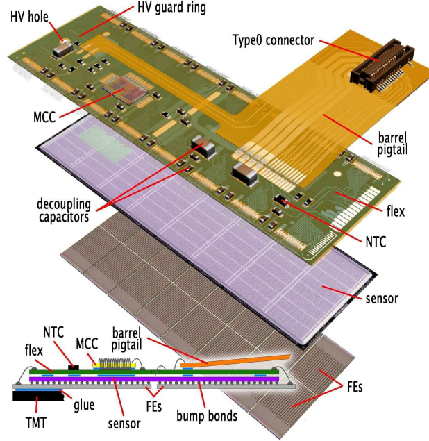
Figure 1.12: Pixel module structure of the ATLAS tracker.
