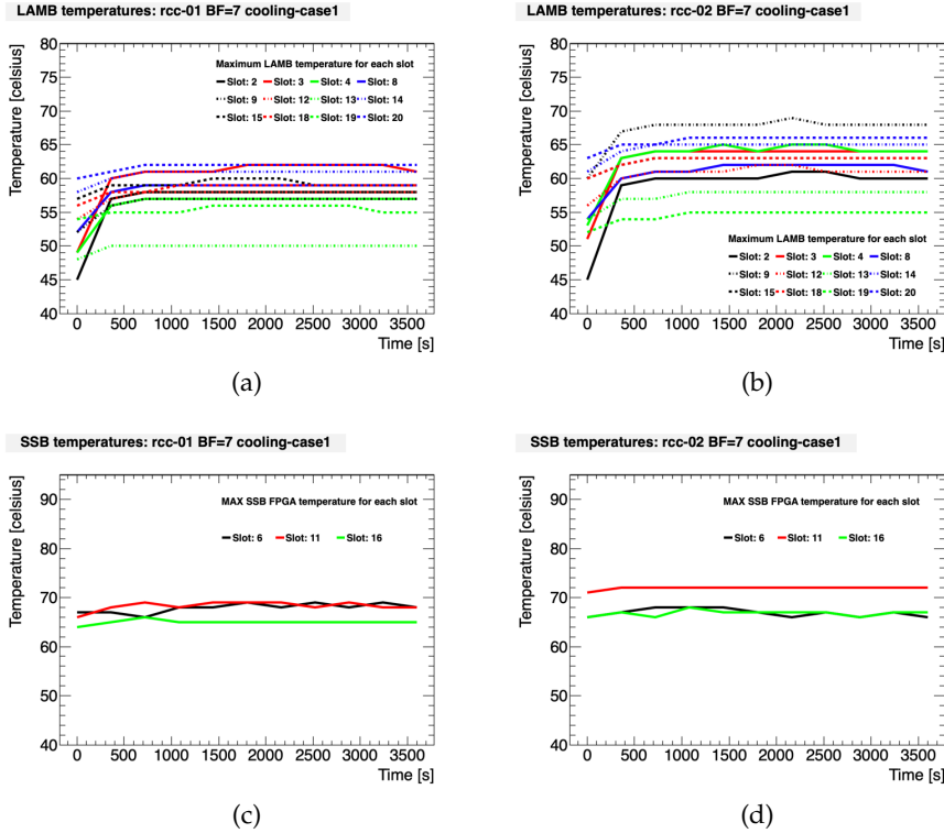
Figure 4.21: Profile of the maximum LAMB temperatures (a),(b) and of the maximum SSB FPGA temperatures (c),(d) for the BF 7 AMB configuration. In this tests only 12 PUs and 3 SSBs where housed in each VME crate.
