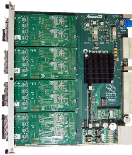
Figure 3.3: Picture of a FTK DF board. The 4 different Input Mezzanines (cards number 3, 6, 7, and 8) are also visible. This board, together with the IMs, is responsible for the reorganization and formatting of the ID data for the FTK processing.
