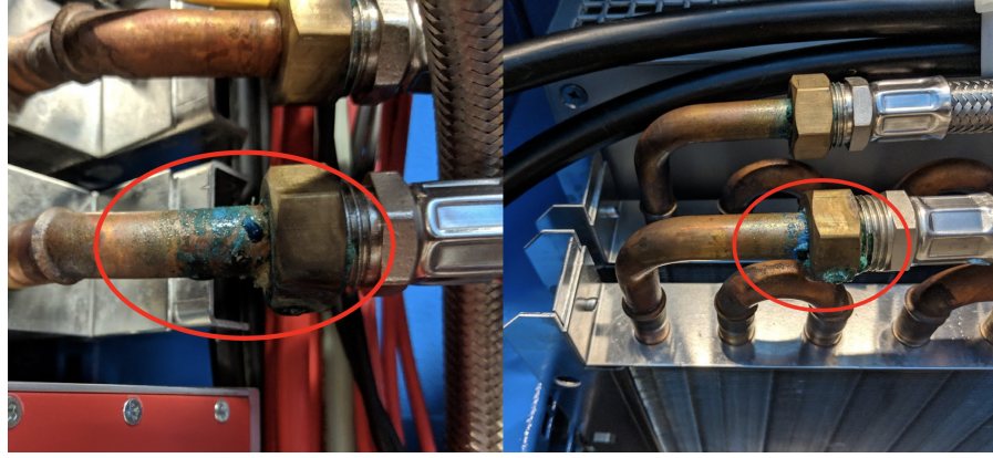
Figure 4.17: The Figure shows an example of the formation of dew happened inside the testing FTK rack during the execution of the chiller configuration cooling test. The pipes visible in the figure are the ones bringing the water in input to the heat exchangers.
