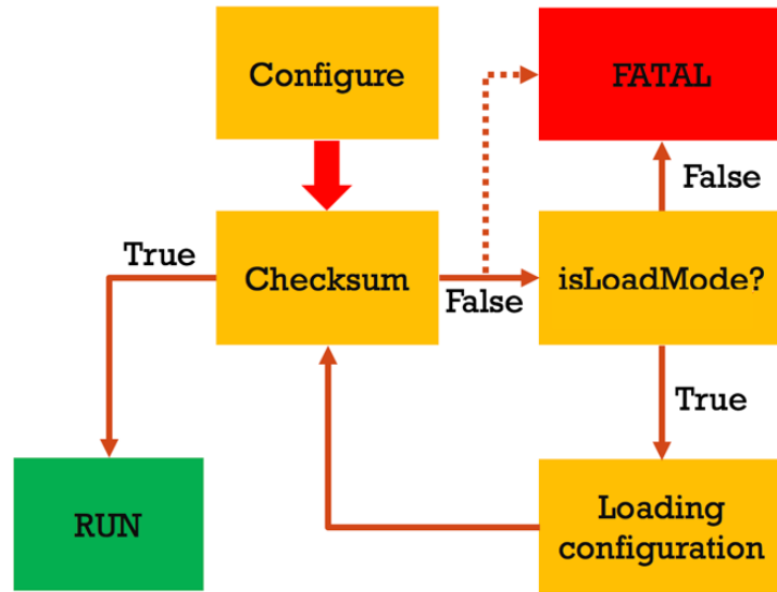
Figure 5.7: FTK configuration loading logic. The loading of the configuration on the boards is performed only during a "configuration run" identified via the isLoadMode flag.
