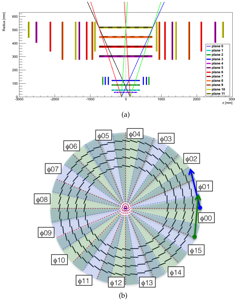
Figure 3.4: (a) The assignment of barrel layers and end-cap disks to FTK logical layers. Layers 0-3 are pixels, the rest are SCT. The division into 4 \eta regions with the appropriate overlap is indicated by the thin colored lines: two endcap regions, one to the left of the black line and the other to the right of the blue line; and two barrel regions, one between the red lines and the other between the green lines.
