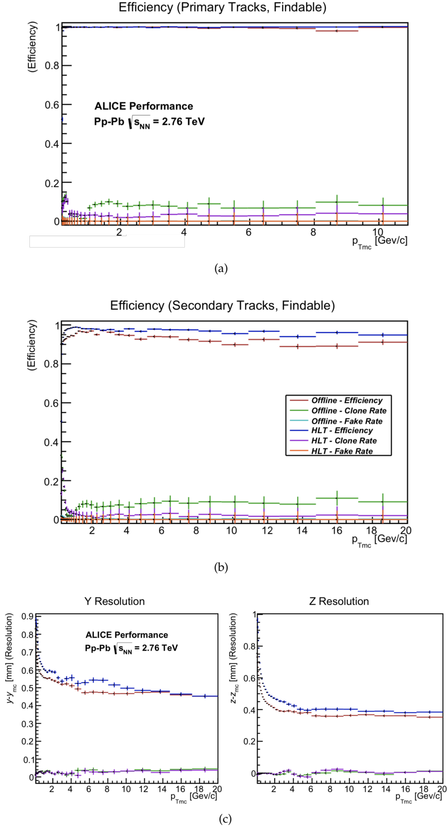
Figure 2.10: Resolution and efficiency of ALICE online and offline tracking for TPC data only [40].
