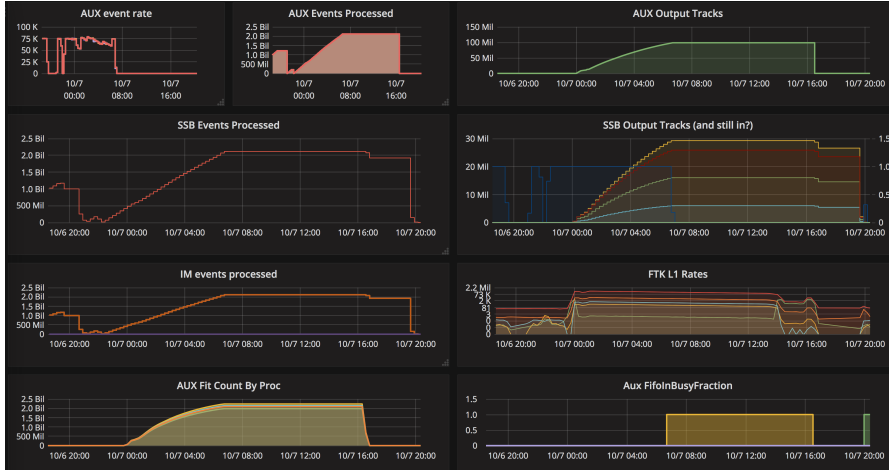
Figure 5.14: Example of high level monitoring of board data-flow variables for FTK (Grafana dashboard)
