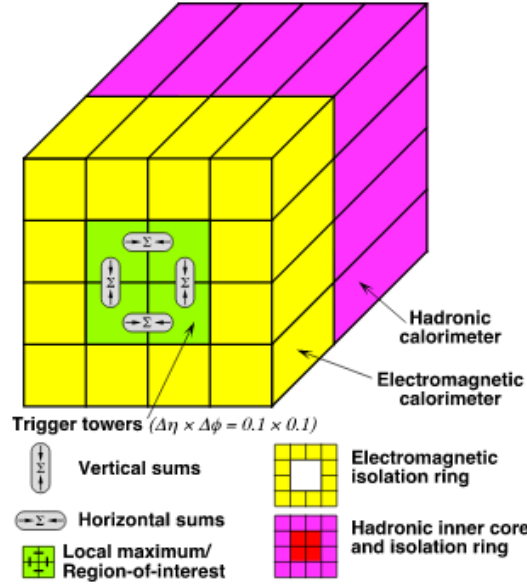
Figure 1.28: Schematic view of the trigger towers used as input to the L1Calo trigger algorithms.
