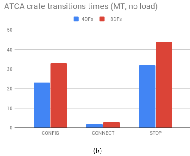
Figure 5.10: Measured transition times for one VME crate (a) and one ATCA shelf (b). Only the transitions with execution times greater than 1 s are shown. The crate (shelf) configurations of 8+2 (4) and 16+4 (8) boards are shown. All the measured FTK transition times are smaller than the ATLAS ones.
