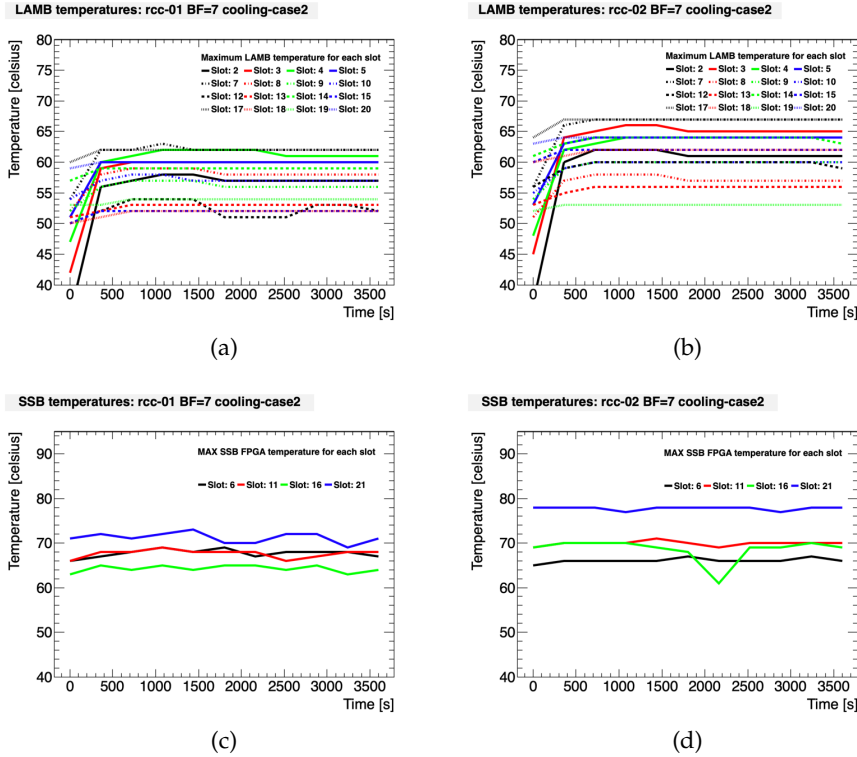
Figure 4.16: Profile of the maximum LAMB temperatures (a),(b) and of the maximum SSB FPGA temperatures (c),(d) for the BF 7 AMB configuration. The test was executed with an increased water flux of the FTK cooling system of 5 bar.
