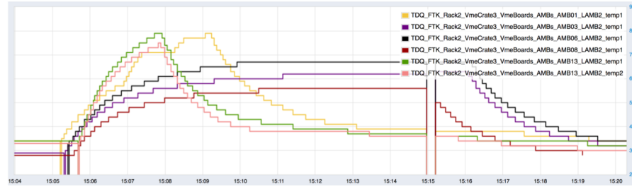
Figure 4.3: Temperature profile of some of the LAMBs during a cooling test. In the test, 16 AMB were running in high power conditions. In this test, the FW temperature protection of two of the LAMBs used has been triggered. From the plot it is possible to see the quick increase of the temperatures of the LAMB 2 (AMB 13 and AMB 1), followed by a quick decrease due to the stop of the dataflow triggered by the AMB FW protection. The protection threshold is set to 80 °C. All the other LAMBs were instead running stably at about 70 °C.
