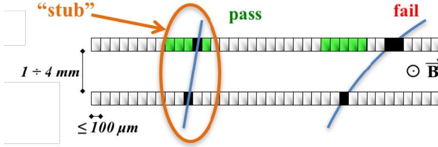
Figure 2.14: Sketch of the p_T modules that will be part of the new Outer Tracker for the upgrade of the CMS Inner Detector. The correlation of the two signals in the sensors allows the rejection of low- p_T tracks using the selection window represented in green.
