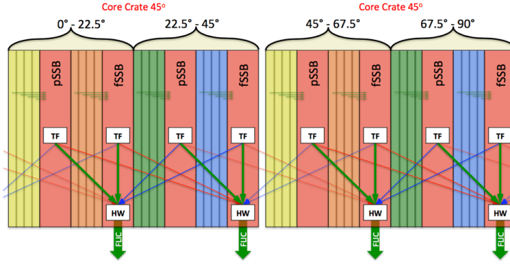
Figure 3.10: Sketch of the inter-module connections between the SSB Track Fitter and Hit Warrior, used for the duplicate removal procedure. Each SSB is connected to 5 other SSBs, and every fSSB has a connection to the FLIC.
