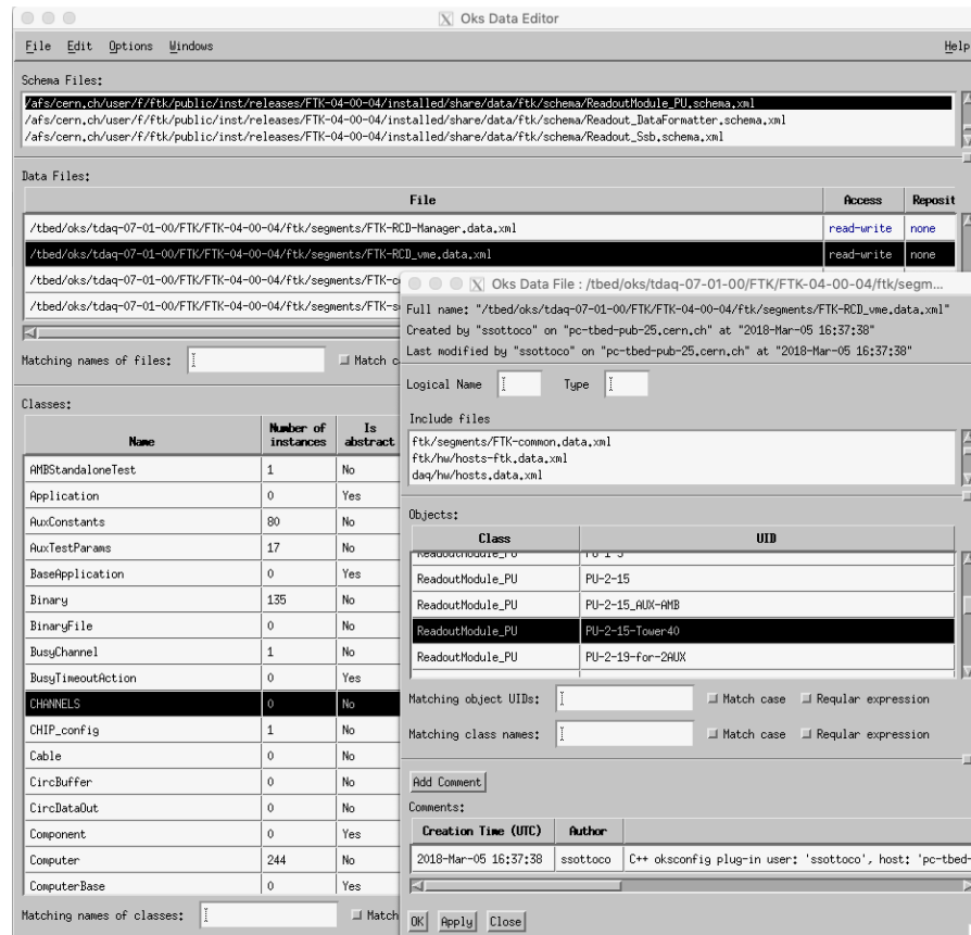
Figure 5.6: Example view of the OKS Data Editor tool for the configuration management of the OKS data files. In this example, the different PU RMs contained in the one of the VME RCD can be seen.
