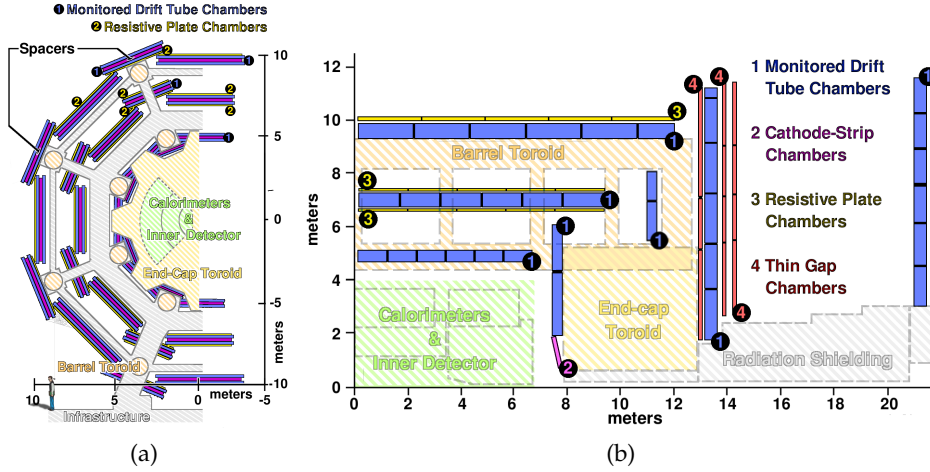
Figure 1.23: (a) Cross-sections of the barrel muon system perpendicular to the beam axis (non-bending plane) and (b) in a plane containing the beam axis (bending plane).
