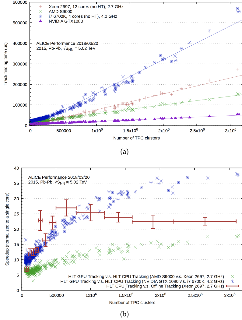
Figure 2.9: (a) Run time of the ALICE HLT TPC Tracking algorithm on CPU and GPU as a function of the event size. This plot shows that the tracking duration is almost linear both on CPU and GPU, irrespectively of the processor model. (b) Speedup of the ALICE TPC tracking on GPU normalized to a single CPU core.
