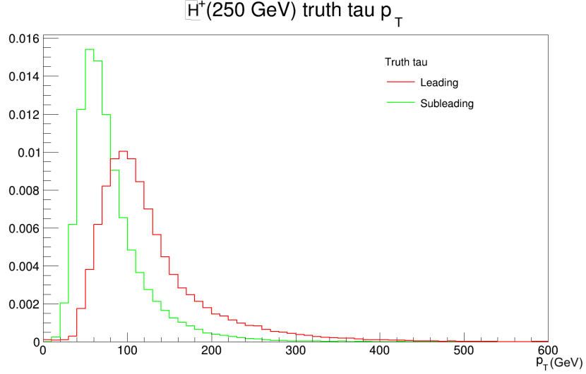
Figure 6.21: Distribution of the truth leading and subleading taus p_T for samples of simulated H^+ \rightarrow \tau_{\text{had}} \nu events, with an H^+ of mass 250 GeV.
