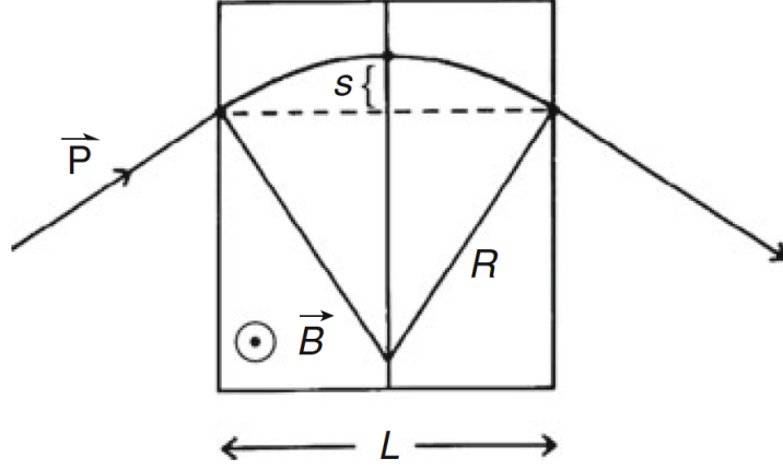
Figure 1.22: Sagitta measurement in magnetic spectrometer.
