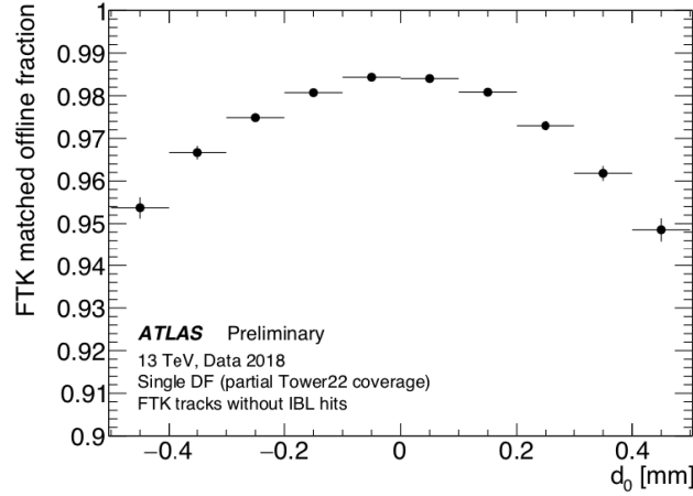
Figure 3.21: Fraction of FTK tracks matched to selected offline tracks, as a function of the FTK track transverse impact parameter d_0 , from the FTK SliceA (FTK tower 22).
