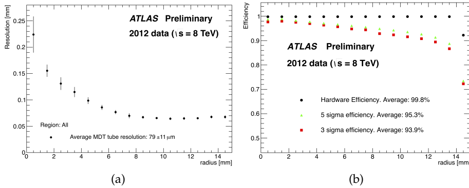
Figure 1.25: (a) MDT tube resolution versus radius (distance of the particle trajectory from the wire) for all MDT chambers. The error bar is a combination of systematics and statistical errors. The tube resolution is derived from the segment track residual distributions for corresponding radius range, and the average is the result of the whole radius range. (b) MDT tube efficiency versus radius of all MDT chambers.
