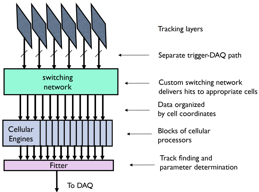
Figure 2.11: TPU architecture overview.
