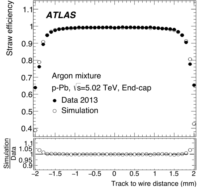
Figure 1.16: Straw efficiency in the end-cap wheels filled with an Ar-based mixture versus track-to-wire distance in the data (solid circles) and simulation (open circles).
