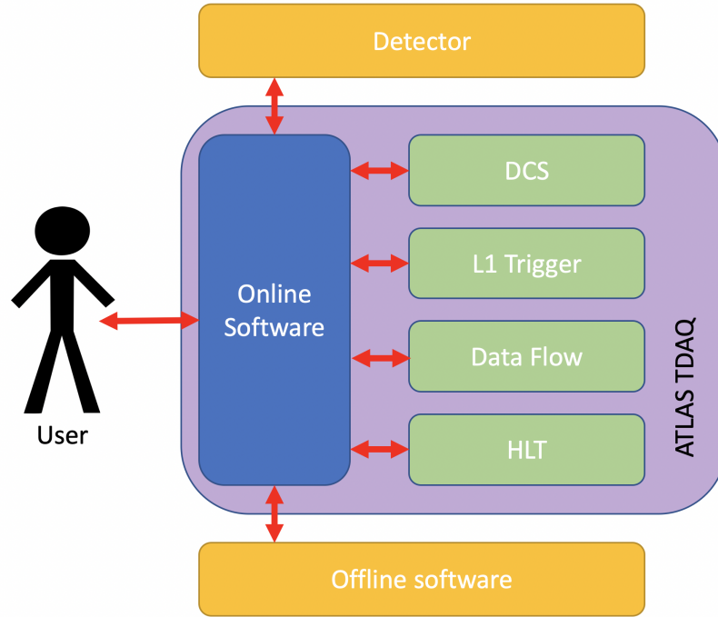
Figure 5.1: Context diagram of the ATLAS online software.
