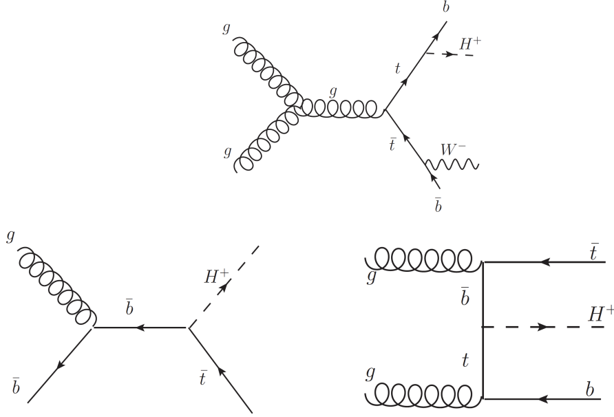
Figure 6.1: Example of leading-order Feynman diagrams for the production of a charged Higgs boson through top-quark decay (upper picture), 5FS production (left picture) and 4FS production (right picture).
