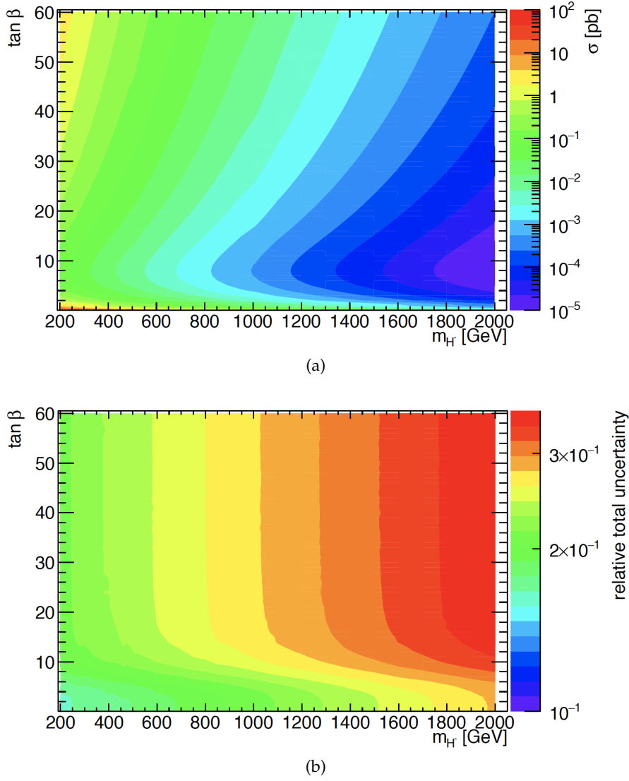
Figure 6.3: Two-dimensional plot of the charged Higgs boson production cross section (a) and average relative uncertainty (b) as a function of \tan \beta and m_{H^\pm} values in the 4FS of the 2DHM [88].
