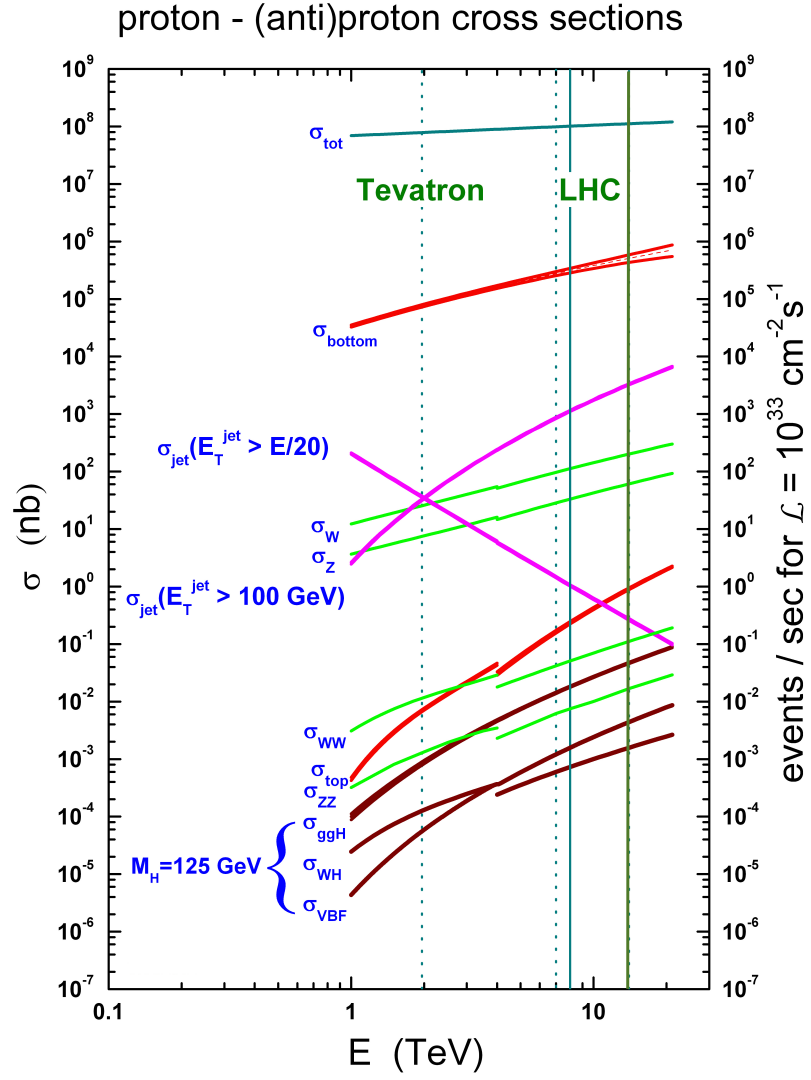
Figure 1.5: Various Standard Model cross-sections at the Tevatron and LHC colliders as function of the centre-of-mass energy ( \sqrt{s} ).
