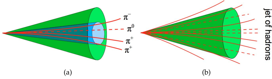
Figure 6.5: (a) Sketch of a three-prong \tau decay. The decay products clustered in a narrow cone (in blue). (b) Sketch of a jet of hadrons. The particles are distributed throughout a large cone.
