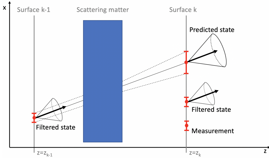
Figure 2.3: Schematic representation of the KF two-steps process. Starting from the filtered state on the surface k - 1 , the application of the prediction step provides the predicted state on surface k . Finally, the filtering step updates this state with the measurements information available, providing the final filtered state on surface k .
