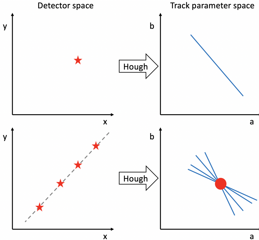
Figure 2.2: Sketch of the Hough transformation principle.
