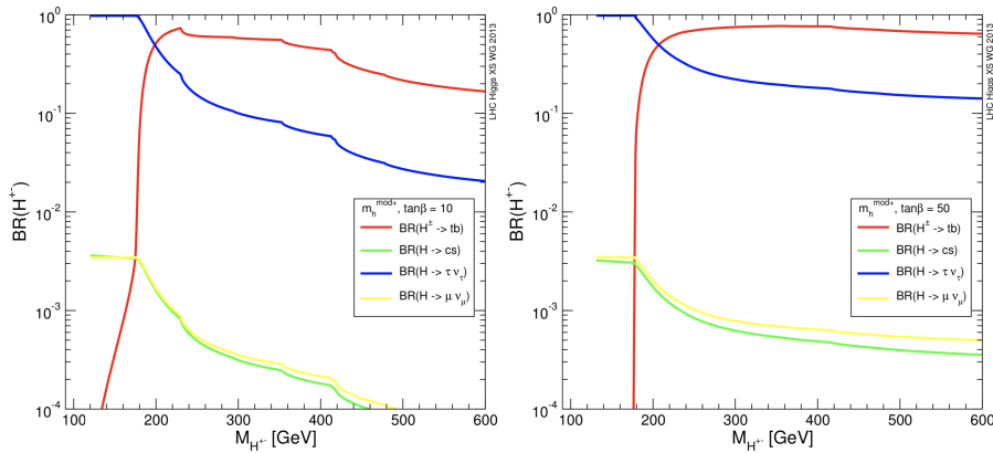
Figure 6.4: Branching fractions of the charged Higgs boson as a function of m_{H^\pm} , for \tan \beta values of 10 (left) and 50 (right).
