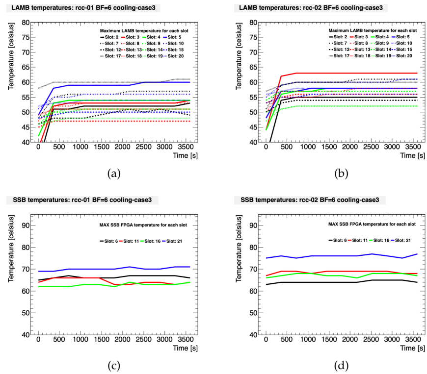
Figure 4.18: Profile of the maximum LAMB temperatures (a),(b) and of the maximum SSB FPGA temperatures (c),(d) for the BF 6 AMB configuration. The test was executed after enabling the water chiller.
