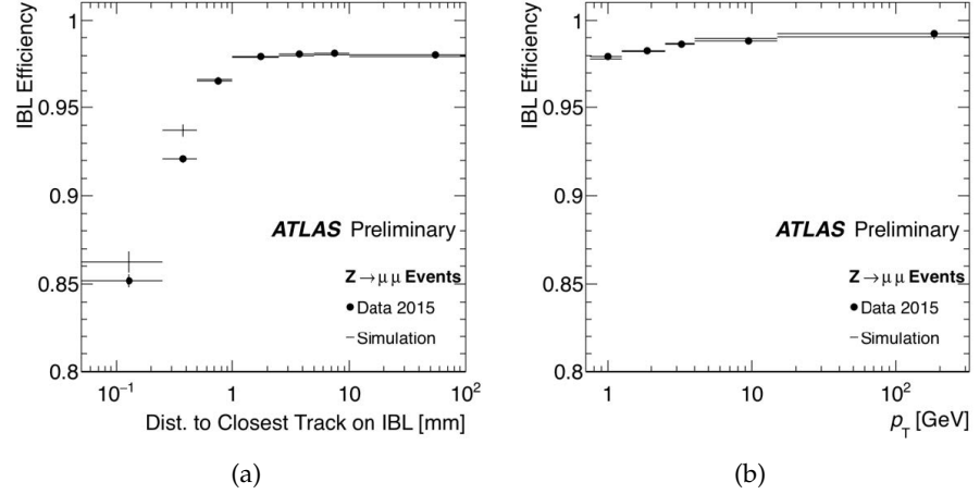
Figure 1.14: Efficiency of associating an IBL hit to a reconstructed particle track as a function of the tracks distance to the closest track on the IBL module (a) and the particle p_T (b) for selected Z \rightarrow \mu\mu events in collision data (circles with error bars) and simulation (lines). The efficiency is computed as the fraction of selected tracks with p_T > 0.7 GeV and |\eta| < 2.5 having an associated IBL cluster. Disabled and unstable IBL modules have been removed.
