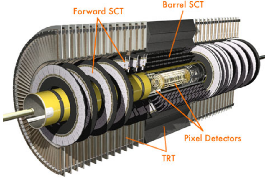
Figure 1.10: Schematic view of the layout of the Inner Detector of ATLAS. The IBL layer, at a radius of 33.25 mm, is not depicted.
