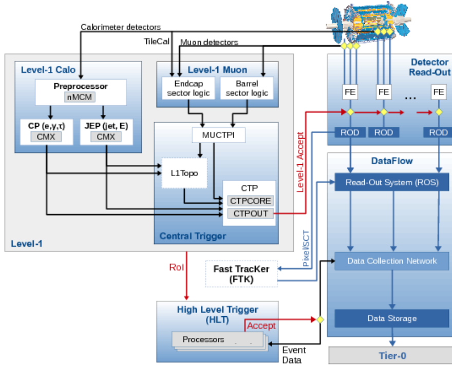
Figure 1.27: Schematic layout of the ATLAS trigger and data acquisition system.
