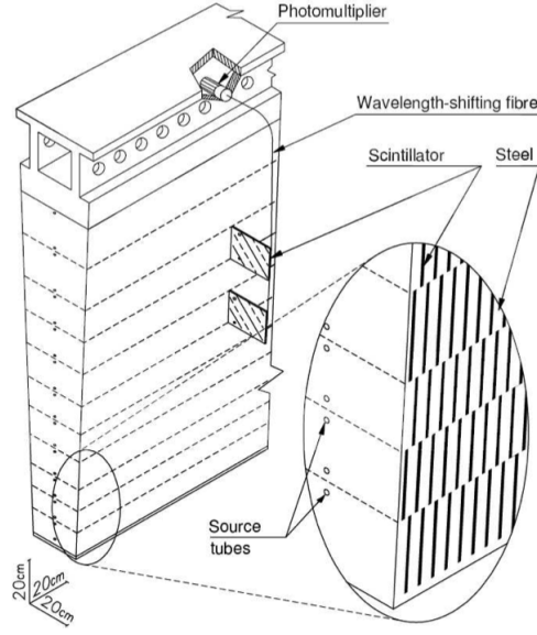
Figure 1.20: Diagram of a TileCal module.
