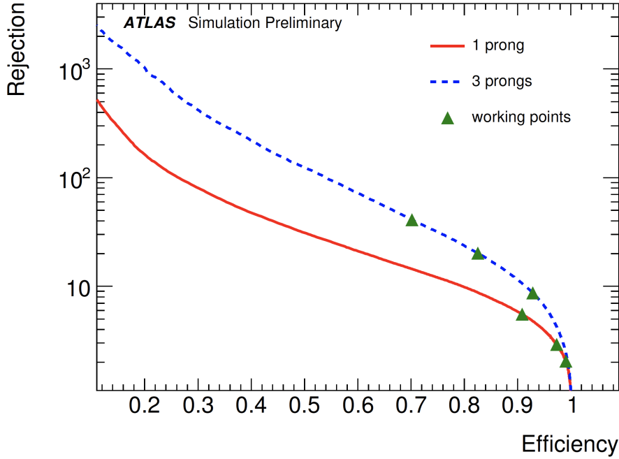
Figure 6.10: Performance of the BDT algorithm in terms of background rejection as a function of the signal efficiency for 1-prong and 3-prong \tau candidates reconstructed offline as 1-prong and 3-prong \tau and passing the HLT p_T and track multiplicity requirements. The working points correspond to the tight , medium and loose identification criteria in order of decreasing background rejection.
