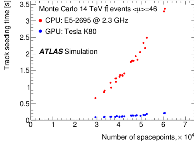
Figure 2.6: Timing of the ATLAS ID track seeding algorithm for the full detector. The red dots represent the standard HLT ID algorithm, running on a single CPU core, the blue dots show the same logic algorithm ported to GPU. The timing is shown as a function of the number of space points in an event.
