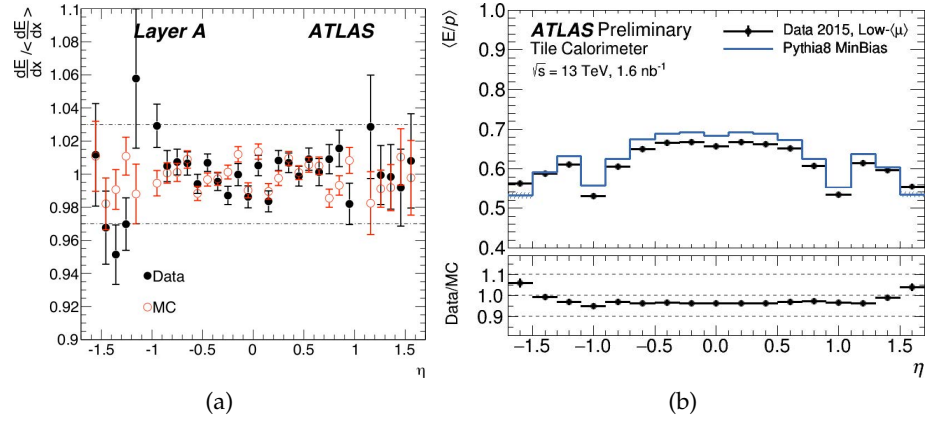
Figure 1.21: (a) Uniformity of the cell response to cosmic muons expressed in terms of the normalised truncated mean of dE/dx , as a function of \eta for radial layer A. (b) Energy over momentum E/p as a function of \eta for isolated hadron track using 2015 data.
