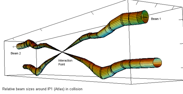
Figure 1.4: Intersection of the two LHC beams. The accelerated beams have transverse dimensions of the order of a few mm, and when they approach the collision point, they get squeezed to approximately 16\text{ }\mu\text{m} .
