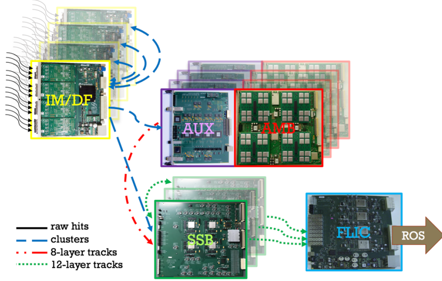
Figure 3.1: Sketch of the internal architecture of FTK. The lines represent the communication links between different boards [50].
