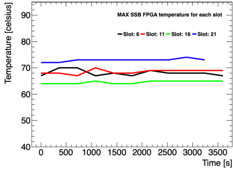
SSB temperatures: rcc-01 BF=6 cooling-case1
