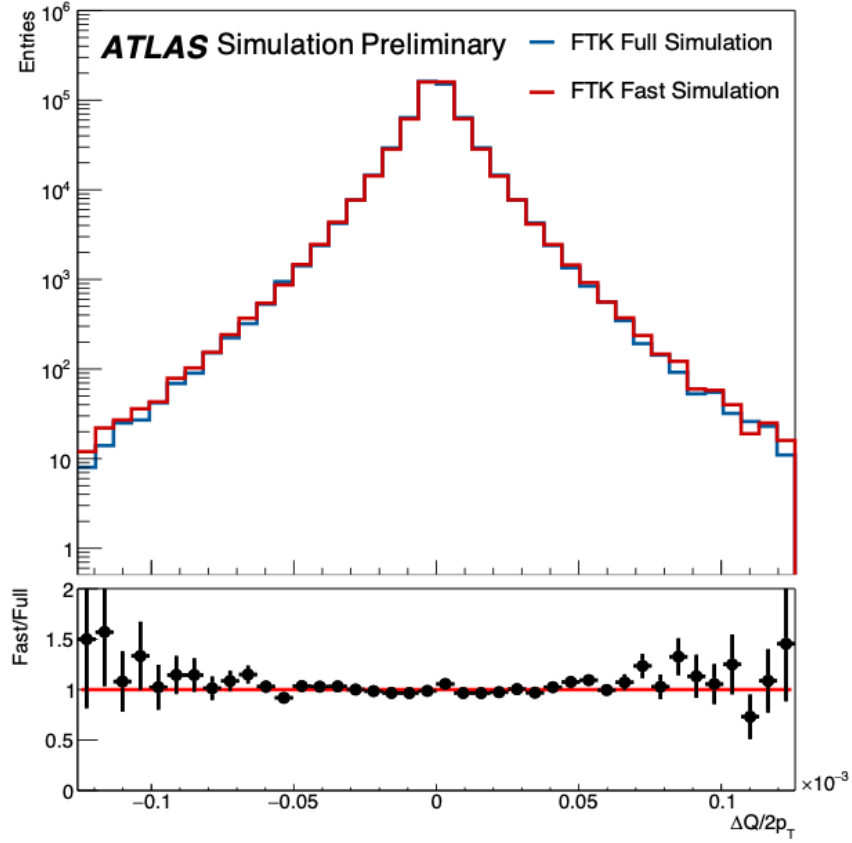
Figure 3.16: The resolution of the FTK track curvature, from functional emulation of FTK using FTKSim (FTK Full Simulation) and a parameterized uncertainty model (FTK Fast Simulation). The difference between the FTK reconstructed and true values of track charge ( \Delta Q ) divided by twice the track transverse momentum is plotted. A fully simulated sample of muons with longitudinal impact parameter |z_0| < 110 cm and pseudo-rapidity |\eta| < 2.5 is used. The resolution for the fast simulation is modeled as a double gaussian derived from full simulation.
