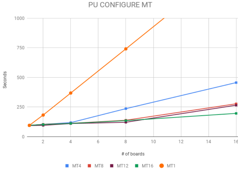
Figure 5.9: Transition times of the PU configure transition as a function of the number of enabled boards, for different values of the maximum number of thread spawned.
