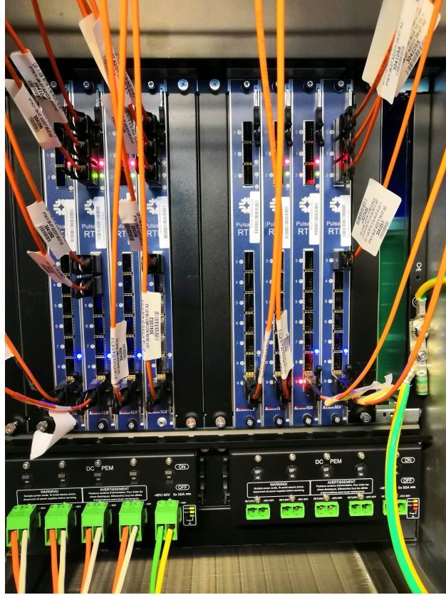
Figure 3.11: Picture of one of the FTK DF shelves in its final configuration. The shelf contains 8 DF boards and 64 IM cards. At the moment in which the picture was taken, not all the DFs were fully cabled.
