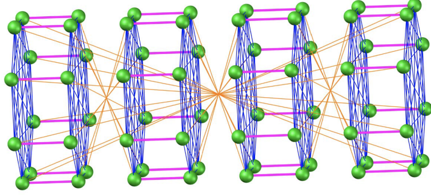
Figure 3.5: The interconnections for data sharing among the 64 \eta - \phi towers within 4 DF crates. A green ball represents one FTK tower. Blue lines represent data sharing between the upper FPGAs or lower FPGAs in a shelf. The red lines represent data sharing between an upper and a lower FPGA, and the yellow lines represent inter-shelf data sharing.
