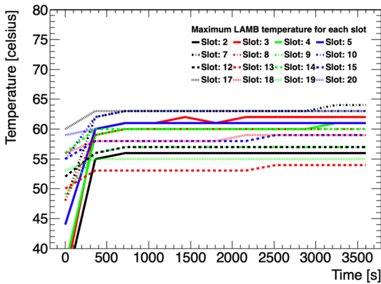
LAMB temperatures: rcc-02 BF=6 cooling-case1
