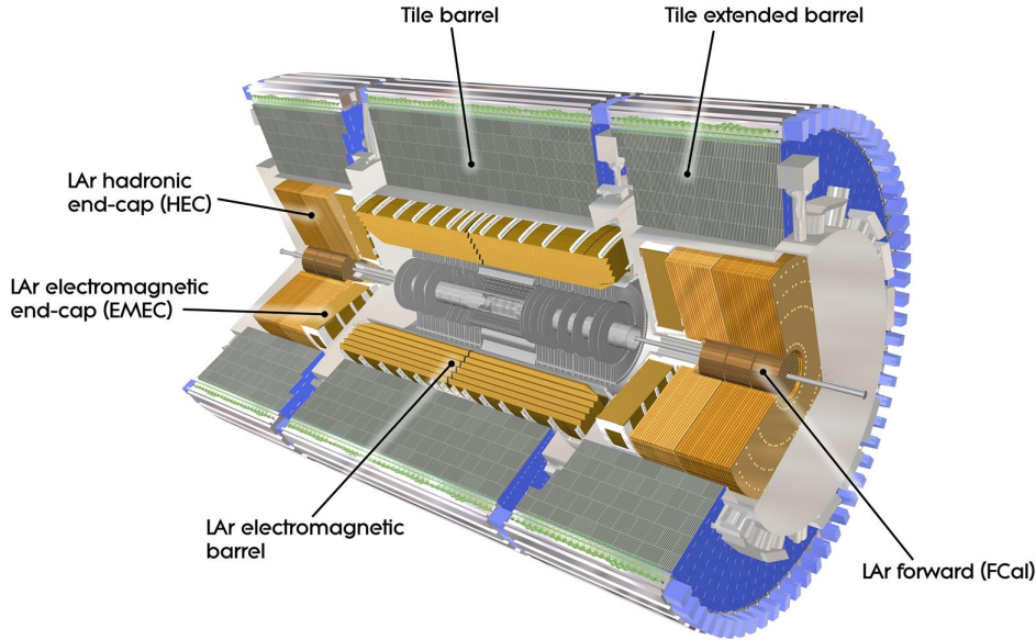
Figure 1.17: Cut-away view of the ATLAS calorimeters.
