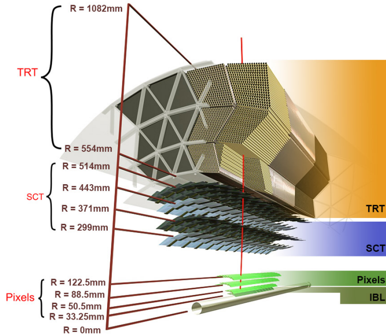
Figure 1.11: The sensors and the structural elements of the Inner Detector.
