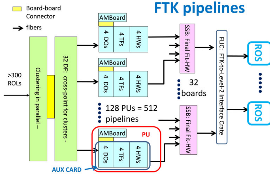
Figure 3.2: Sketch of FTK seen as a set of 512 pipelines up to the final 12-layer fit in the SSBs. The black arrows show the connections through fibers and the yellow rectangles show high frequency connections between mezzanine cards and motherboards or between two boards in the same crate slot.
