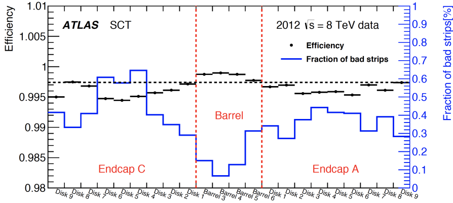
Figure 1.15: Mean intrinsic hit efficiency for each layer of the SCT measured in proton-proton data at \sqrt{s} = 8 TeV in 2012. The dashed line indicates the overall mean value. The blue line and right-hand axis show the fraction of strips in the layer which are disabled (dead or noisy).
