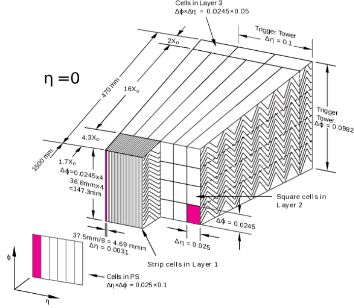
Figure 1.18: Electromagnetic calorimeter granularities.
