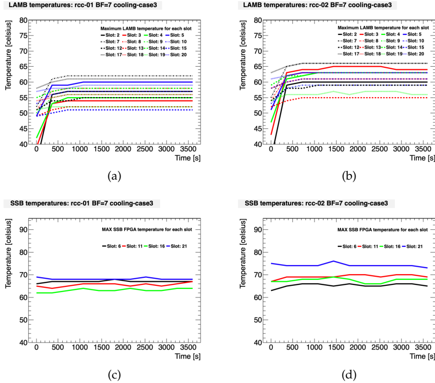
Figure 4.19: Profile of the maximum LAMB temperatures (a),(b) and of the maximum SSB FPGA temperatures (c),(d) for the BF 7 AMB configuration. The test was executed after enabling the water chiller.
