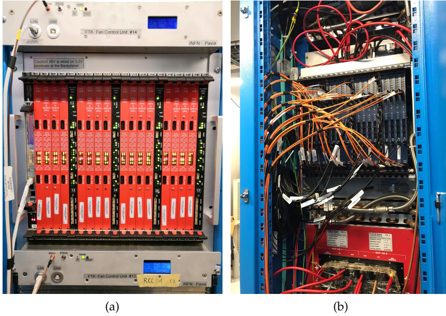
Figure 3.12: (a) Picture of one of the FTK VME crates in their final configuration. It is possible to see the 16 AMBs (red boards), the 4 SSBs (black boards), and the controller Single Board Computer (SBC) in slot 0. The 16 AUXs and 4 SSB RTMs are not visible, in the back of the crate.
