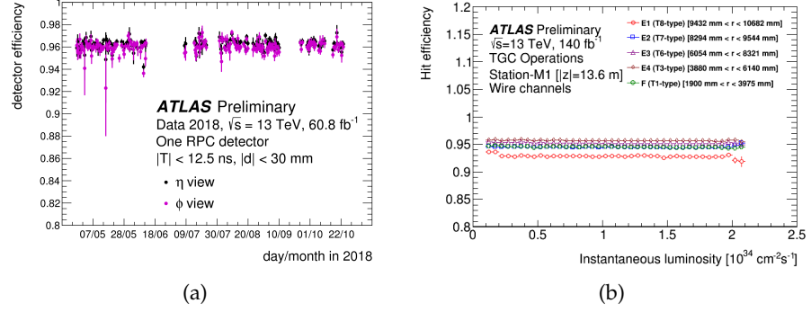
Figure 1.26: (a) RPC efficiency as a function of time for one readout panel in the \eta (black) and \phi (magenta) views. Each point corresponds to a different ATLAS run recorded in 2018 during pp collisions. (b) Averaged hit efficiency for particular chamber type in one of the ATLAS TGC station ( |z| = 13.6 \text{ m} ) as a function of instantaneous luminosity in Run2.
