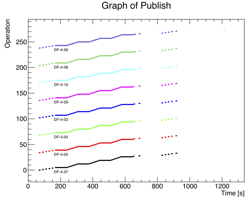
Figure 5.13: Plot of the time execution of the two RM monitoring functions for the DF boards. In the plot, the y value represent the execution of a given operation, i.e. the execution of one of the monitoring functions. The faster operations (the short lines on a given y value) represent the execution of the publish function, while the longer operations represent the execution of publishFullStat.
