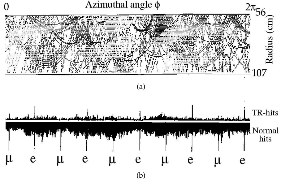
Figure 2.1: Histogramming for pattern recognition in the ATLAS TRT detector: R\phi view of all the TRT hits (a) and histogram for muon and electron tracks with pile-up background (b). The upper part of the histogram contains the \phi position of high threshold hits generated by transition radiation from electrons. The lower part contains normal tracking hits in the TRT. The histogramming technique allows to identify high momentum tracks and to distinguish between different kind of particles.
