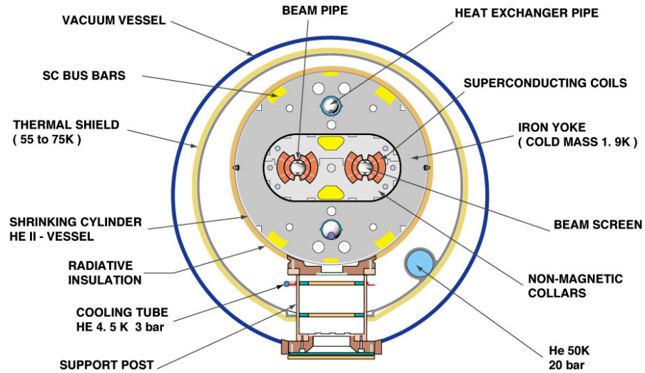
Figure 1.3: Cross-section of an LHC dipole.
