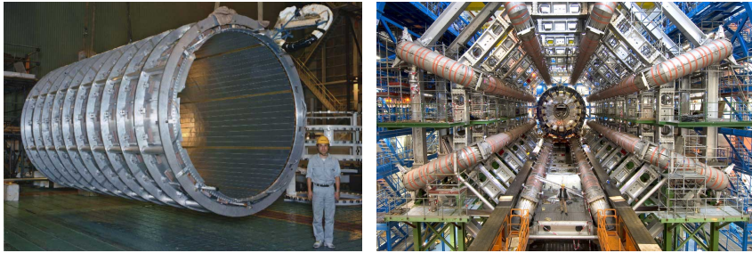
Figure 1.9: (a) The ATLAS solenoid providing the magnetic field in the inner detector. (b) Photograph of the toroid magnet in the barrel region of ATLAS.
