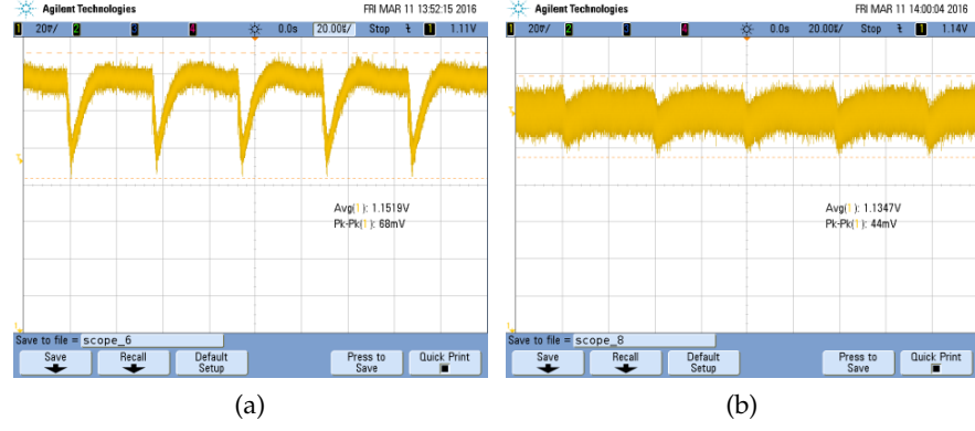
Figure 4.1: Effect on the voltage ripple of the module dummy hit. The quiescent current is increased in order to reduce the effect of the current peak. In Figure (a), without the use of dummy hit a quiescent current of 3 A per LAMB results in a peak to peak variation of 68 mV. In Figure (b), using the dummy hit the quiescent current is increased to 38 A per LAMB, reducing the peak to peak voltage variation to 44 mV. In both the figures, the time scale is 20 \mu\text{V}/\text{div} , and the vertical scale is 50 mV/div.
