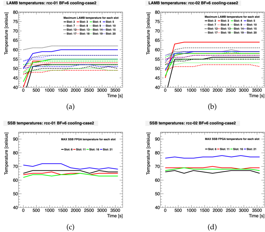
Figure 4.15: Profile of the maximum LAMB temperatures (a),(b) and of the maximum SSB FPGA temperatures (c),(d) for the BF 6 AMB configuration. The test was executed with an increased water flux of the FTK cooling system of 5 bar.
