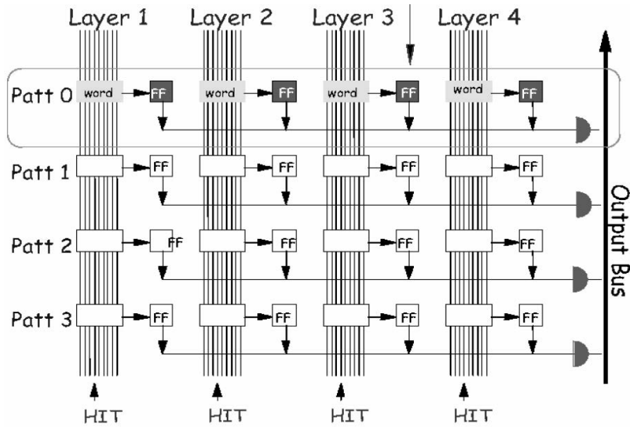
Figure 2.7: Sketch of an Associative Memory chip basic circuit.
