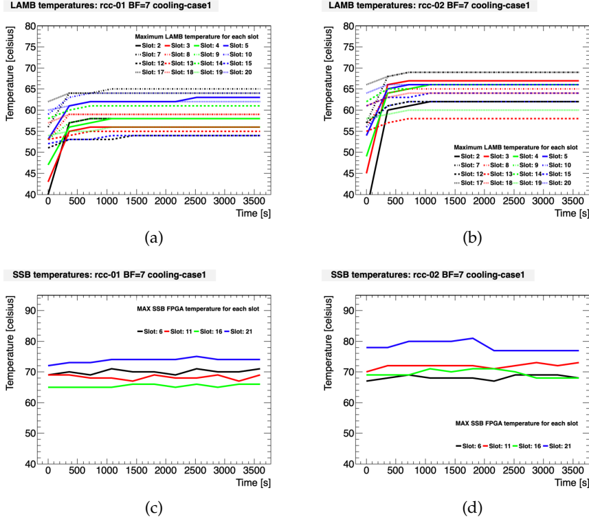
Figure 4.14: Profile of the maximum LAMB temperatures (a),(b) and of the maximum SSB FPGA temperatures (c),(d) for the BF 7 AMB configuration. All the temperatures are well under the respective board operational limits.
