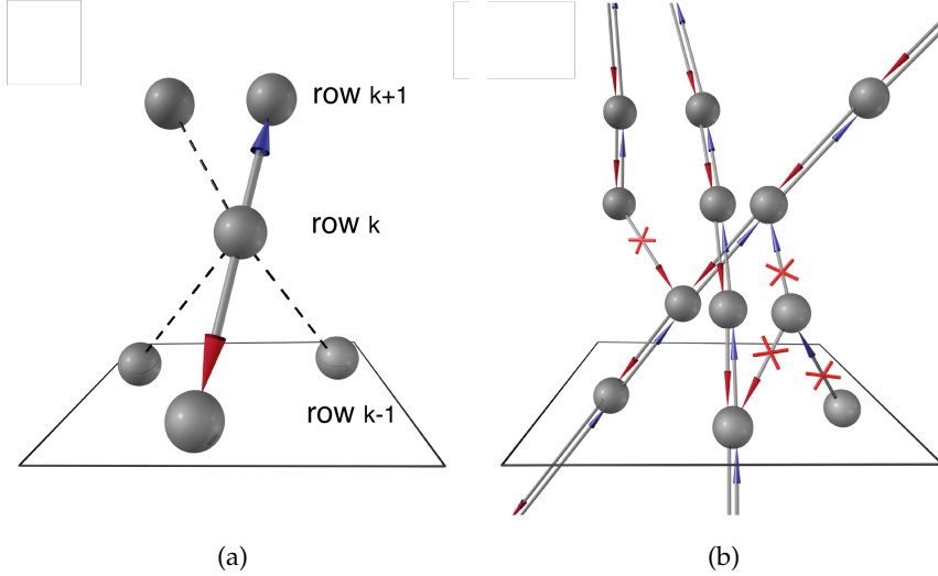
Figure 2.8: Illustration of the Cellular Automaton algorithm. (a) Neighbour finder. (b) Evolutional step.
