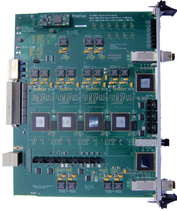
Figure 3.6: Picture of an FTK AUX card. This board is responsible for the first stage processing of the tracks.
