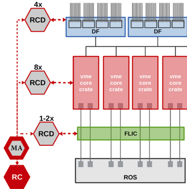
Figure 5.12: Sketch of the stopless-recovery procedure infrastructure of FTK. The Manager Application (MA) manages the communications between the board controller applications (RCDs), dispatching the recovery transition actions and managing the internal FTK FSM.
