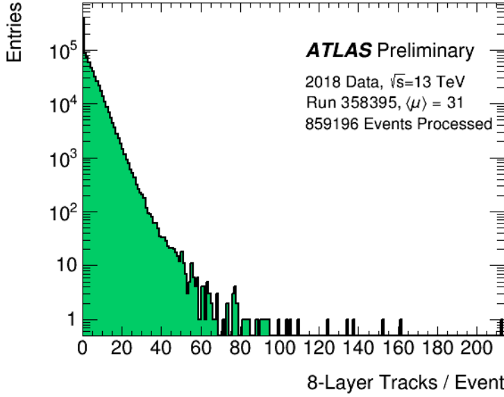
Figure 3.17: Results from a subset of 859 196 events from Run 358 395, a 13 TeV pp run which began on August 2018 with the FTK Slice2 (FTK tower 40). The plot is showing the number of 8-layer tracks produced per event.
