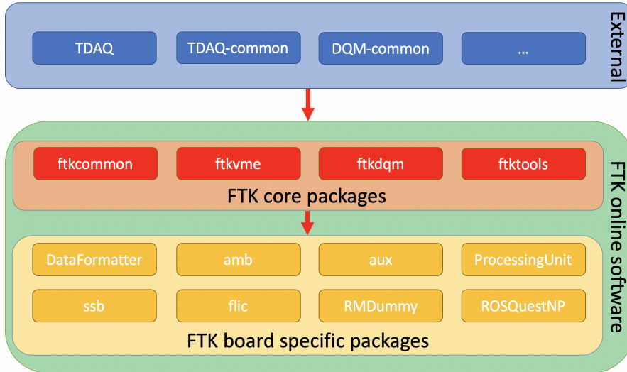
Figure 5.3: Sketch of the FTK online SW structure. The FTK online SW is composed of 12 different packages: 4 of them form the core SW, while the others are FTK HW components specific.
