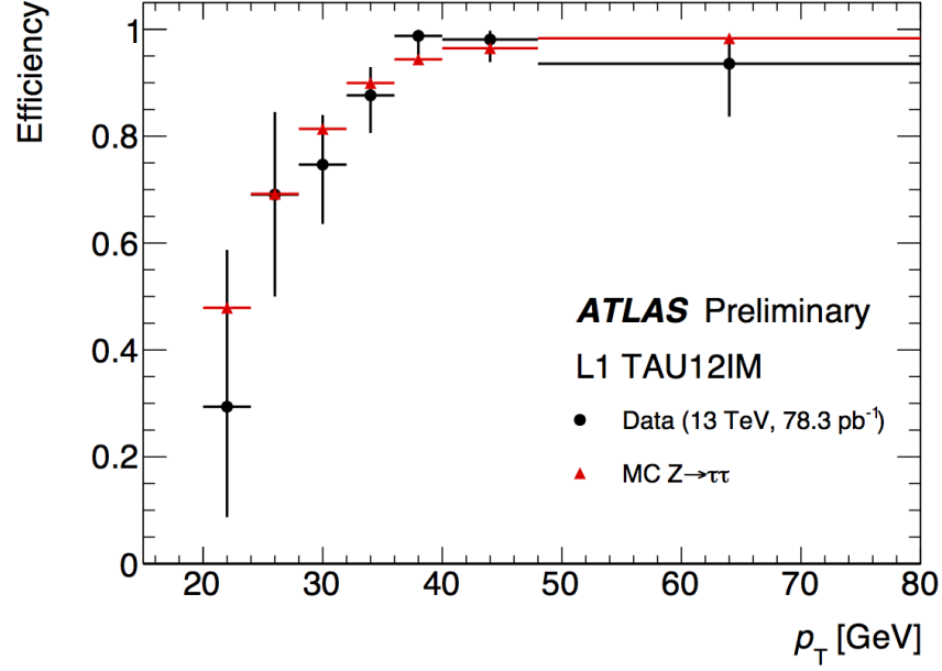
Figure 6.6: The Level-1 tau trigger efficiency measured in data and compared to simulation, with respect to offline reconstructed tau candidates transverse momentum with p_T above 20 GeV. The online tau candidates are reconstructed at L1 of the ATLAS trigger and are required to have a transverse energy of 12 GeV.
