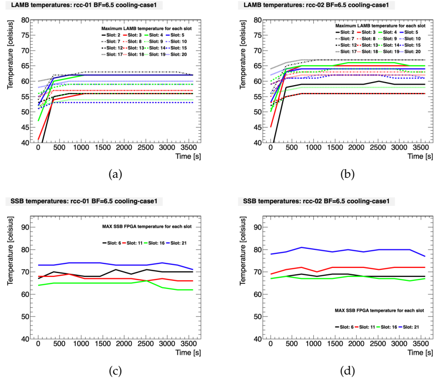
Figure 4.13: Profile of the maximum LAMB temperatures (a),(b) and of the maximum SSB FPGA temperatures (c),(d) for the BF 6.5 AMB configuration. All the temperatures are well under the respective board operational limits.
