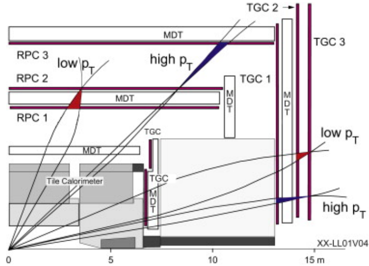
Figure 1.29: The layout of L1Muon showing the requirements for the different muon triggers.
