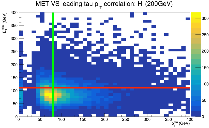
Figure 6.18: Leading tau p_T distribution vs missing transverse energy for the decay of a charged Higgs boson of 200 GeV in the H^+ \rightarrow \tau_{\text{had}}^+ \nu decay channel. The red line represents the 110 GeV MET threshold of the E_T^{\text{miss}} trigger chain used in the original analysis, while the green line represent the 80 GeV tau p_T threshold of the FTK based single-tau trigger chain.
