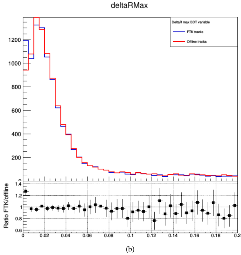
Figure 6.15: Distribution of the f_{iso}^{track} (a) and of the \Delta R_{Max} (b) BDT variables computed with offline and FTK tracks.
