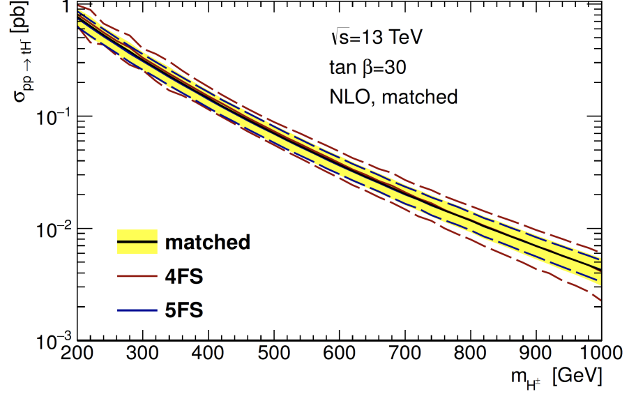
Figure 6.2: Production cross section for the heavy charged Higgs boson (i.e. resulting from the associated production with a top quark), as a function of m_{H^+} , in a type-II 2HDM with \tan \beta = 30 [87]. The predictions are shown for the left (5FS) and right (4FS) diagrams of Figure 6.1.
