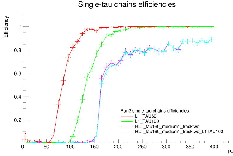
Figure 6.11: Efficiency of the Run2 L1 and HLT single-tau trigger chains as a function of the offline tau p_T . The efficiencies have been calculated on a sample of simulated \tau\bar{\tau} events.
