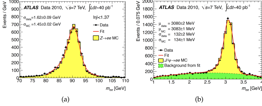
Figure 1.19: Reconstructed dielectron mass distribution for Z \rightarrow ee (a) and J/\psi \rightarrow ee (b) decays and comparison with simulation.
