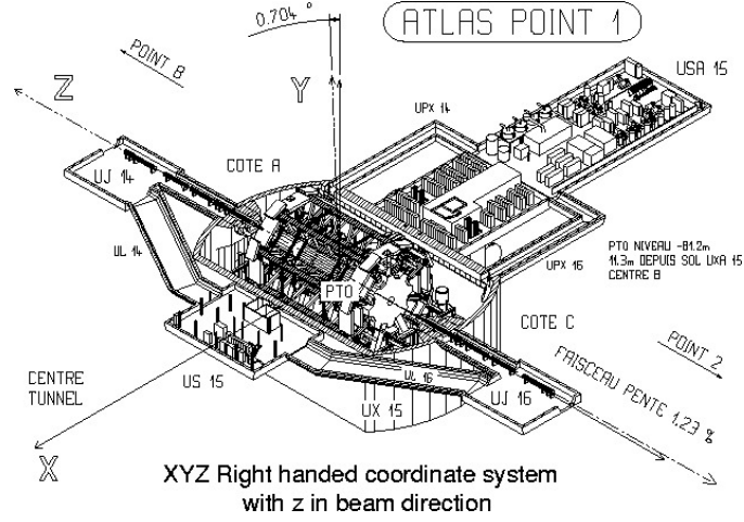
Figure 1.7: The coordinate system of the ATLAS detector.
