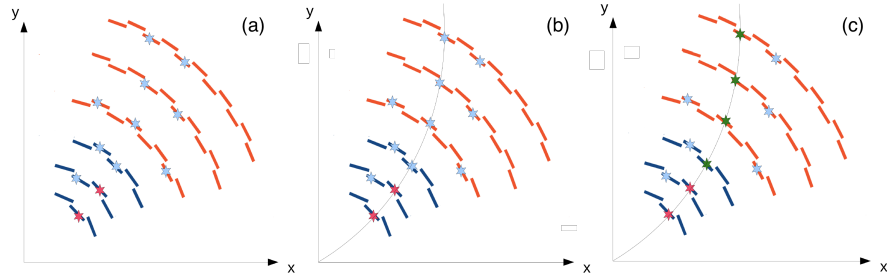
Figure 2.15: In the first step (a) of the algorithm a pair of stubs (red) in adjacent layers are combined to form a tracklet. The trajectory of the tracklet is projected (b) to the other layers. Stubs in the other layers that are close to the projection (green) are selected as matched (c) to the tracklet. Final track parameters are calculated using all associated stubs.
