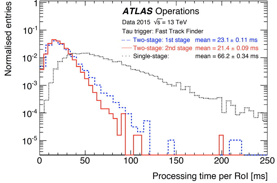
Figure 6.9: The ID trigger tau tracking processing time for the fast-track finder comparing the single-stage and two-stage tracking approach.
