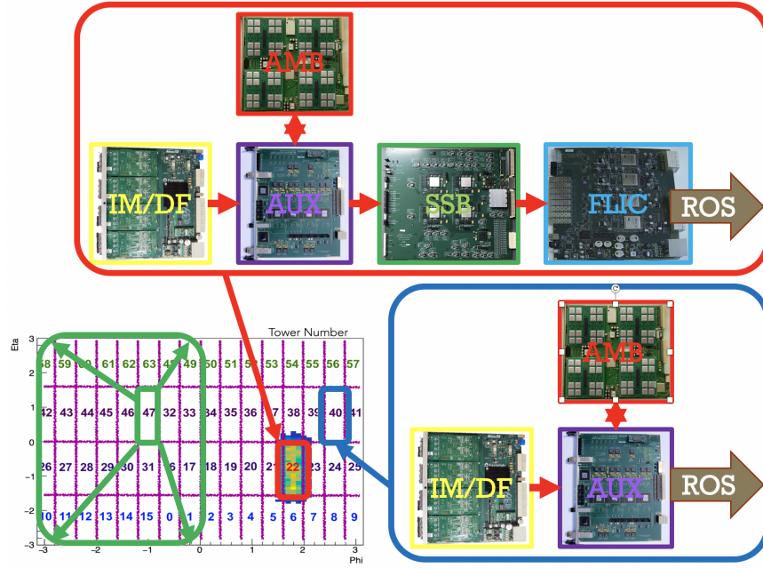
Figure 3.14: Tower distribution of the 3 FTK slices that were commissioned during 2018. A sketch of the composition of the SliceA (red box) and Slice2 (blue box) is also presented. Slice47 (green in the tower distribution plot) started its commissioning as a single tower, but will be expanded to cover the Hemisphere , corresponding to half of the full FTK system.
