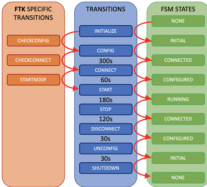
Figure 5.5: Sketch representing the FSM states and transitions available for ATLAS and all its subsystems. The average ATLAS transition times are shown under each of the transitions. The FTK specific sub-transitions are also shown. These sub-transitions are executed by the FTK subsystem only, and are executed before the given common transition, to which they are associated to, takes place. More details about the FTK specific transitions will be given in Subsection 5.5
