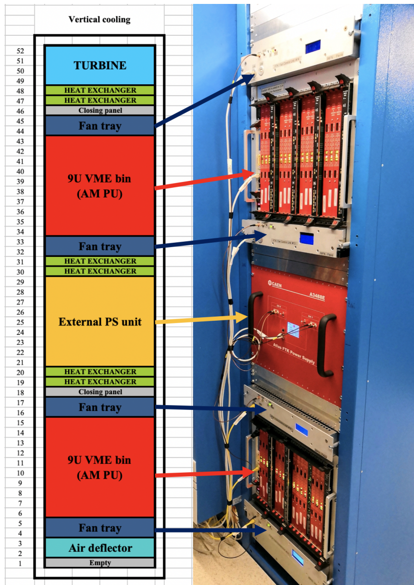
Figure 4.6: Sketch representing the VME rack configuration, together with a picture of a fully populated rack.
