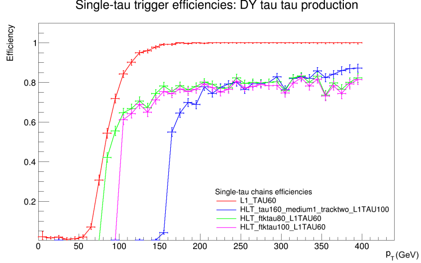
Figure 6.16: Selection efficiency of the two FTK based single-tau trigger chains, together with the efficiencies of the L1 and HLT single-tau standard chains, as a function of the offline tau p_T . The efficiencies have been calculated on a sample of simulated \tau\bar{\tau} events.
