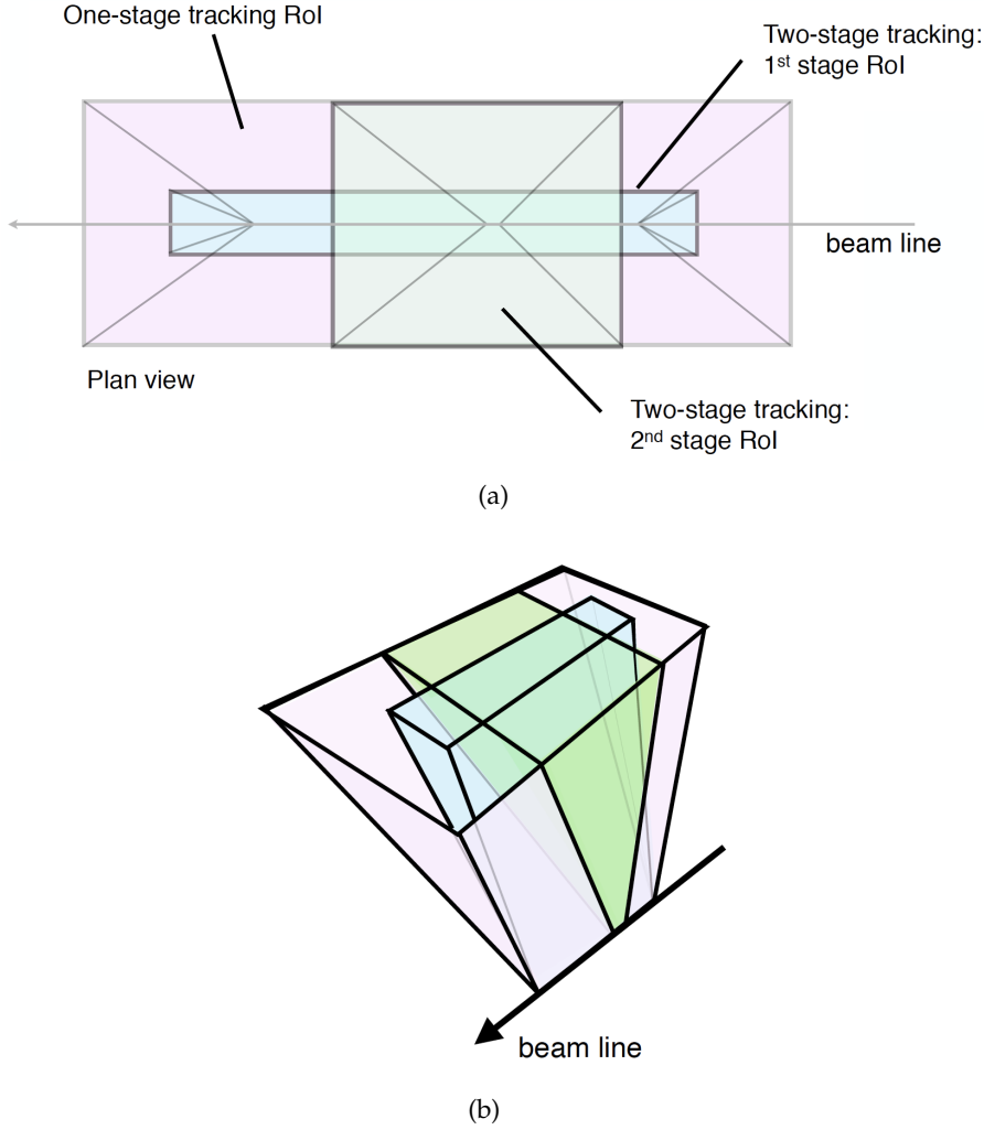
Figure 6.8: Sketch illustrating the RoI from the single-stage and two-stage tau lepton trigger tracking in plan view (x-z plane) along the transverse direction (a) and in perspective view (b).
