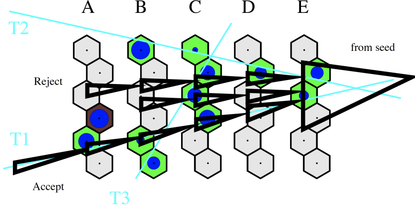
Figure 2.4: Sketch of the track search using a combinatorial Kalman filter. In the sketch the track search is performed along different branches starting from a given track seed.
