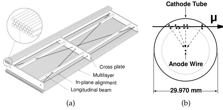
Figure 1.24: (a) Schematic view of the mechanical structure of an MDT chamber. (b) Cross section of an aluminium tube.
