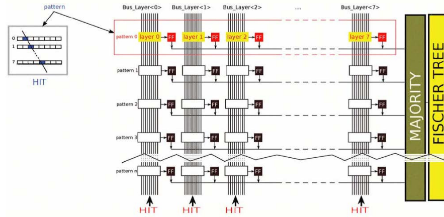
Figure 3.8: The AMchip array.
