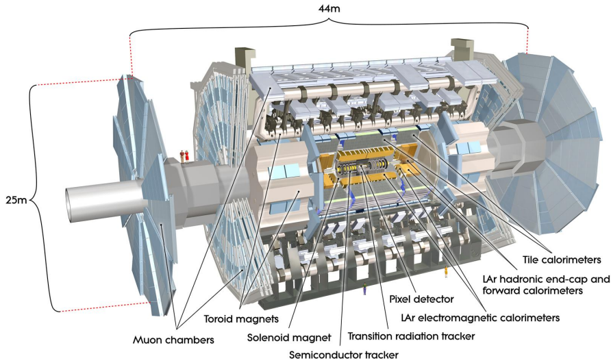
Figure 1.6: View of the ATLAS detector, showing the different subdetectors and layers around the proton beam axis. The collisions occur in the centre of the detector. The main detector components are indicated.
