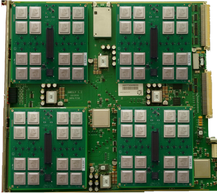
Figure 3.7: Picture of an AM Board. In the picture it is possible to see the AMB, the 4 LAMBs, and the 64 AMchips. The LAMBs in the picture show their internal face, in order to make it possible to see the AMchips. When the LAMBs are plugged, the AMchips are facing the AMB.
