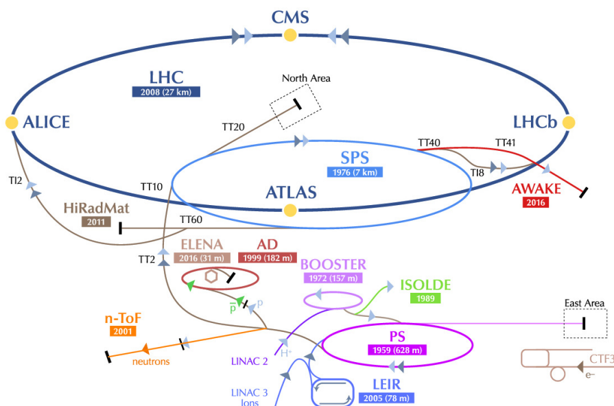
Figure 3.1: Schematic of the CERN accelerator complex. The locations of the four main LHC experiments (ALICE, ATLAS, CMS and LHCb) are shown around the LHC ring. Image (edited) from [143].
