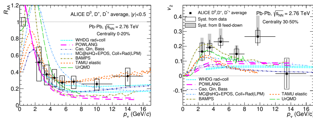
Figure 2.16: ALICE results for D^0 -, D^+ - and D^{*+} -meson (left) R_{AA} and (right) v_2 as a function of p_T , compared with theoretical calculations [100–111]. Figures from [99].
