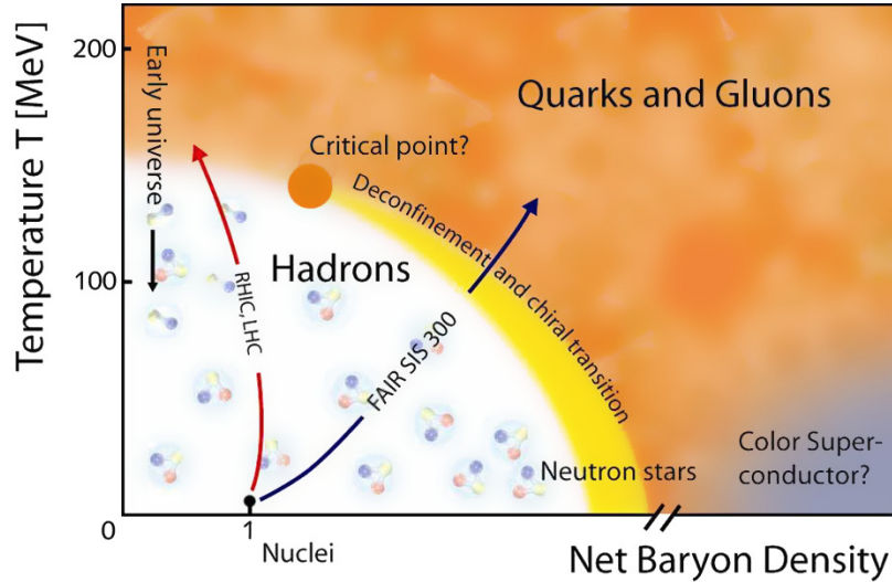
Figure 2.3: The phase diagram for QCD matter, as a function of net baryonic density and temperature. The arrows indicate regions of the phase diagram that are probed by collider experiments. Figure (edited) from [34].
