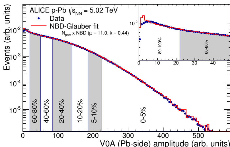
Figure 3.8: Distribution of the sum of amplitudes in the V0A hodoscopes in p–Pb collisions at \sqrt{s_{\text{NN}}} = 5.02 TeV. The boundaries between centrality classes are indicated by vertical lines. An NBD-Glauber fit [146, 155–158] to the distribution is shown as a red line. The inlay shows a zoomed-in view of the 0–50 amplitude region, corresponding to the 40% most peripheral events. Figure from [131].
