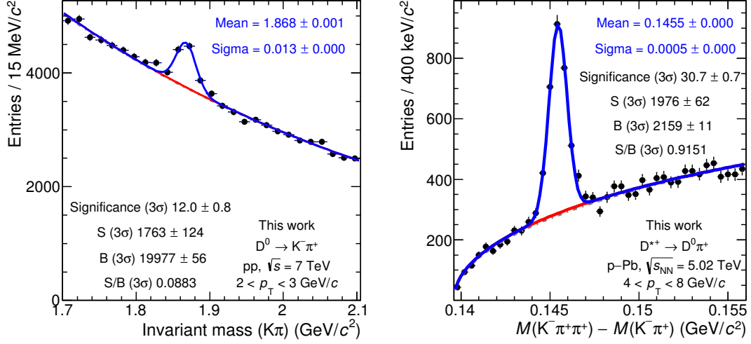
Figure 4.2: Invariant mass histograms for D-meson reconstruction. Left: D^0 mesons with 2 < p_T < 3 GeV/c in pp collisions at \sqrt{s} = 7 TeV. Right: D^{*+} mesons with 4 < p_T < 8 GeV/c in p-Pb collisions at \sqrt{s_{NN}} = 5.02 TeV. The background functions are given by red curves; the sum of signal + background by blue curves. Each plot shows the signal, background statistical significance and signal-to-background ratio given by the fit in the signal region.
