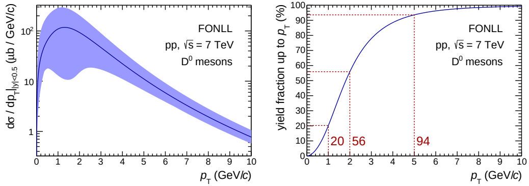
Figure 2.10: FONLL calculations [61,62] of the p_T -differential D^0 -meson production cross section at mid-rapidity, as a function of p_T . Left: p_T spectrum; right: cumulative fraction of the total cross section as a function of p_T . The calculations are shown as a curve, and their uncertainties as a shaded band. The red numbers and dashed lines mark percentiles of the cumulative distribution, integrated from p_T = 0 GeV/ c . Figures from [65].
