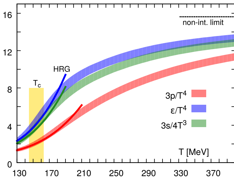
Figure 2.4: Calculations of 3p/T^4 , \varepsilon/T^4 and 3s/4T^3 on the lattice as a function of temperature, shown alongside calculations under a hadron resonance gas (HRG) approximation. The critical temperature T_c = 154 \pm 9 MeV is shown as a vertical shaded band, and the Stefan–Boltzmann limit for the energy density of an ideal gas ( 95\pi^2/60 ) as a horizontal dashed line. Figure from [40].
