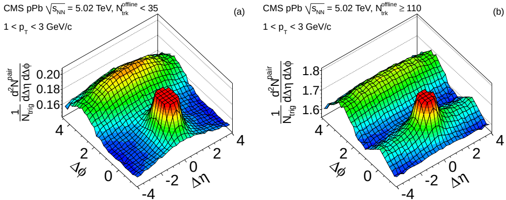
Figure 2.19: Plots of angular two-particle correlations in p–Pb collisions at \sqrt{s_{NN}} = 5.02 TeV at (left) low and (right) high multiplicity, measured by the CMS Collaboration. Figure from [7].
