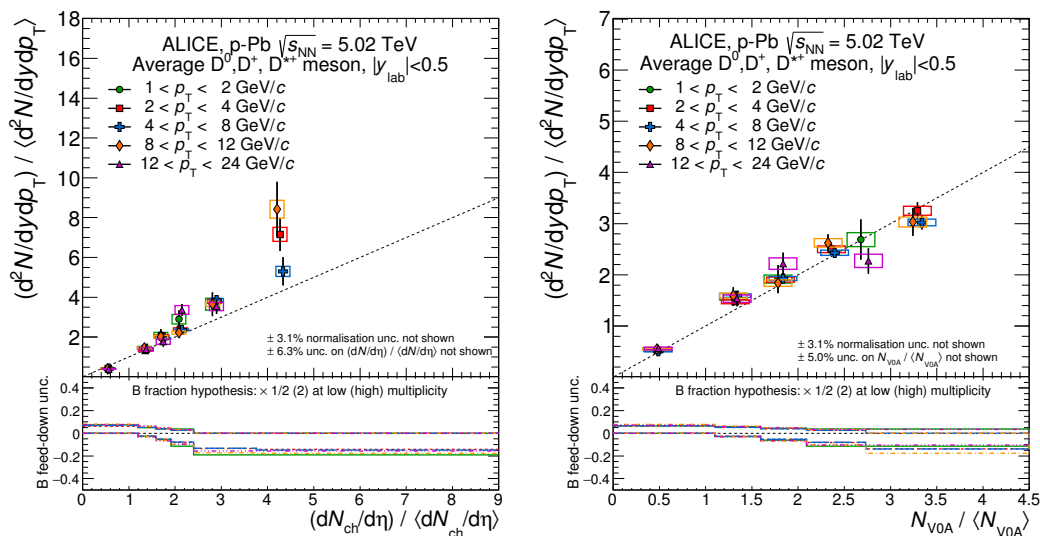
Figure 6.11: Average relative yield for D^0 , D^+ and D^{*+} mesons as a function of charged-particle multiplicity at (left) mid- and (right) backward rapidity in p-Pb collisions at \sqrt{s_{NN}} = 5.02 TeV. Results are shown for five p_T intervals within the range 1 < p_T < 24 GeV/c. The lower panels show the systematic uncertainties due to the feed-down from B-meson decays. Figures from [17].
