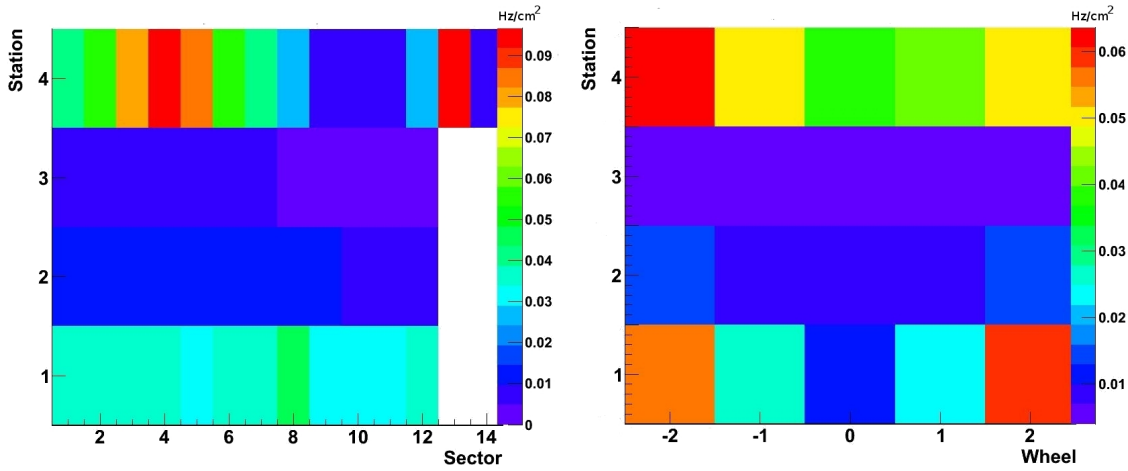
Figure 6.24: Average noise for a instantaneous luminosity of the LHC of 10^{32} \text{ cm}^{-2}\text{s}^{-1} . Left plot shows a station-sector map, averaging over all wheels. Right plot shows the dependency with the wheel and station, averaging over all sectors.
