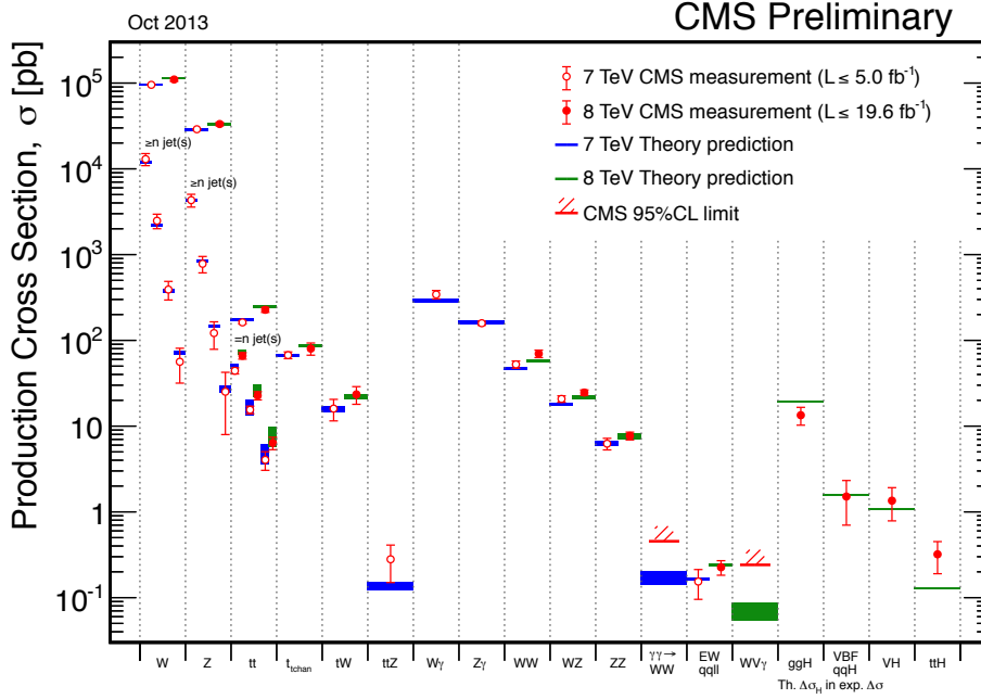
Figure 5.1: Summary of inclusive production cross sections measured in collisions at \sqrt{s}=7 and 8 TeV.
