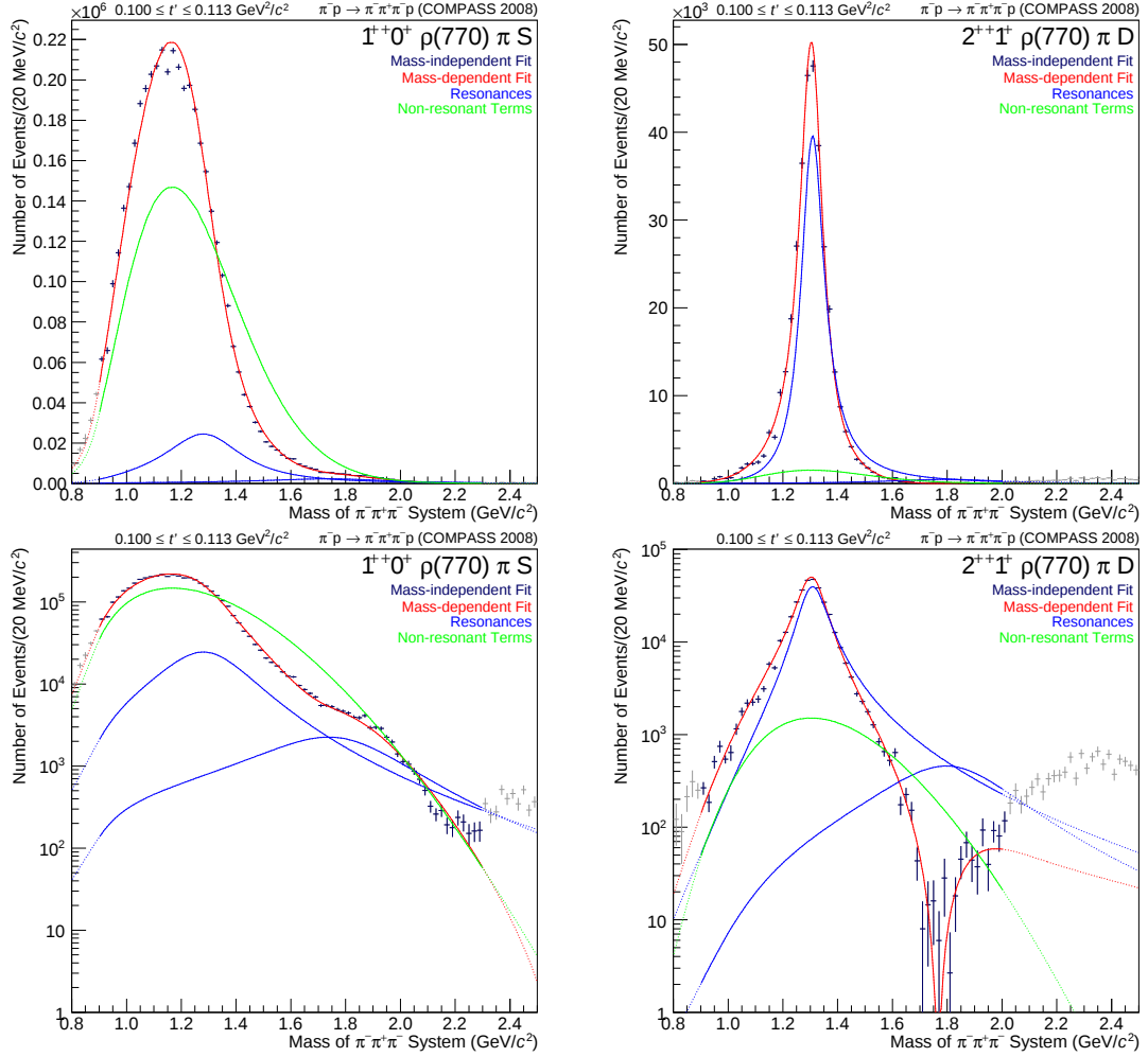
Figure 4.2: Intensity of the 1^{++}0^{+}\rho(770)\pi S (left) and the 2^{++}1^{+}\rho(770)\pi D (right) partial waves for the lowest t' bin in linear (upper row) and logarithmic scale (lower row). The red line represents the total mass-dependent fit, whereas the other lines show the individual components, being the resonant terms (blue) and the non-resonant terms (green). While the lines are solid inside and dotted outside of the fit range of the mass-dependent fit, the markers representing the mass-independent fit are blue inside and grey outside of this fit range.
