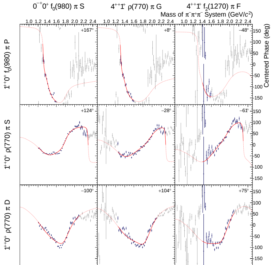
Figure A.7: Part 4 of 10 of the fitted spin-density matrix from figure 4.25. Please refer to the text there for further information.
