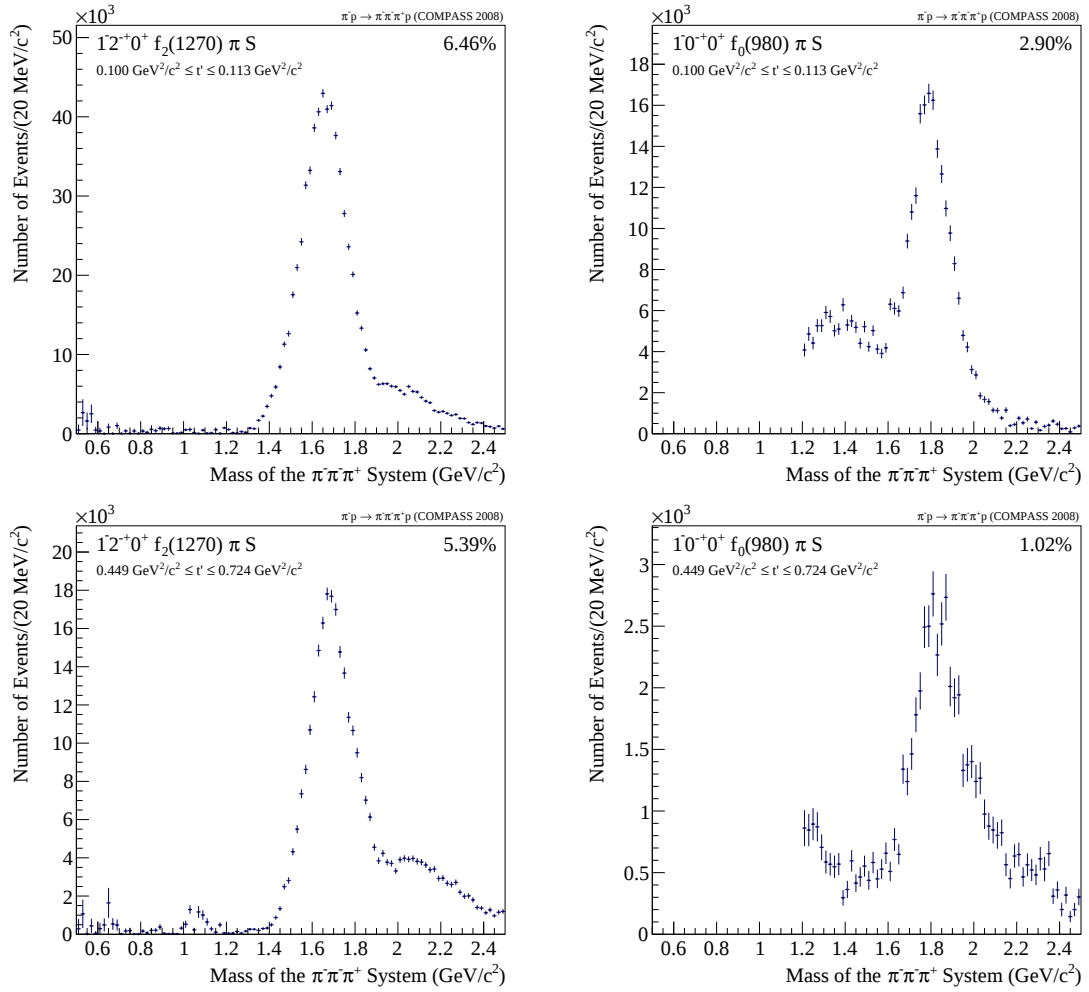
Figure 3.6: Intensities of the 2^{-+}0^{+}f_2(1270)\pi S (left) and 0^{-+}0^{+}f_0(980)\pi S (right) waves for the lowest (upper row) and the second highest (lower row) t' bin [17]. The percentages give the intensity integrals normalised to the total number of events in the respective t' bin.
