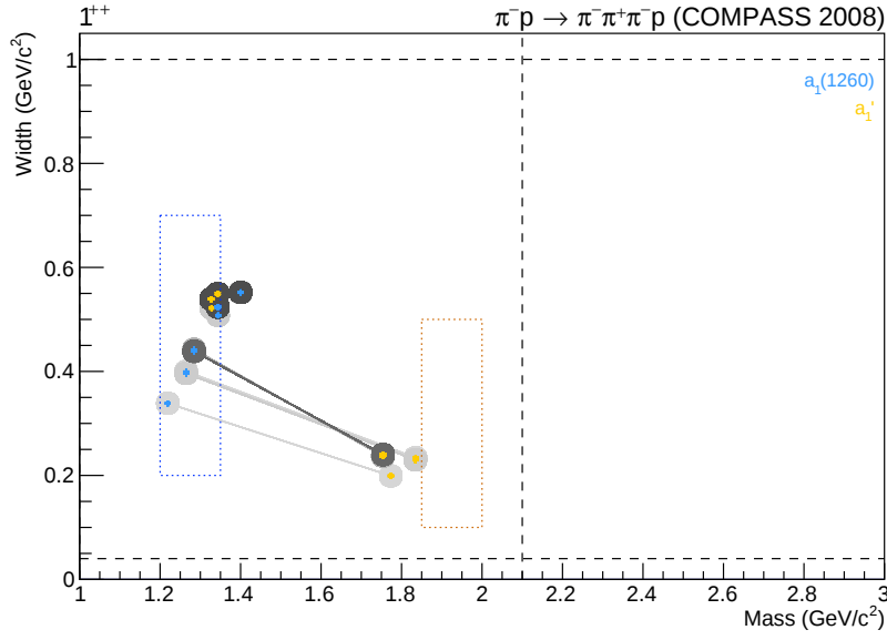
Figure 4.39: Mass and width of a_1(1260) (blue) and a_1'(1260) (yellow) after the removal of spurious solutions for the extended wave set without the 2^{-+}1^+ f_2(1270)\pi S and 2^{-+}0^+ \rho(770)\pi F waves. An explanation of the used plotting scheme can be found in figure 4.12.
