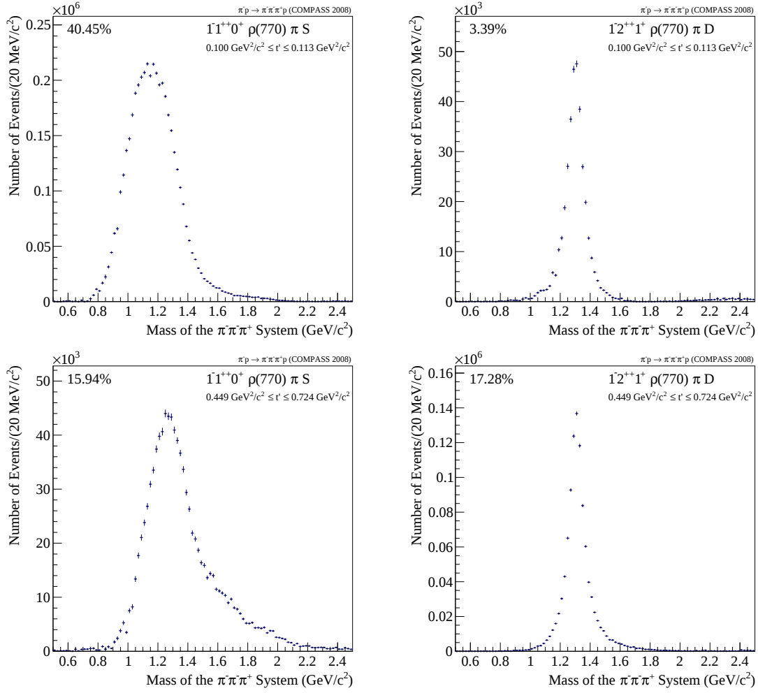
Figure 3.5: Intensities of the 1^{++}0^+ \rho(770) \pi S (left) and 2^{++}1^+ \rho(770) \pi D (right) waves for the lowest (upper row) and the second highest (lower row) t' bin [17]. The percentages give the intensity integrals normalised to the total number of events in the respective t' bin.
