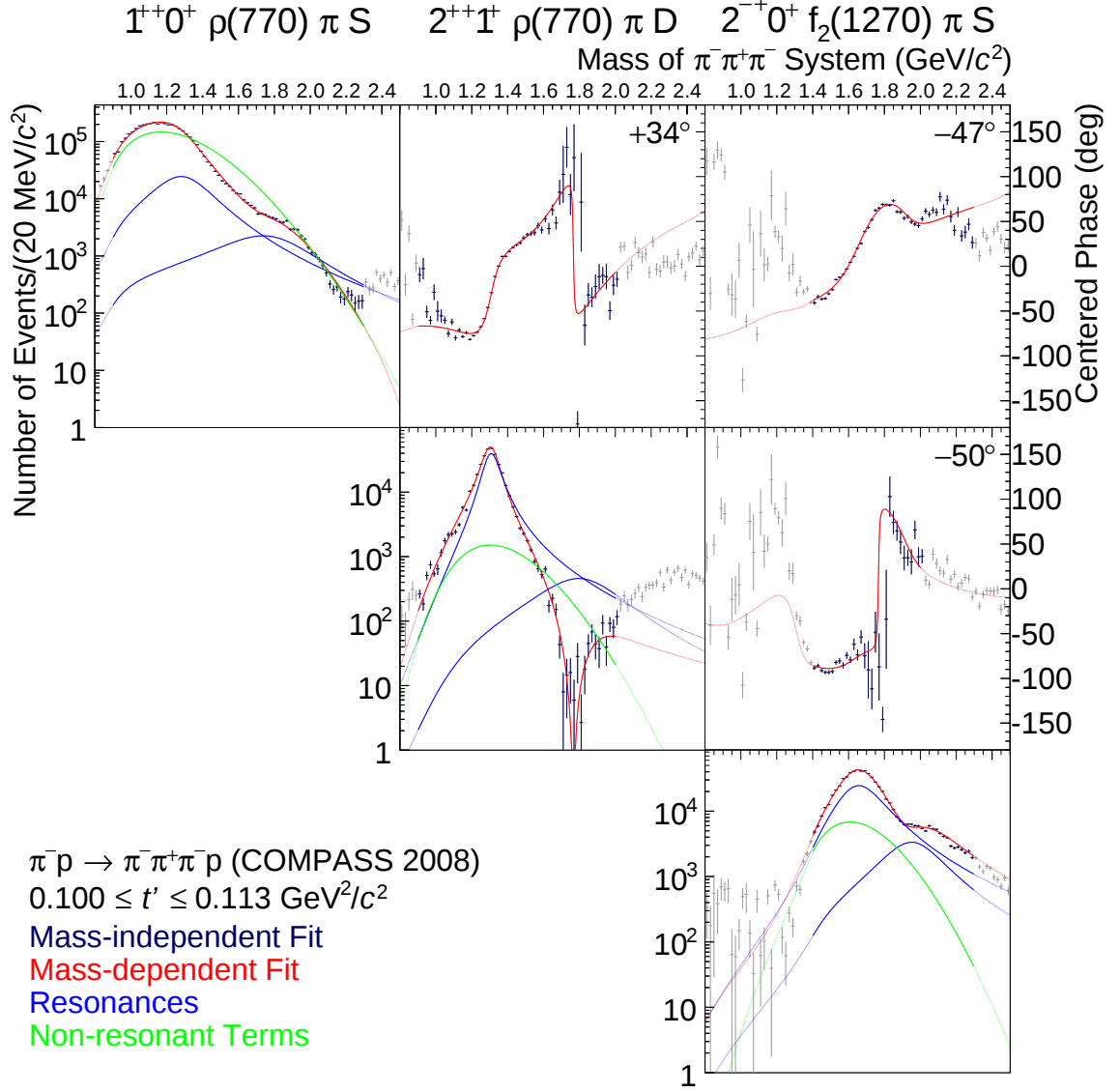
Figure A.1: Part 1 of 3 of the fitted spin-density matrix from figure 4.4. Please refer to the text there for further information.
