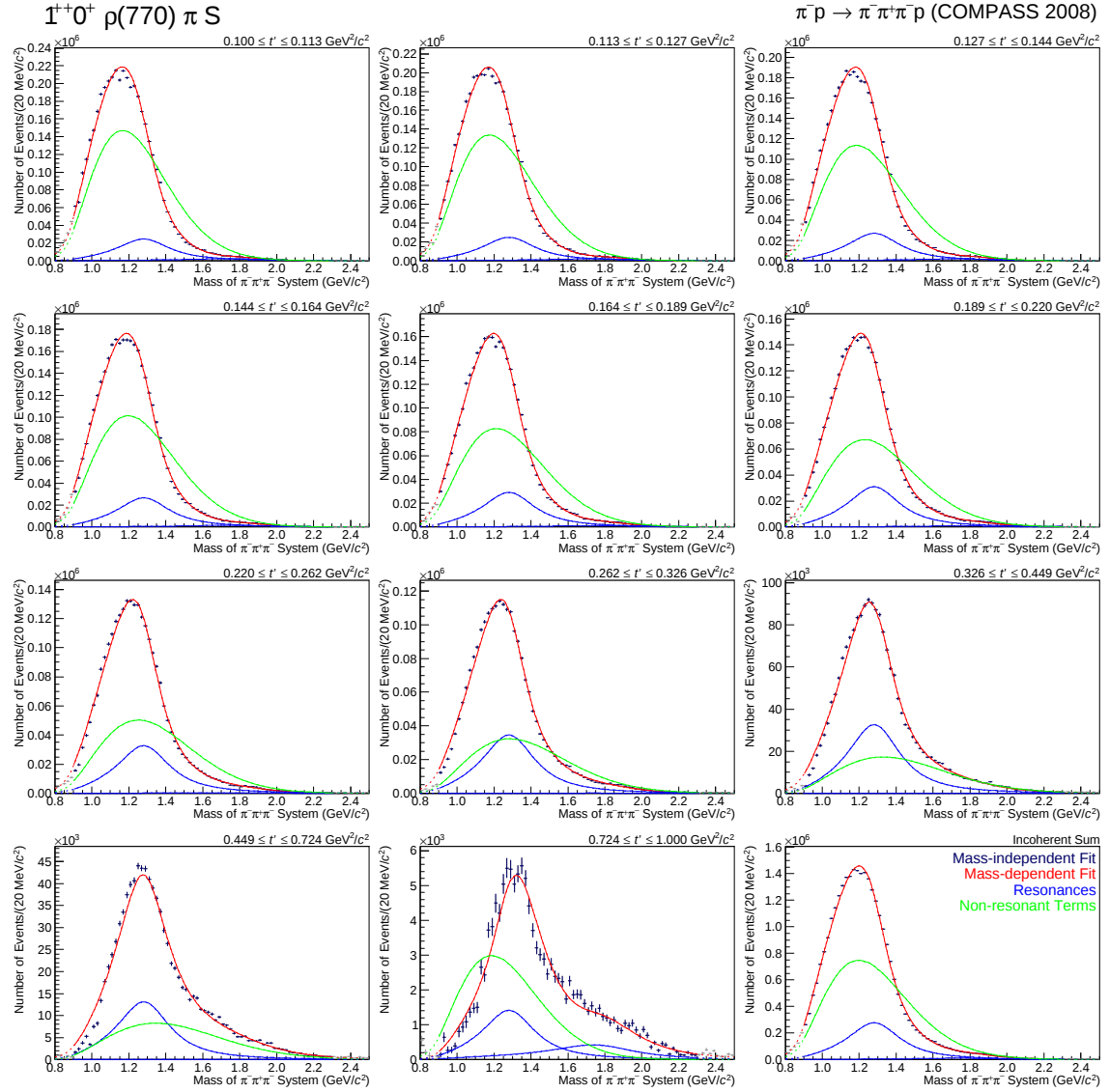
Figure 4.5: Intensity of the 1^{++}0^{+}\rho(770)\pi S wave as a function of t' in linear scale. t' is increasing first from left to right and then from top to bottom. The lower right corner shows the intensity sum of all eleven t' bins. The colour scheme is the same as in the previous plots and described in figure 4.2.
