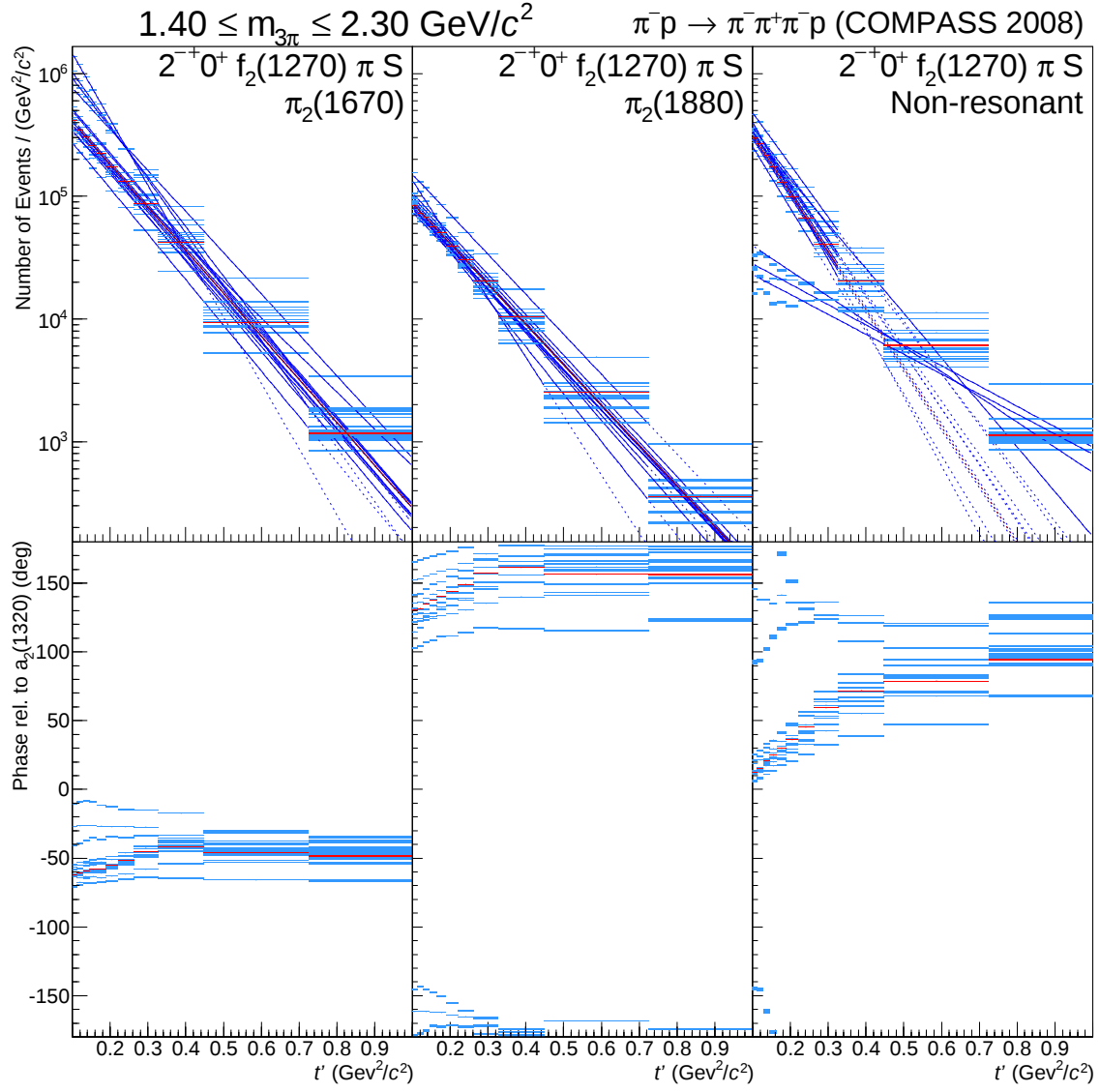
Figure 5.7: t' dependence of the intensity (upper row) and the phase (lower row) of the \pi_2(1670) (left), the \pi_2(1880) (centre) and the non-resonant term (right) in the 2^{-+}0^{+}f_2(1270)\pi S wave. The plotting scheme is the same as in figure 5.3.
