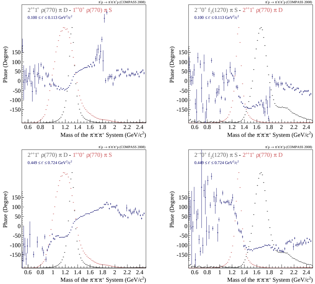
Figure 3.8: Relative phase motions of the 2^{++}1^+ \rho(770) \pi D wave with respect to the 1^{++}0^+ \rho(770) \pi S (left) and the 2^{-+}0^+ f_2(1270) \pi S (right) wave for the lowest (upper row) and the second highest (lower row) t' bin [17]. The intensities of the corresponding waves are also plotted (red, grey) in order to make the correlation to the phases easier to observe.
