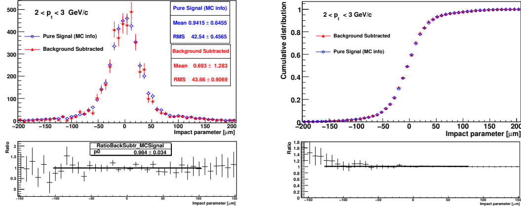
Figure 7.15: Same as in Fig. 7.14 but for a different D^0 transverse momentum interval.
