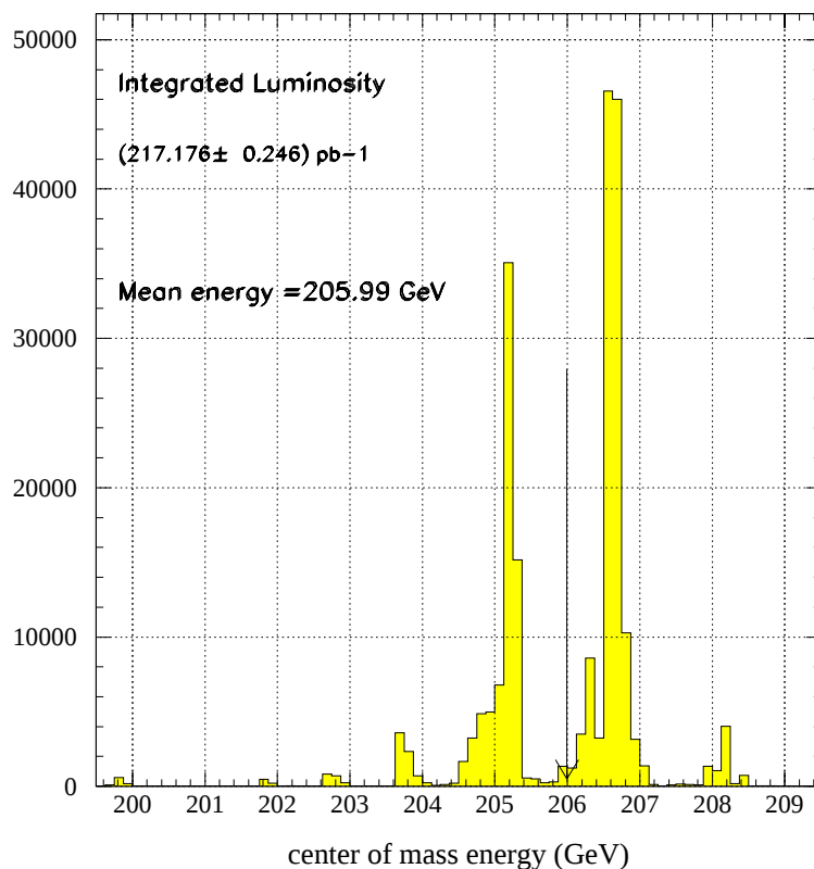
Figure 3.2: Distribution of the integrated luminosity in 2000 as a function of the CM energy. The mean energy of 205.99 GeV is indicated by the downward vertical arrow.
