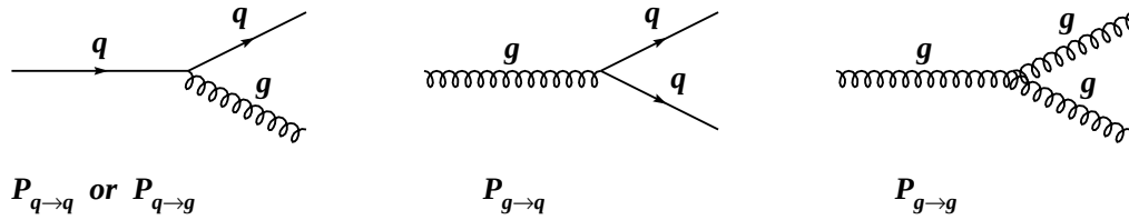
Figure 4.2: Schematic view of the three possible processes in the parton shower: Radiation of a gluon, production of a quark antiquark pair and gluon splitting.
