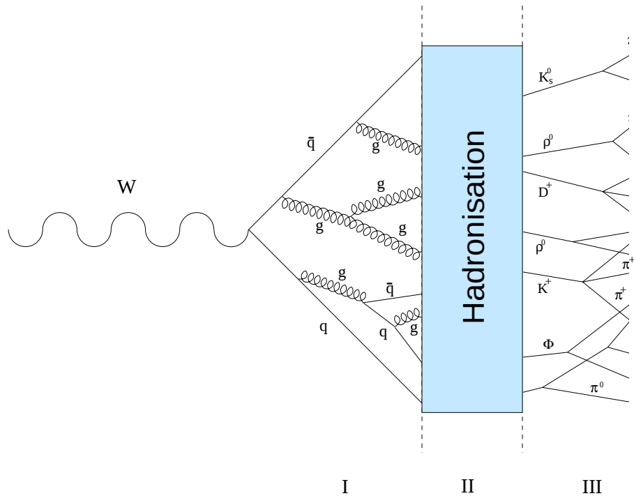
Figure 4.1: View of the parton shower and the fragmentation process. The three phase are explained in the text.
