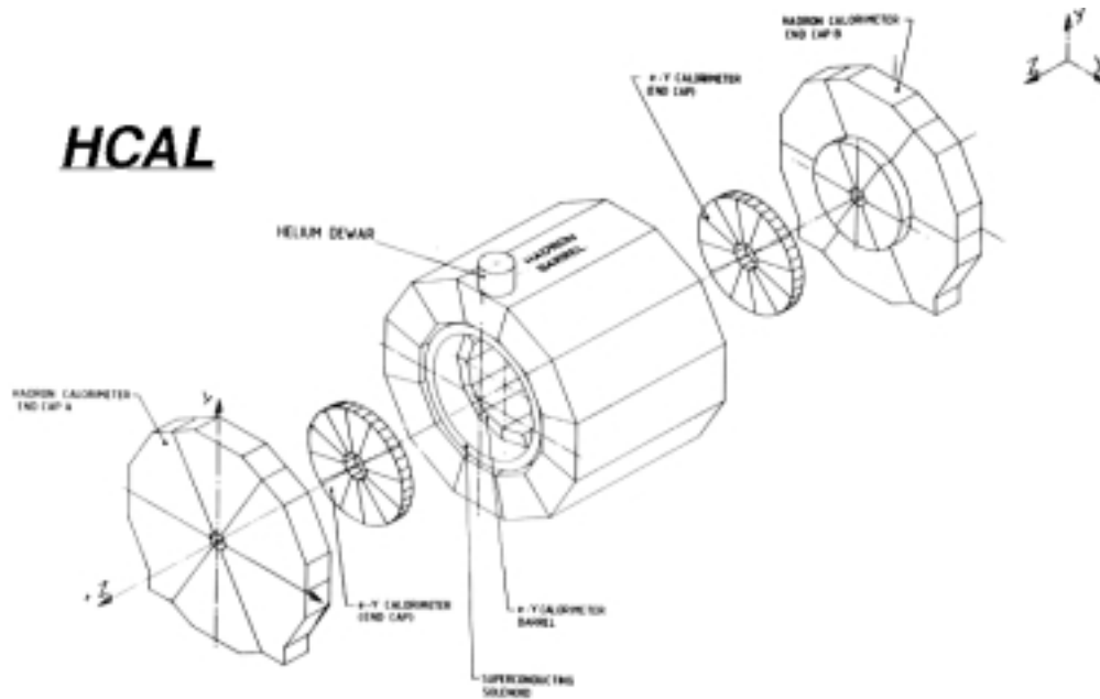
Figure 3.8: Overall view of the HCAL, showing the individual modules of the end-caps and barrel regions.
