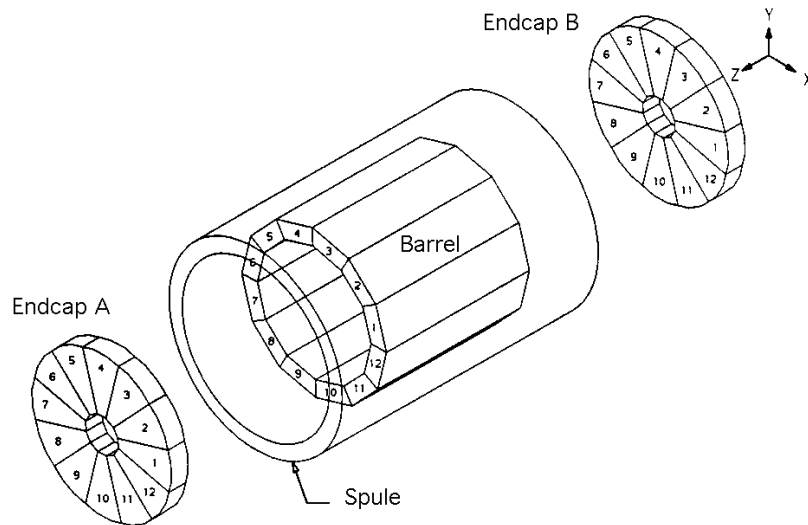
Figure 3.7: Overall view of the ECAL.
