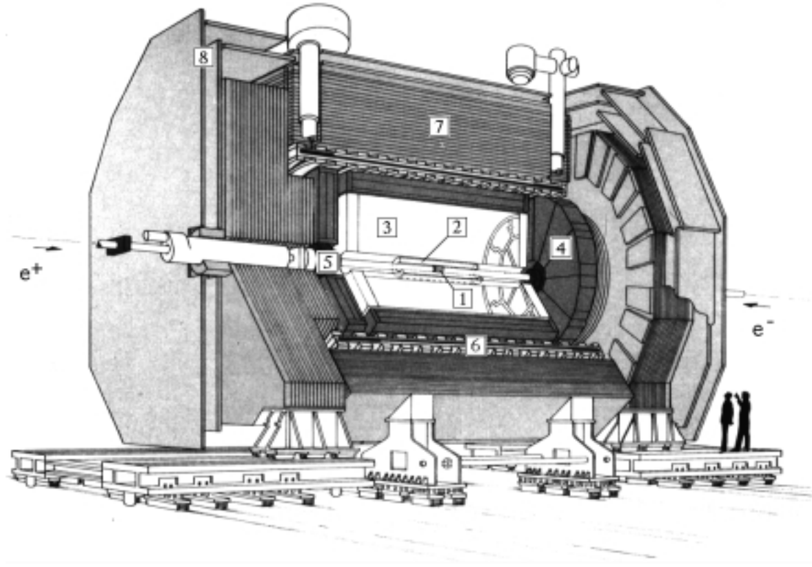
Figure 3.3: The ALEPH-Detector. [1]: Vertex detector, VDET. [2]: Inner Tracking chamber, ITC. [3]: Time Projection Chamber, TPC. [4]: Electromagnetic Calorimeter, ECAL. [5]: Luminosity Monitors, LCAL. [6]: Superconducting Magnet Coil. [7]: Hadron Calorimeter, HCAL. [8]: Muon Detection Chambers.
