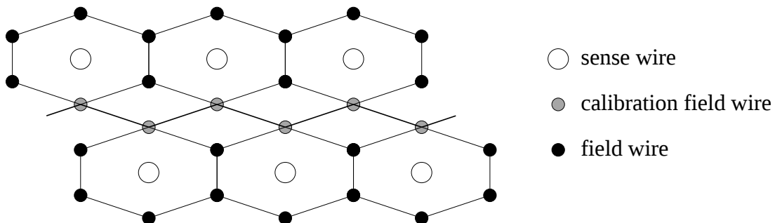
Figure 3.5: Schematic view of drift cell in the ITC.
