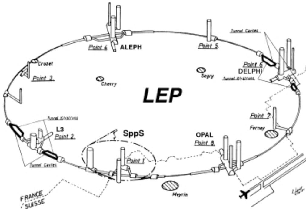
Figure 3.1: Schematic view of the LEP ring with the four experiments and a part of the injector chain.
