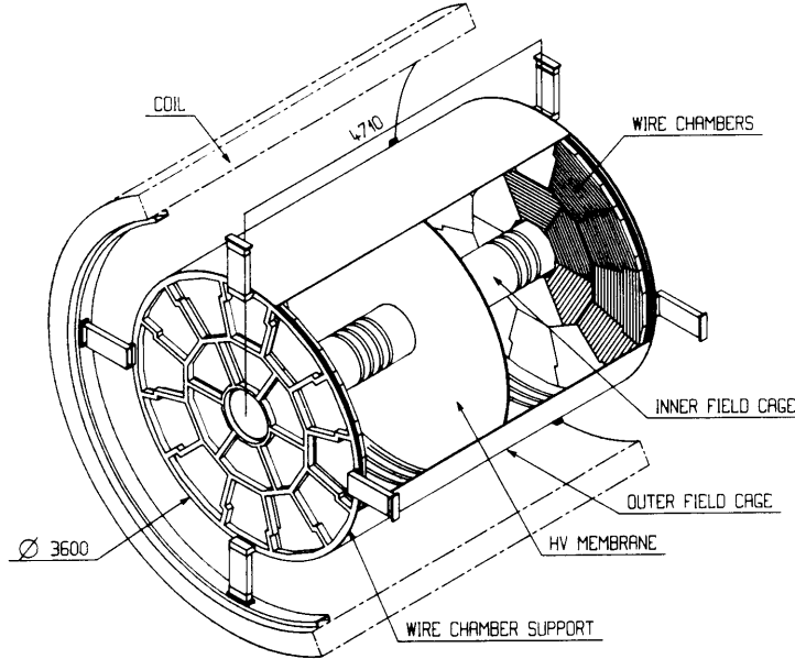
Figure 3.6: Overall view of the TPC.
