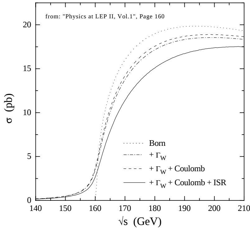
Figure 2.4: The cross-section for e^+e^- \rightarrow W^+W^- in various approximations: (i) Born (on-shell) cross-section, (ii) Born (off-shell) cross-section, (iii) with first order Coulomb correction, and (iv) with initial state radiation.
