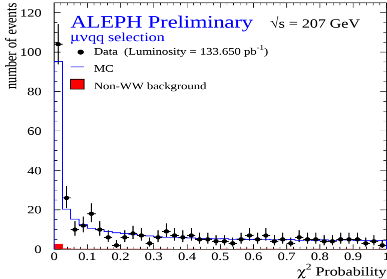
Figure 6.4: \chi^2 Probability of the constrained fit for data and simulated events.
