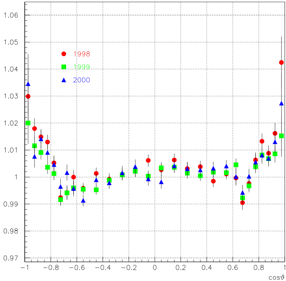
Figure 7.1: Ratio (E_{jet}/E_{beam})_{data}/(E_{jet}/E_{beam})_{MC} of the jet correction as a function of the polar angle for the 1998, 1999 and 2000 Z^0 calibration run.
