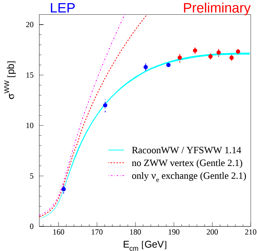
Figure 2.3: Preliminary WW cross section as function of the CM energy measured by the four LEP experiments [22]. The Monte Carlo simulations RacoonWW and YFSWW will be described in chapter 4. GENTLE [57] is a semi-analytic program.
