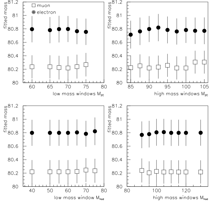
Figure 6.9: Mass windows study for the 2C mass (upper plot) and for the hadronic mass (lower plot). All the units are in \text{GeV}/c^2 .
