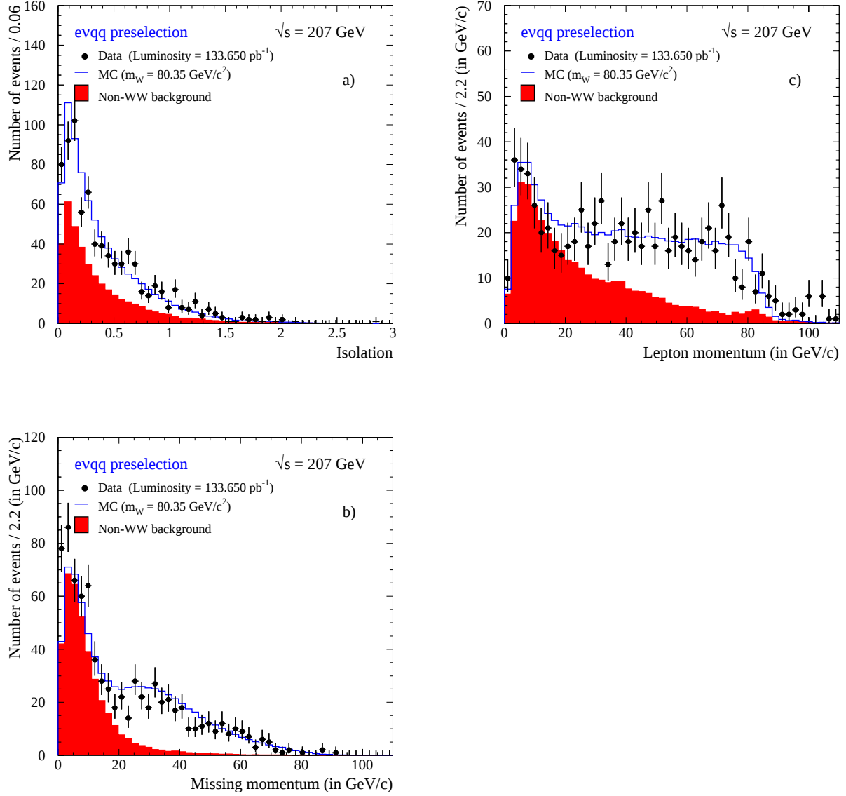
Figure 5.2: Distribution of c) the lepton momentum, b) the missing momentum and a) the isolation of the evq\bar{q} . These three variables are the input of the neural network.
