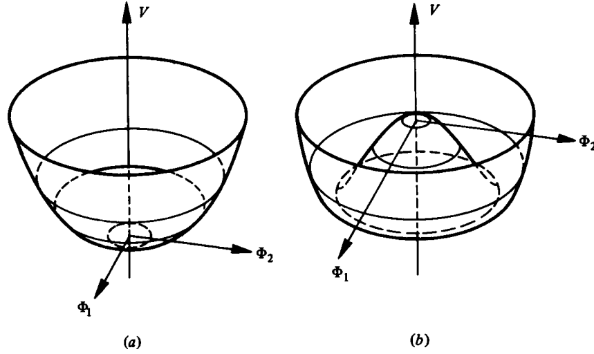
Figure 2.1: The Higgs potential V(\Phi) with: a) unique ground state corresponding to \mu^2 > 0 and b) degenerate ground state corresponding to \mu^2 < 0 (Mexican hat).
