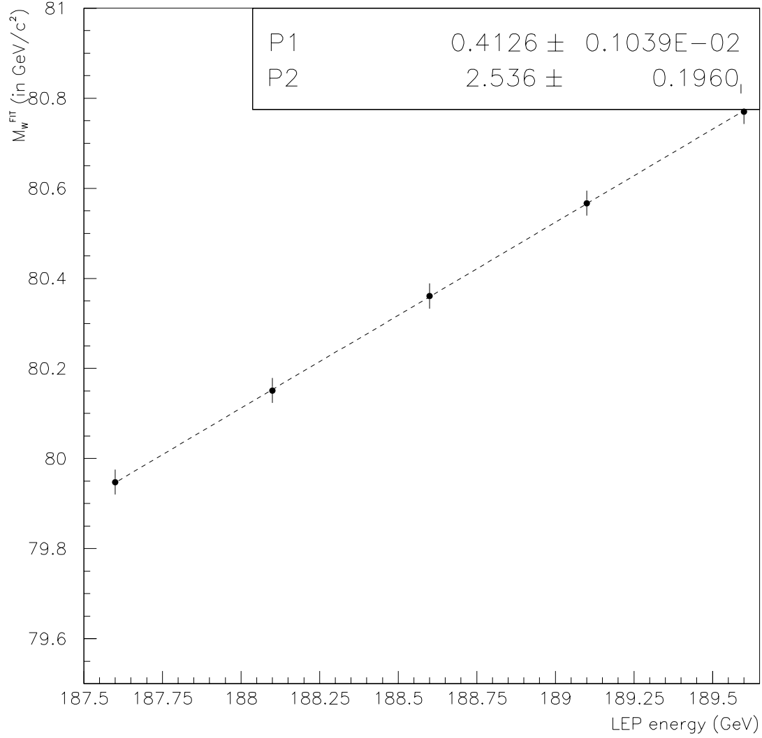
Figure 7.3: Dependence of the W mass as a function of the CM energy. This study is performed for the evq\bar{q} channel at a CM energy of 188.6 GeV. A straight line fit with slope P1 and offset P2 (in \text{GeV}/c^2 ) is also shown.
