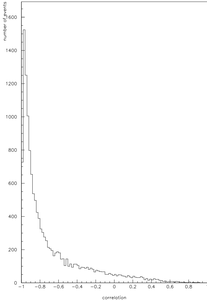
Figure 6.3: Correlation between the 1C hadronic and leptonic mass distribution.
