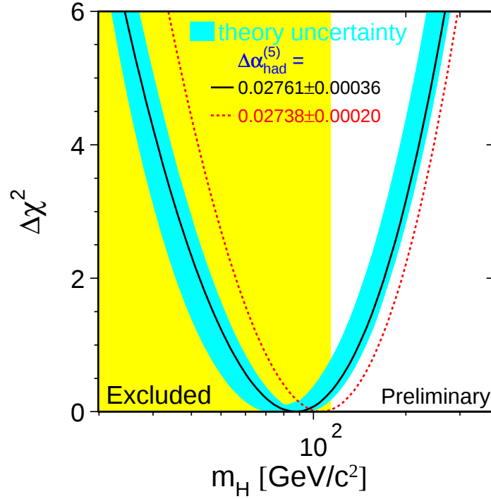
Figure 8.4: \Delta\chi^2 of the global electroweak [75] fit as a function of the Higgs boson mass. The width of the band represents the theoretical uncertainties. The left part of the plot is excluded by direct searches at 95 % Confidence Level. The dash curve is the result obtained using an other evaluation of \Delta\alpha_{\text{had}}^{(5)} which is the contribution of the light quarks to the photon vacuum polarisation ([77] and [78]) .
