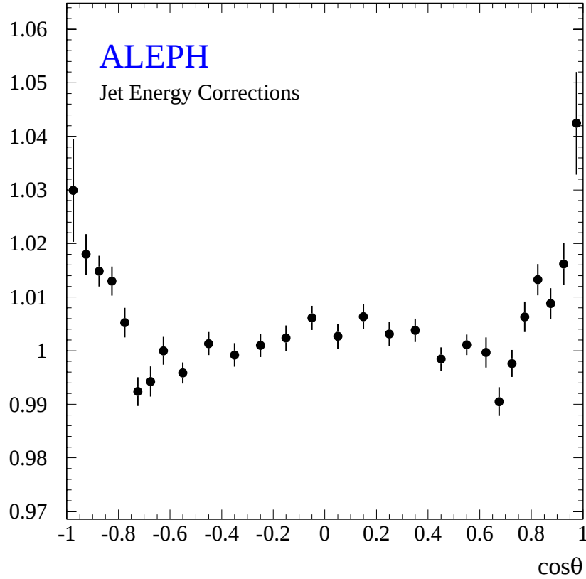
Figure 5.1: The jet energy corrections ( Ratio = \frac{(E_{jet}/E_{beam})_{data}}{(E_{jet}/E_{beam})_{MC}} ) for the year 1998 as a function of the polar angle [19].
