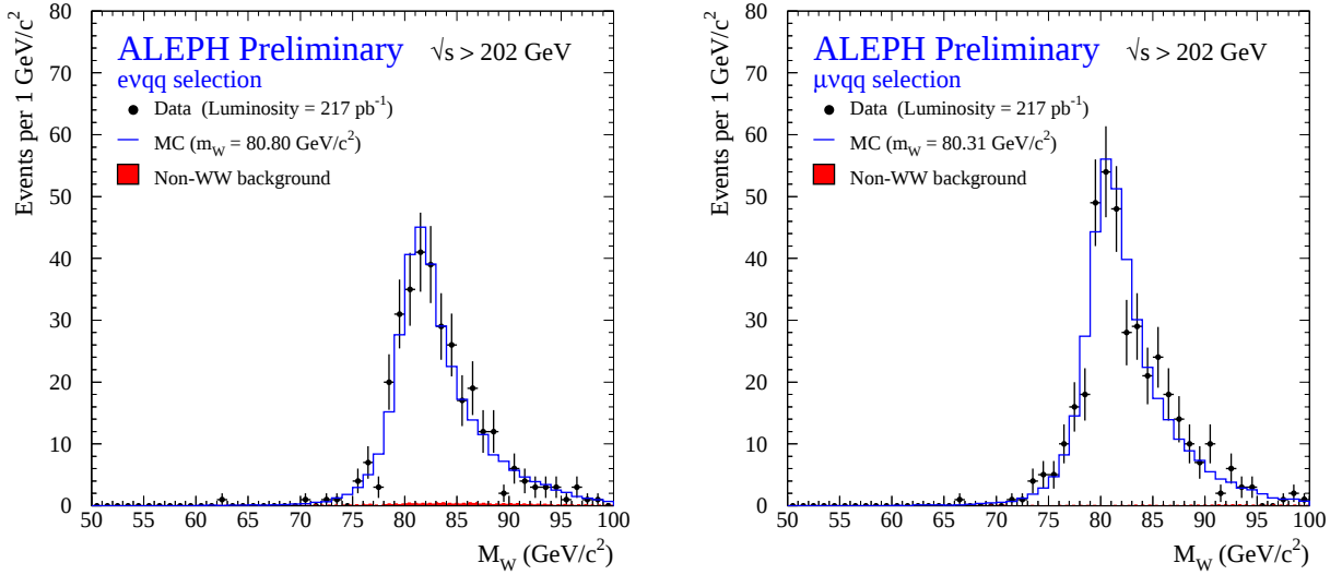
Figure 6.8: e\nu q\bar{q} and \mu\nu q\bar{q} Invariant Mass Distributions for the data taken in 2000. The histograms represent the Monte Carlo simulation, split into non WW background and signal. The signal Monte Carlo has been weighted to the measured W mass in the data sample. The dots represent the data.
