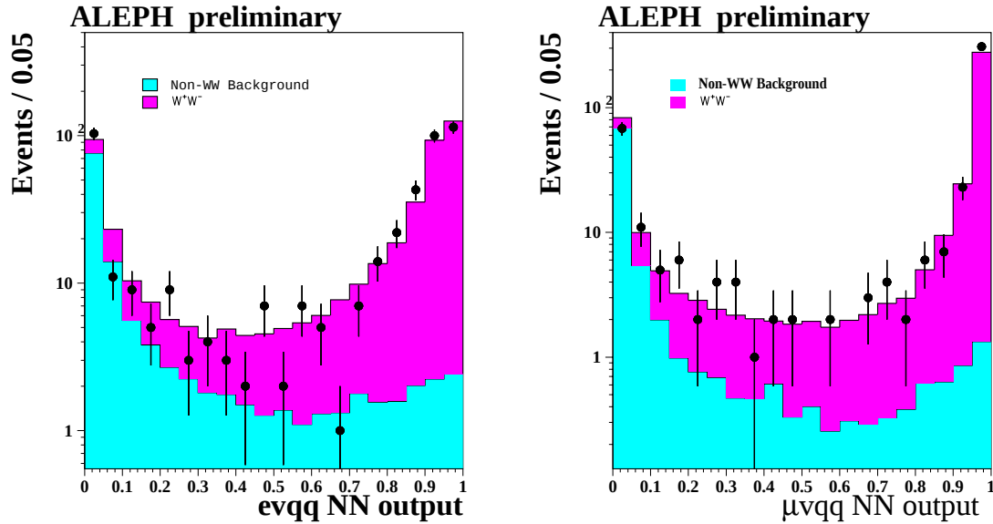
Figure 5.4: evq\bar{q} and \mu\nu q\bar{q} Neural Network output for Monte Carlo and data. An event with a probability larger than 0.6 is assumed to be a semi-leptonic event (CM energy of 207 GeV).
