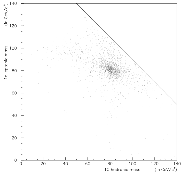
Figure 6.2: The two-dimensional mass distribution. The line represents the kinematic limit due to energy conservation.
