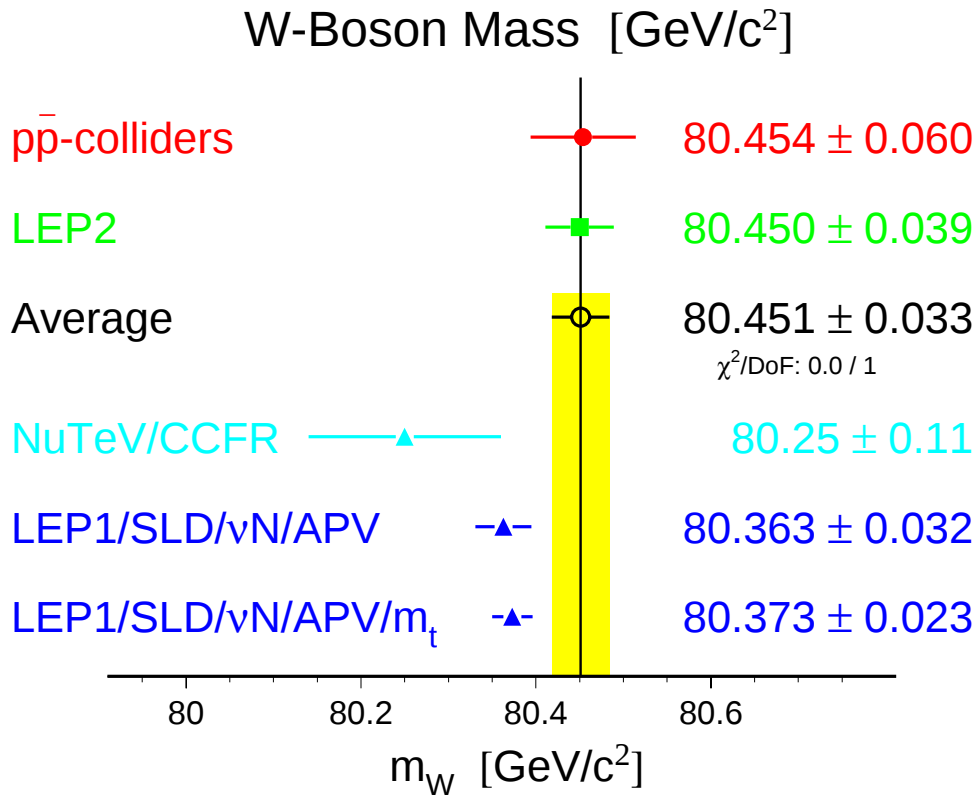
Figure 8.2: The preliminary world average W mass (summer 2001). The value p\bar{p} -collider is the combined mass from hadron machine whereas the value LEP2 is the LEP combination. The indirect W mass measurement is also shown, with and without the top mass as a fixed parameter.
