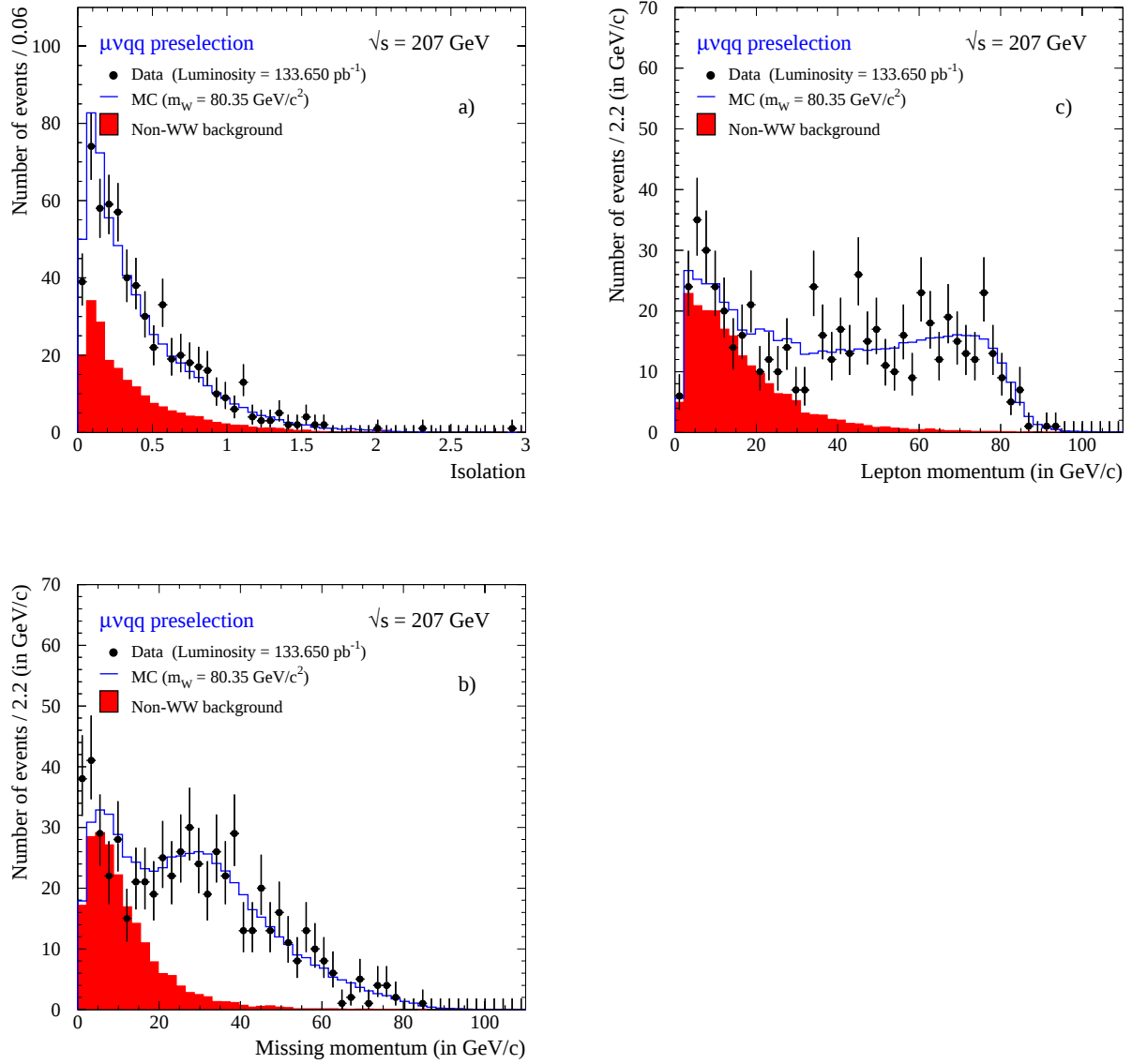
Figure 5.3: Distribution of c) the lepton momentum, b) the missing momentum and a) the isolation of the \mu\nu q\bar{q} channel. These three variables are the input of the neural network.
