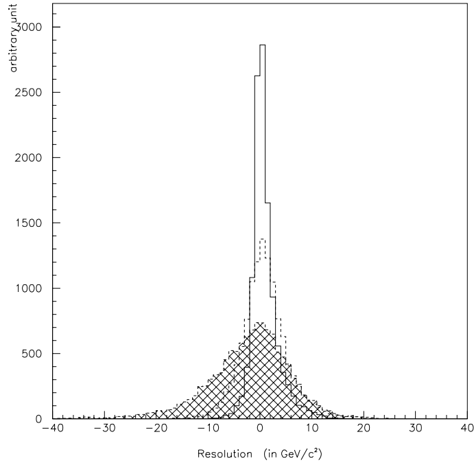
Figure 6.1: The mass resolution: for measured di-jet (hatched histogram), 1C di-jet mass (dashed line), 2C mass (solid line).
