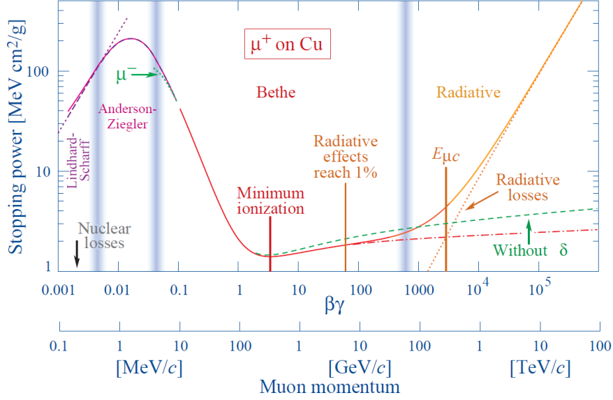
Figure 3.5: Stopping power ( = dE/dx ) for positive muons in copper as a function of \beta\gamma = p/Mc over nine orders of magnitude in momentum. The depicted effect is the fundamental working principle of ionizing particle detectors [O + 14].
