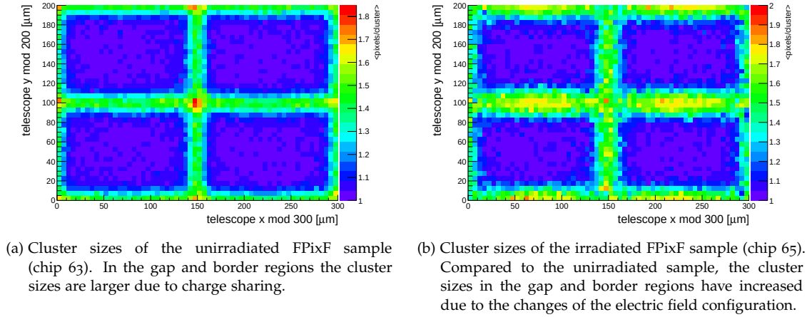
Figure 9.8: Comparison of the average cluster sizes of unirradiated and irradiated FPiXF layouts. Particles that hit the pixel cells at the implant positions mostly create single pixel clusters while hits in between two implants are more likely to share the generated charge and produce two pixel clusters. The largest clusters are thus created in the border regions where four neighboring pixels meet.
