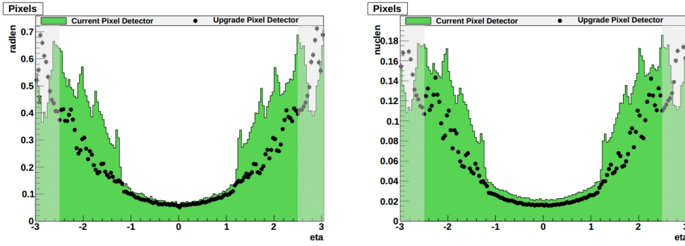
Figure 4.3: Material budget simulation of the CMS pixel detector as a function of pseudorapidity \eta . The green histogram is the data for the current pixel detector while the black points represent the new Phase I pixel detector. The left plot shows the amount of material in units of radiation length (radlen) and the right plot in units of nuclear interaction length (nuclen). The shaded bands at |\eta| \geq 2.5 denote regions outside the active tracker volume. The effort to decrease the amount of material is clearly visible in the regions above |\eta| = 1.2 from where services like electronics boards and power supply have been moved further out [DAA + 12].
