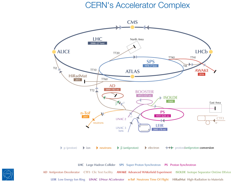
Figure 3.2: CERN's accelerator complex schematic, with the accelerator chain of the LHC (Linac2 → Proton Synchrotron Booster (PSB) → Proton Synchrotron (PS) → Super Proton Synchrotron (SPS) → LHC) and experiments shown. Taken from Ref. [37].
