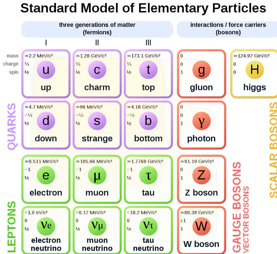
Figure 2.1: Elementary particles of the Standard Model. Quarks and leptons, collectively referred to as fermions (spin quantum number is 1/2 ) constitute matter. Interactions between particles are mediated by bosons: gluons for strong interaction, Z and W bosons and the photon for the electroweak interaction, and the Higgs boson. All known bosons are vector particles (spin 1), except the Higgs, which is the only scalar boson (spin 0). Taken from Ref. [12].
