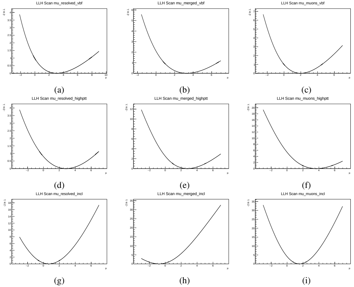
Figure B.1: Profile of the negative log-likelihood ratio as a function of signal strength \mu (main result).
