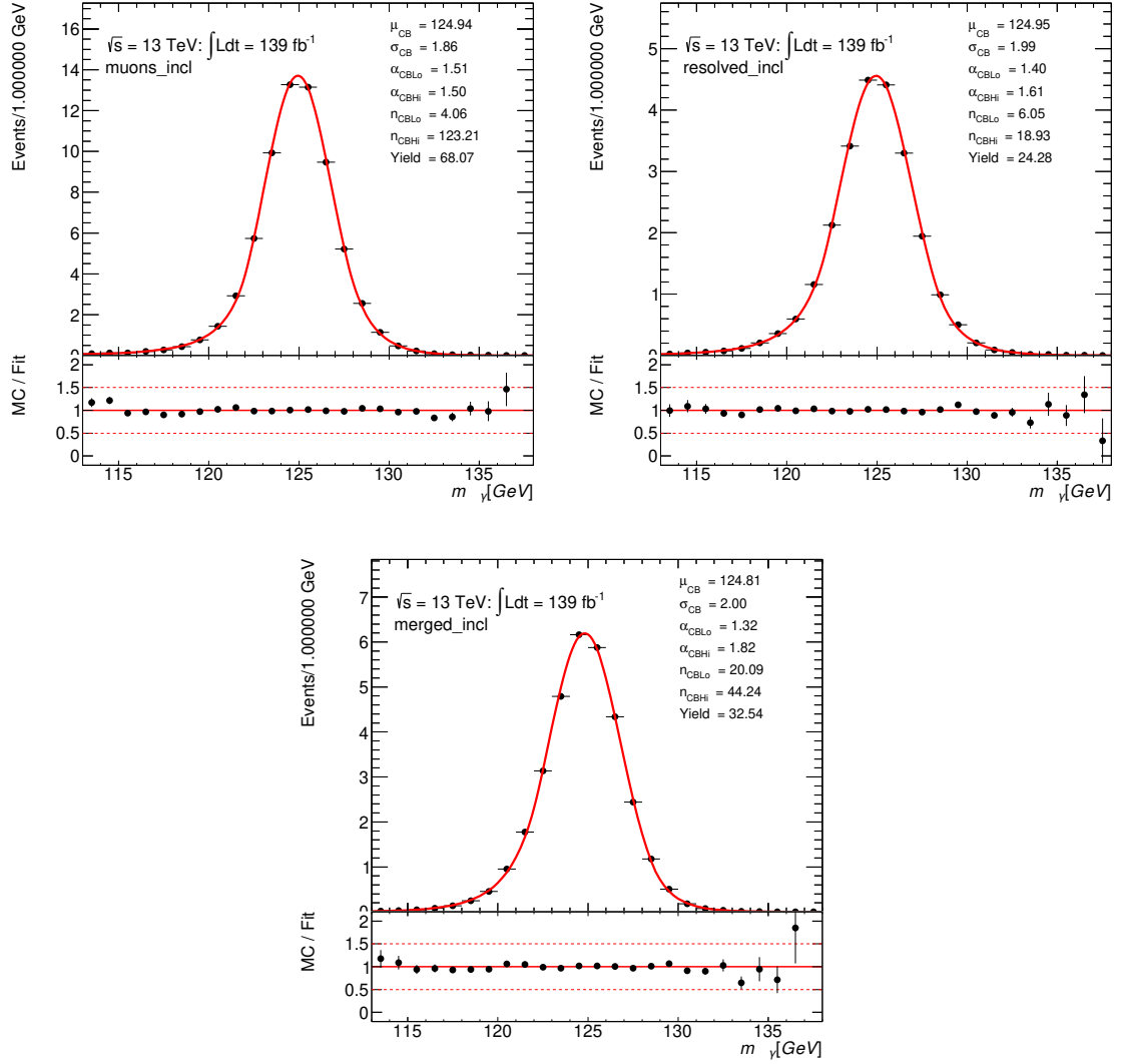
Figure A.1: Signal fit in low- p_{T}^{\ell\ell\gamma} analysis categories using a double-sided Crystal Ball function.
