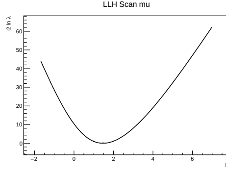
Figure B.1: Profile of the negative log-likelihood ratio as a function of signal strength \mu (main result).
