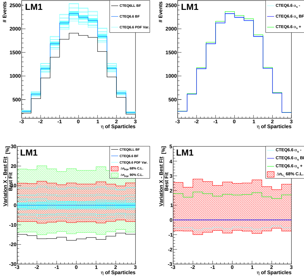
Figure D.11: \eta distribution of the produced particles for the estimation of PDF and \alpha_s uncertainties with sets from CTEQ6.6. Legend entries labeled “BF” refer to the best fit member of the PDF set and “PDF Var.” stands for members where fit parameters have been varied.
