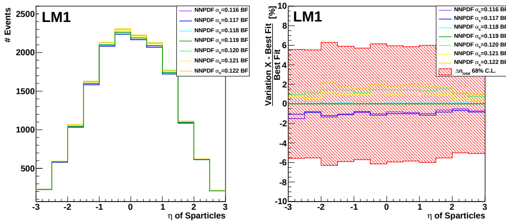
Figure D.13: \eta distribution of the produced particles for the estimation of combined PDF and \alpha_s uncertainties with sets from NNPfDf.
