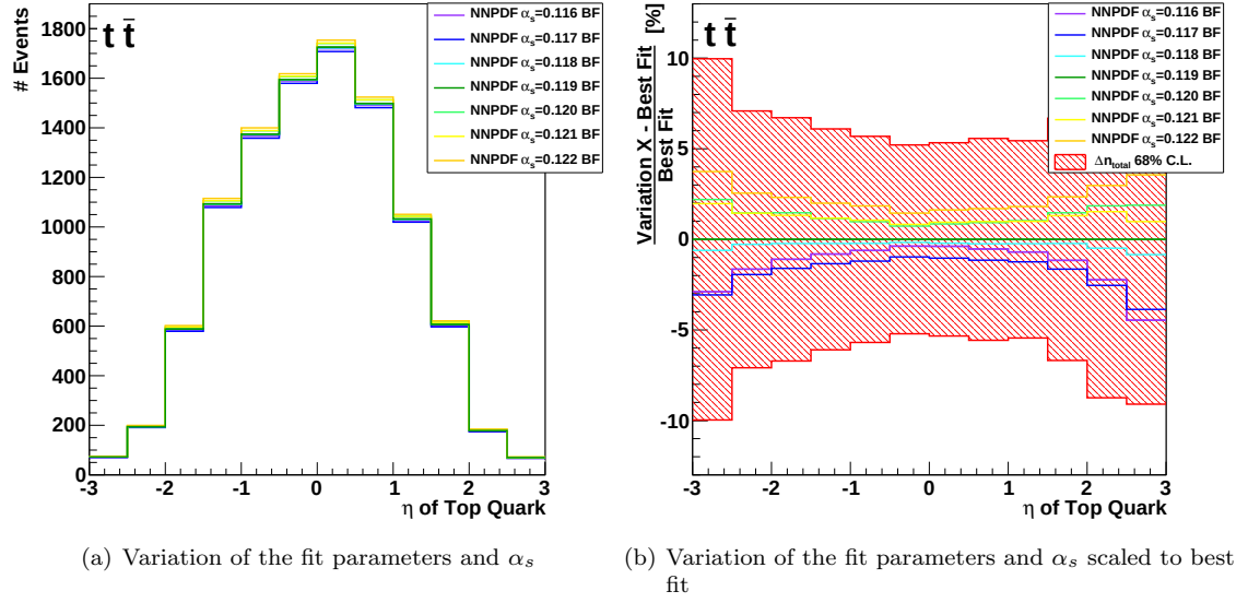
Figure 5.27: \eta distribution of top quark for estimation of PDF and \alpha_s uncertainties with sets from NNPDF.
