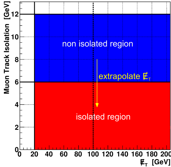
Figure 5.14: The data-driven method for QCD background in short.
