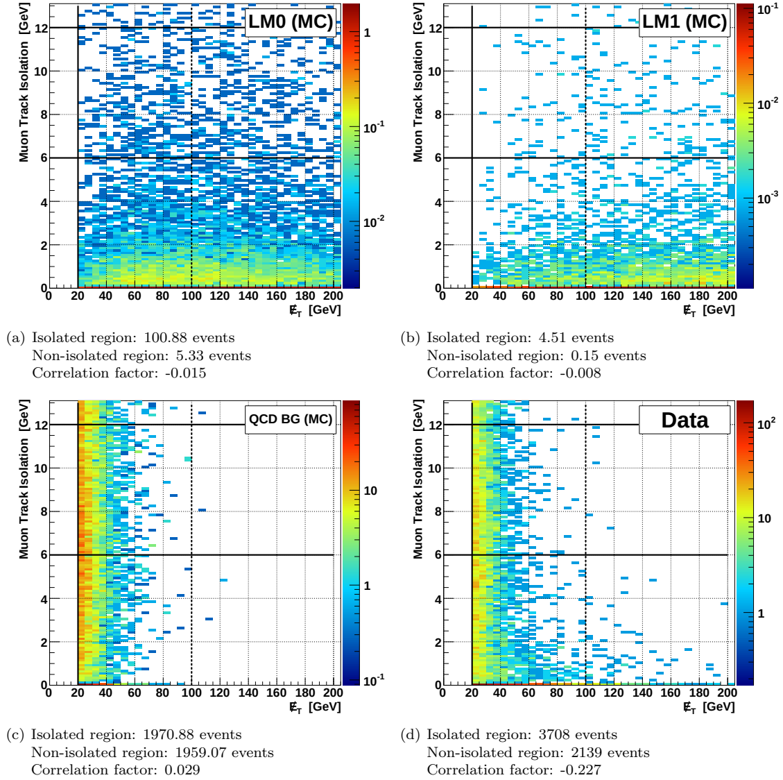
Figure 5.15: The four diagrams show the distribution of the LM0, LM1 and QCD background Monte Carlo samples and the data in the \cancel{E}_T\text{--TrkIso}^\mu plane. The number of events for the isolated and non-isolated region are given in the caption of each diagram, along with the correlation factor between both variables.
