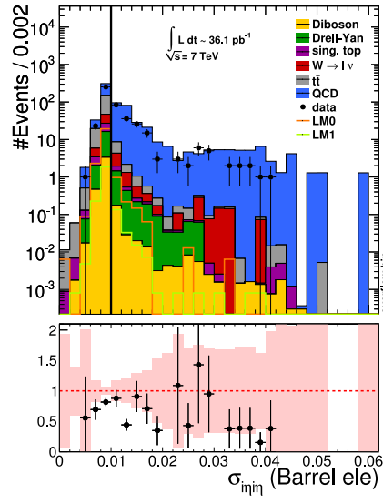
(a) Spread in \eta of energy in a 5x5 cluster (cut: \sigma_{i\eta i\eta} < 0.01 )
