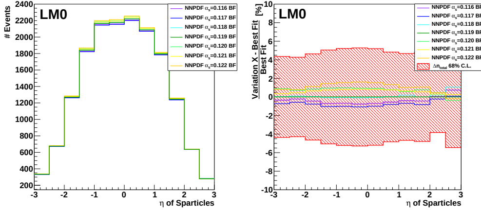
Figure D.10: \eta distribution of the produced particles for the estimation of combined PDF and \alpha_s uncertainties with sets from NNPDF.
