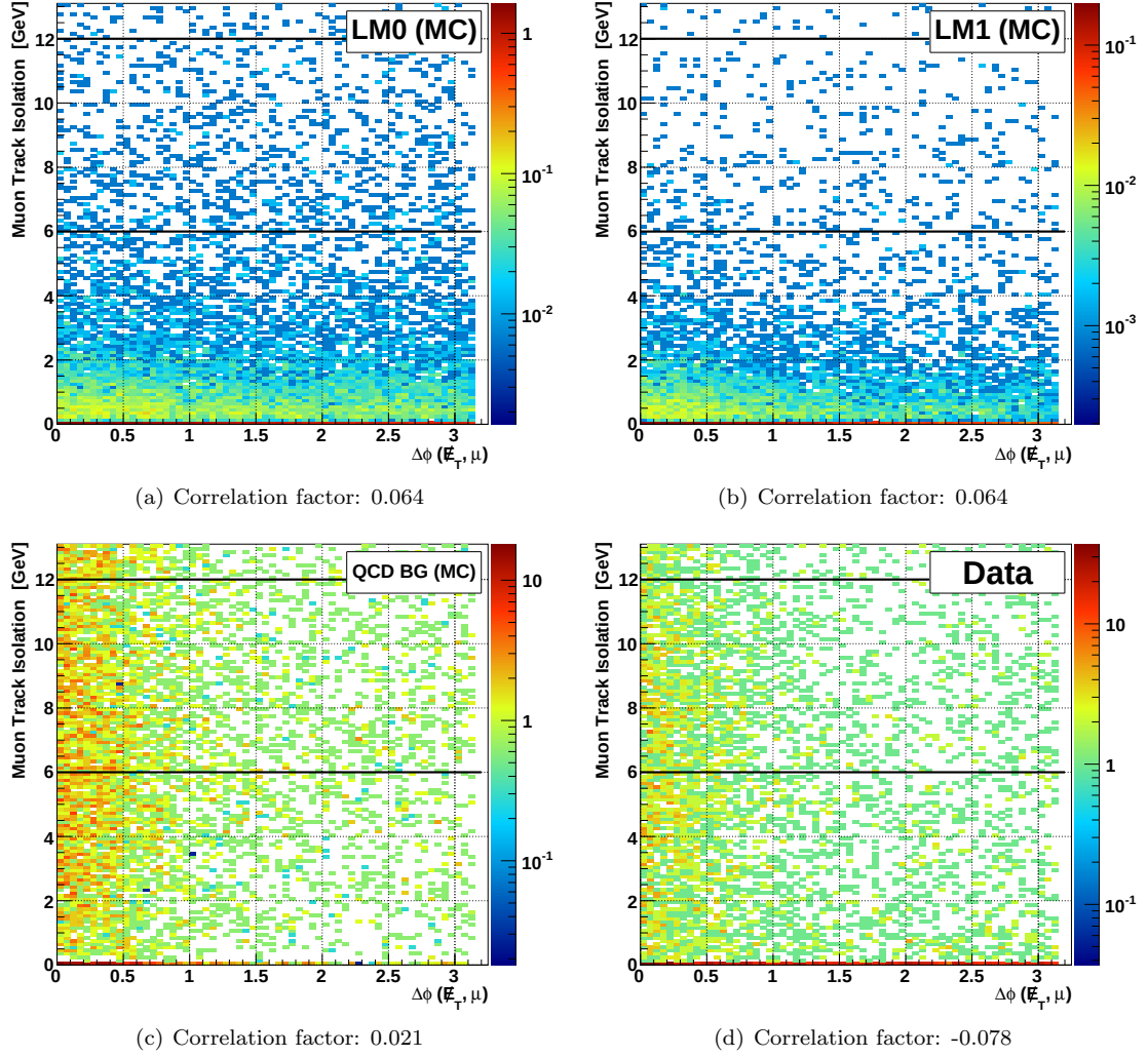
Figure 5.16: The four diagrams show the distribution of the LM0, LM1 and QCD background Monte Carlo samples and the data in the \Delta\phi(\ell_T, \mu) – \text{TrkIso}^\mu plane. The correlation factor between both variables is given in the caption of each diagram.
