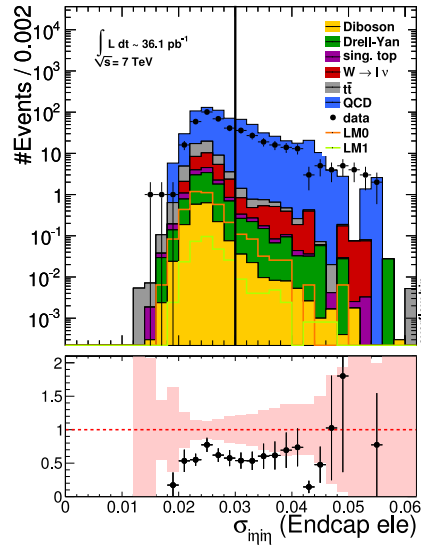
(a) Spread in \eta of energy in a 5x5 cluster (cut: \sigma_{\eta|\eta} < 0.03 )
