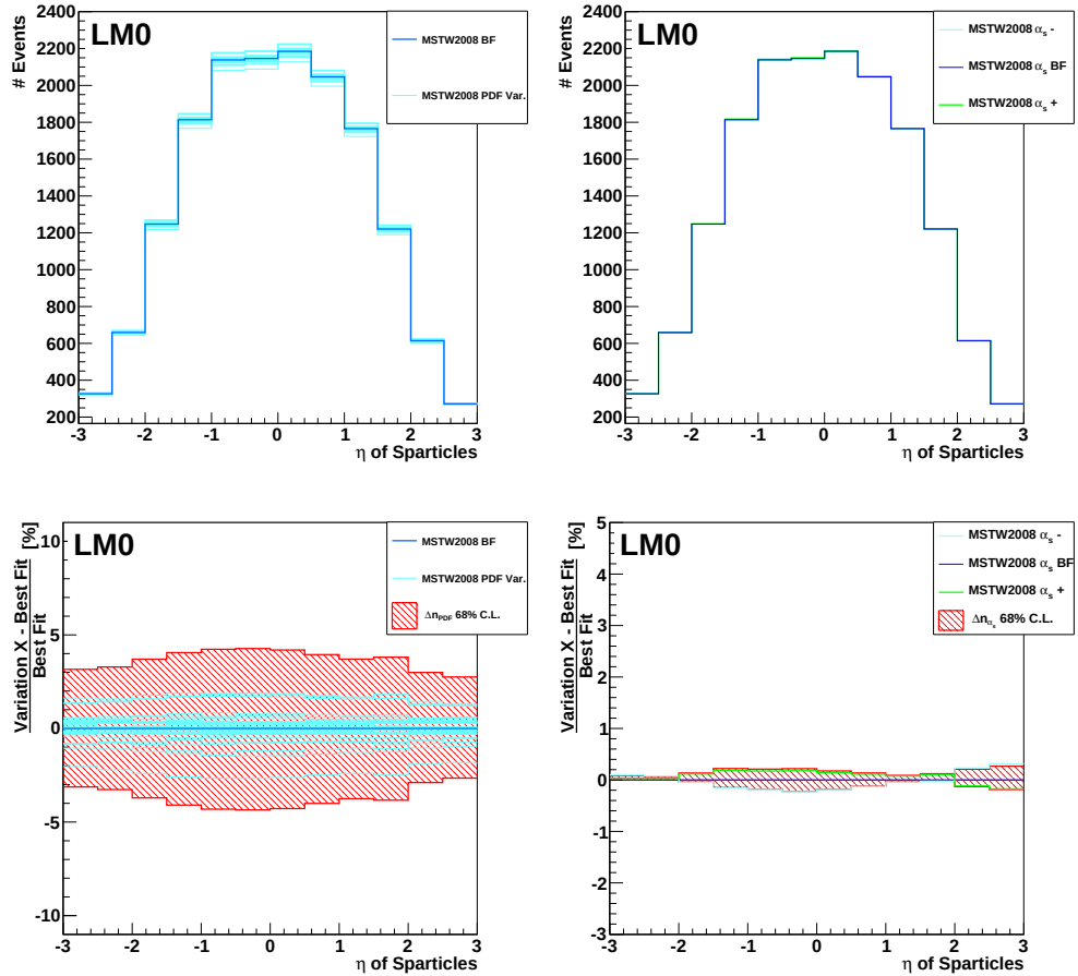
Figure D.9: \eta distribution of the produced sparticles for the estimation of PDF and \alpha_s uncertainties with sets from MSTW2008. Legend entries labeled “BF” refer to the best fit member of the PDF set and “PDF Var.” stands for members where fit parameters have been varied.
