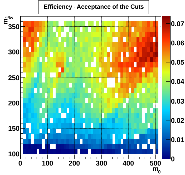
Figure 5.29: Scan of the mSUGRA plane with \tan\beta=3 , A_0=0 , \mu > 0 . The efficiency times acceptance of the analysis cuts is shown, where blue bins correspond to a low efficiency and red bins represent higher values.
