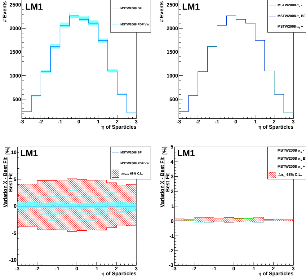
Figure D.12: \eta distribution of the produced particles for the estimation of PDF and \alpha_s uncertainties with sets from MSTW2008. Legend entries labeled “BF” refer to the best fit member of the PDF set and “PDF Var.” stands for members where fit parameters have been varied.
