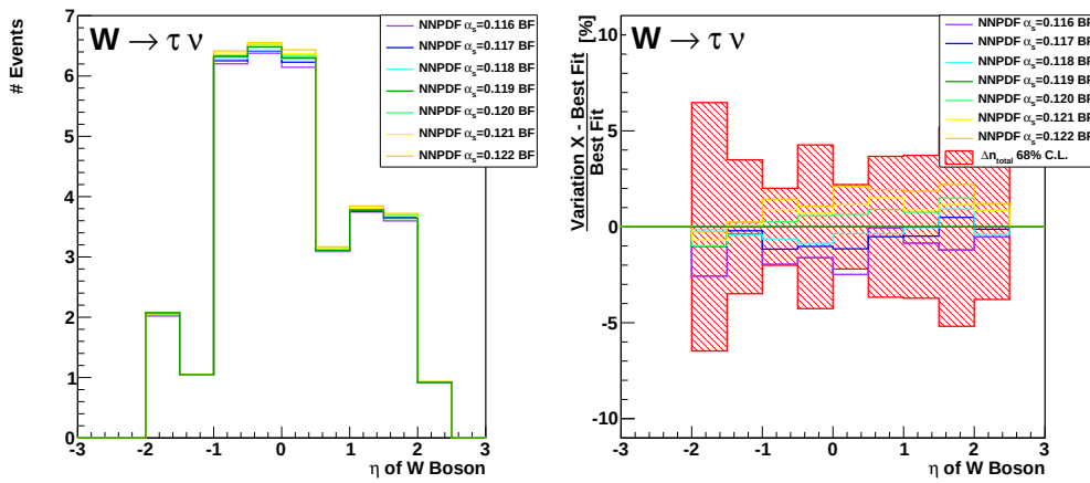
Figure D.7: \eta distribution of W boson for the estimation of combined PDF and \alpha_s uncertainties with sets from NNPfDf.
