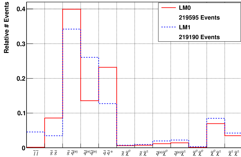
Figure 3.3: Comparison of LM0 and LM1 production channels used in this thesis. The histograms have been normalized to area, the absolute number of generated events is given in the legend.
