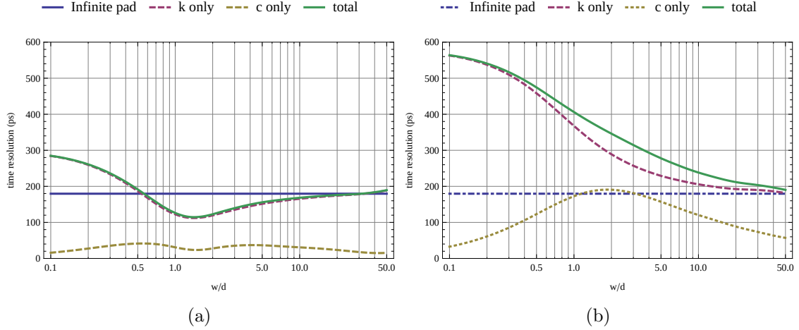
Figure 5.15.: Time resolution for values of d = 200 \mu\text{m} and V = 200 \text{ V} as a function of the pixel size w assuming the Landau theory for the charge deposit. The "c only" curve refers to the effect from a uniform line charge. In 5.15a the electrons move towards the pixel while in 5.15b the holes move towards the pixel. From [96].
