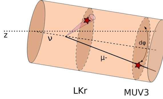
Figure 4.17.: Schematic of the implementation of the d\phi_{\text{LKr-MUV3}} cut. The direction of the neutrino allows building a cylindrical coordinates reference frame in which the \nu_\mu direction is the z axis.
