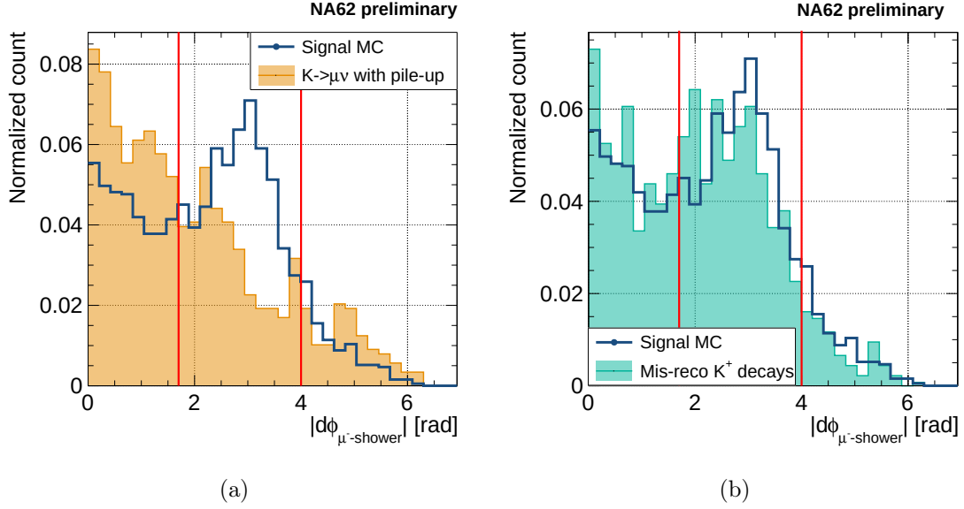
Figure 4.16.: Normalized distributions of the variable d\phi_{LK\tau-MUV3} for signal (blue line) and background of overlaid K\mu\nu (4.16a) (orange fill), and for signal (blue line) and background of mis-reconstructed K^+ decays (4.16b) (green fill). The red solid lines represent the cuts.
