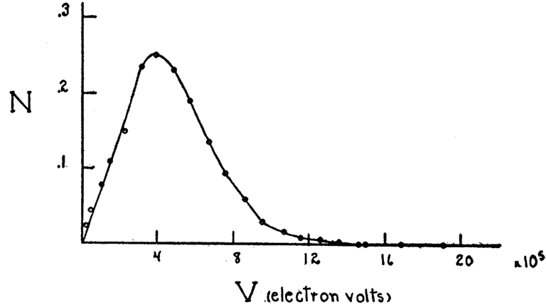
Figure 1.1.: Energy spectrum of the emitted electron in a \beta decay experiment. From [102].
