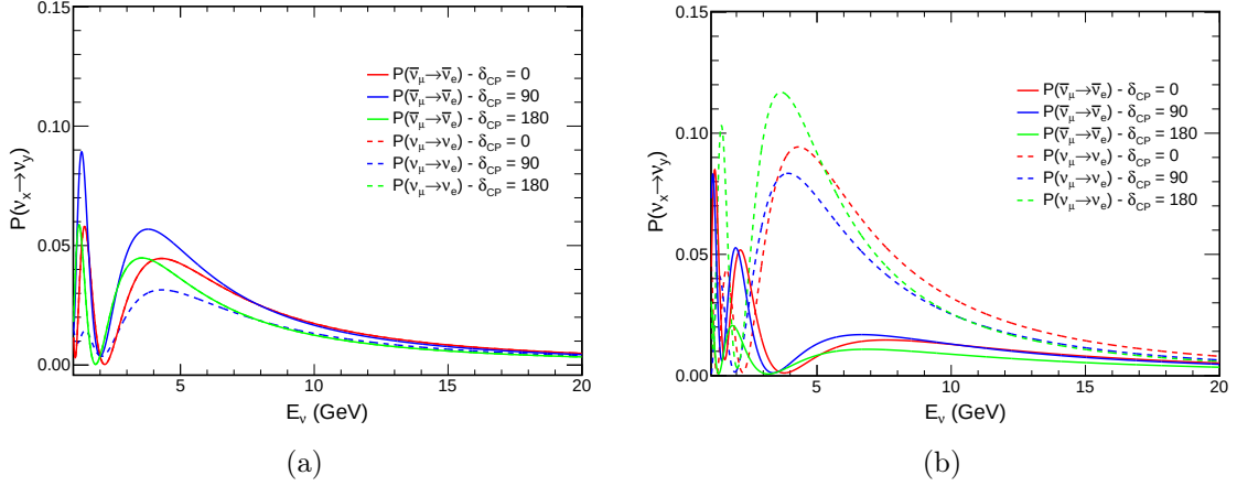
Figure 1.6.: Oscillation probability for CP-effect sensitive channel \bar{\nu}_\mu \rightarrow \bar{\nu}_e as function of the neutrino energy in vacuum (1.6a) and in matter (1.6b) for a baseline of 2000 km and for different values of \delta_{CP} , reported in degrees in the legend. The oscillation probabilities are computed with the OscProb software package using the oscillation parameters in Table 1.1.
