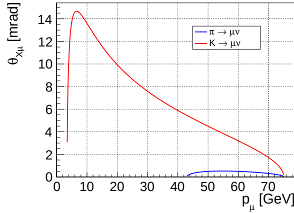
Figure 4.25.: Opening angle between muon daughter and mother for K^+ \rightarrow \mu^+ \nu_\mu decay (red) and for \pi^+ \rightarrow \mu^+ \nu_\mu decay (blue) as function of the \mu^+ momentum from simulation.
