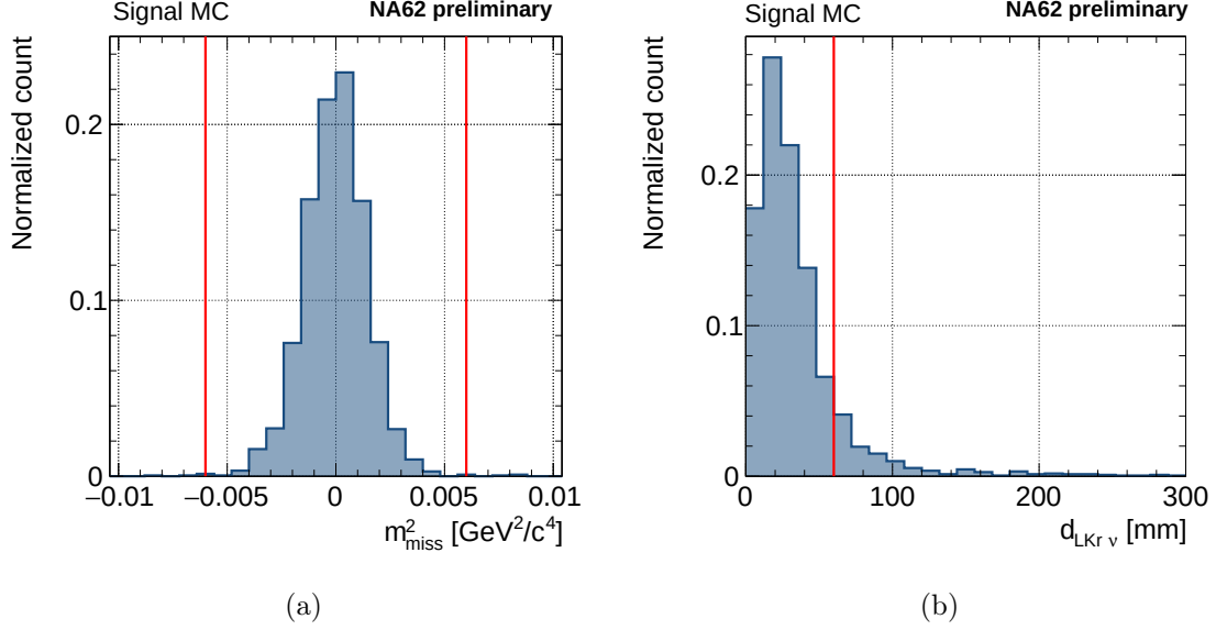
Figure 4.2.: Distribution of m_{\text{miss}}^2 (4.2a) and of d_{\text{LKr } \nu} (4.2b) for the simulated signal. The red solid lines represent the cuts separating the signal region from the control region.
