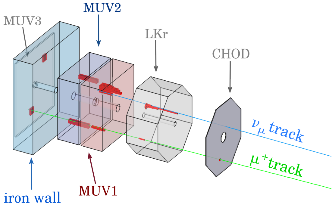
Figure 4.36.: Annotated event display for Event A. The 3-dimensional volumes represent the active volumes of the downstream detectors. The green line is the track of the \mu^+ ; the blue line represents the neutrino trajectory reconstructed from the K^+ and \mu^+ . The red boxes represent the activity in the detector. For the LKr, MUV1 and 2 the length of the box is the normalized energy deposit in each cell.
