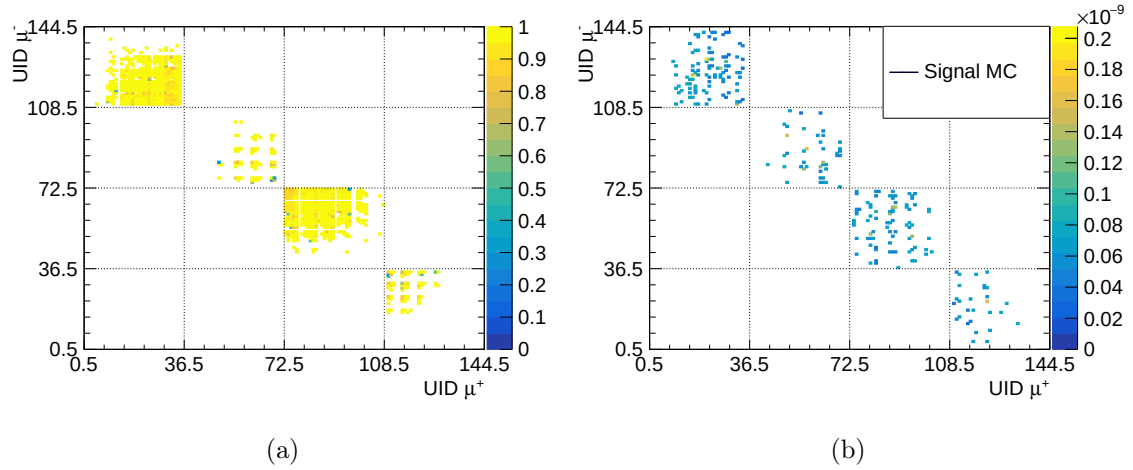
Figure 4.27.: 4.27a: Efficiency map of the MQQX condition. 4.27b: Spatial distribution of signal events from the MC passing the signal selection.
