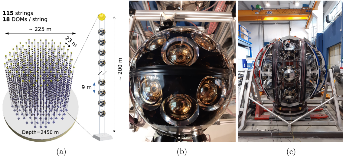
Figure 1.10.: 1.10a: Schematic of the layout of the completed KM3NeT/ORCA site, from [16]. 1.10b: a DOM being calibrated, photo taken in the CPPM assembly lab. 1.10c: photo of a launch vehicle deployment that exploits the unfurling of the string, taken in the CPPM assembly lab.
