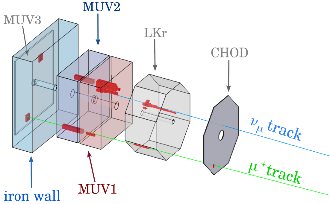
Figure 4.37.: Annotated event display for Event B. The 3-dimensional volumes represent the active volumes of the downstream detectors. The green line is the track of the \mu^+ ; the blue line represents the neutrino trajectory reconstructed from the K^+ and \mu^+ . The red boxes represent the activity in the detector. For the LKr, MUV1 and 2 the length of the box is the normalized energy deposit in each cell. Apart from the neutrino cluster, some extra low energy hits have been found in LKr.
