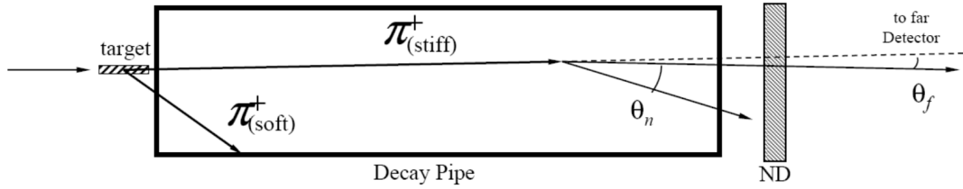
Figure 2.4.: Not-to-scale demonstration of the solid angle differences in a two-detector neutrino experiment. From [67].
