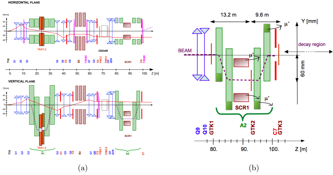
Figure 3.2.: 3.2a: Upstream region from T10 target to decay volume with both horizontal and vertical views, for Run1. In each view, the solid line corresponds to the trajectory of a particle leaving the target from the centre at nominal momentum and at the angle indicated. The dashed line indicates the trajectory of an initially on-axis 75 GeV/c momentum particle. 3.2b: Schematic description of the beam spectrometer in the second achromat (A2). Muons are swept away by the scraper SCR1. From [81].
