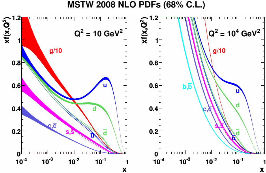
Figure 2.2.: Parton distribution functions as a function of momentum fraction x for two momentum transfer scales Q^2 = 10 \text{ GeV}^2 (left) and Q^2 = 10^4 \text{ GeV}^2 (right), provided by the PDF fitting group MSTW [32].
