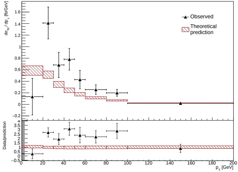
FIGURE 6.13: The measured differential cross-section in p_T , in the region 0–200 GeV. The measurement from data is shown by the black points, and the error bars on each point show the combined statistical and systematic uncertainty. The shaded red area indicates the theoretical prediction described in section 6.5. The uncertainty on the theoretical prediction is indicated by the shaded area.
