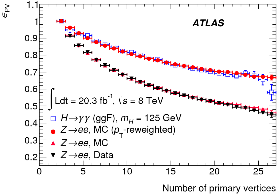
FIGURE 6.4: This figure[97] shows the efficiency, \varepsilon_{PV} , of the neural network algorithm determining a primary vertex within 0.3 mm of the true primary vertex, as determined from studies performed on MC data. The unfilled blue squares show \varepsilon_{PV} for simulated gluon-gluon fusion events with a Higgs boson of mass m_H = 125 GeV decaying to two unconverted photons. The performance of the algorithm on Z \rightarrow e^+e^- events, with electron tracks removed, is shown for both data and MC as black and red triangles respectively. The red circles illustrate the performance on the same simulated Z \rightarrow e^+e^- sample with reweighting applied to reproduce the harder p_T distribution of the simulated H \rightarrow \gamma\gamma events.
