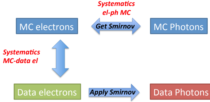
FIGURE 5.5: Diagram representing which samples are involved in each stage of the Smirnov transformation method of electron extrapolation.
