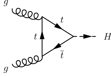
FIGURE 2.3: This Feynman diagram shows the production of a Higgs boson via gluon-gluon fusion, the dominant production mode according to SM predictions.
