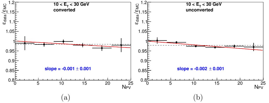
FIGURE 5.32: The measured ratio \varepsilon_{\text{data}}/\varepsilon_{\text{MC}} as a function of N_{\text{PV}} for converted ((a)) and unconverted ((b)) photons with p_T in the range 10 \text{ GeV} < p_T < 30 \text{ GeV}
