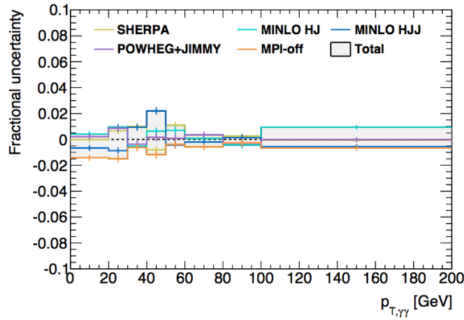
FIGURE 6.9: The fractional difference between the nominal correction factors and those obtained with alternate MC samples[2]. The envelope of these variations is assigned as a systematic uncertainty on the correction factors.
