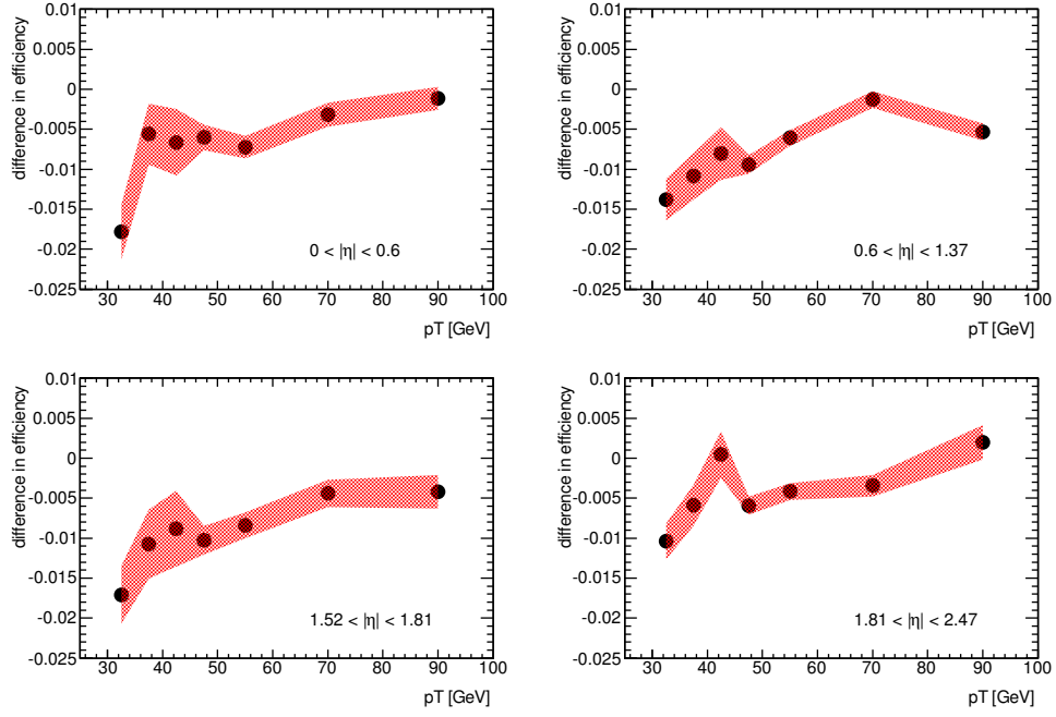
FIGURE 5.7: The closure test ( \varepsilon_{\text{MC,photon}} - \varepsilon_{\text{MC,electron,Smirnov}} ) for converted photons, in four regions of |\eta| . The shaded area indicates the combined statistical uncertainty resulting from the sizes of the photon and electron MC samples.
