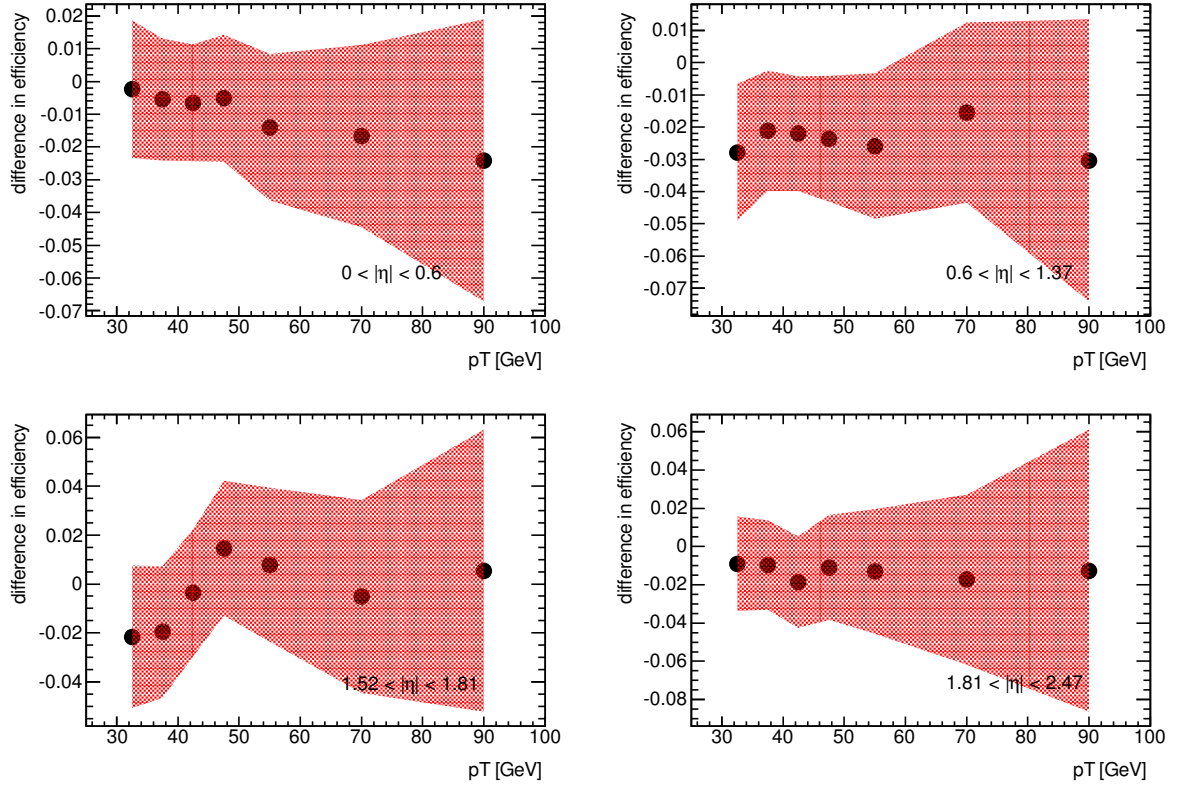
FIGURE 5.22: A comparison between data and FPMC efficiency measurements in the form of the absolute efficiency difference for unconverted photons ( \varepsilon_{data} - \varepsilon_{MC} ).
