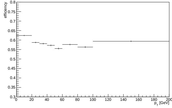
FIGURE 6.6: The efficiency of each p_T bin. The error bars indicate the statistical uncertainty resulting from the size of the MC sample.
