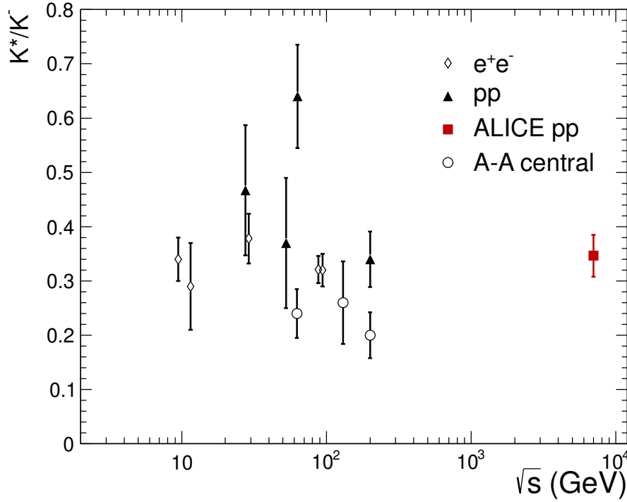
Figure 2.5: The ratio of K^{*0}/K^- for e^+ + e^- , p+p, and central A+A collisions as a function of collision energy. Figure taken from Ref. [58].
