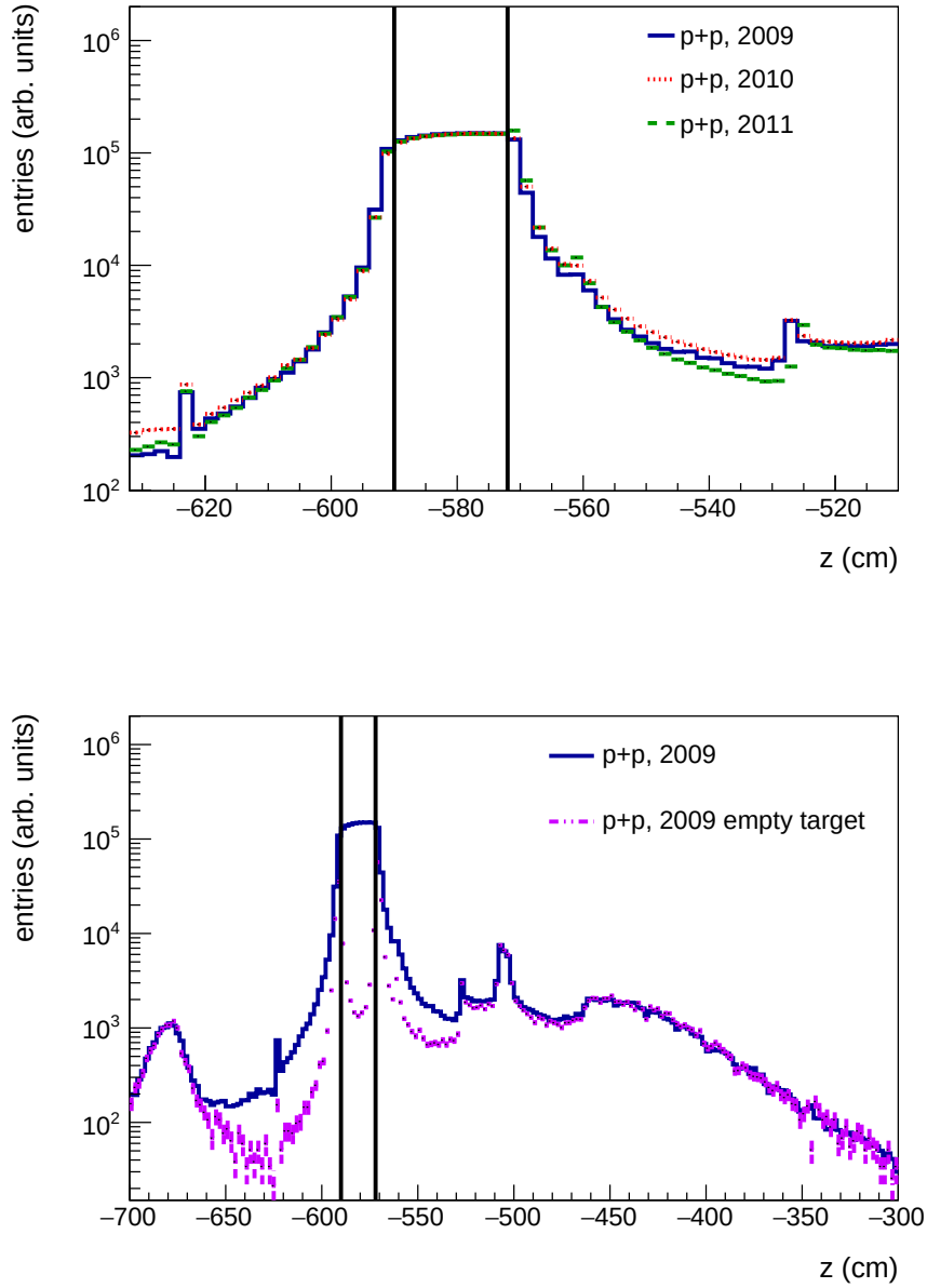
Figure 4.1: Top: Distributions of the z -coordinate of the reconstructed interaction vertex ( z ) for events recorded with the target inserted (2009, 2010, and 2011 data). Histograms are normalized to the same integral in the range -590 < z < -572 cm. Bottom: Distributions of the z -coordinate of the reconstructed interaction vertex for target-inserted (solid histogram) and target-removed (dash-dotted histogram) 2009 data. Histograms are normalized to the same integral in the range -450 < z < -300 cm. All event cuts were applied (see Sec. 4.2) with exception of cut (ii) and (v). Black vertical lines indicate the cuts used for the analysis (see Sec. 4.2).
