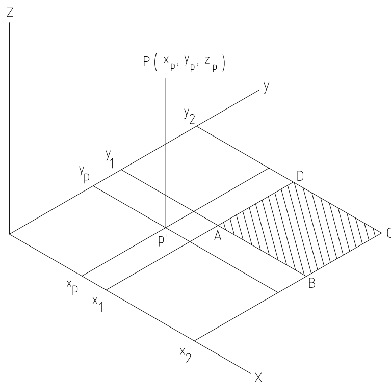
Figure 3.11: The geometry in which equation 3.1 applies. The hatched rectangular region, ABCD , defines the solid angle, d\Omega , with respect to the point P(x_p, y_p, z_p) .
