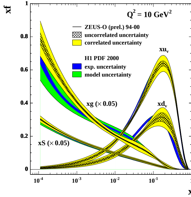
Figure 3.1.: Parton density functions. Here a comparison of ZEUS and H1. Shown are the density of u and d valence quarks, gluons and sea quarks. [26]
