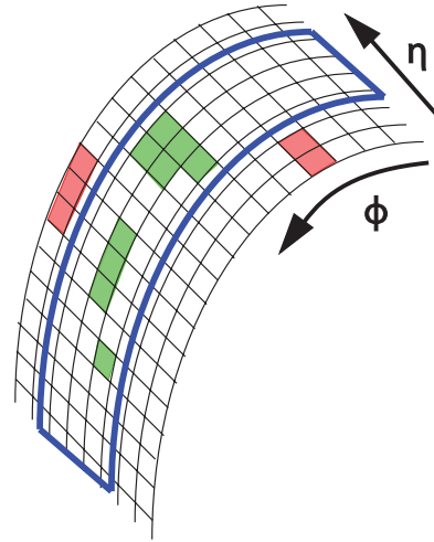
Figure 6.9.: The energy depositions corresponding to one electron (green) can be separated in \phi due to several effects. The super cluster algorithm is used to combine the energy of several clusters into a supercluster, here indicated by the blue line. [78]
