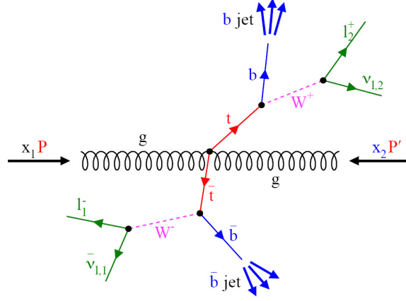
Figure 4.4.: The dileptonic decay of t\bar{t} -pairs is characterized by two b -quarks, two charged leptons and two neutrinos in the final state. In the detector the b -quarks will be visible as b -jets and together with the two charged leptons, this decay leaves a clear experimental signature.
