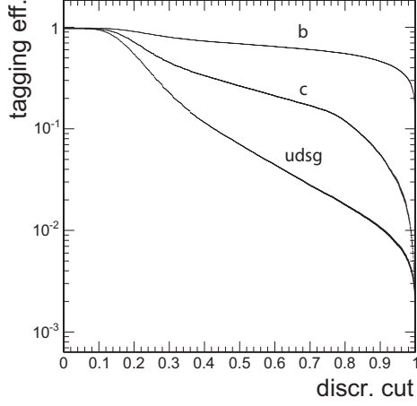
Figure 6.16.: The efficiency of the b tagging algorithm for different flavours and discriminator cuts. It was created using QCD events with 30 \text{ GeV} < p_T < 200 \text{ GeV} and |\eta| < 2.4 . [87]
