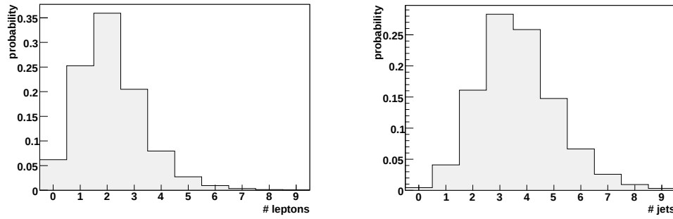
Figure 7.2.: Number of leptons (left) and jets (right) after reconstruction. The proper leptons and jets have to be selected.
